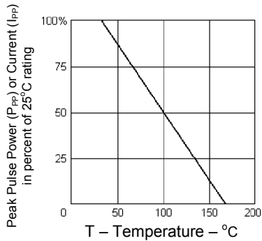
FIGURE 3 DERATING CURVE
