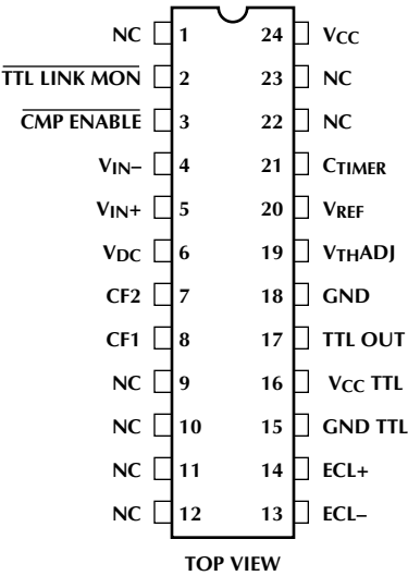
ML4624 24-Pin Narrow DIP
