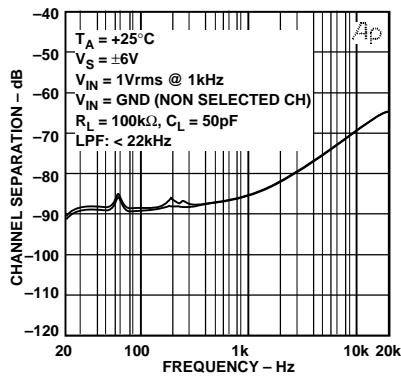
Figure 6. Channel Separation vs. Frequency
