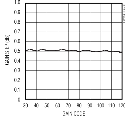
GAIN STEP vs. GAIN CODE LOW-NOISE MODE
