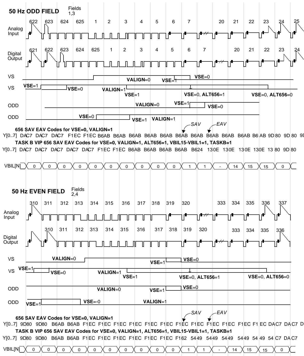
Figure 37. Vertical Timing For 50 Hz Video
