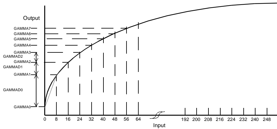
Figure 33. Gamma LUT Programming
