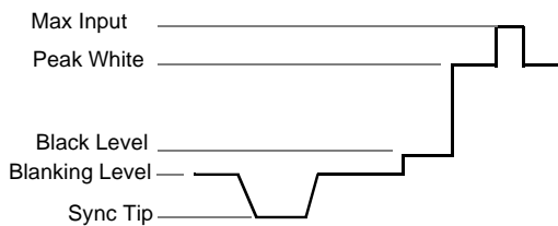
Figure 12. Luminance Signal
