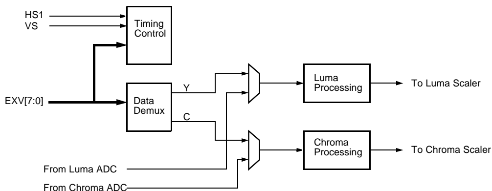
Figure 3. 8-bit YCbCr Input Data Path
