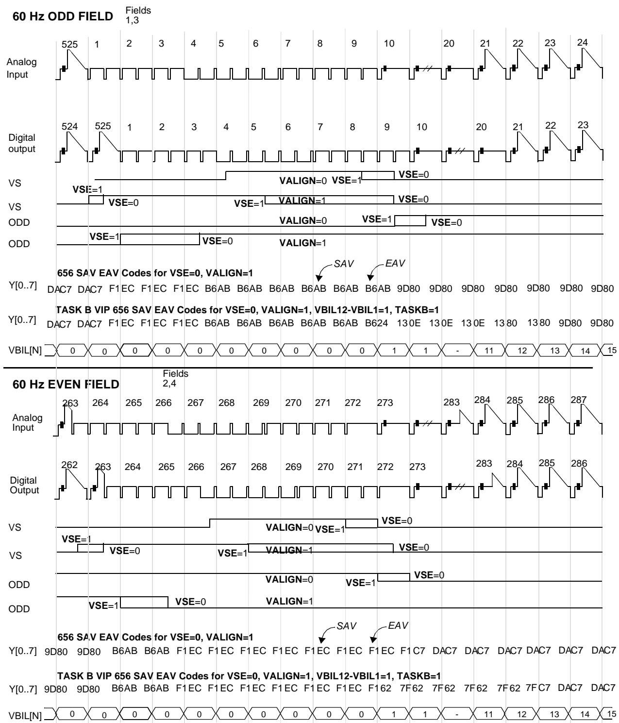
Figure 36. Vertical Timing for 60 Hz Video
