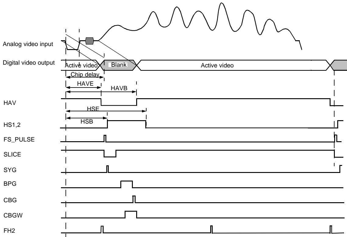
Figure 6. Approximate Locations for the Horizontal Timing Signals
