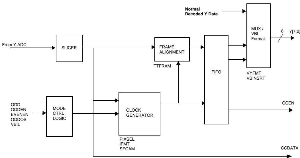
Figure 30. VBI Decoder Block Diagram
