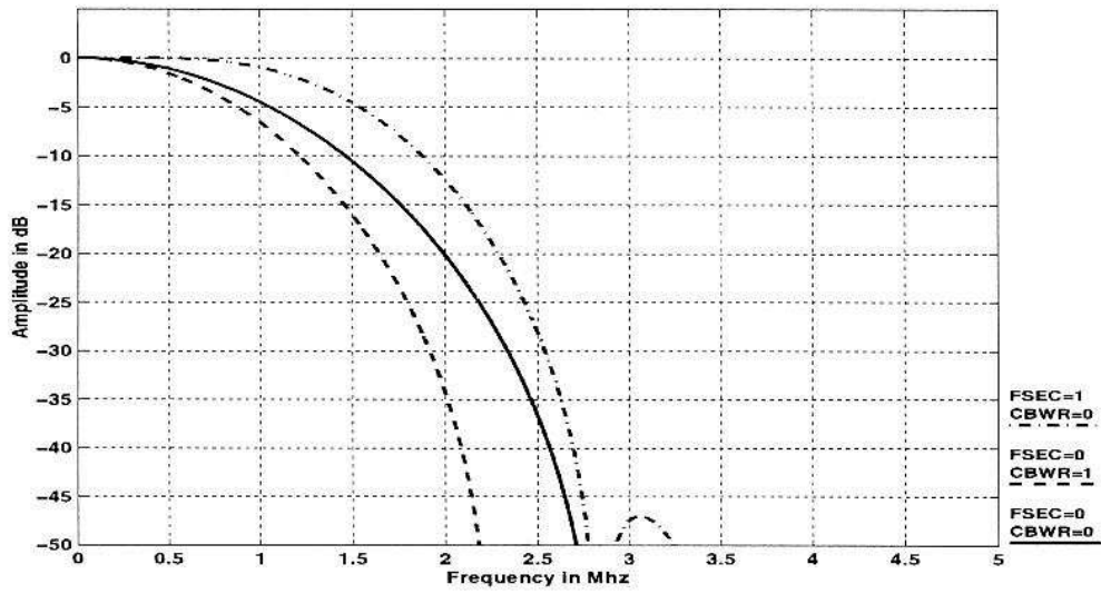
Figure 19. Chroma Low Pass Filter Frequency Response
