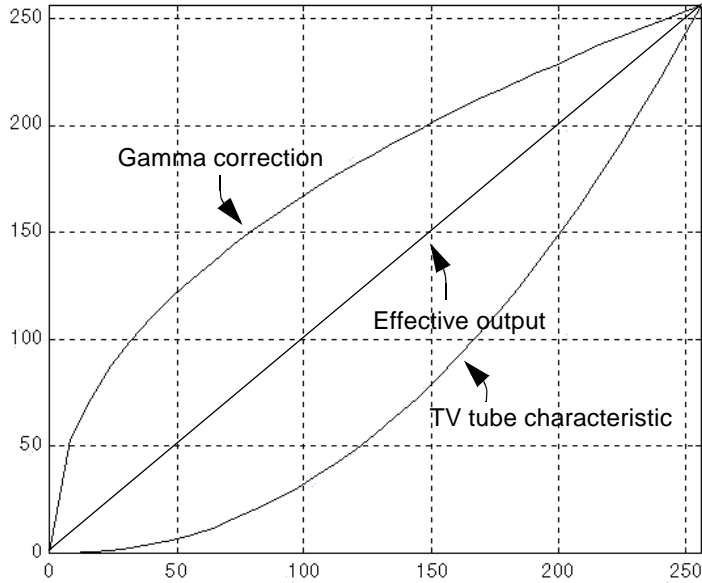
Figure 32. RGB Gamma Correction
