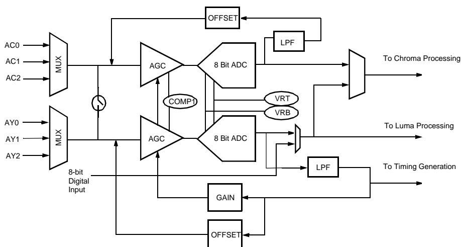
Figure 1. Analog Front End
