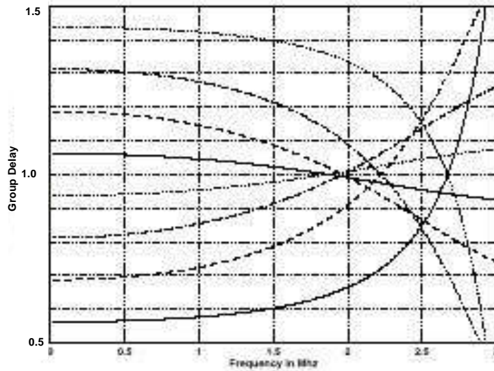
Figure 27. Horizontal Chroma Scaler Interpolation Filter Group Delay
