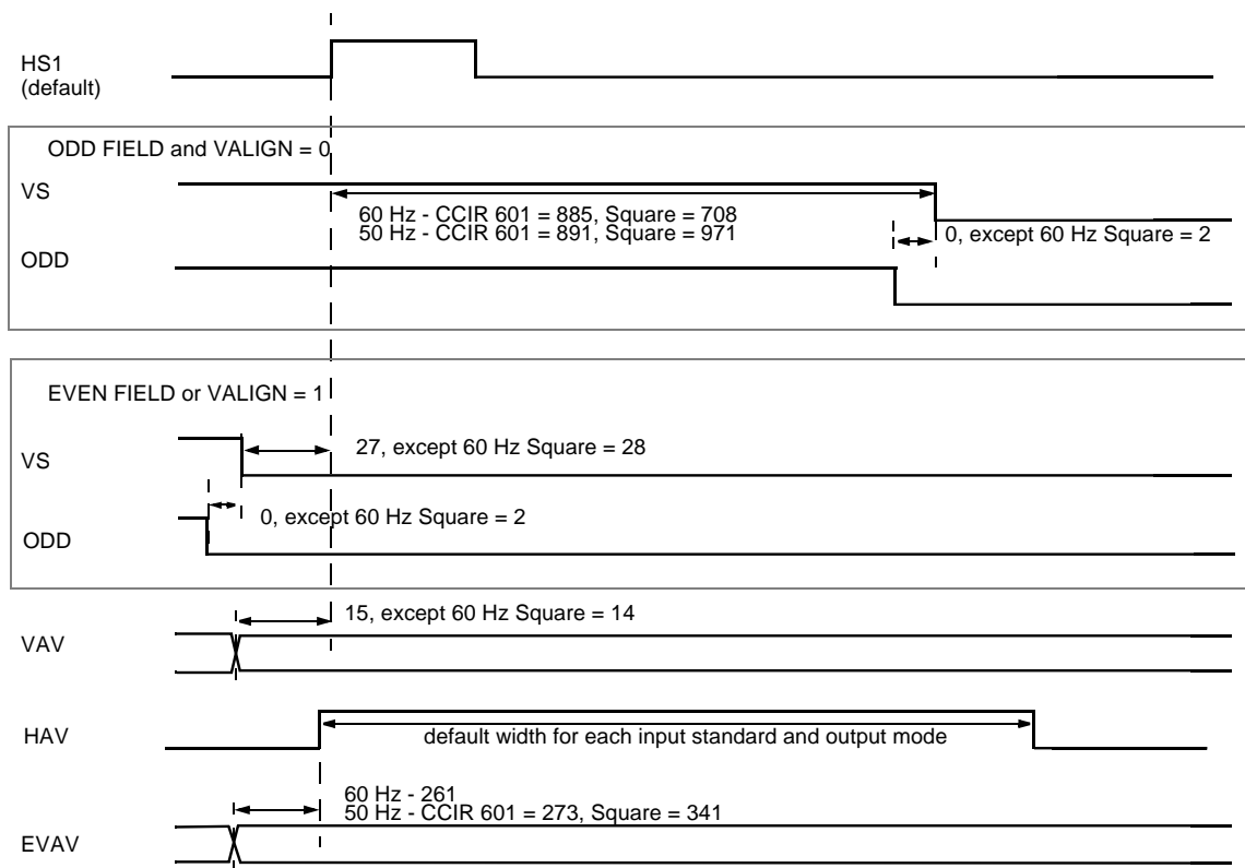
Figure 7. Short Term Vertical Timing
