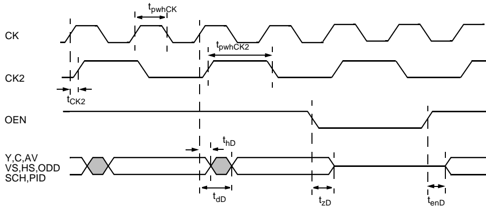
Figure 41. Data Output
