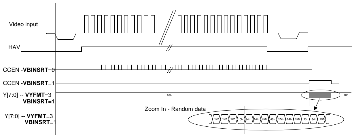
Figure 31. VBI Insertion Timing for VYFMT[1:0]=3
