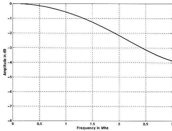
Figure 26. Horizontal Chroma Scaler Interpolation Filter Frequency Response
