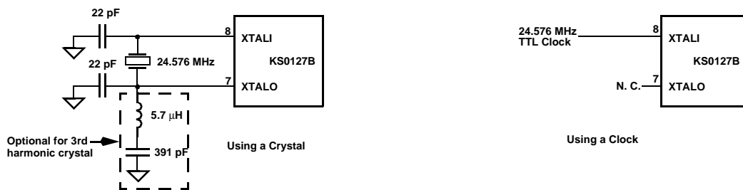
Figure 5. Standard Clock Configurations
