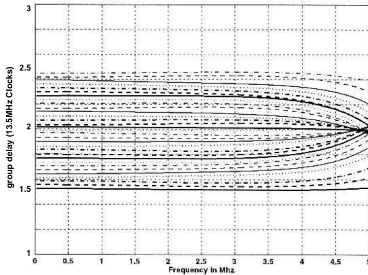
Figure 25. Horizontal Luma Scaler Interpolation Filter Group Delay
