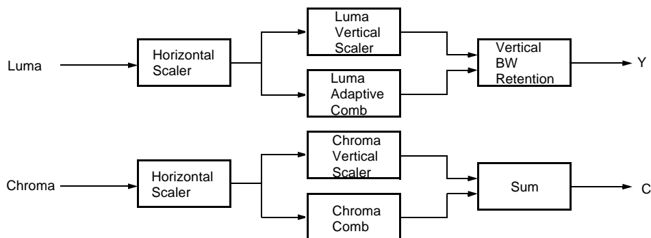
Figure 22. Vertical Processing
