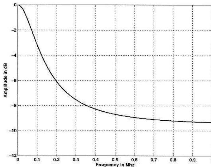
Figure 21. De-emphasis Filter Frequency Response
