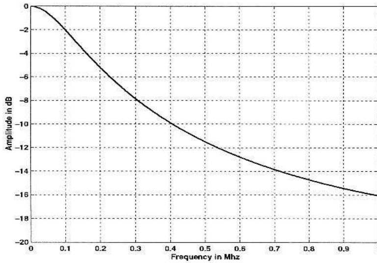
Figure 20. Cloche Filter Frequency Characteristic
