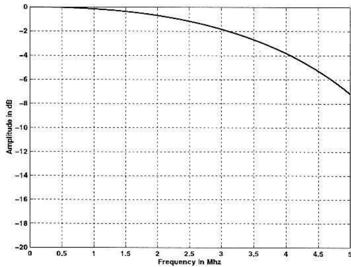
Figure 24. Horizontal Luma Scaler Interpolation Filter Frequency Response
