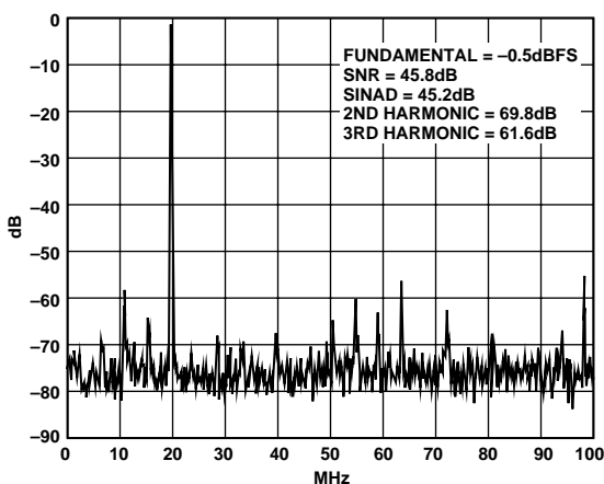
Figure 24. Spectrum: f_s = 140 MSPS, f_{IN} = 19.57 MHz
