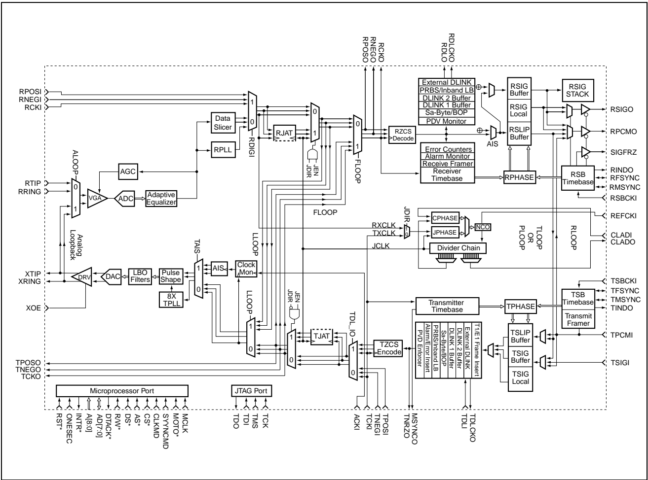
Figure 2-1. Detailed B18370 Block Diagram
