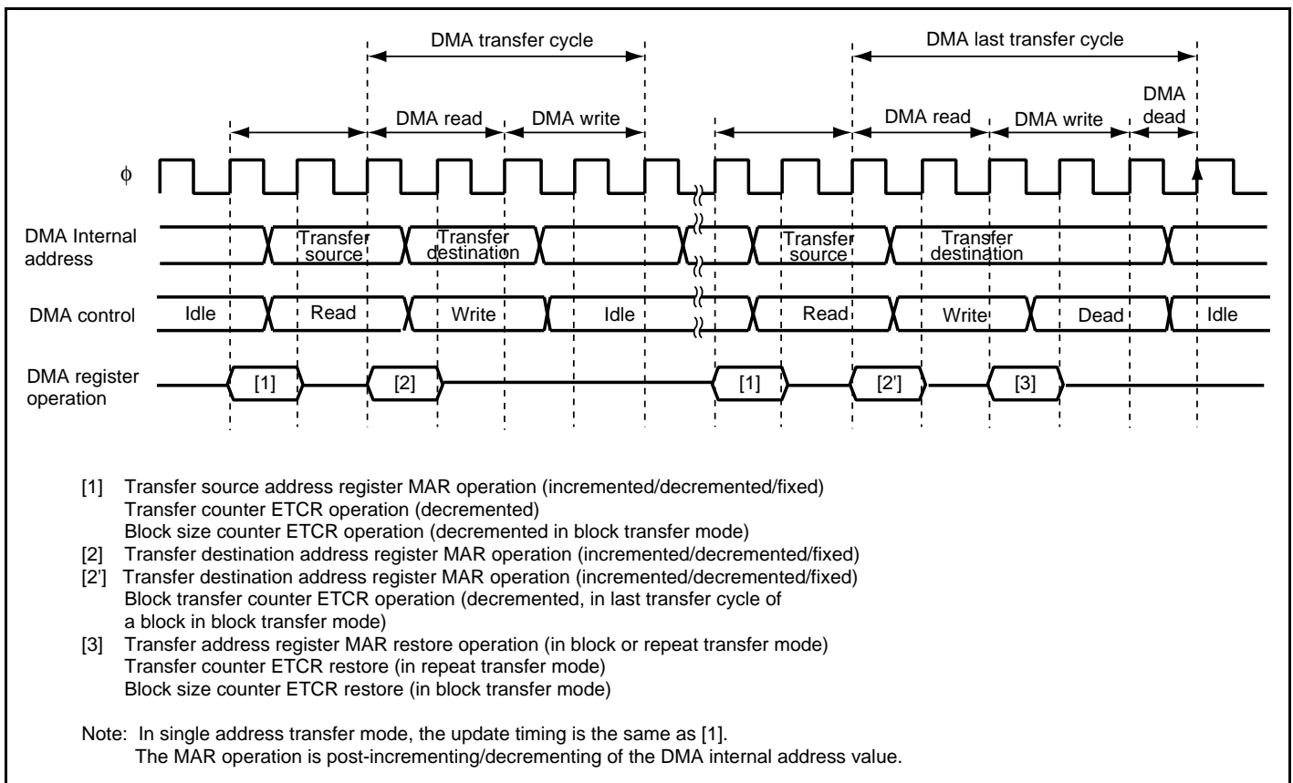
Figure 8.38 DMAC Register Update Timing
