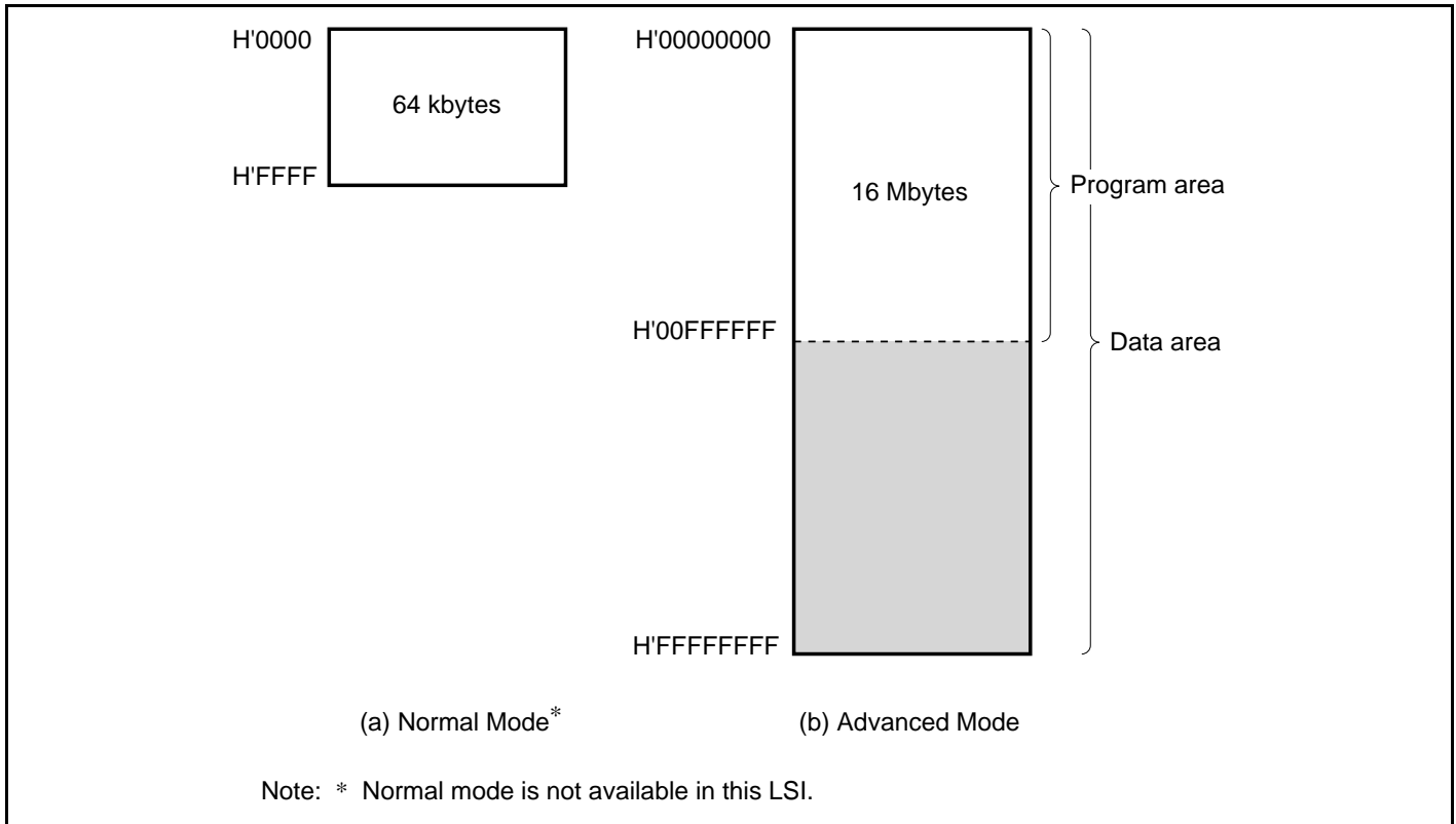
Figure 2.5 Memory Map
