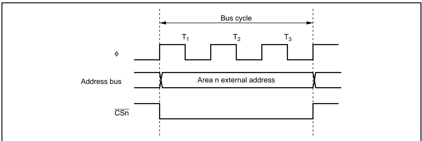
Figure 7.3 \overline{CSn} Signal Output Timing ( n = 0 to 7)
