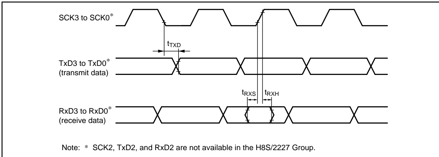
Figure 27.32 SCI Input/Output Timing (Clocked Synchronous Mode)
