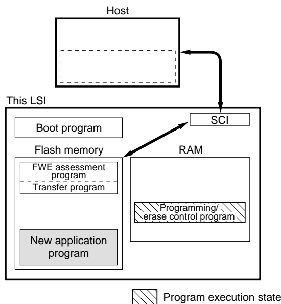
Figure 20.4 User Program Mode (Example)
