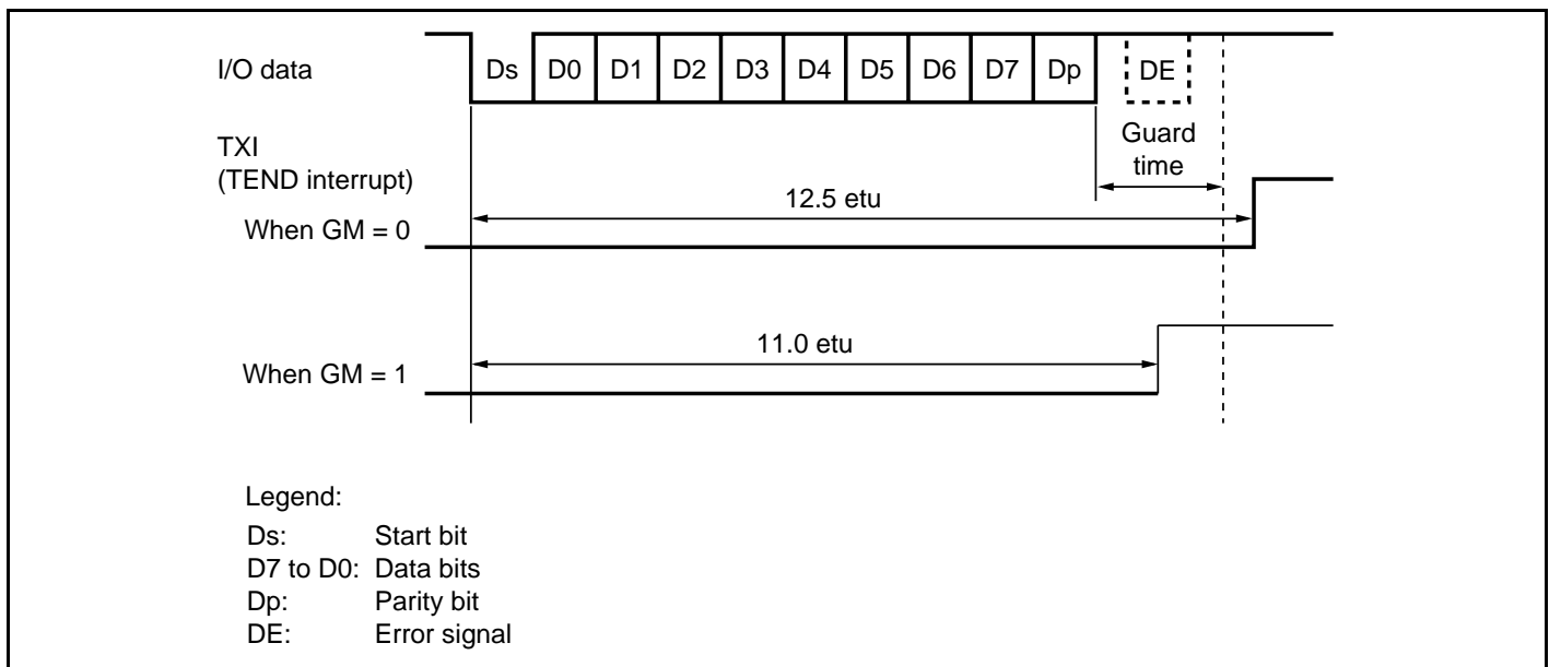
Figure 15.30 TEND Flag Generation Timing in Transmission Operation
