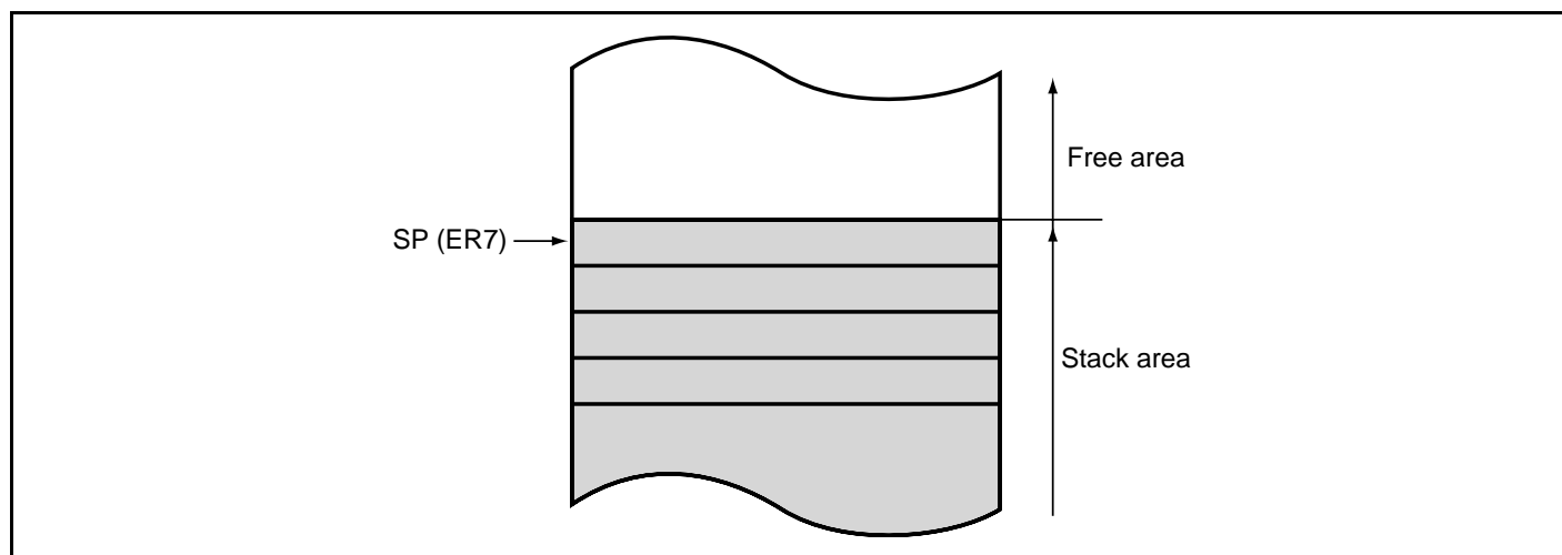
Figure 2.8 Stack Status
