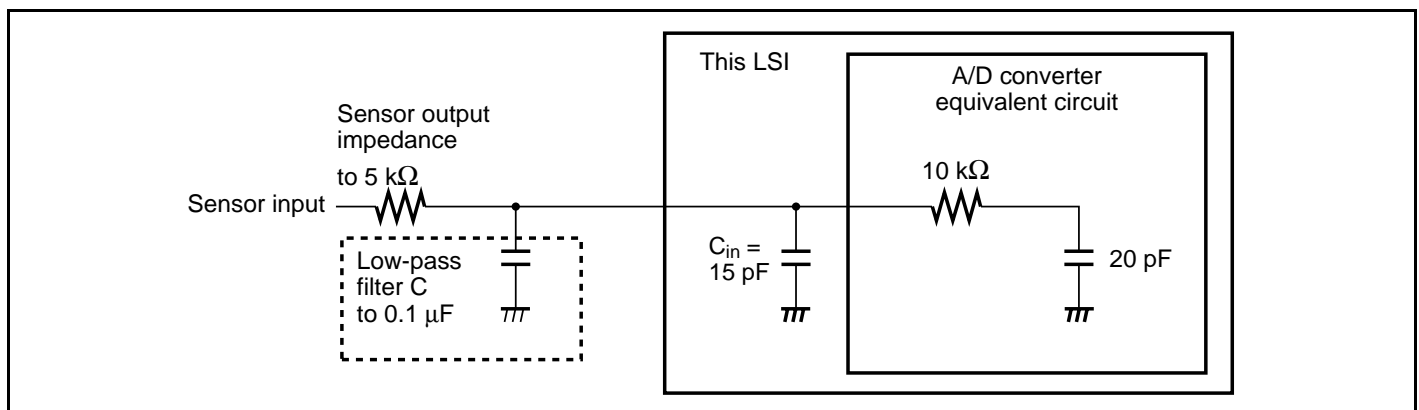
Figure 17.9 Example of Analog Input Circuit
