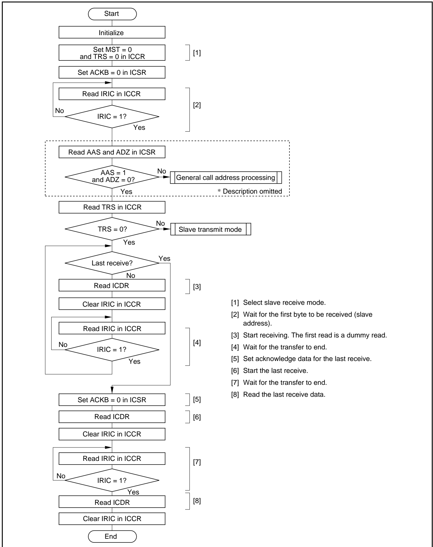
Figure 16.14 Flowchart for Slave Transmit Mode (Example)
