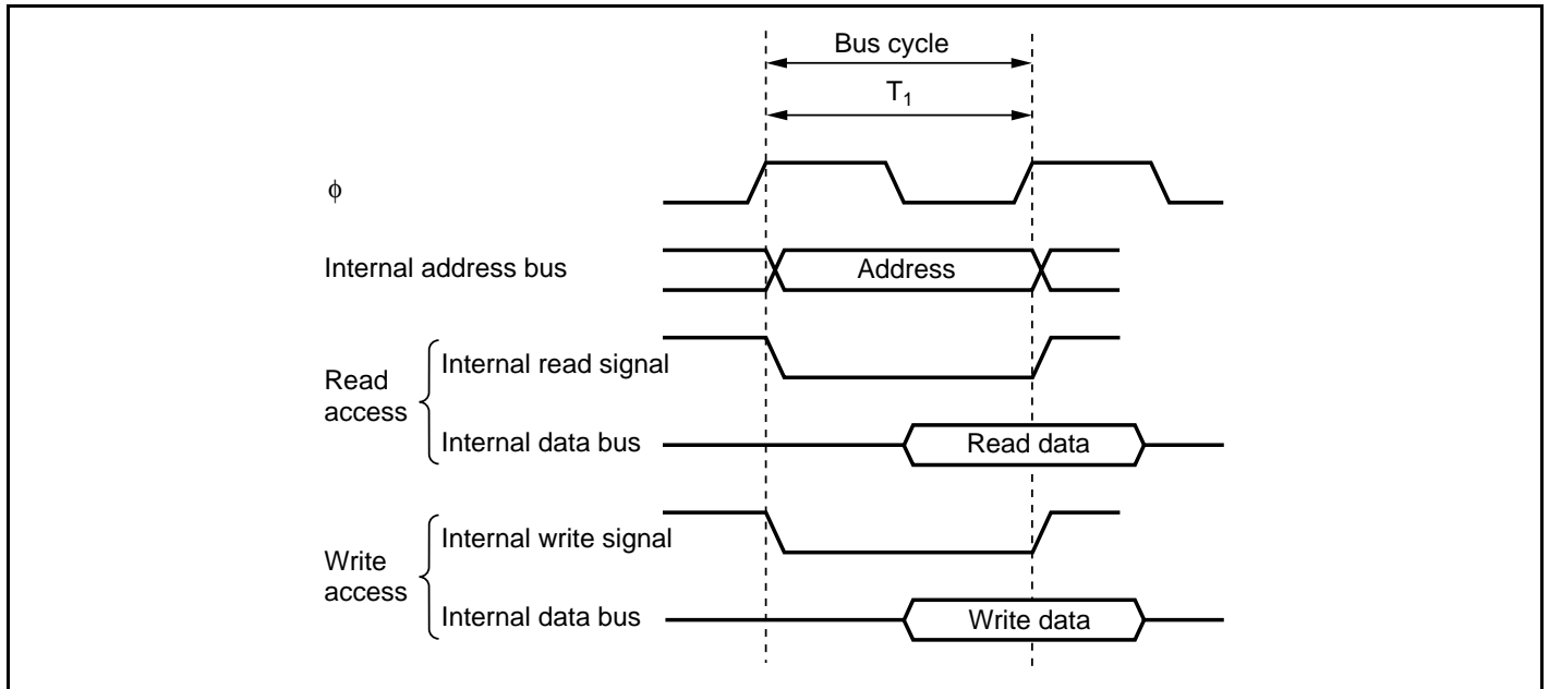
Figure 7.4 On-Chip Memory Access Cycle
