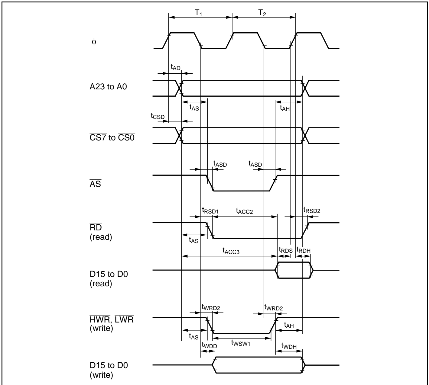
Figure 27.14 Basic Bus Timing (Two-State Access)
