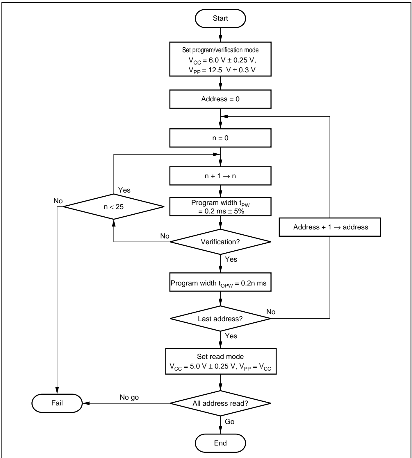
Figure 22.4 High-Speed Programming Flowchart
