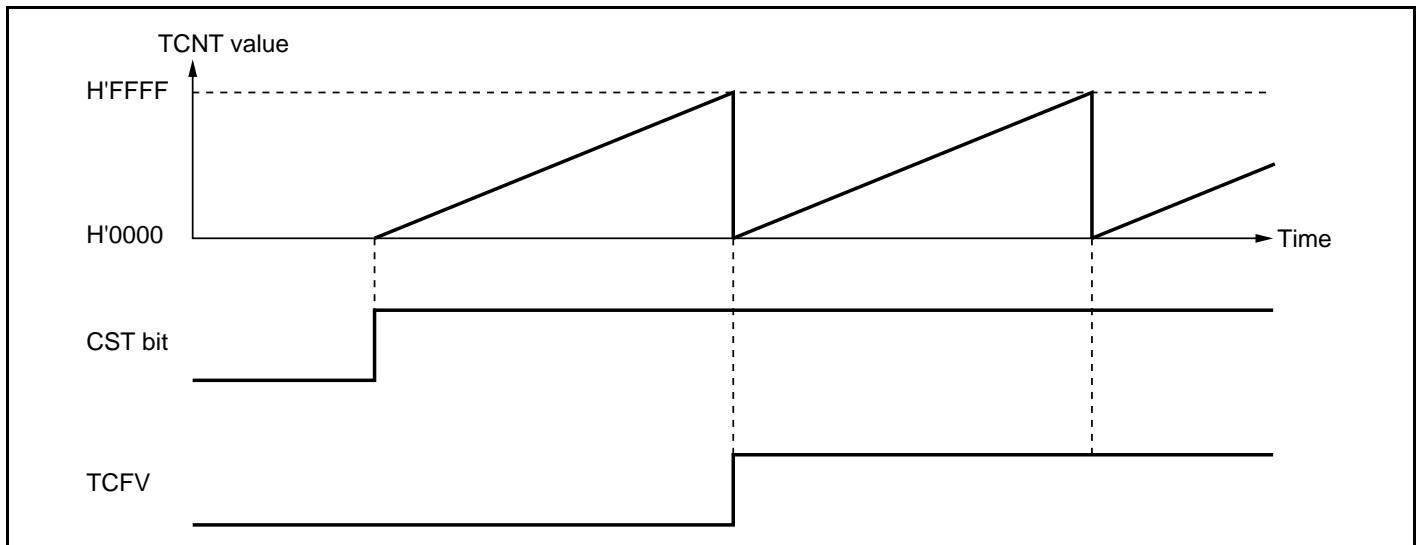
Figure 11.4 Free-Running Counter Operation
