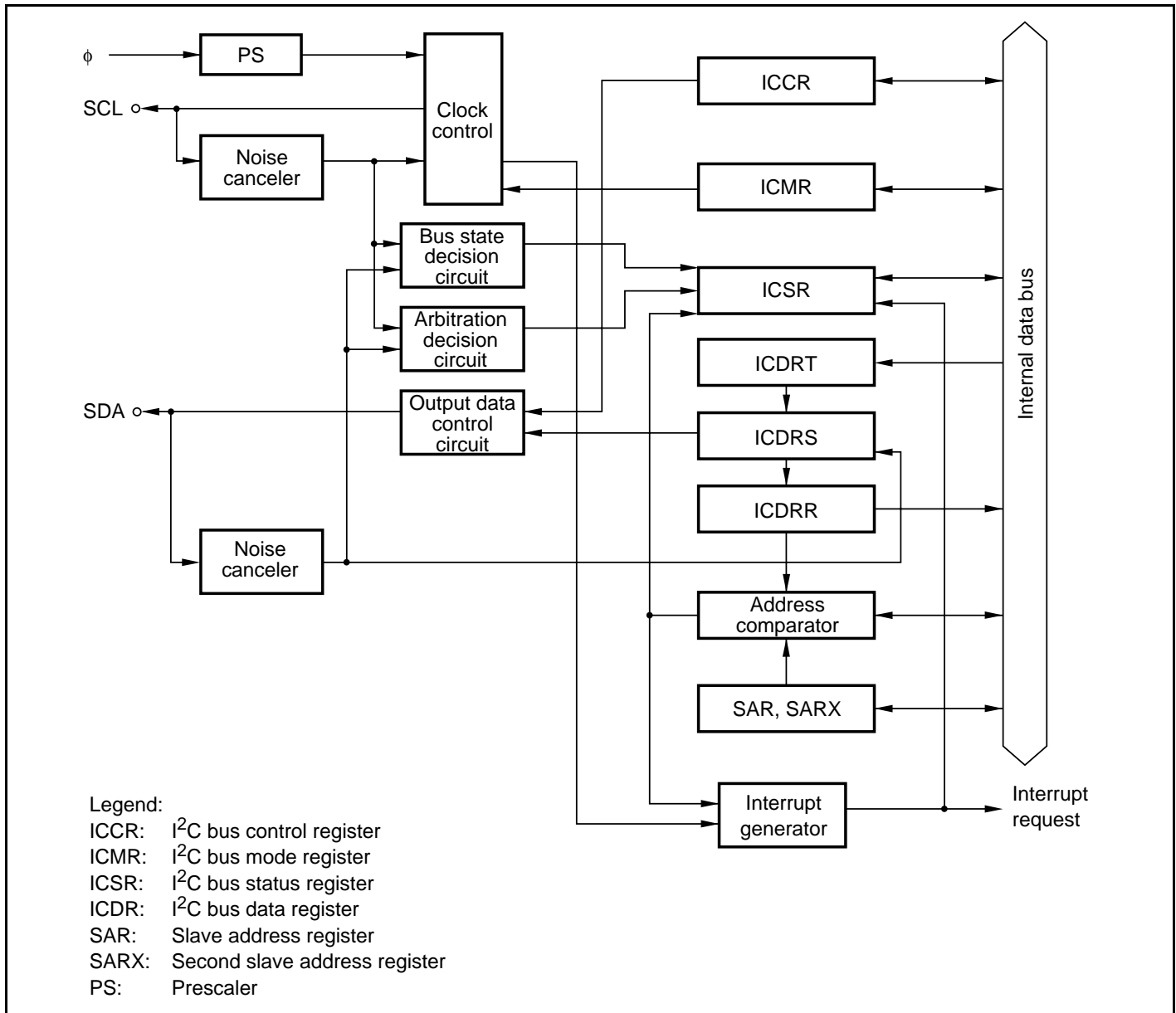
Figure 16.1 Block Diagram of I 2 C Bus Interface
