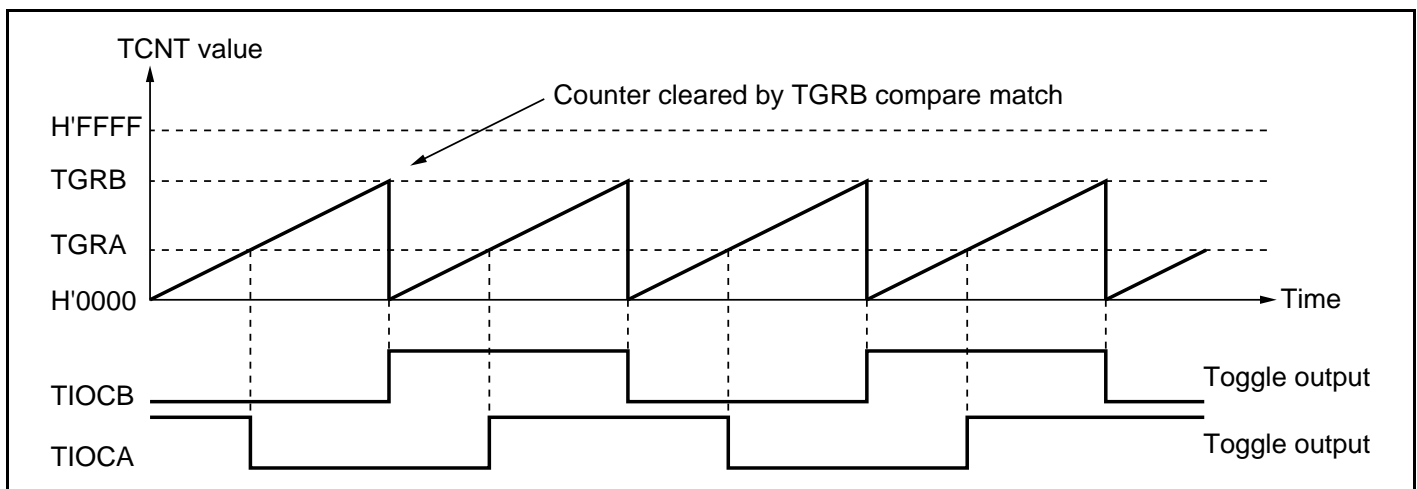
Figure 11.8 Example of Toggle Output Operation
