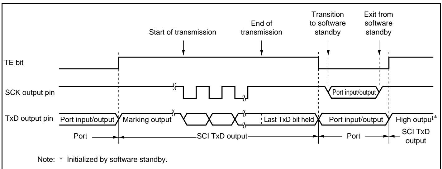
Figure 15.41 Synchronous Transmission Using Internal Clock
