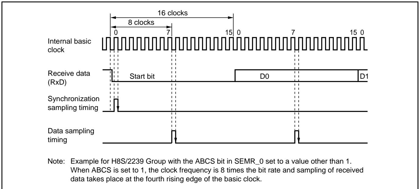
Figure 15.6 Receive Data Sampling Timing in Asynchronous Mode
