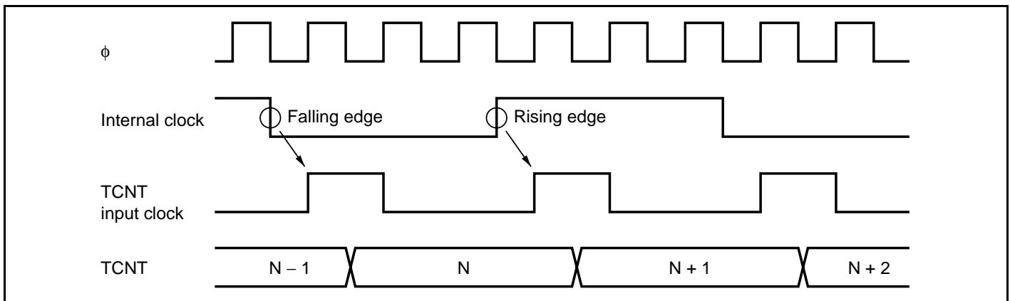
Figure 11.31 Count Timing in Internal Clock Operation
