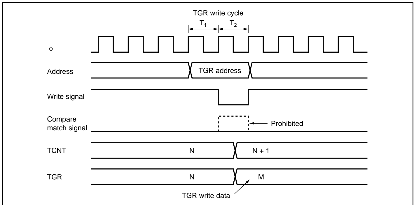
Figure 11.48 Contention between TGR Write and Compare Match
