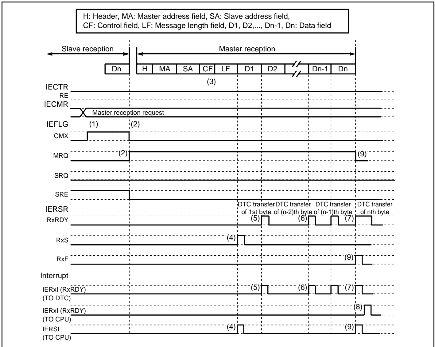
Figure 14.11 Master Receive Operation Timing
