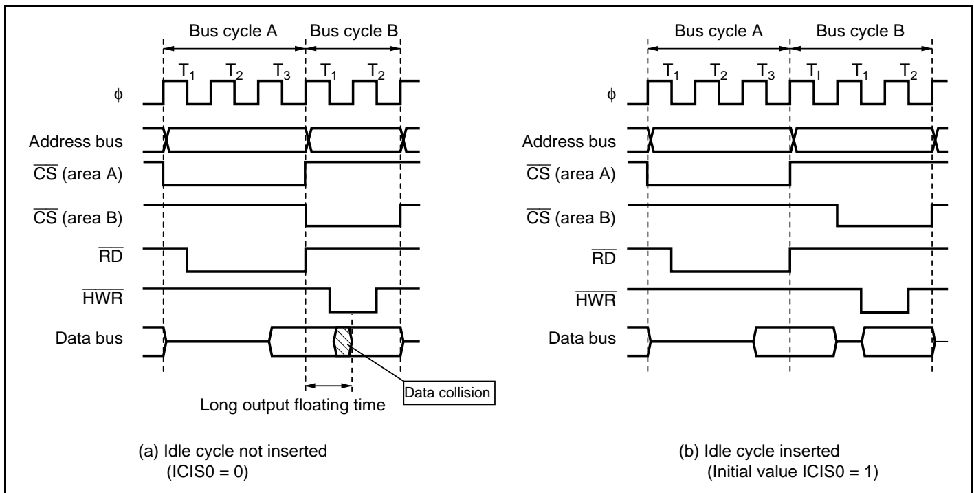
Figure 7.22 Example of Idle Cycle Operation (2)
