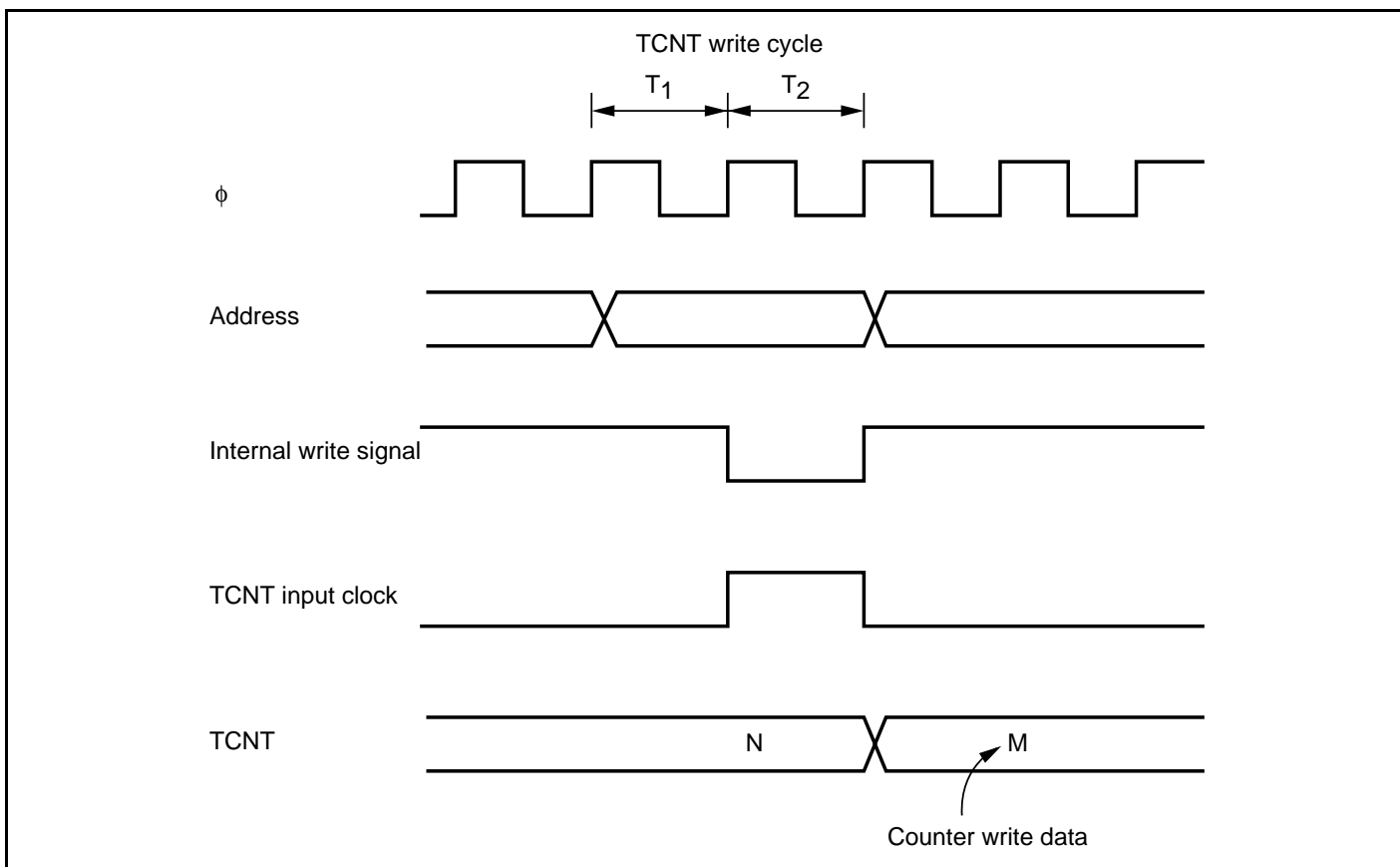
Figure 13.8 Contention between TCNT Write and Increment
