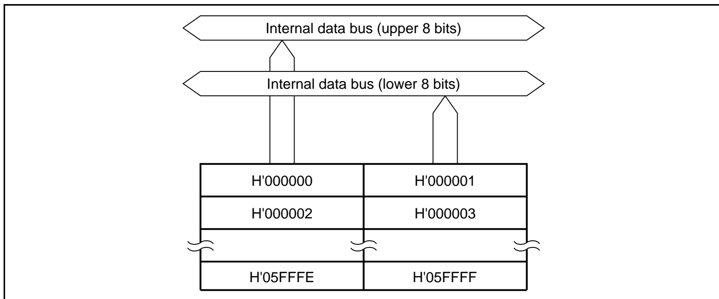
Figure 21.1 Block Diagram of On-Chip Masked ROM (384 kbytes)
