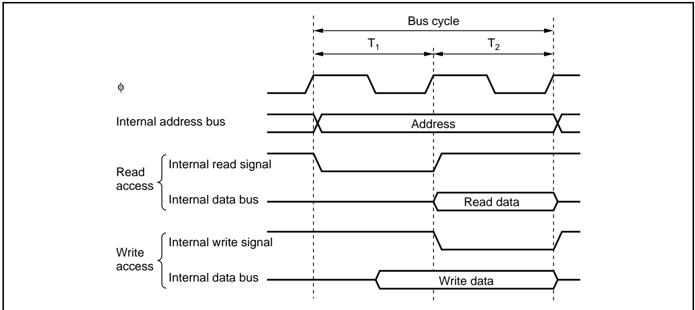
Figure 7.6 On-Chip Peripheral Module Access Cycle
