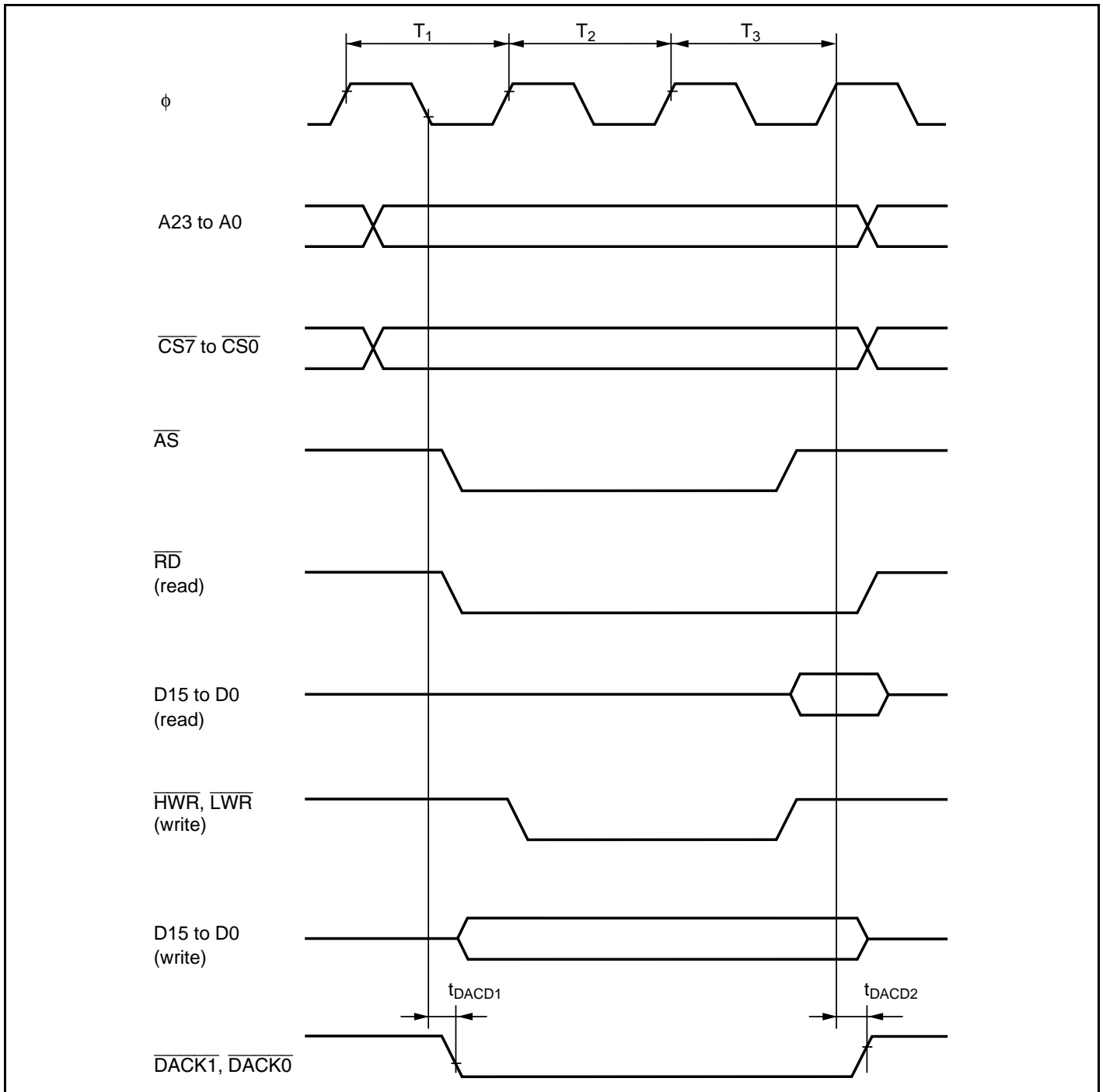
Figure 27.21 DMAC Single Address Transfer Timing (Three-State Access)
