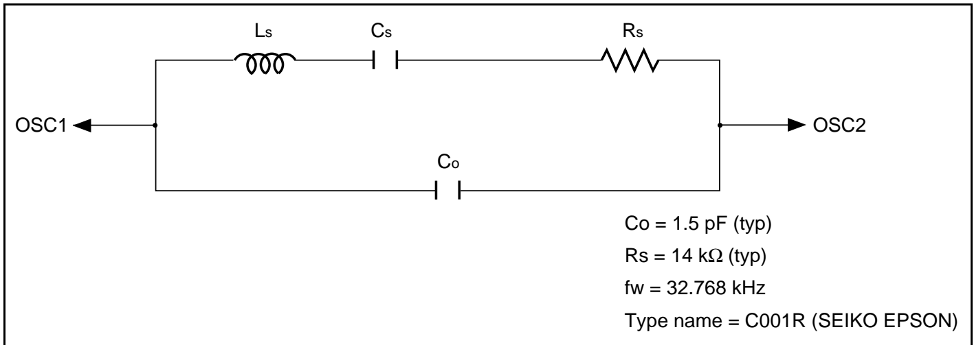
Figure 23.9 Equivalence Circuit for 32.768-kHz Oscillator
