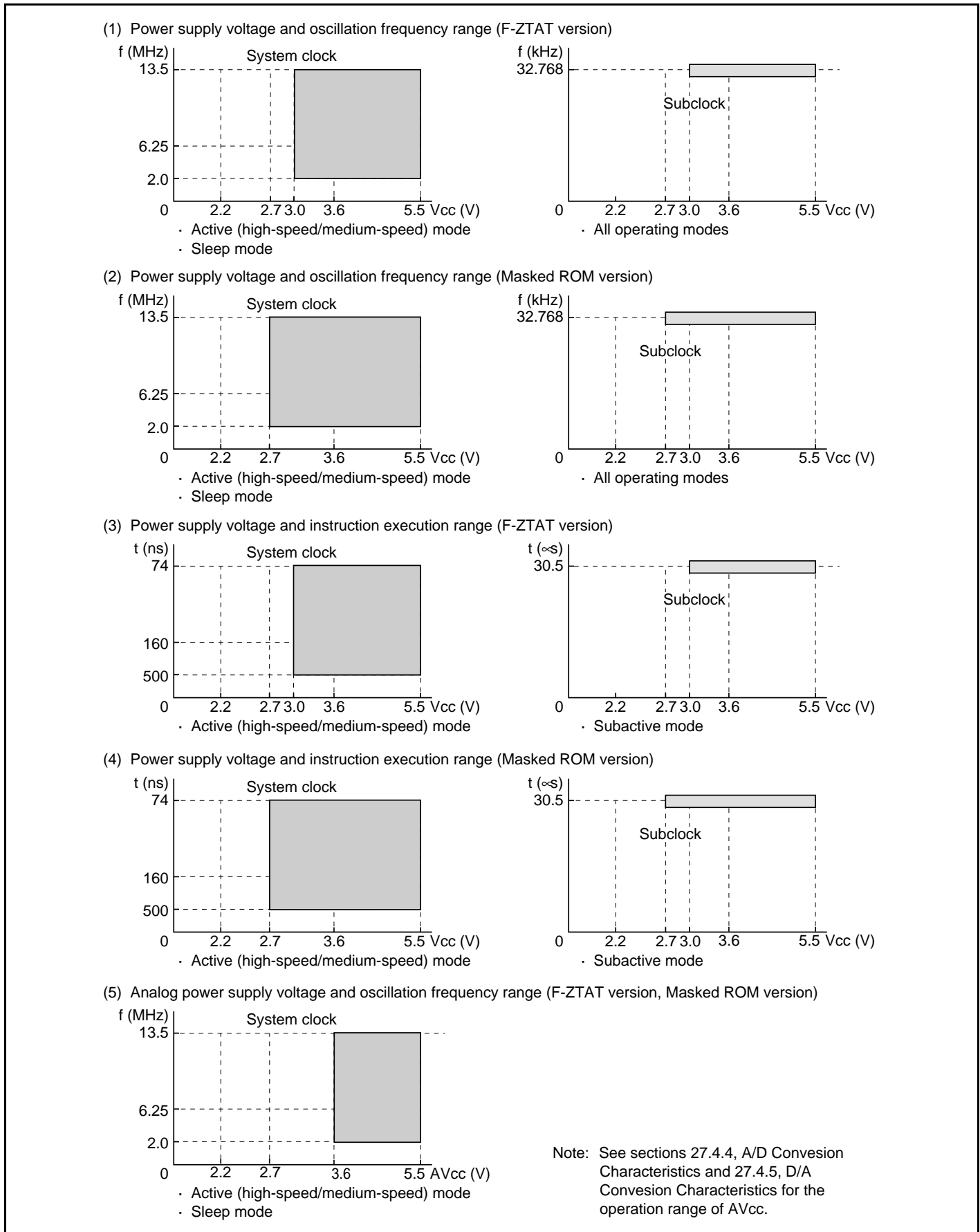
Figure 27.3 Power Supply Voltage and Operating Ranges (H8S/2238B and H8S/2236B)
