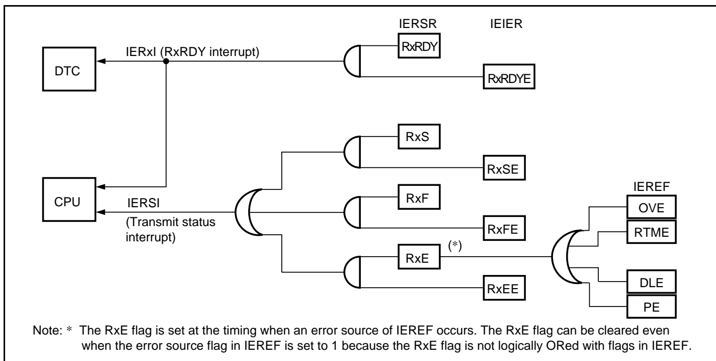
Figure 14.14 Relationships among Receive Interrupt Sources
