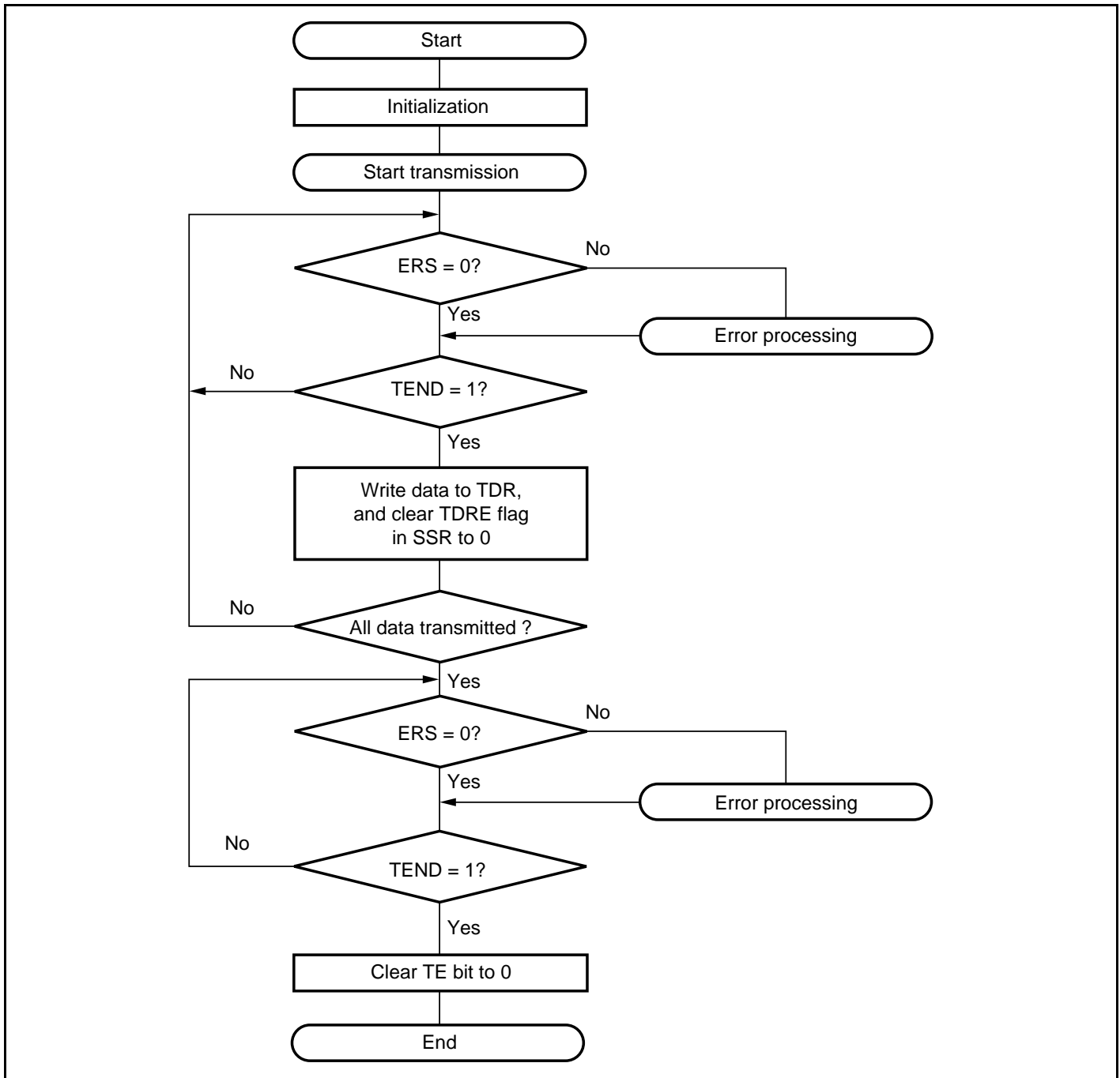
Figure 15.31 Example of Transmission Processing Flow
