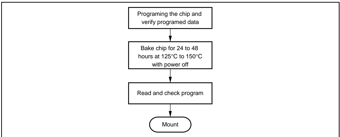
Figure 22.6 Recommended Screening Procedure
