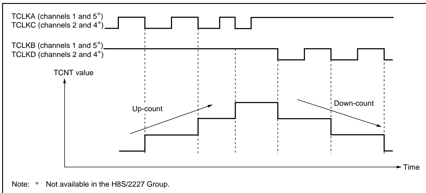
Figure 11.28 Example of Phase Counting Mode 3 Operation
