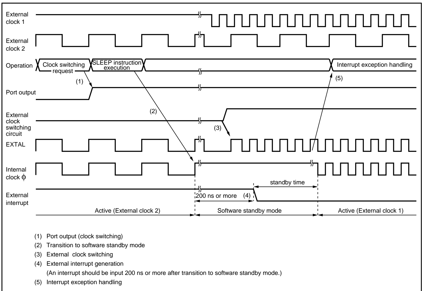
Figure 23.7 External Clock Switching Timing (Example)
