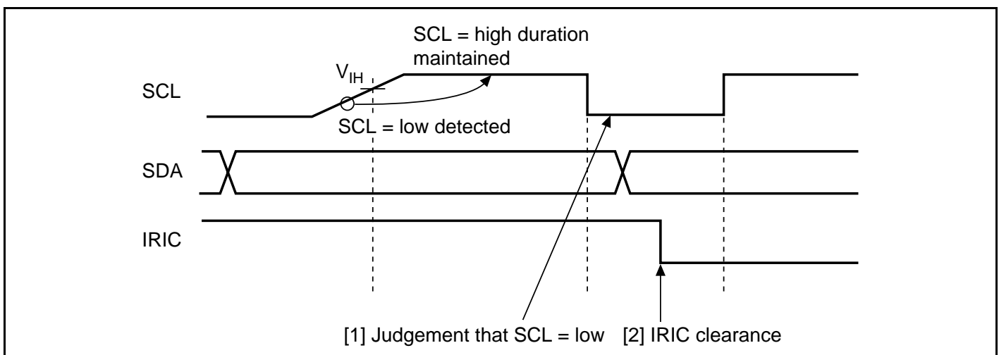
Figure 16.24 IRIC Flag Clearance in WAIT = 1 Status
