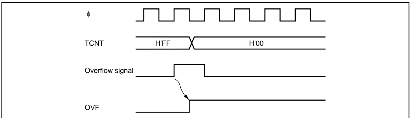
Figure 12.9 Timing of OVF Setting
