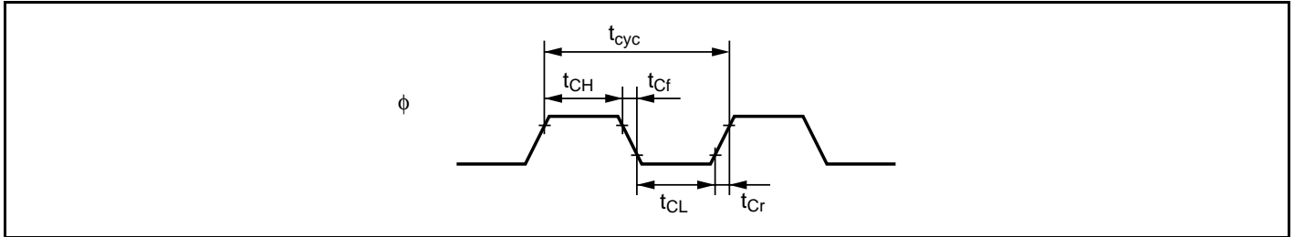
Figure 27.10 System Clock Timing
