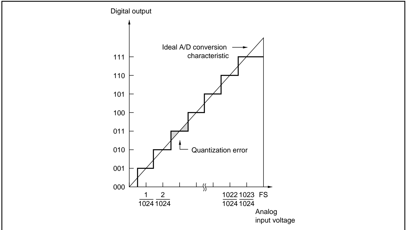
Figure 17.7 A/D Conversion Accuracy Definitions
