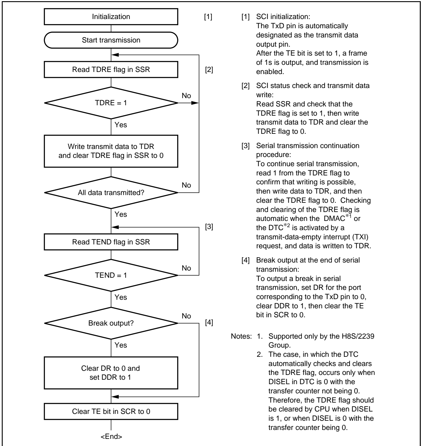
Figure 15.10 Sample Serial Transmission Flowchart
