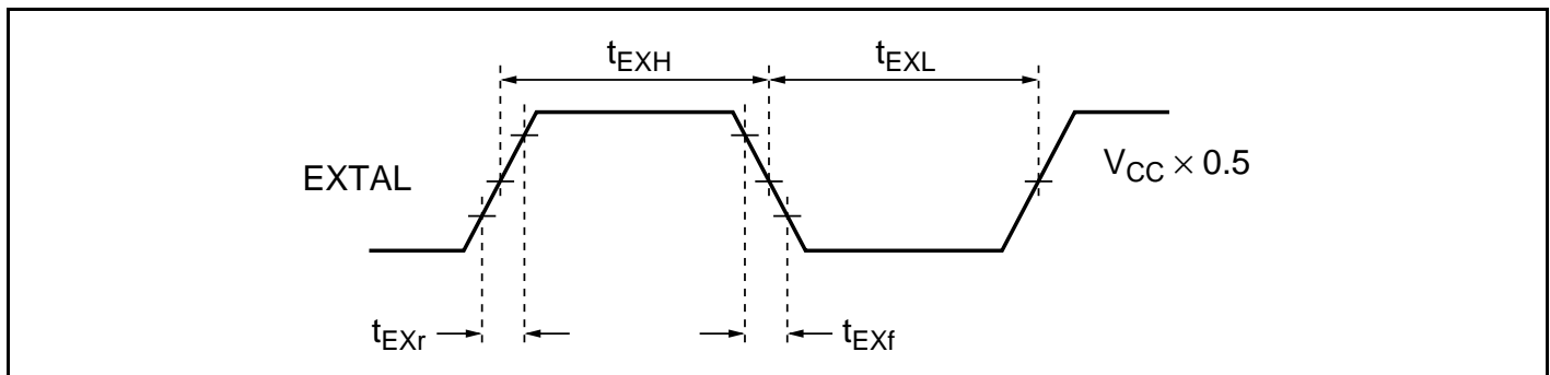
Figure 23.5 External Clock Input Timing
