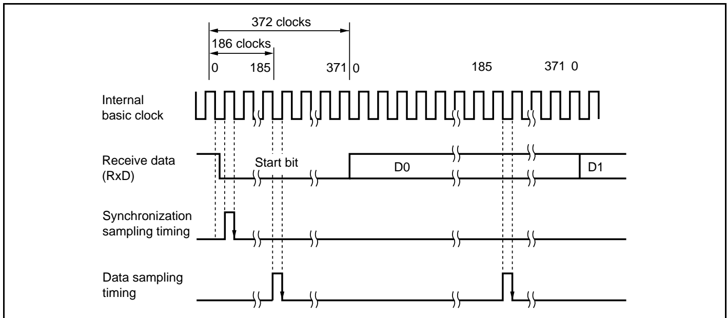
Figure 15.28 Receive Data Sampling Timing in Smart Card Mode (Using Clock of 372 Times the Transfer Rate)
