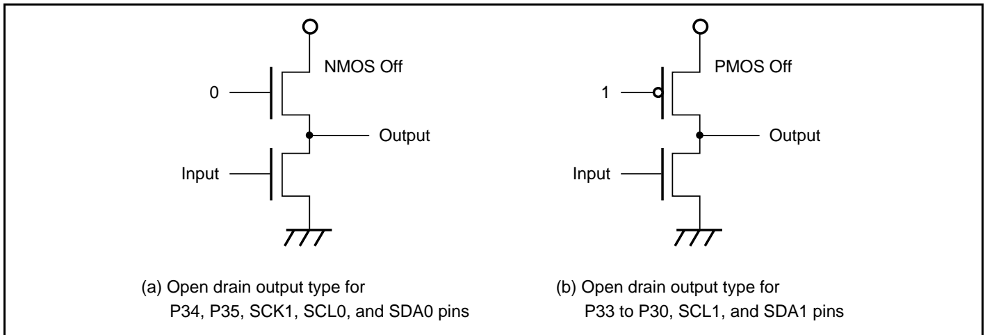
Figure 10.1 Types of Open Drain Outputs
