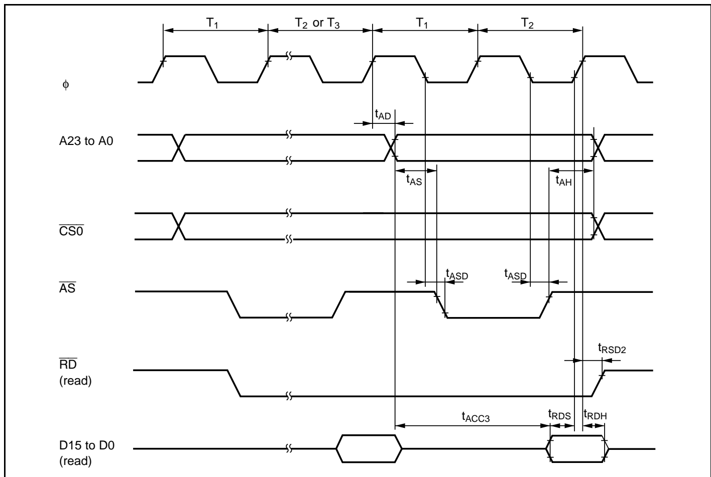
Figure 27.17 Burst ROM Access Timing (Two-State Access)
