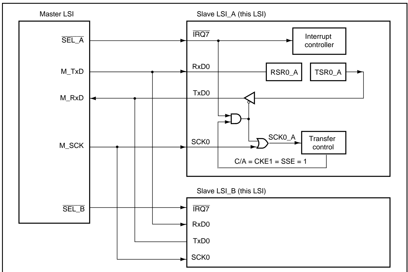
Figure 15.36 Example of Communication Using SCI Select Function
