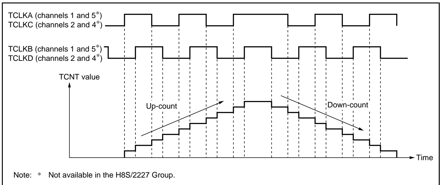
Figure 11.26 Example of Phase Counting Mode 1 Operation
