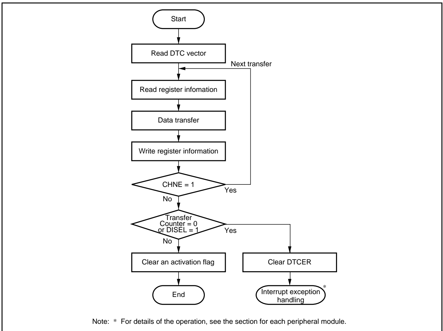
Figure 9.5 Flowchart of DTC Operation
