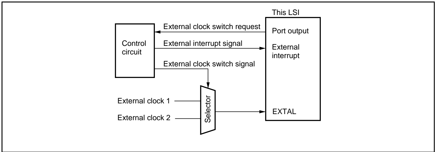
Figure 23.6 External Clock Switching Circuit (Example)
