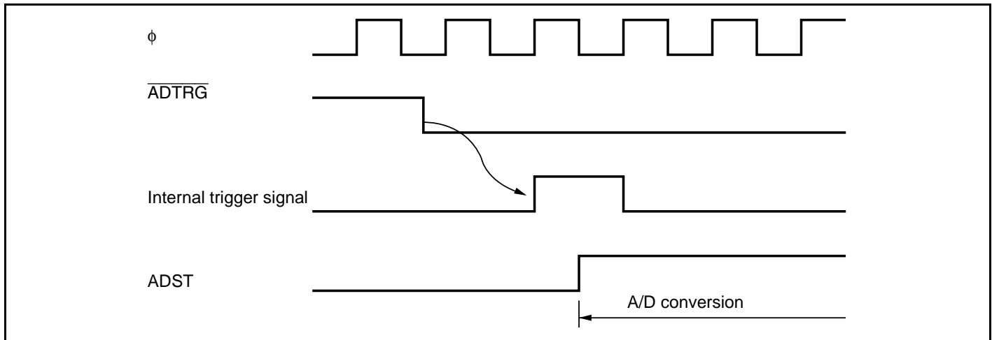
Figure 17.6 External Trigger Input Timing
