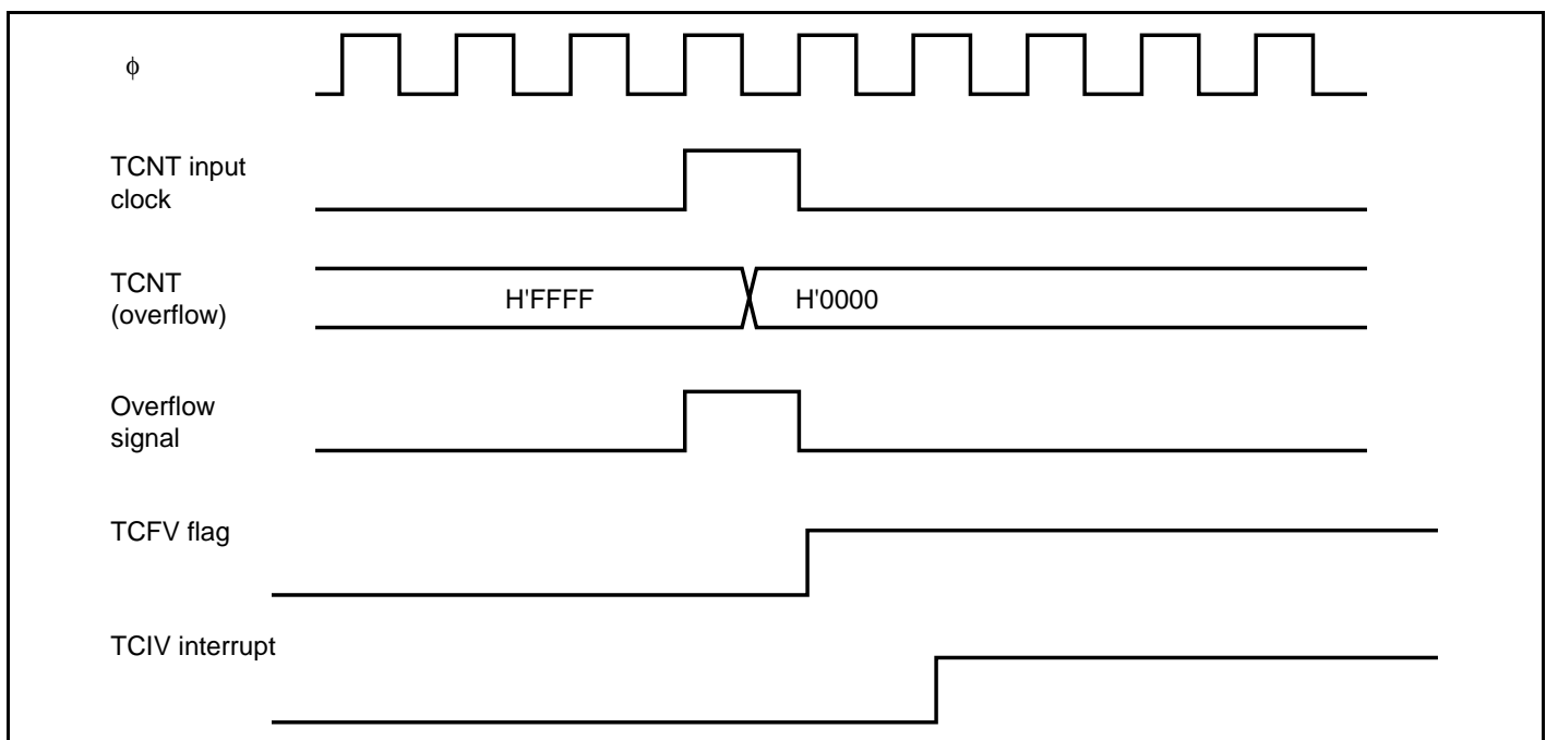
Figure 11.41 TCIV Interrupt Setting Timing
