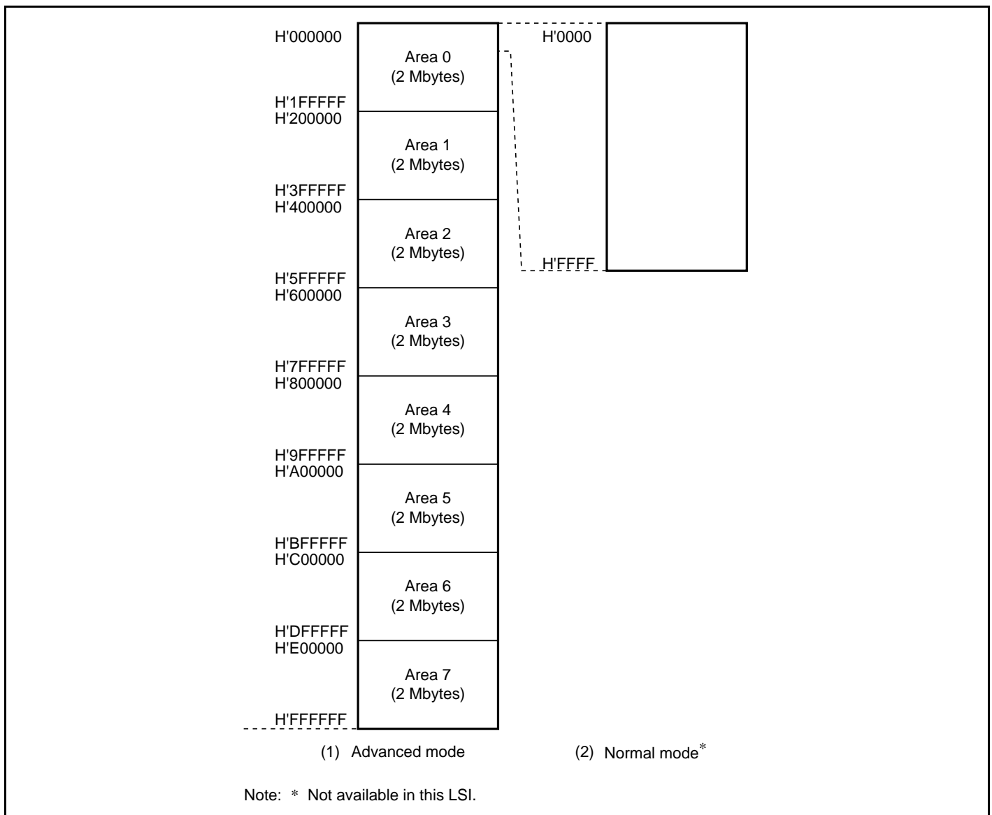
Figure 7.2 Overview of Area Divisions
