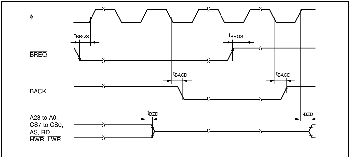
Figure 27.19 External Bus Release Timing
