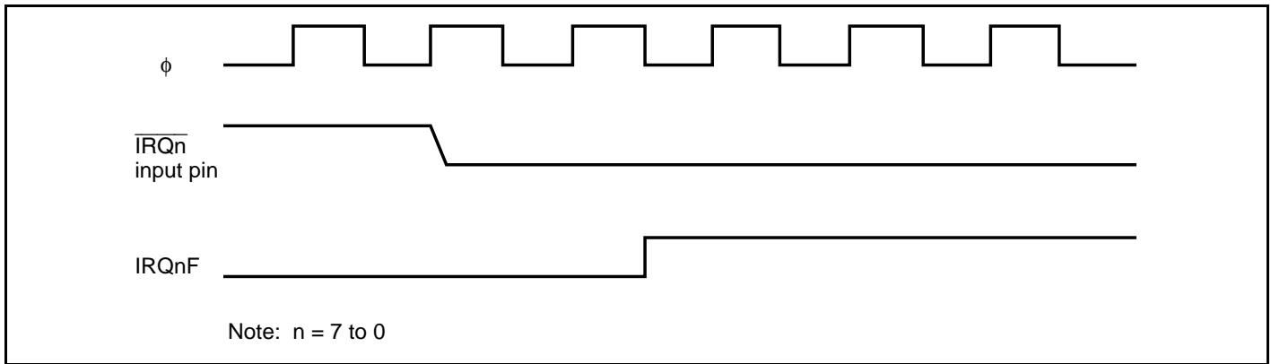
Figure 5.3 Set Timing for IRQnF
