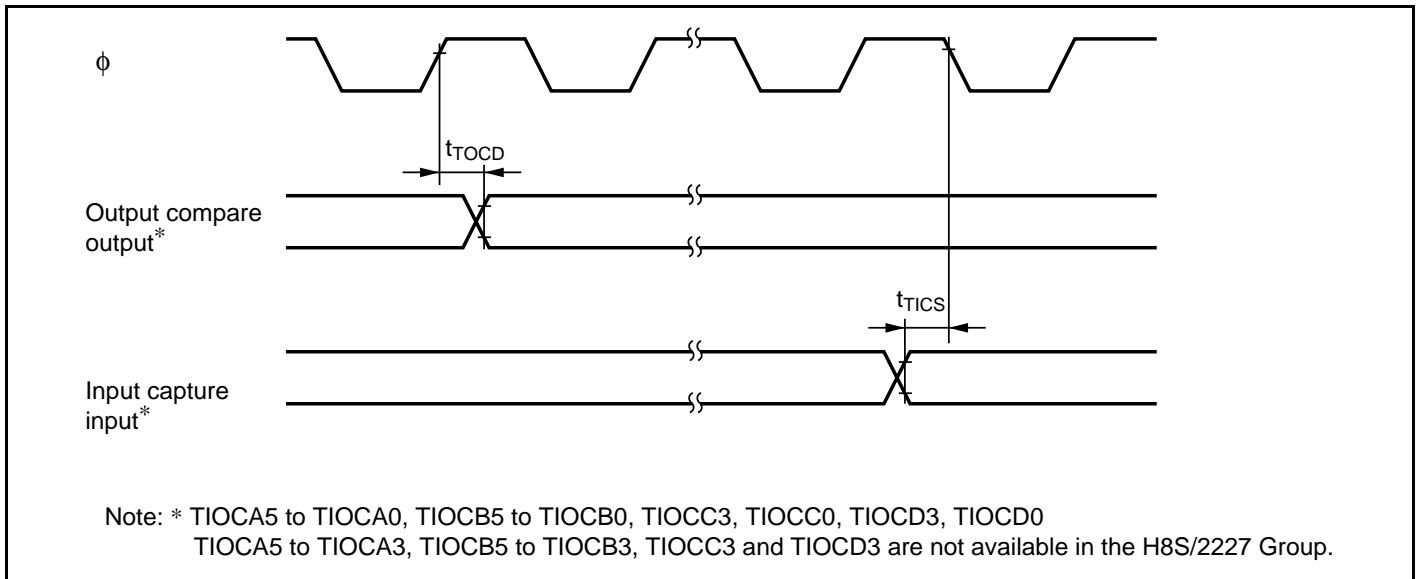
Figure 27.25 TPU Input/Output Timing
