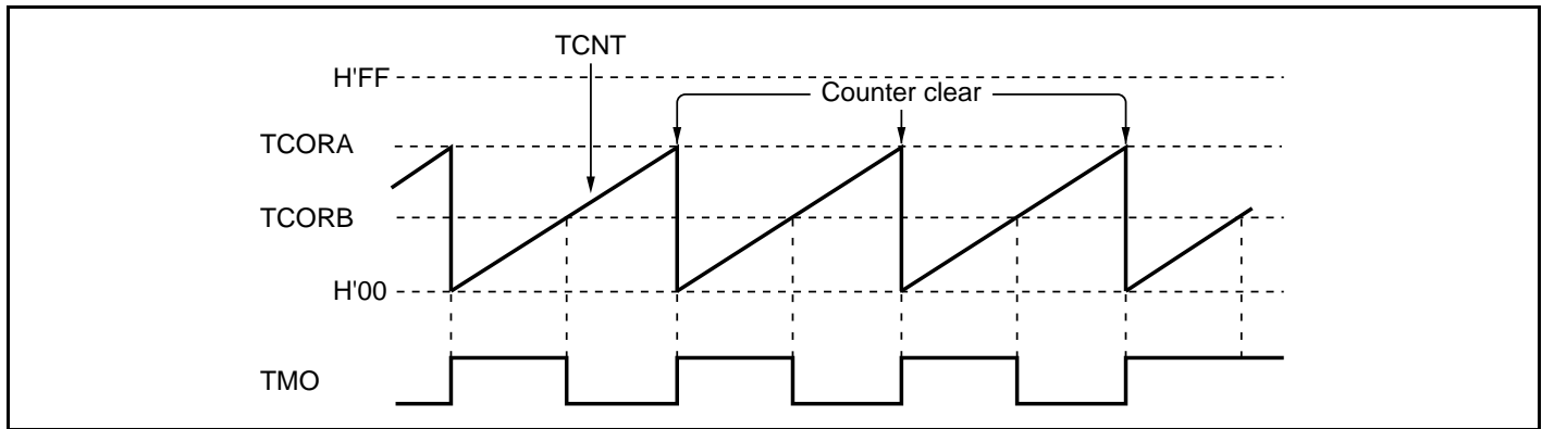
Figure 12.2 Example of Pulse Output
