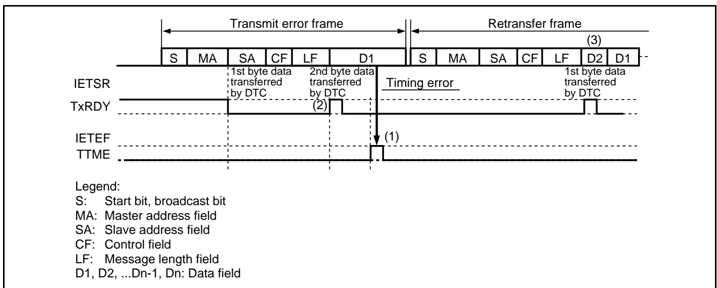
Figure 14.15 Error Processing in Transfer
