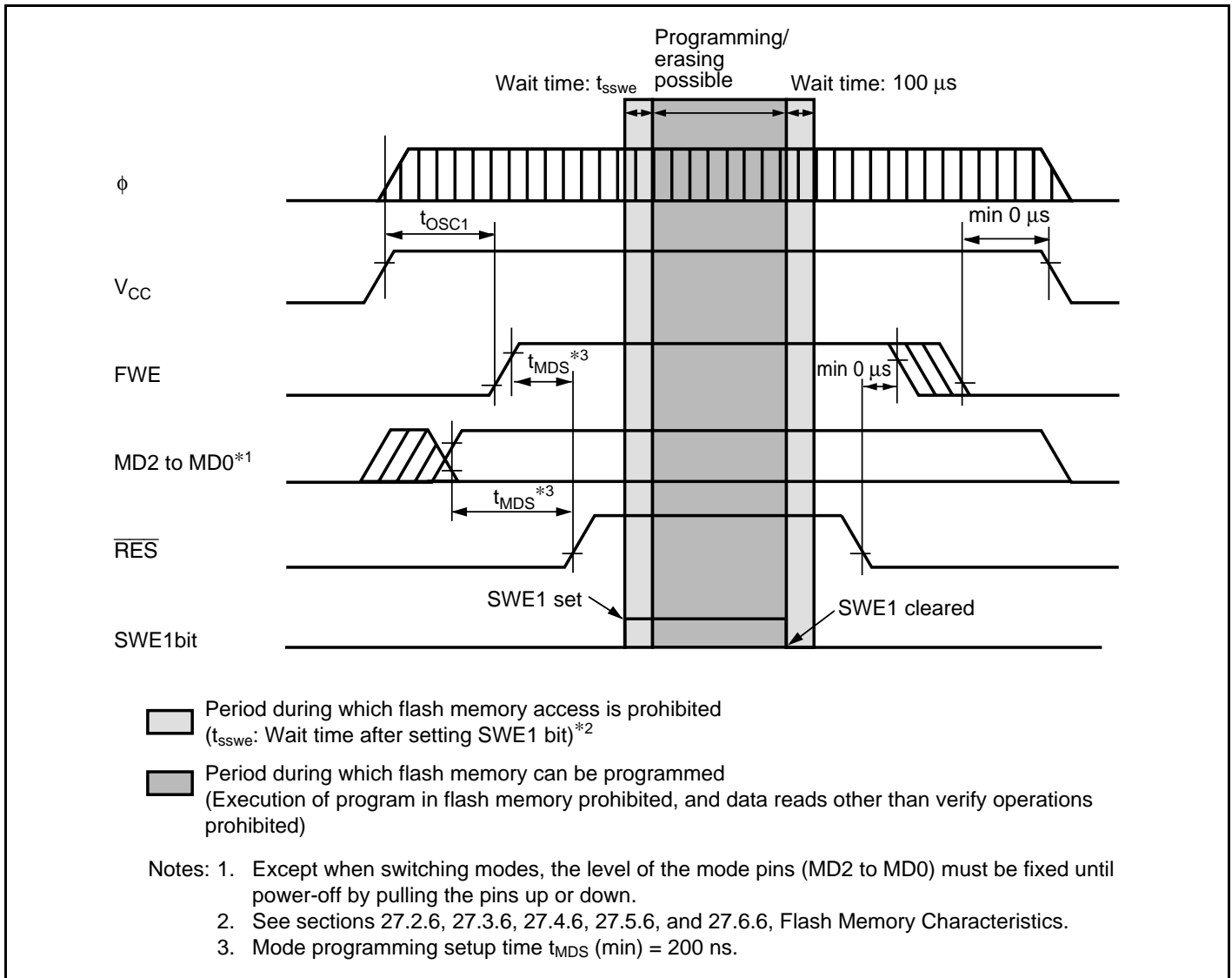
Figure 20.14 Power-On/Off Timing (Boot Mode)
