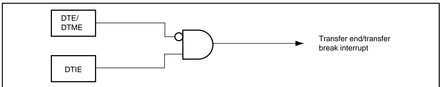
Figure 8.37 Block Diagram of Transfer End/Transfer Break Interrupt
