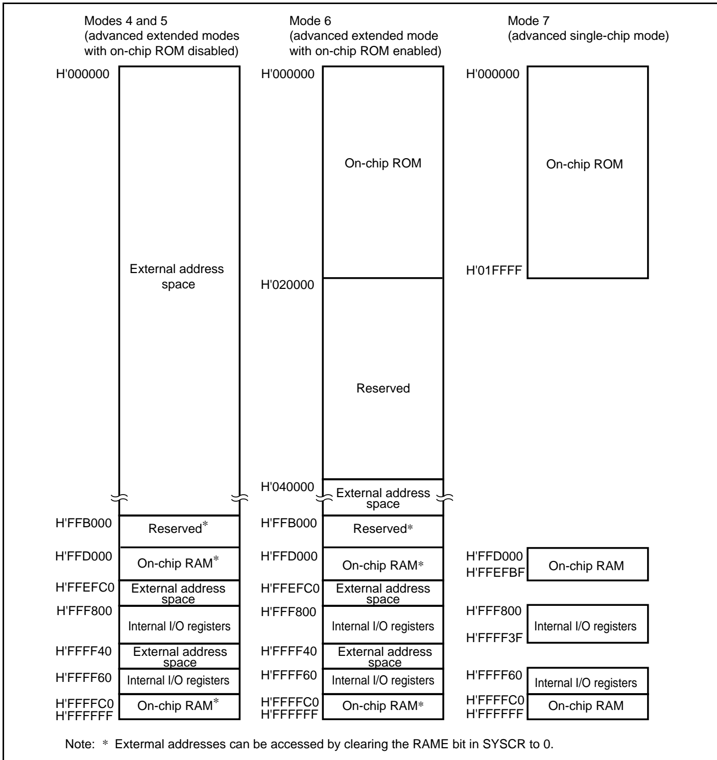
Figure 3.2 H8S/2256 Memory Map in Each Operating Mode
