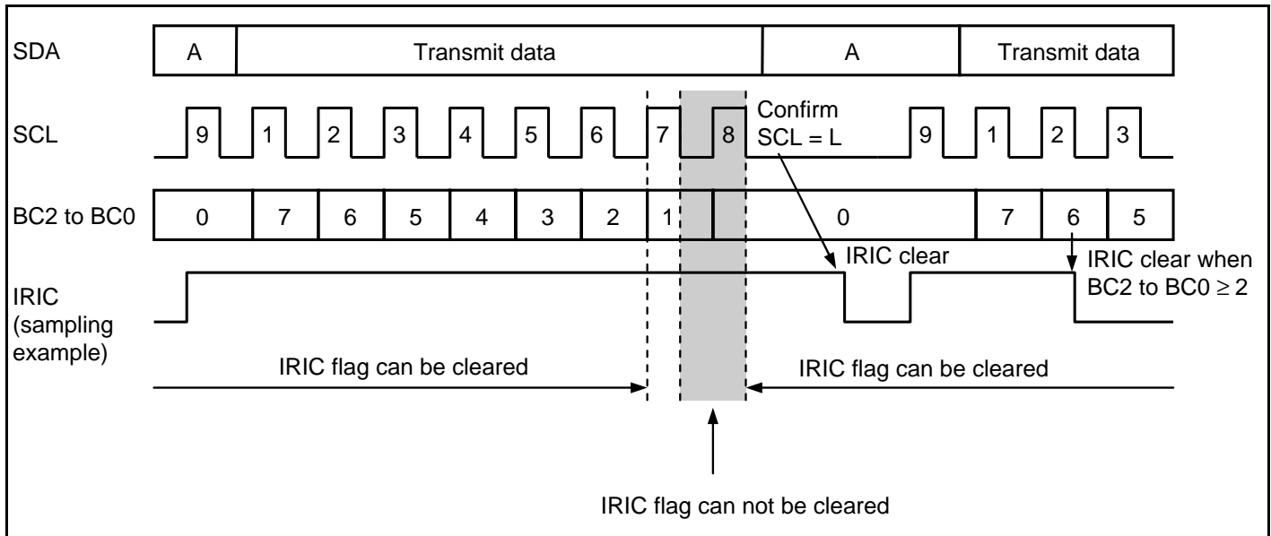
Figure 16.28 IRIC Flag Clearing Timing in Wait Operation
