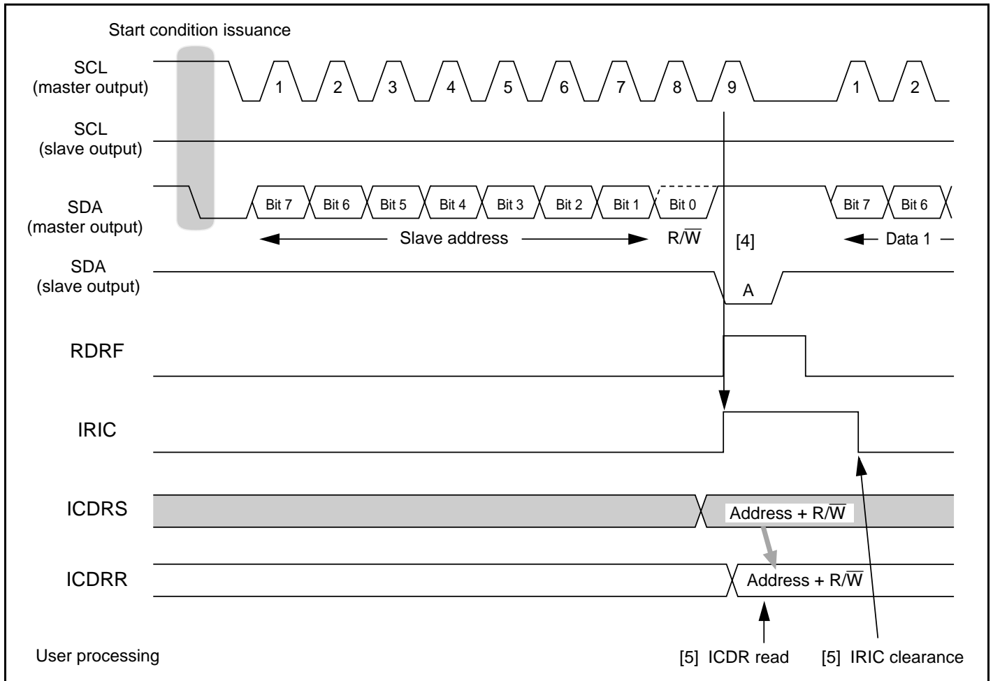
Figure 16.15 Example of Slave Receive Mode Operation Timing (1) (MLS = ACKB = 0)
