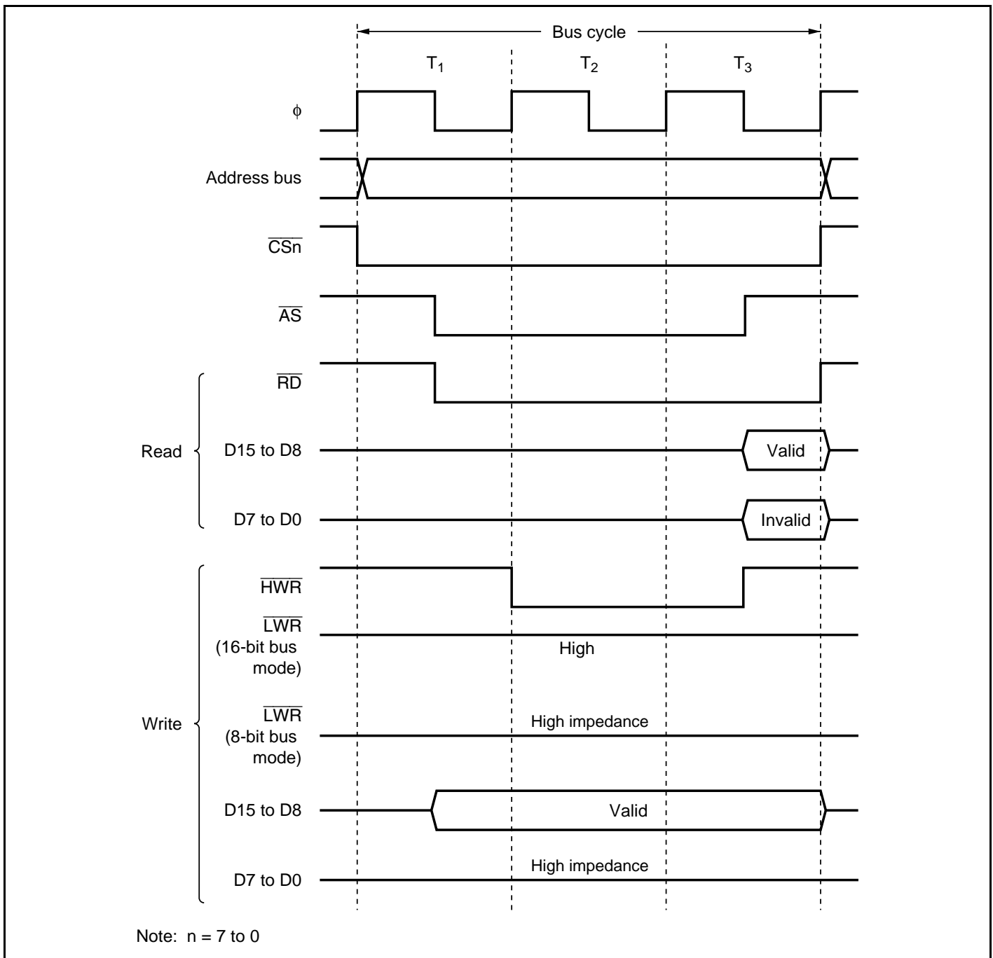
Figure 7.11 Bus Timing for 8-Bit 3-State Access Space
