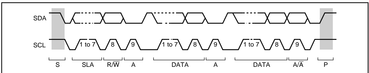
Figure 16.5 I 2 C Bus Timing
