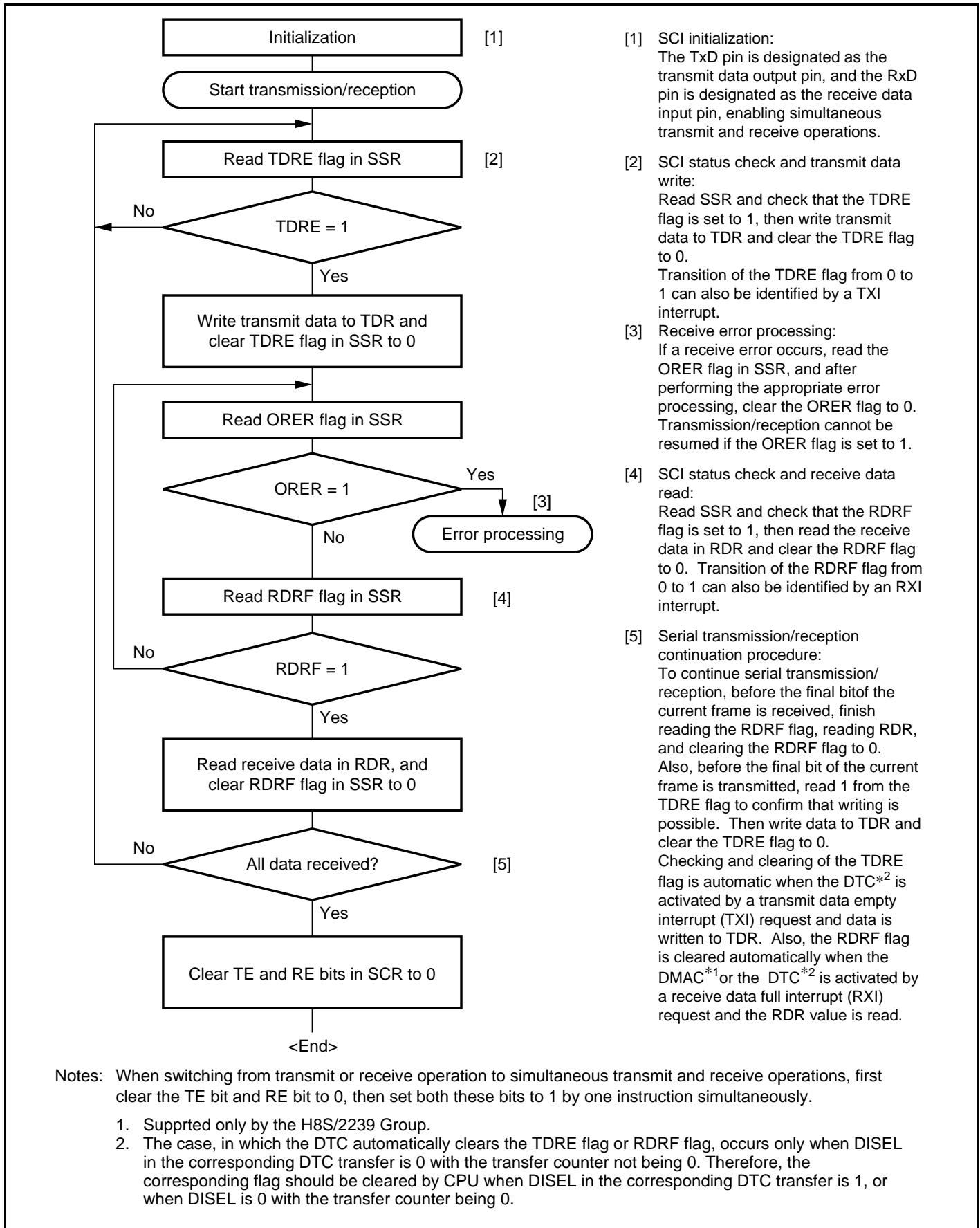
Figure 15.23 Sample Flowchart of Simultaneous Serial Transmit and Receive Operations
