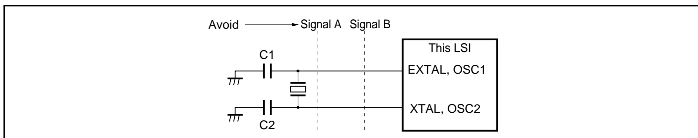
Figure 23.11 Note on Board Design of Oscillator Circuit
