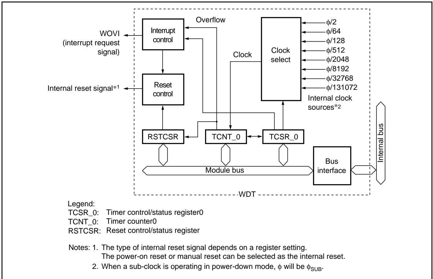
Figure 13.1 Block Diagram of WDT_0 (1)
