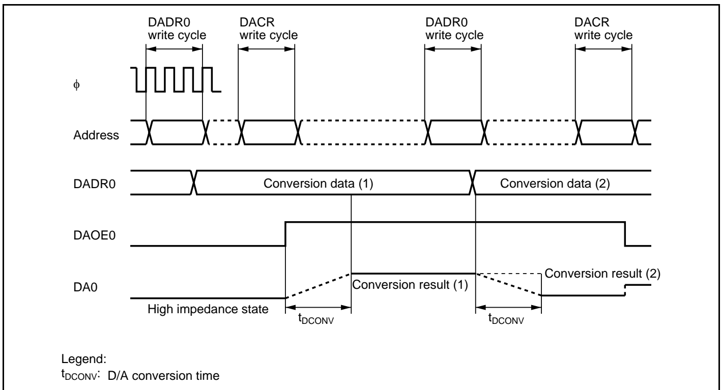
Figure 18.2 D/A Converter Operation Example
