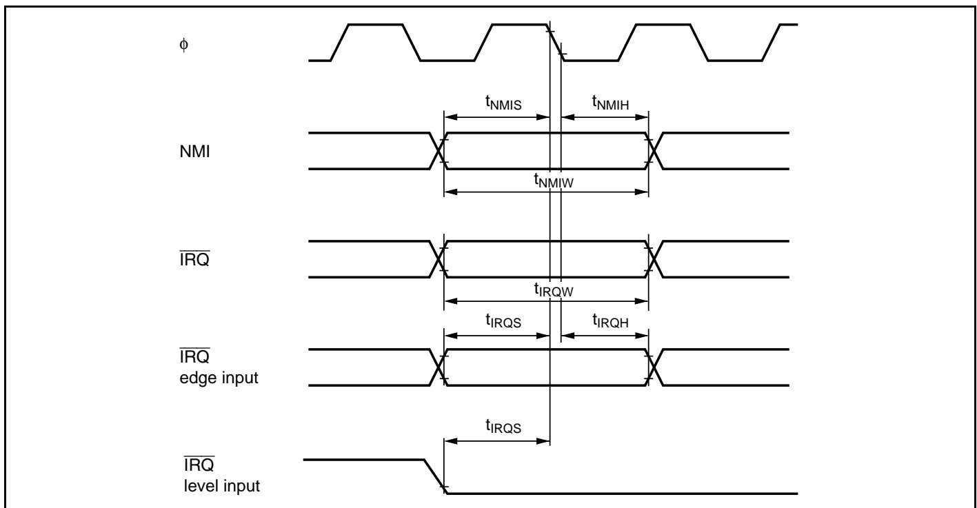
Figure 27.13 Interrupt Input Timing
