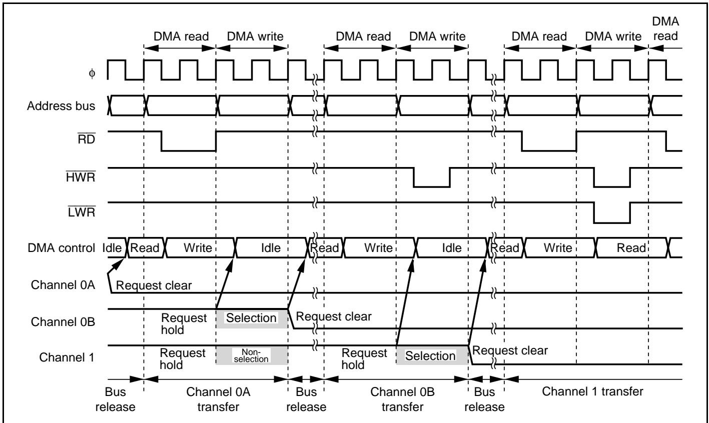
Figure 8.33 Example of Multi-Channel Transfer
