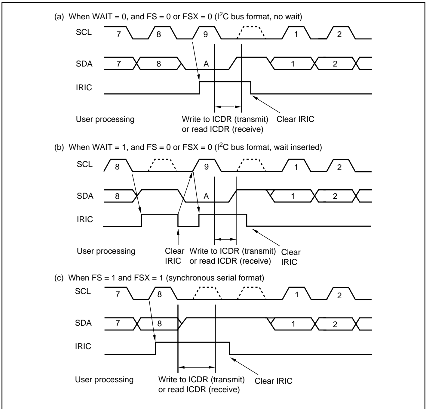
Figure 16.19 IRIC Setting Timing and SCL Control
