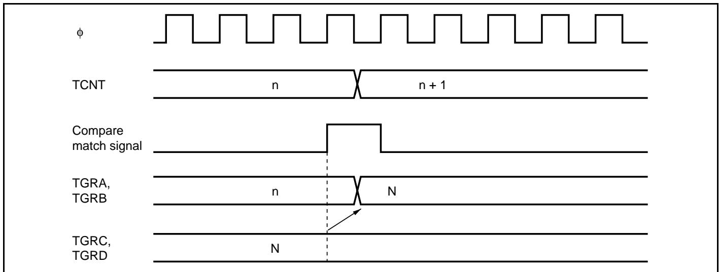
Figure 11.37 Buffer Operation Timing (Compare Match)
