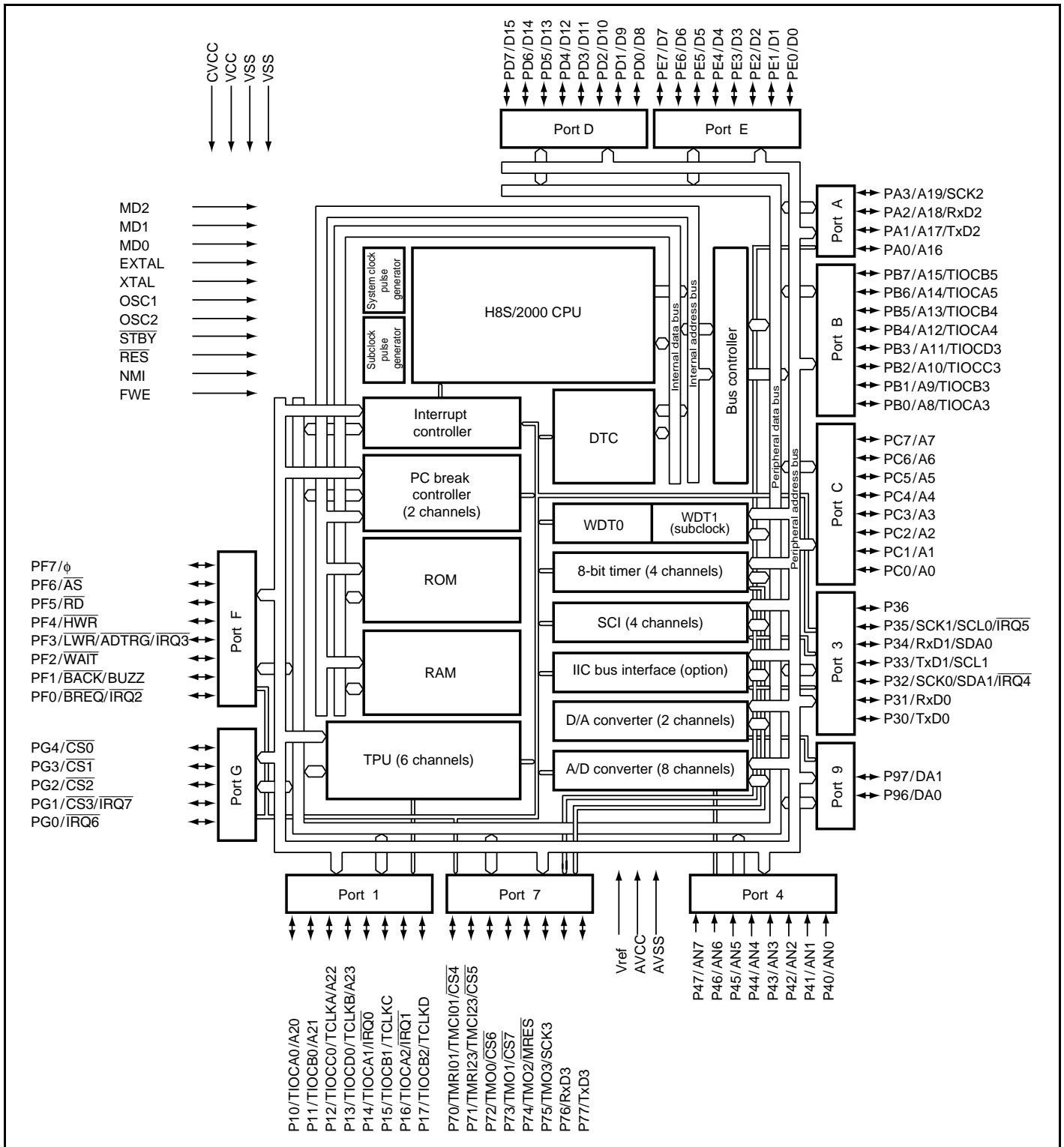
Figure 1.3 Internal Block Diagram of H8S/2238 Group
