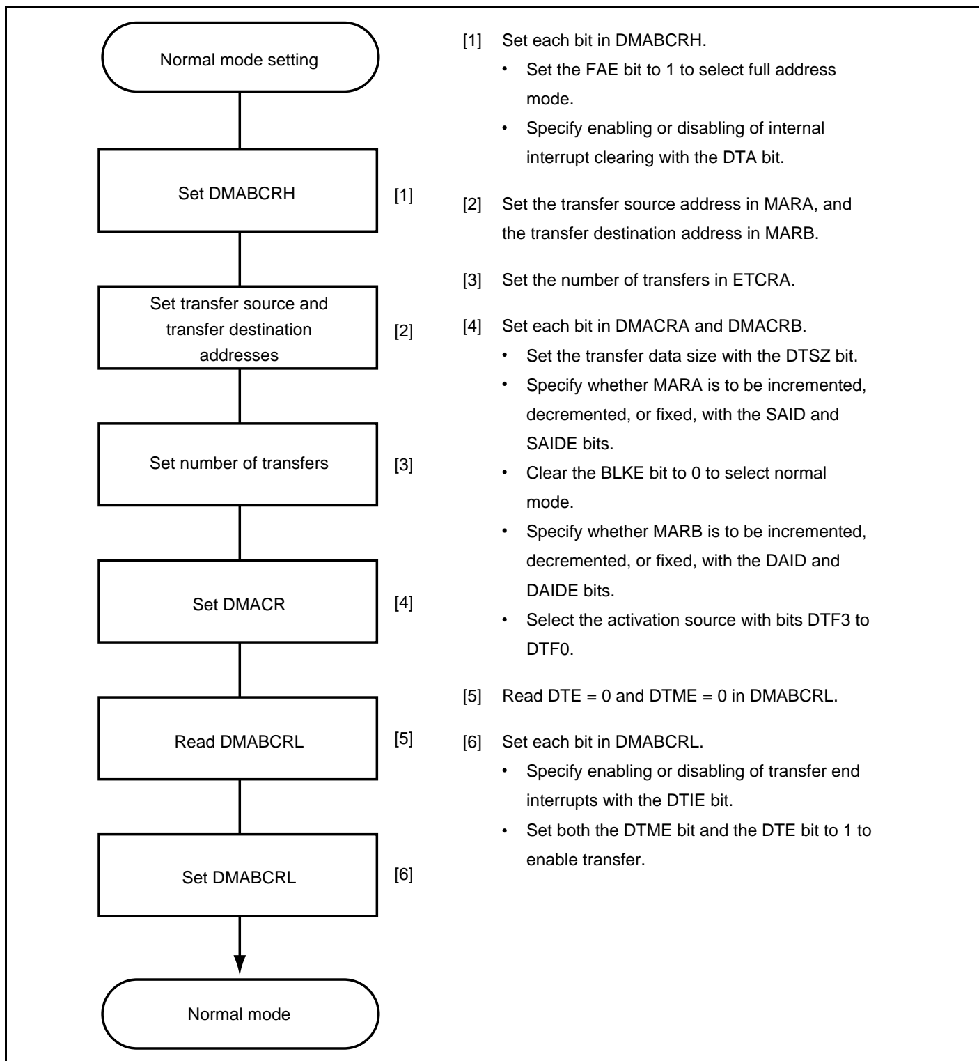
Figure 8.13 Example of Normal Mode Setting Procedure
