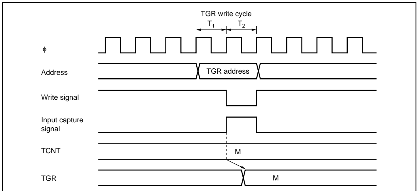
Figure 11.51 Contention between TGR Write and Input Capture
