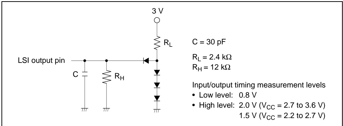
Figure 27.8 Output Load Circuit
