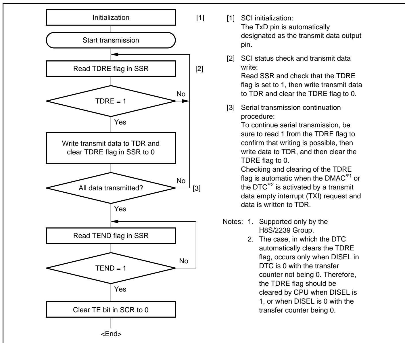
Figure 15.20 Sample Serial Transmission Flowchart
