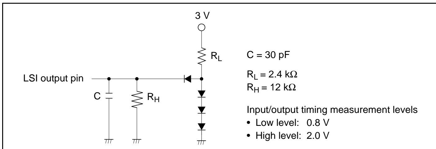
Figure 27.9 Output Load Circuit
