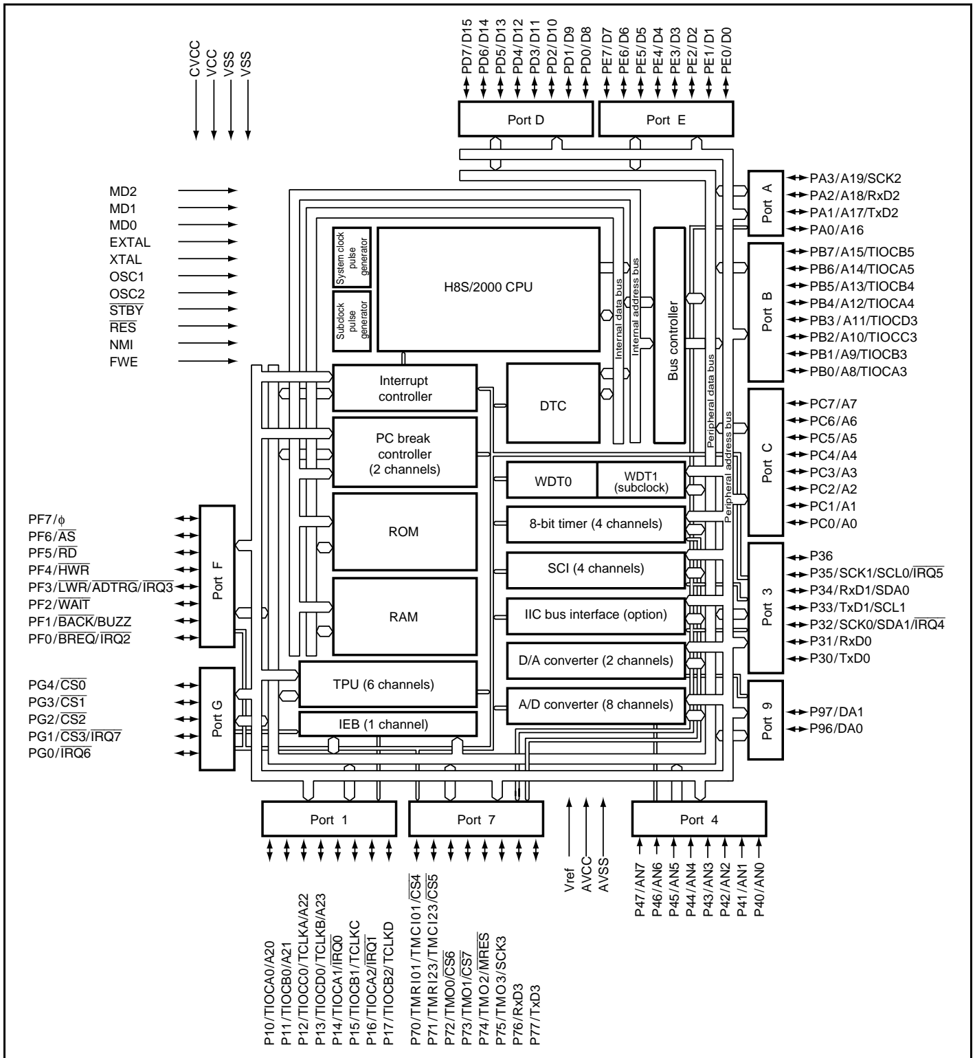
Figure 1.1 Internal Block Diagram of H8S/2258 Group
