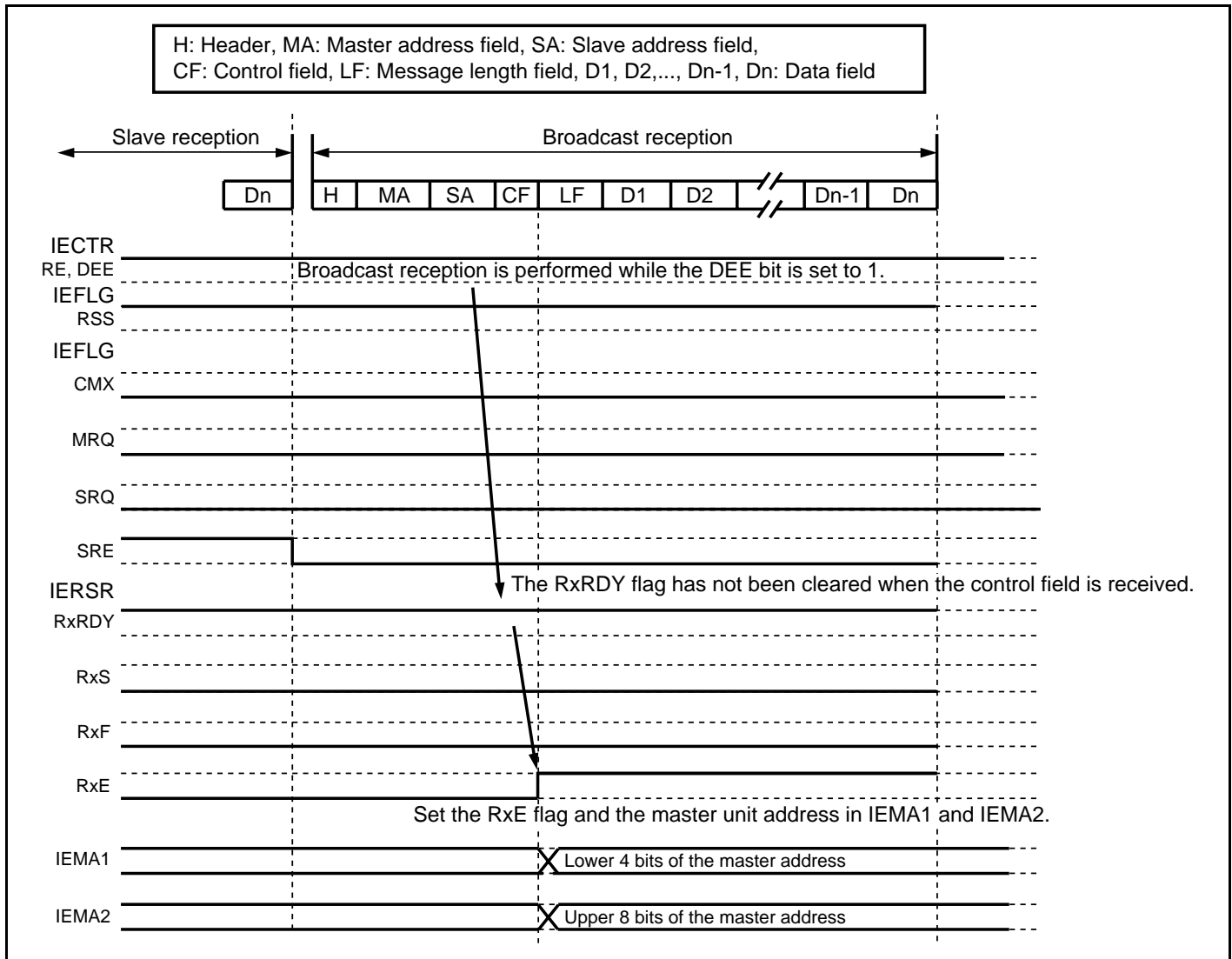
Figure 14.10 Error Occurrence in the Broadcast Reception (DEE = 1)
