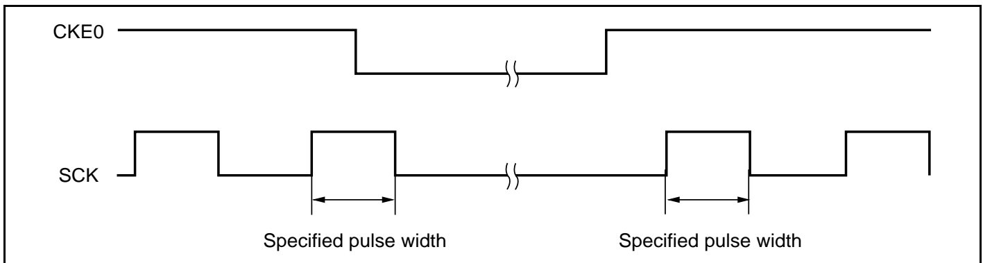
Figure 15.34 Timing for Fixing Clock Output Level
