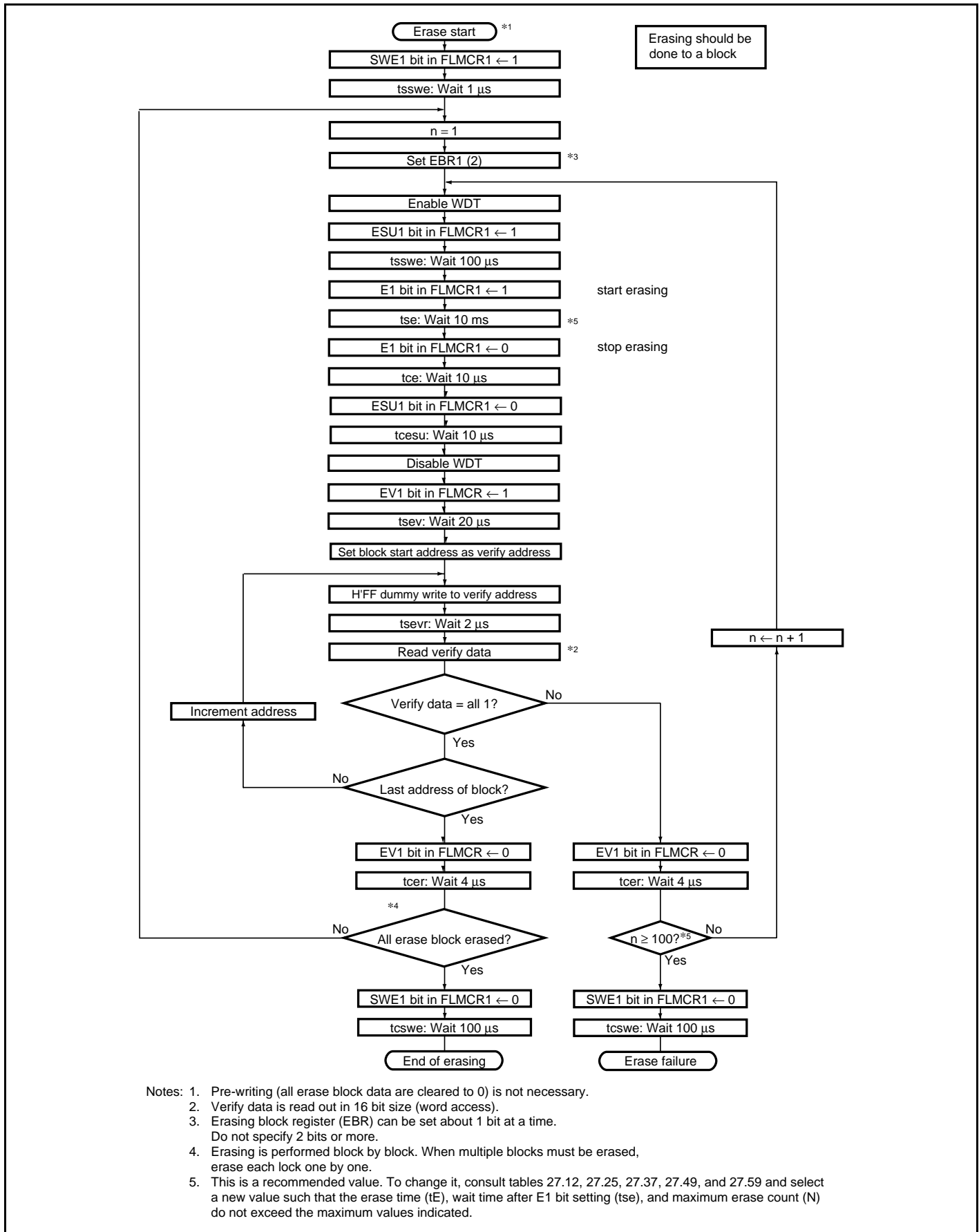
Figure 20.12 Erase/Eraser-Verify Flowchart
