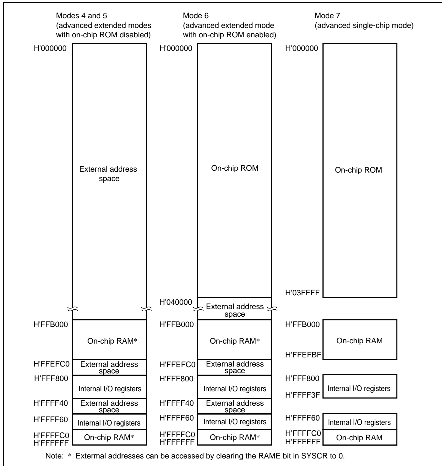
Figure 3.1 H8S/2258 Memory Map in Each Operating Mode
