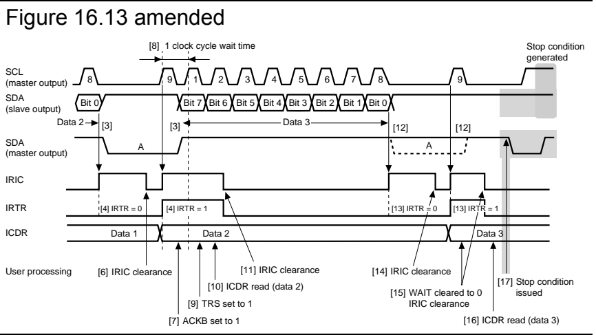
Figure 16.13 Example of Master Receive Mode top condition Generation Timing (MLS = ACKB = 0, WAIT = 1)
