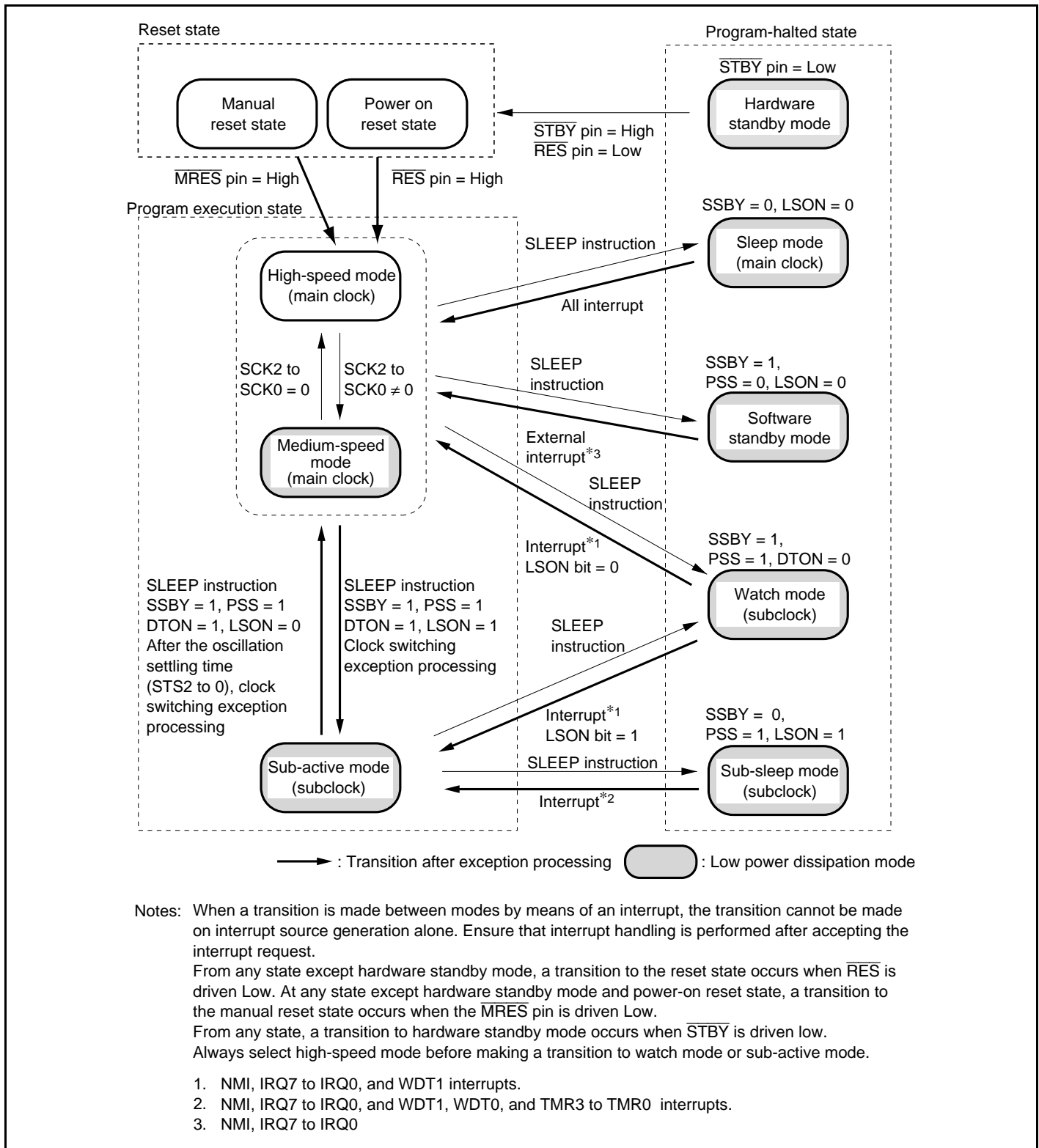
Figure 24.1 Mode Transition Diagram
