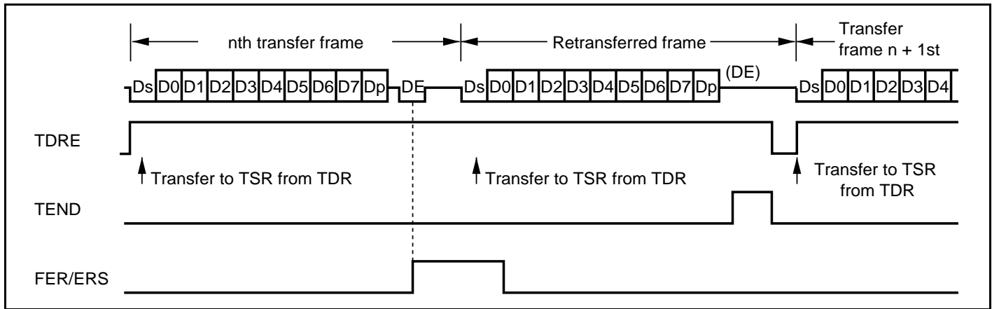
Figure 15.29 Retransfer Operation in SCI Transmit Mode
