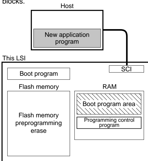
Figure 20.3 Boot Mode (Example)
