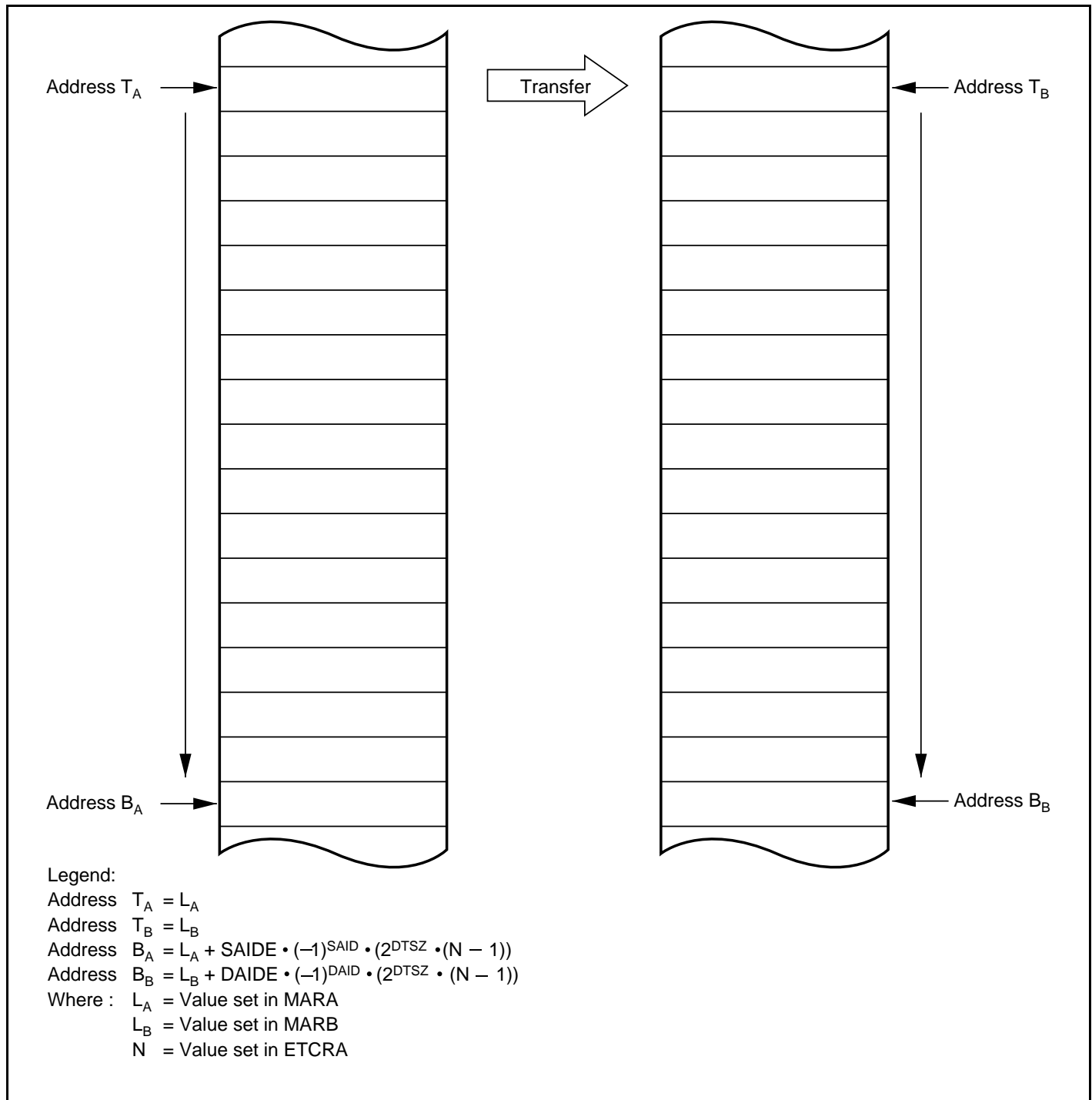
Figure 8.12 Operation in Normal Mode
