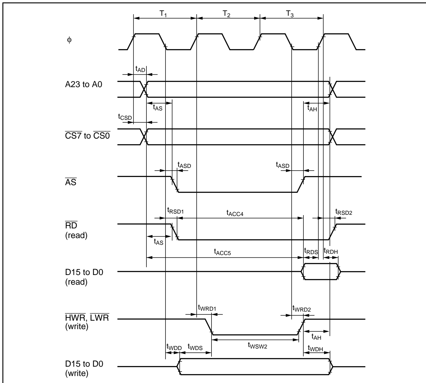
Figure 27.15 Basic Bus Timing (Three-State Access)
