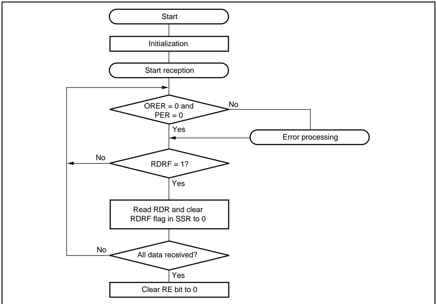
Figure 15.33 Example of Reception Processing Flow
