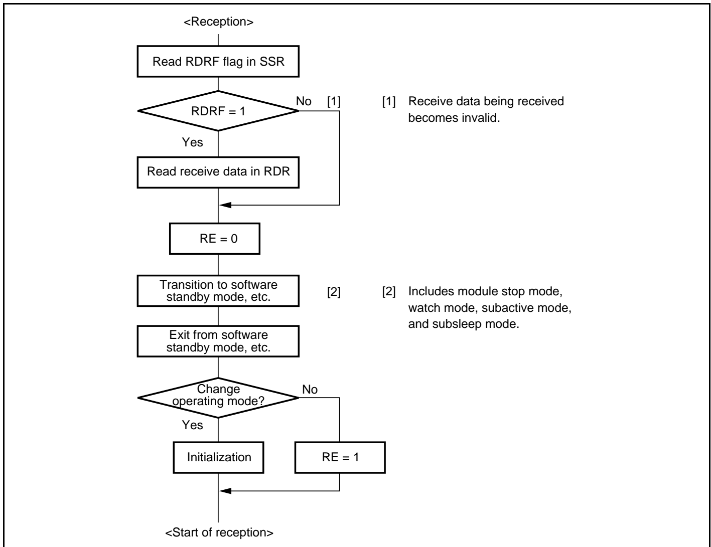
Figure 15.42 Sample Flowchart for Mode Transition during Reception
