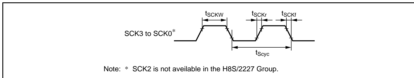
Figure 27.31 SCK Clock Input Timing
