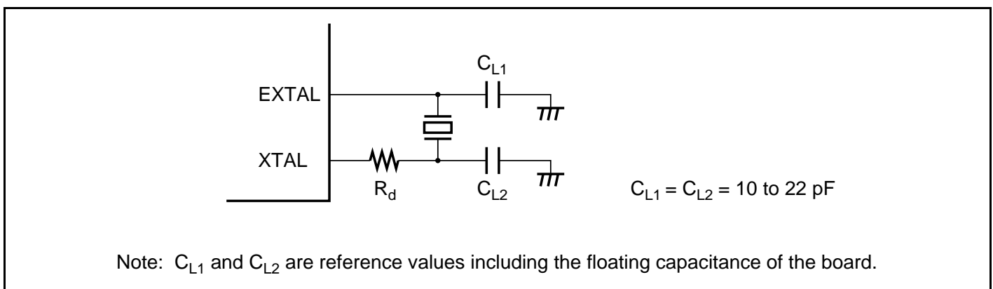
Figure 23.2 Connection of Crystal Resonator (Example)
