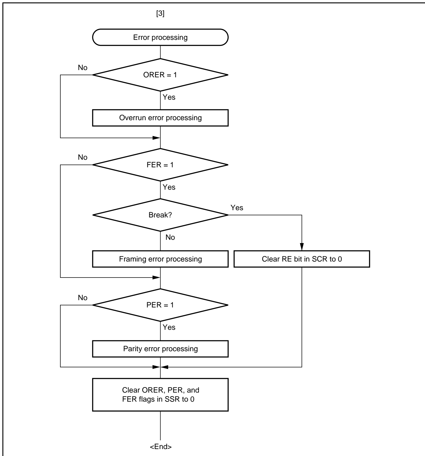
Figure 15.12 Sample Serial Reception Data Flowchart (2)
