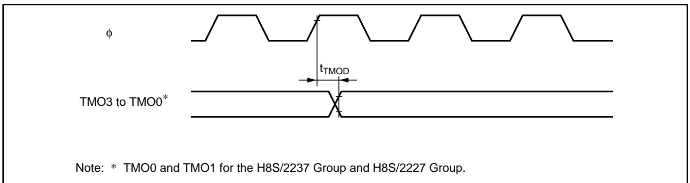
Figure 27.27 8-Bit Timer Output Timing
