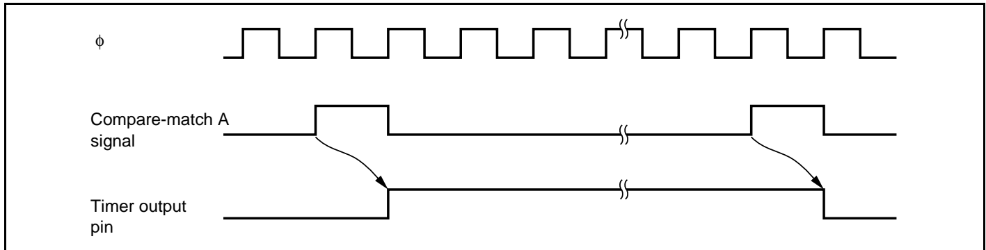
Figure 12.6 Timing of Timer Output
