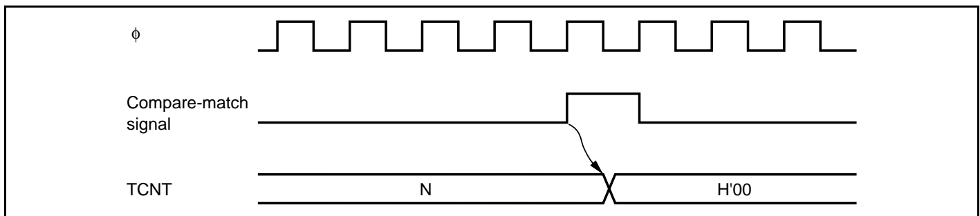
Figure 12.7 Timing of Compare-Match Clear
