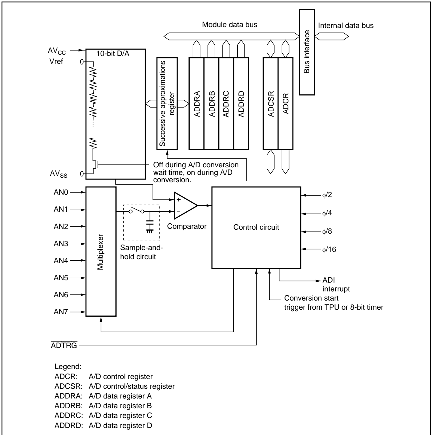
Figure 17.1 Block Diagram of A/D Converter
