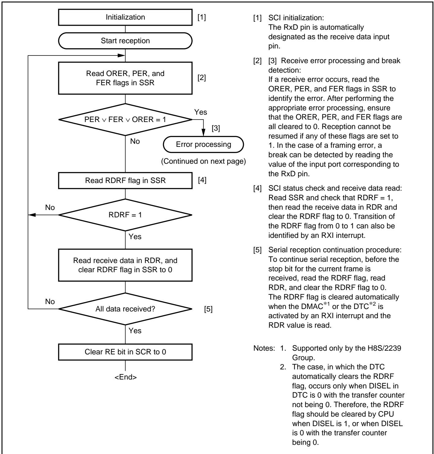
Figure 15.12 Sample Serial Reception Data Flowchart (1)
