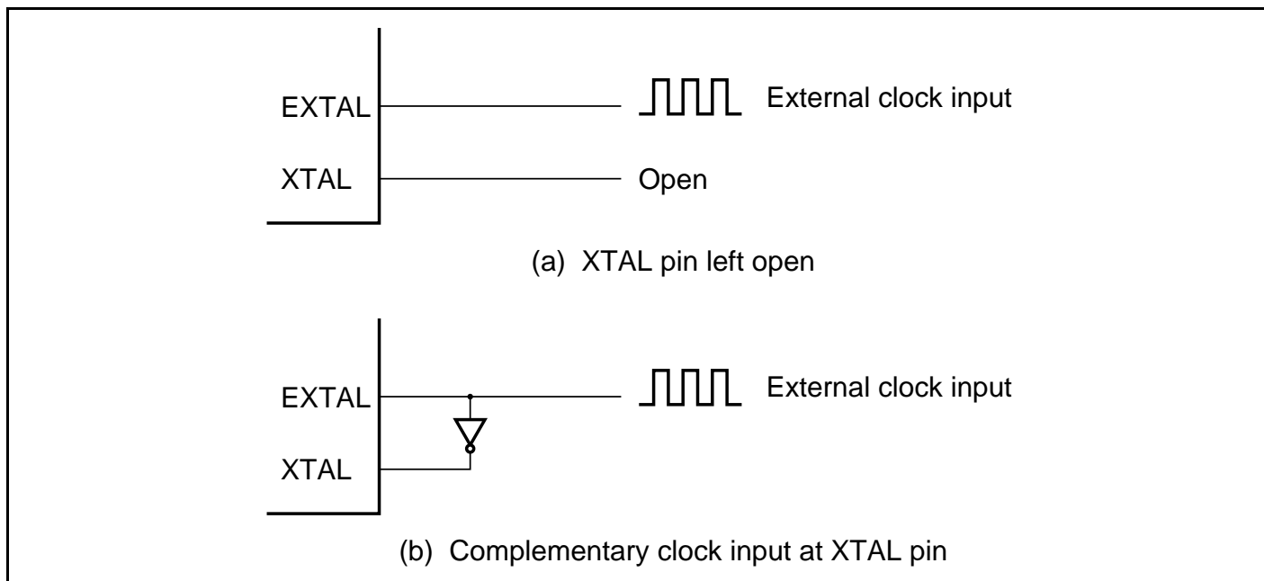
Figure 23.4 External Clock Input (Examples)
