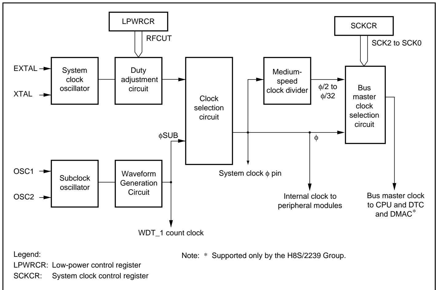
Figure 23.1 Block Diagram of Clock Pulse Generator
