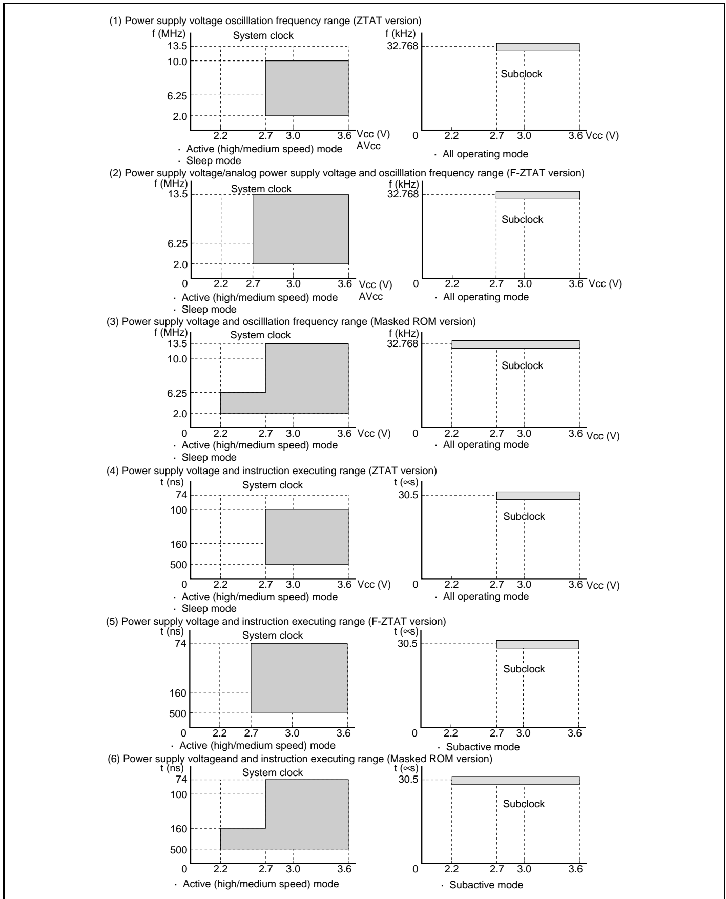
Figure 27.5 Power Supply Voltage and Operating Ranges (H8S/2237 Group and H8S/2227 Group)
