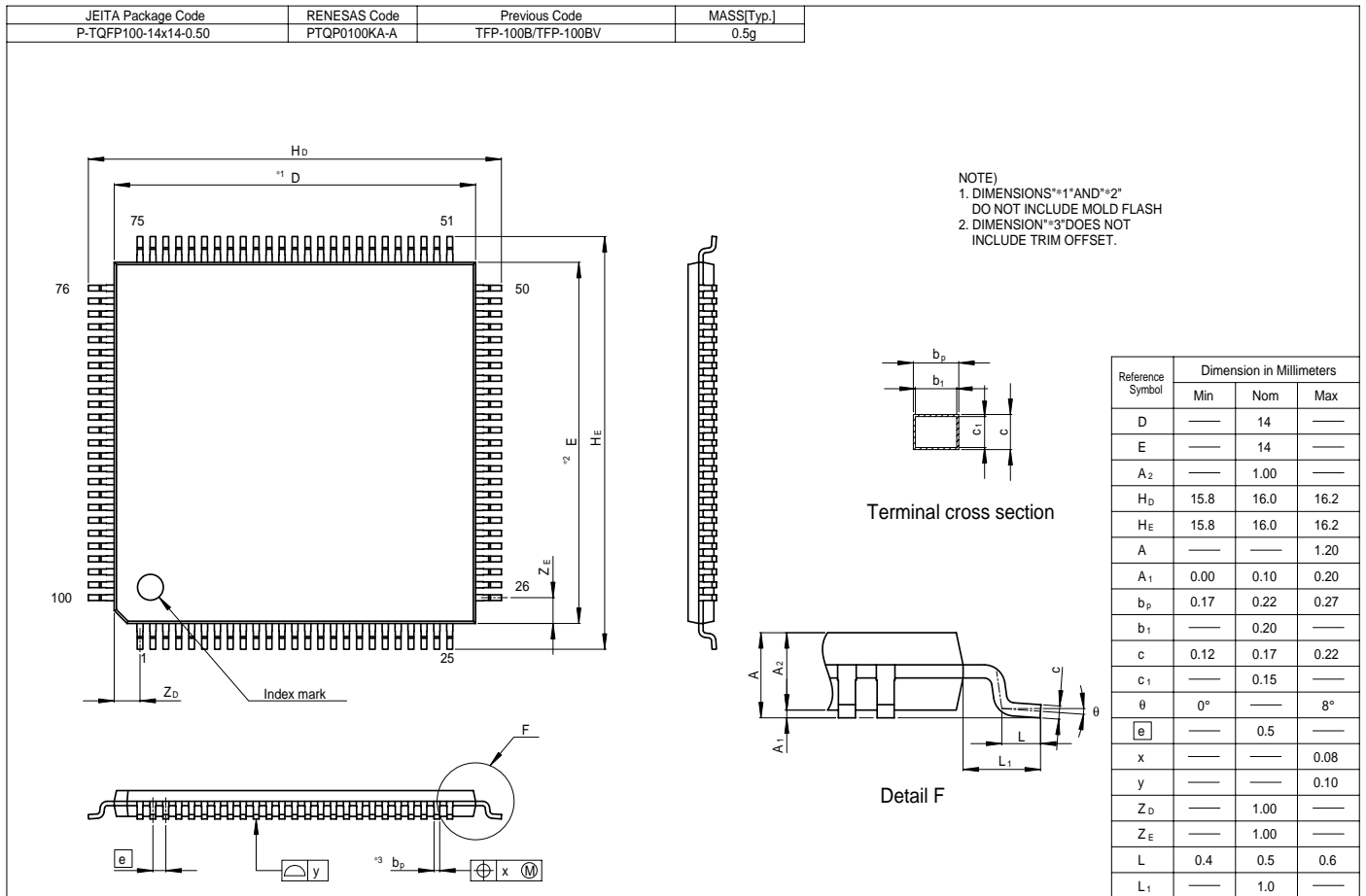
Figure C.1 TFP-100B Package Dimensions
