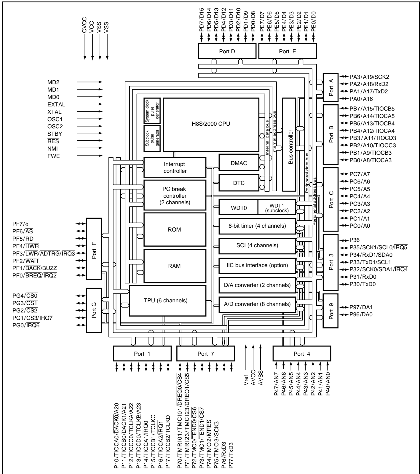
Figure 1.2 Internal Block Diagram of H8S/2239 Group
