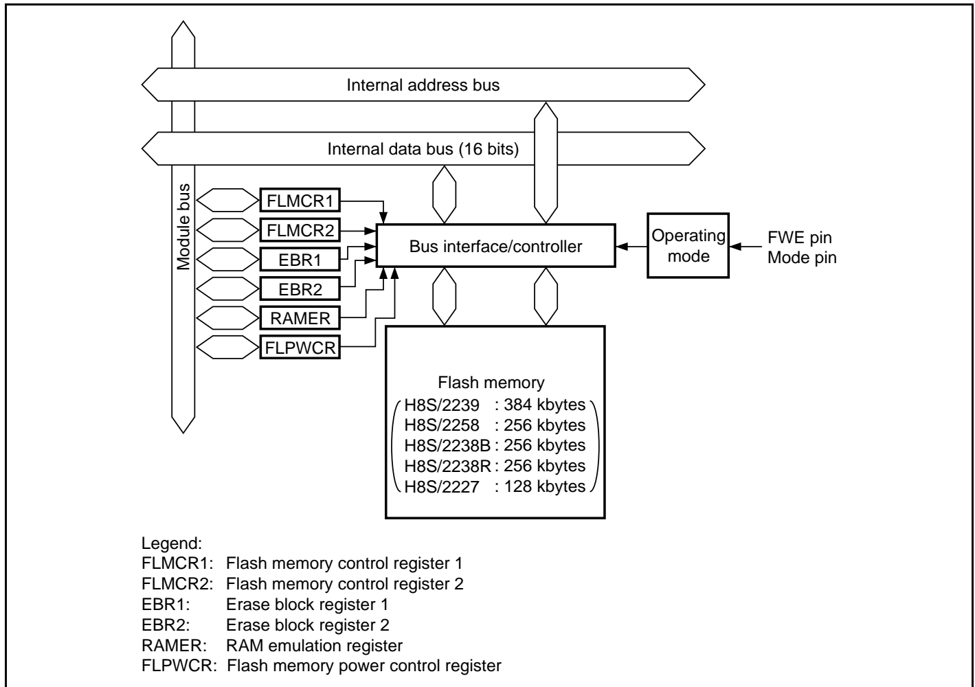
Figure 20.1 Block Diagram of Flash Memory
