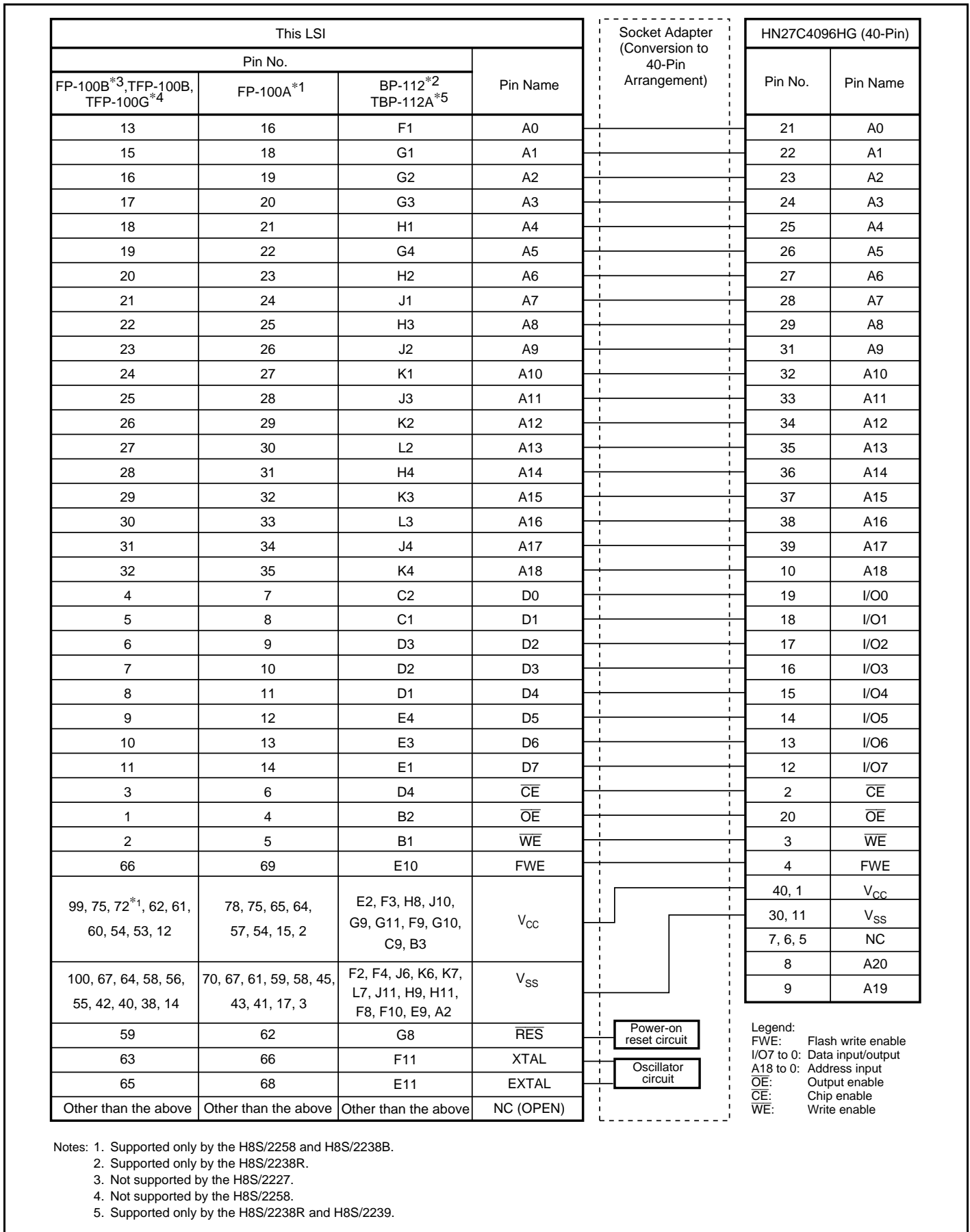
Figure 20.13 Socket Adapter Pin Correspondence Diagram
