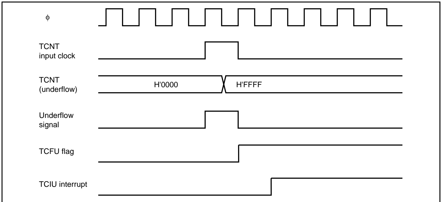
Figure 11.42 TCIU Interrupt Setting Timing
