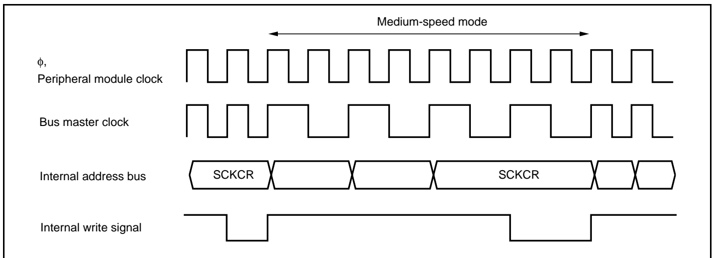
Figure 24.2 Medium-Speed Mode Transition and Clearance Timing
