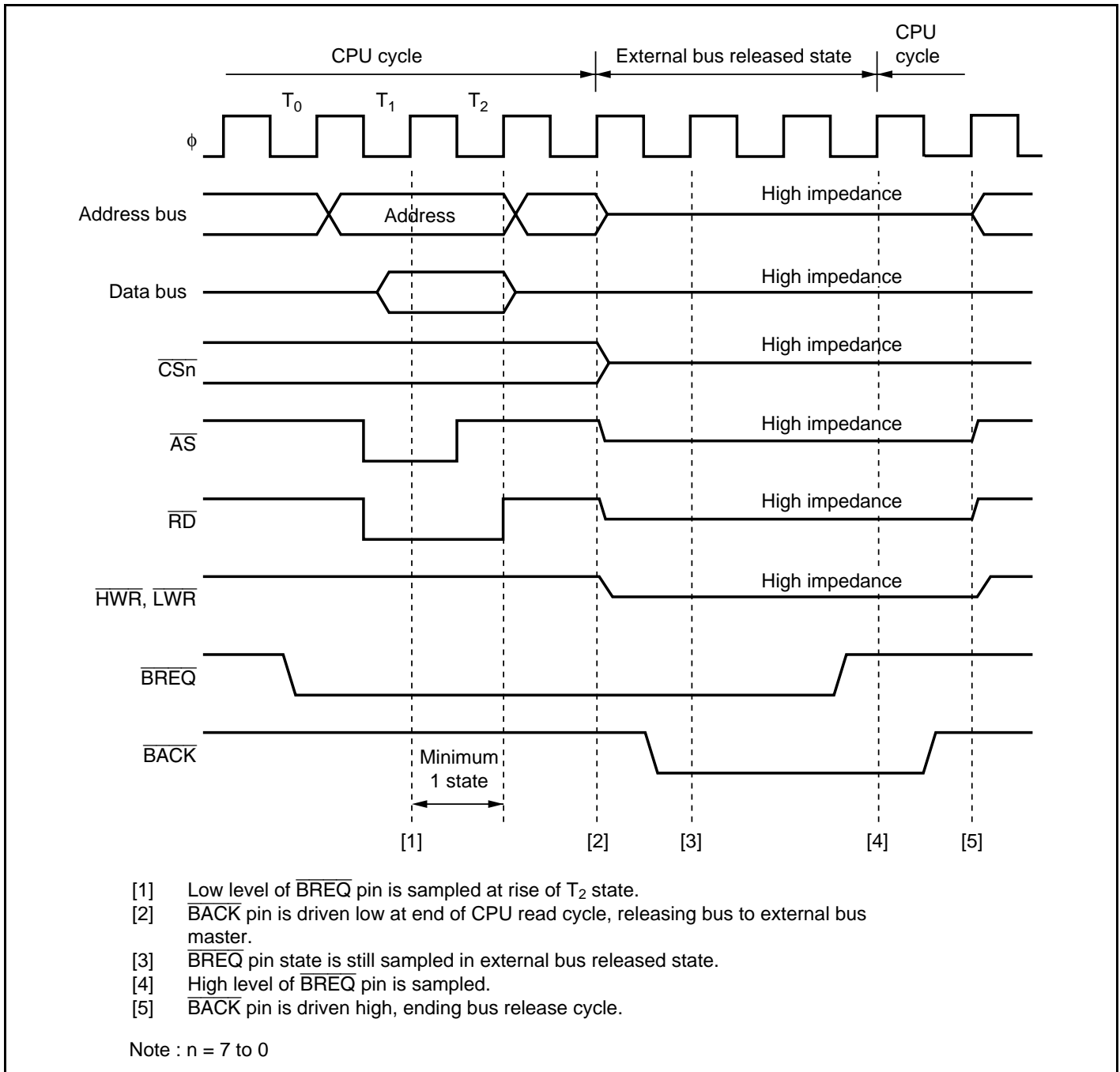
Figure 7.24 Bus-Released State Transition Timing
