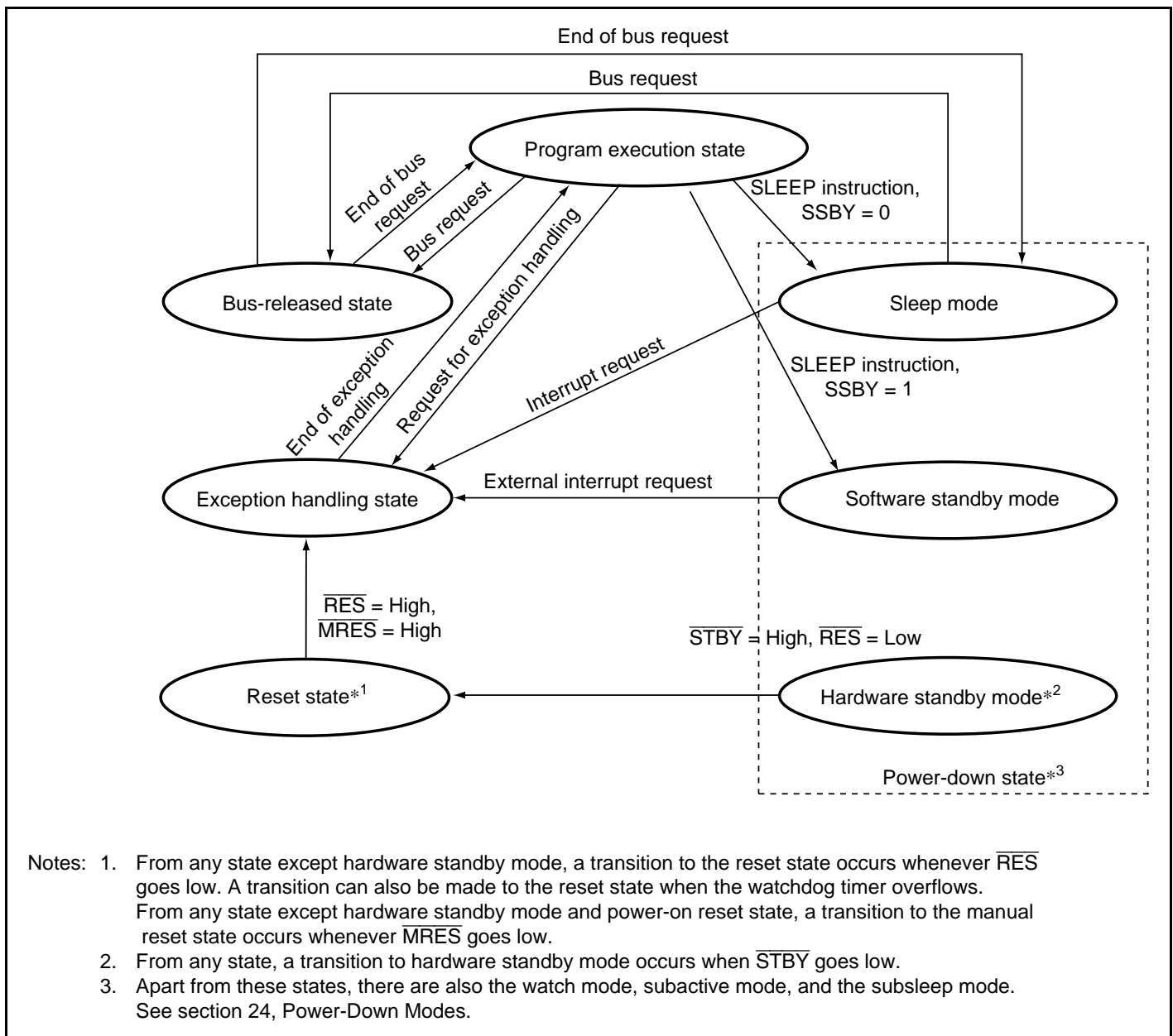
Figure 2.13 State Transitions
