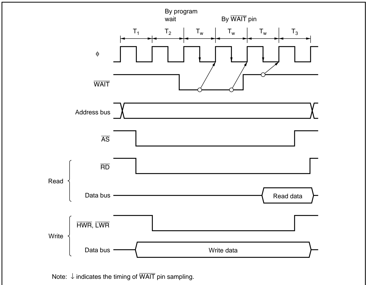
Figure 7.18 Example of Wait State Insertion Timing
