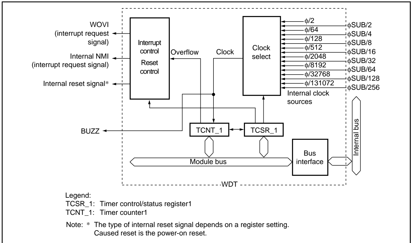
Figure 13.1 Block Diagram of WDT_1 (2)
