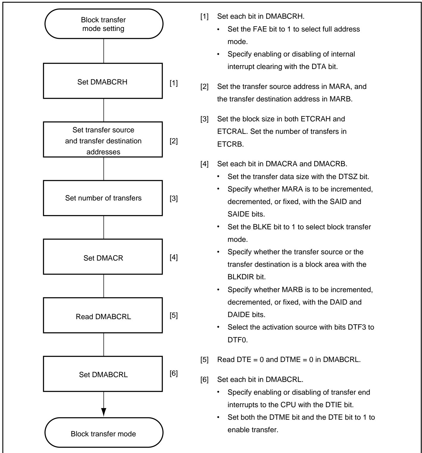
Figure 8.17 Example of Block Transfer Mode Setting Procedure
