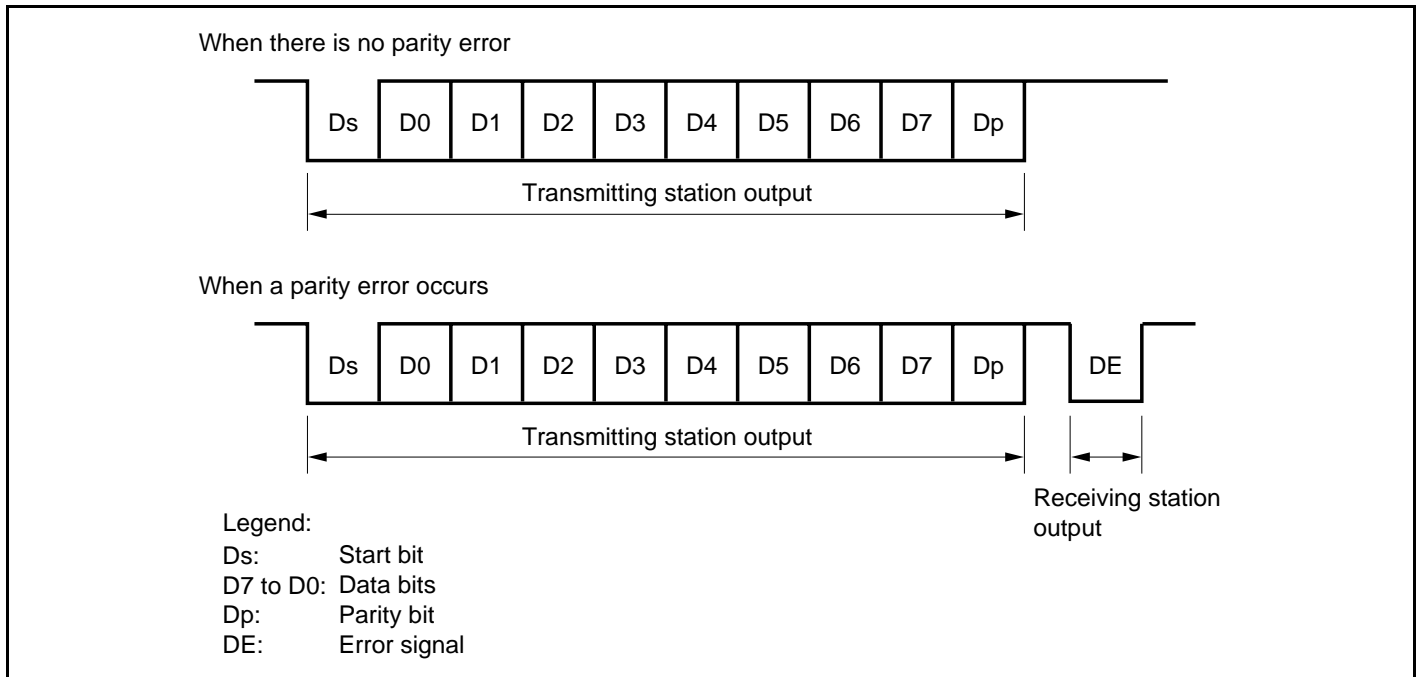
Figure 15.25 Normal Smart Card Interface Data Format
