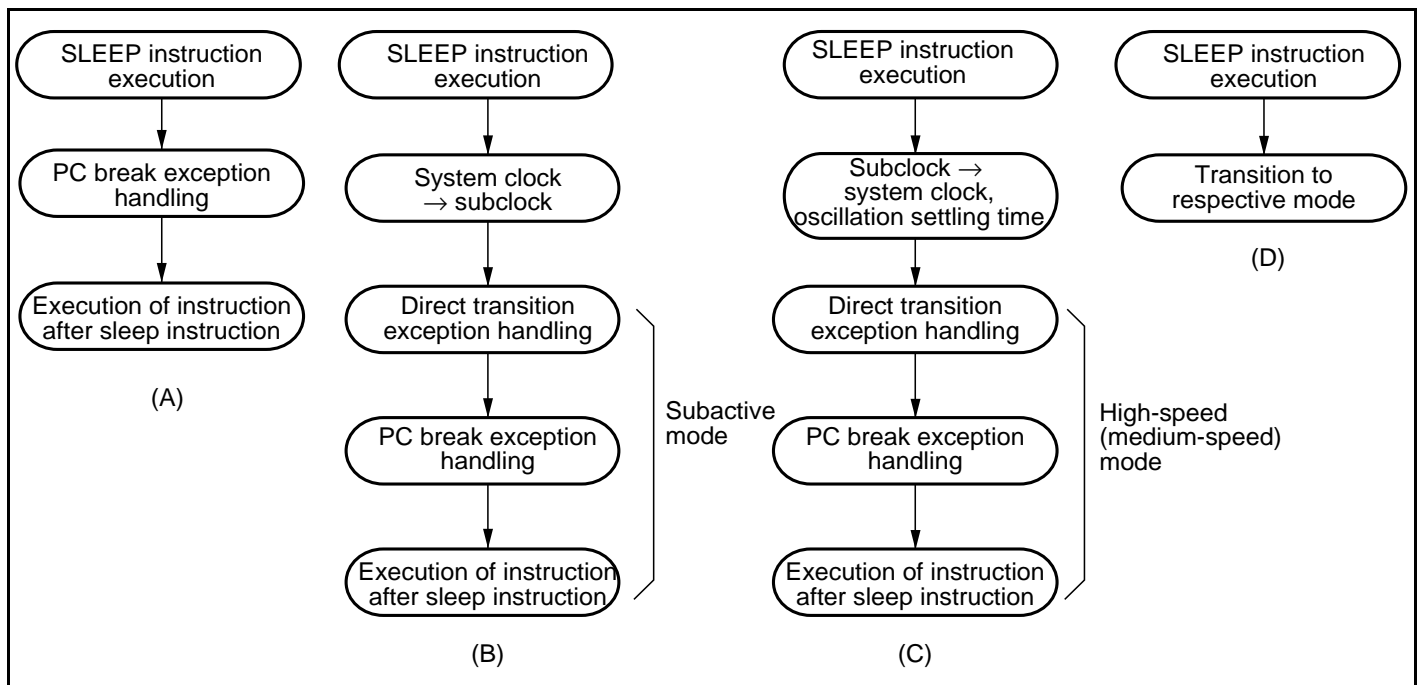
Figure 6.2 Operation in Power-Down Mode Transitions
