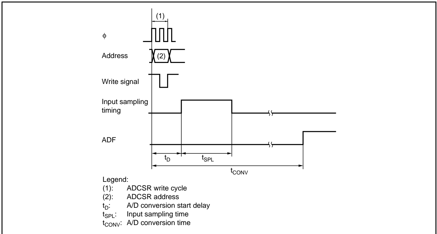
Figure 17.5 A/D Conversion Timing
