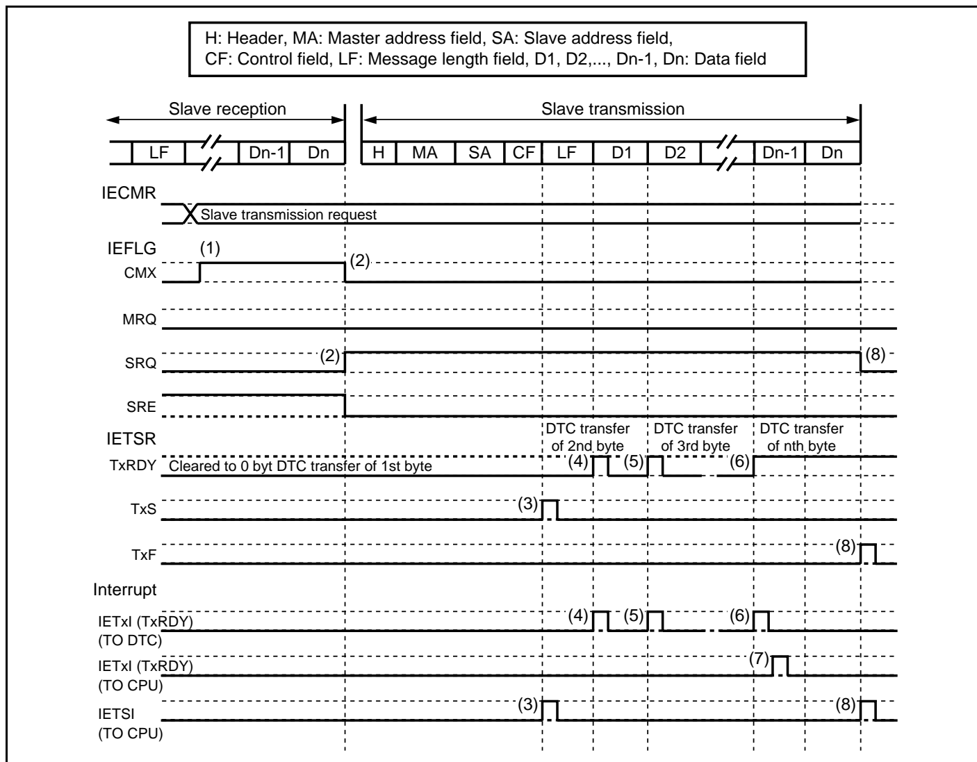
Figure 14.12 Slave Transmit Operation Timing
