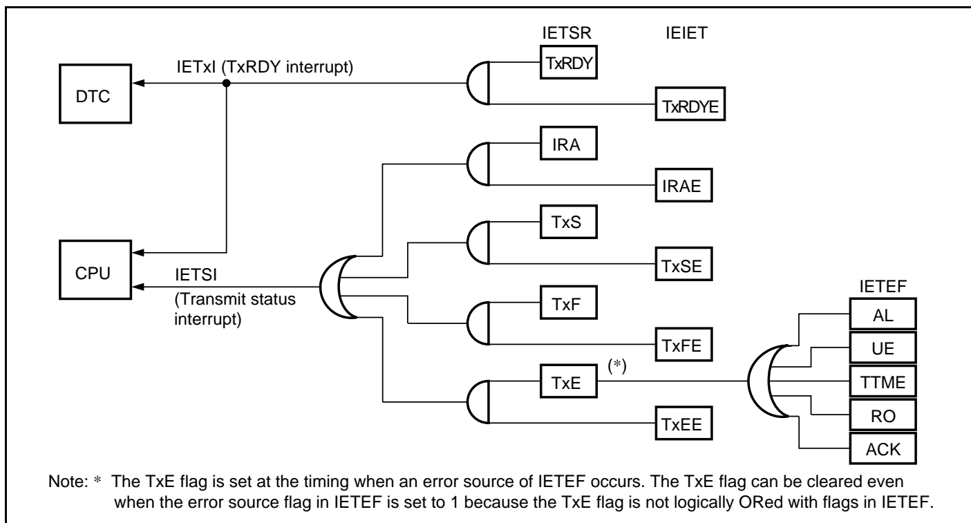
Figure 14.13 Relationships among Transfer Interrupt Sources
