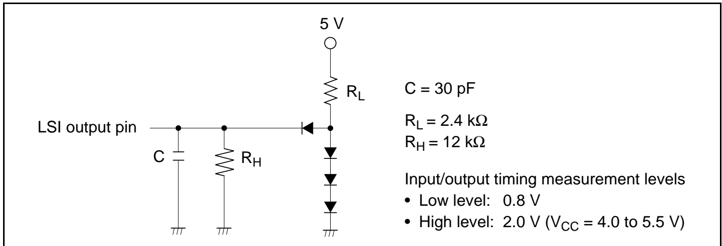
Figure 27.6 Output Load Circuit
