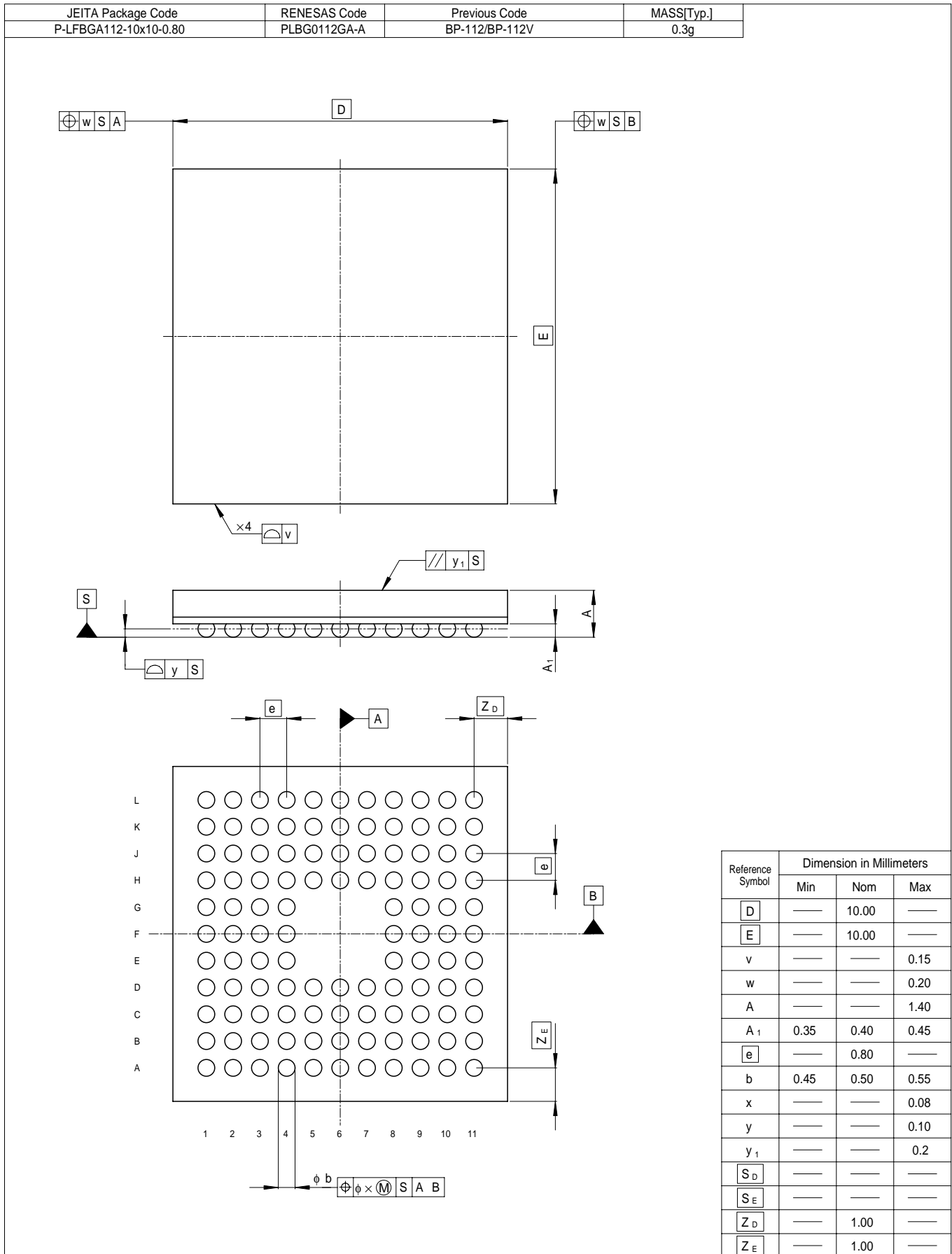
Figure C.5 BP-112 Package Dimensions
