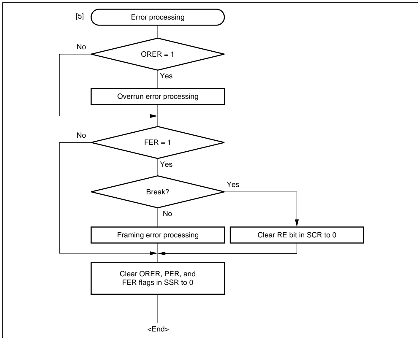
Figure 15.16 Sample Multiprocessor Serial Reception Flowchart (2)
