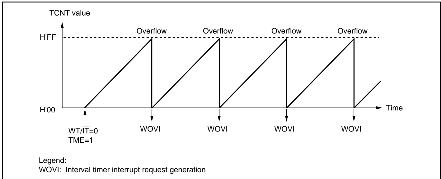
Figure 13.3 Interval Timer Mode Operation
