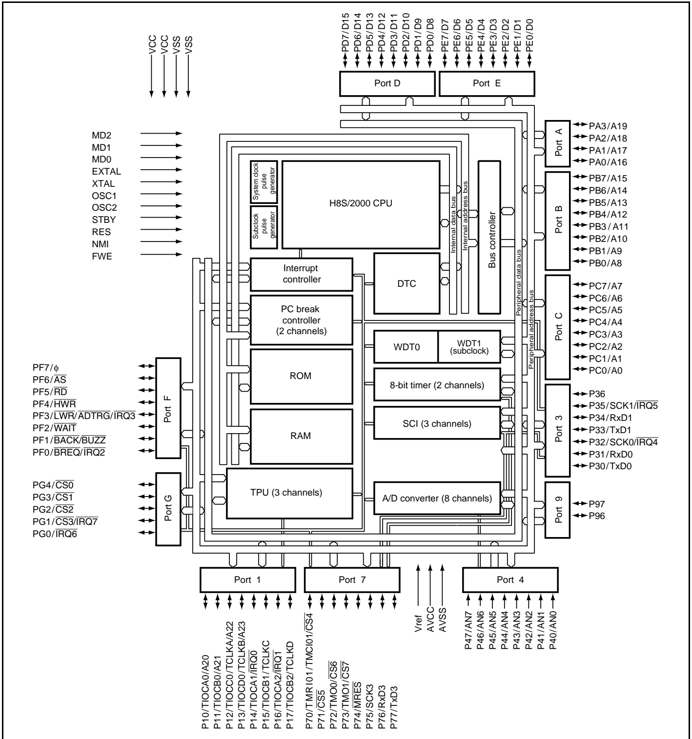
Figure 1.5 Internal Block Diagram of H8S/2227 Group
