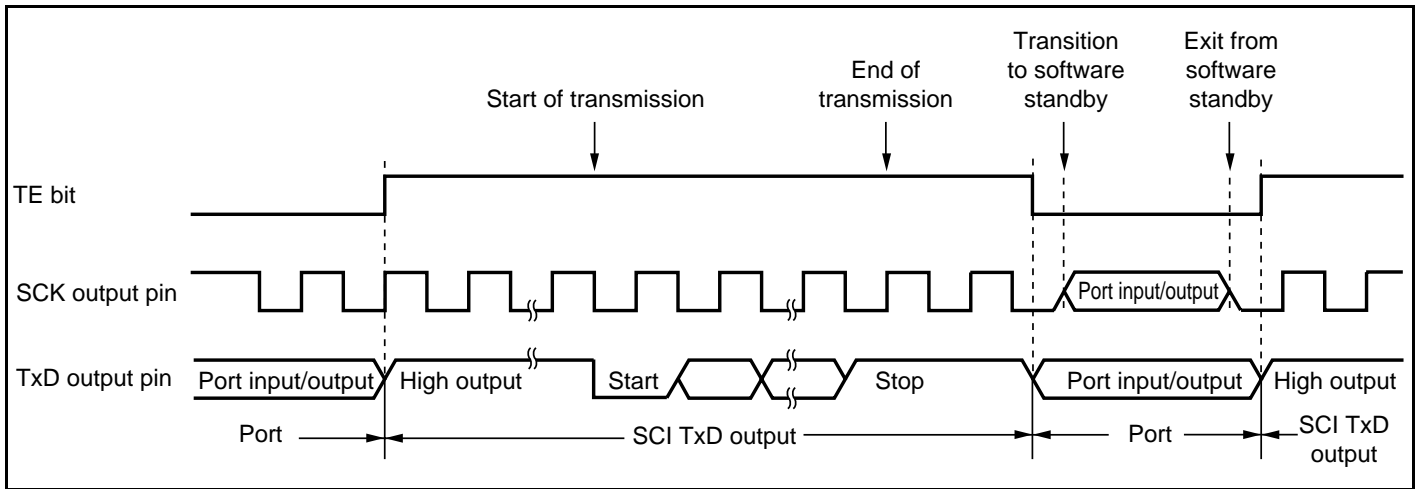
Figure 15.40 Asynchronous Transmission Using Internal Clock
