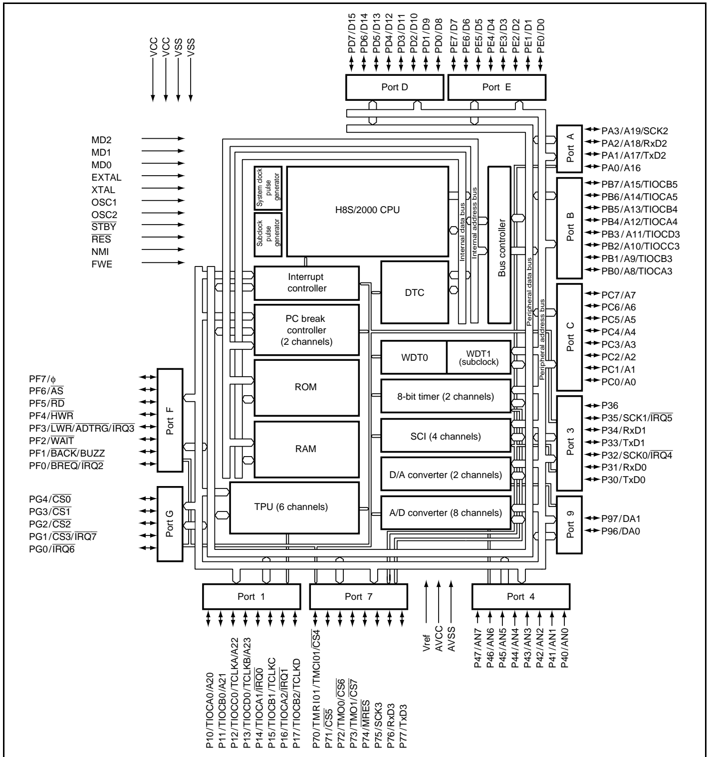
Figure 1.4 Internal Block Diagram of H8S/2237 Group
