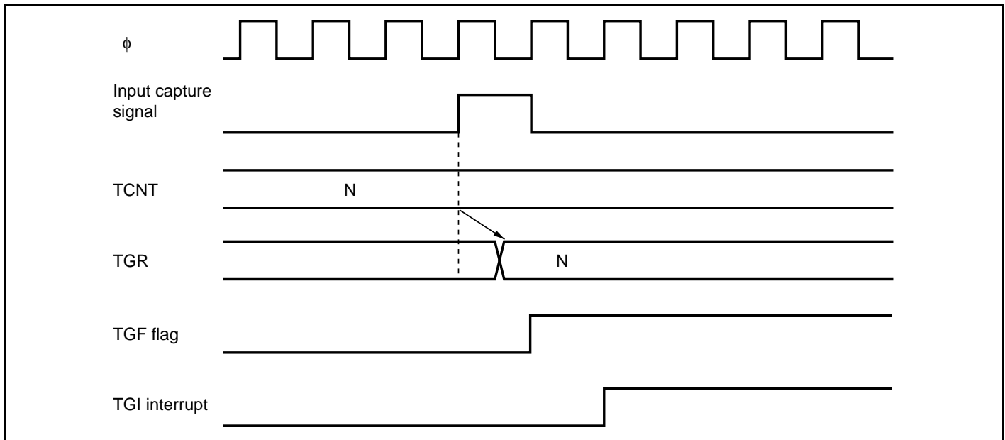
Figure 11.40 TGI Interrupt Timing (Input Capture)
