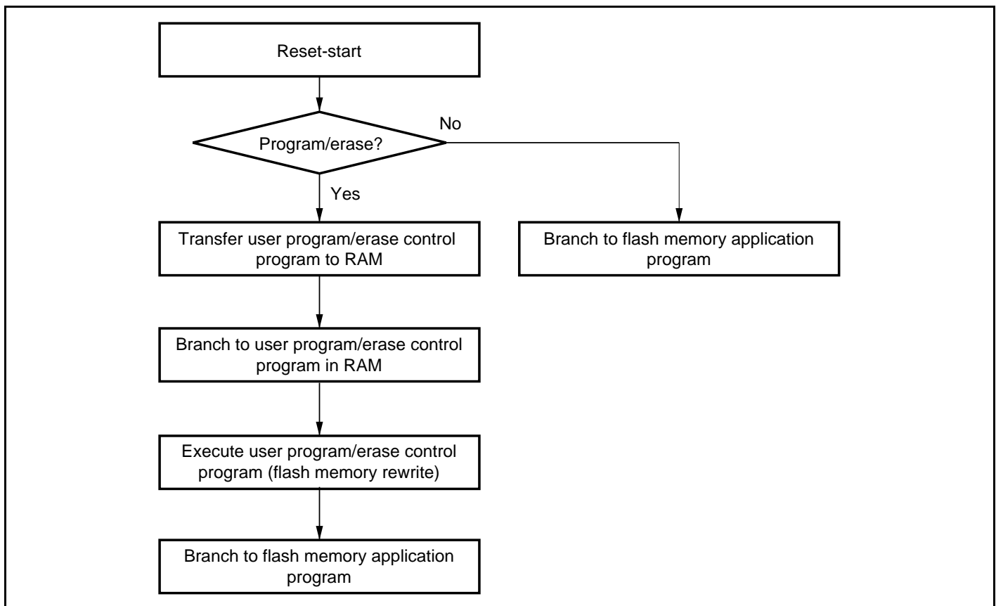
Figure 20.8 Programming/Erasing Flowchart Example in User Program Mode
