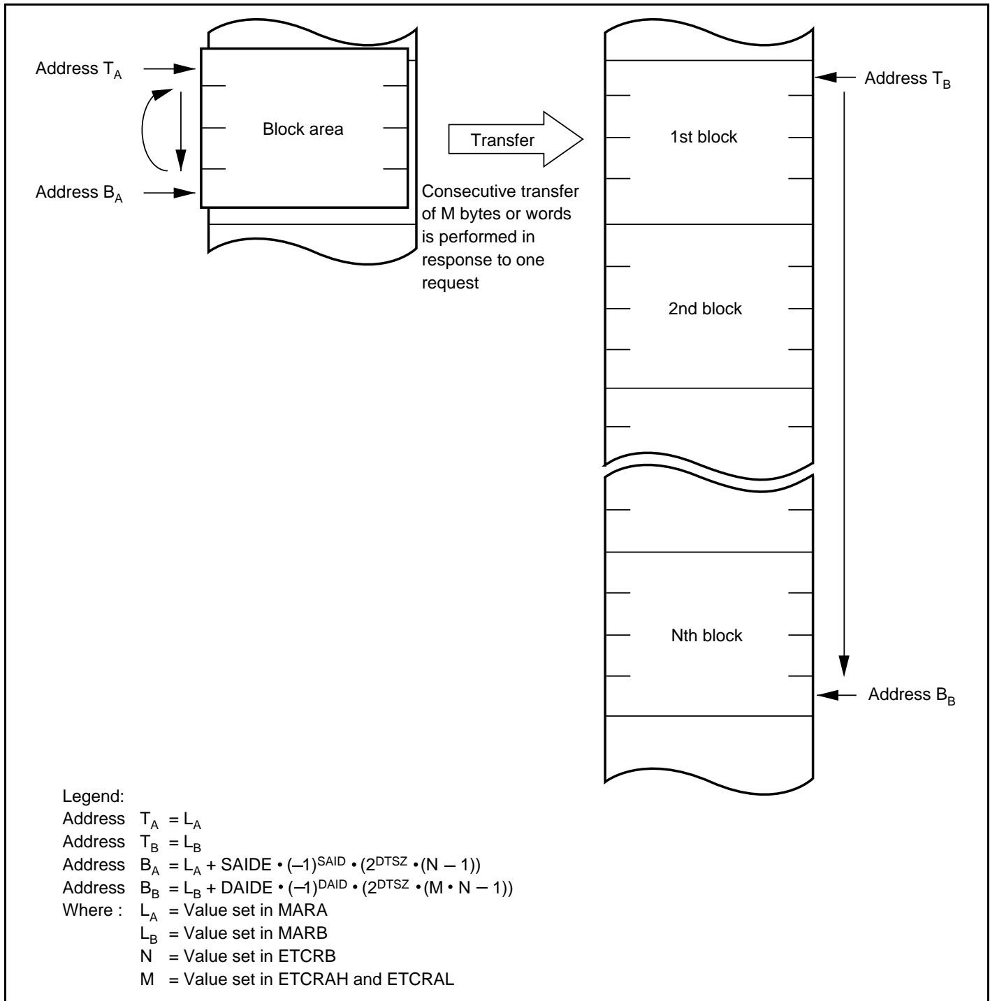
Figure 8.15 Operation in Block Transfer Mode (BLKDIR = 1)
