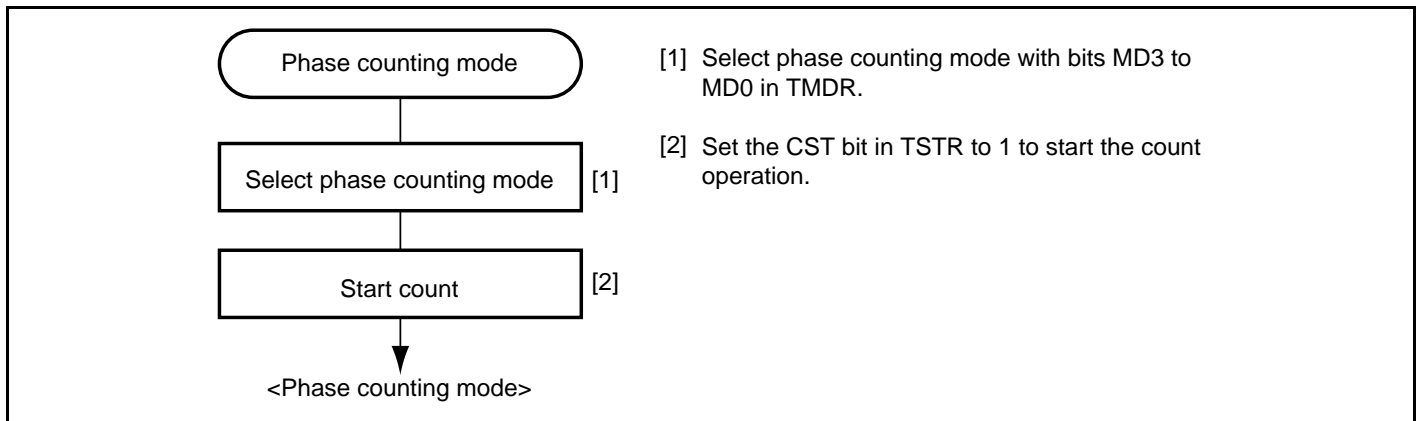
Figure 11.25 Example of Phase Counting Mode Setting Procedure
