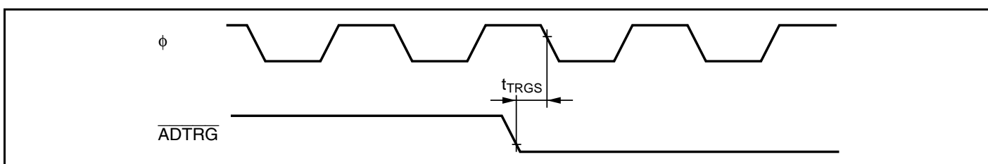
Figure 27.33 A/D Converter External Trigger Input Timing
