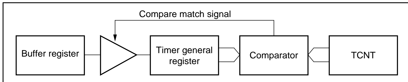
Figure 11.13 Compare Match Buffer Operation
