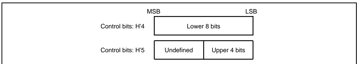
Figure 14.4 Locked Address Configuration
