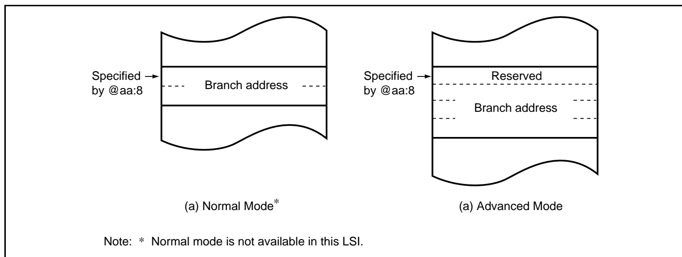
Figure 2.12 Branch Address Specification in Memory Indirect Mode
