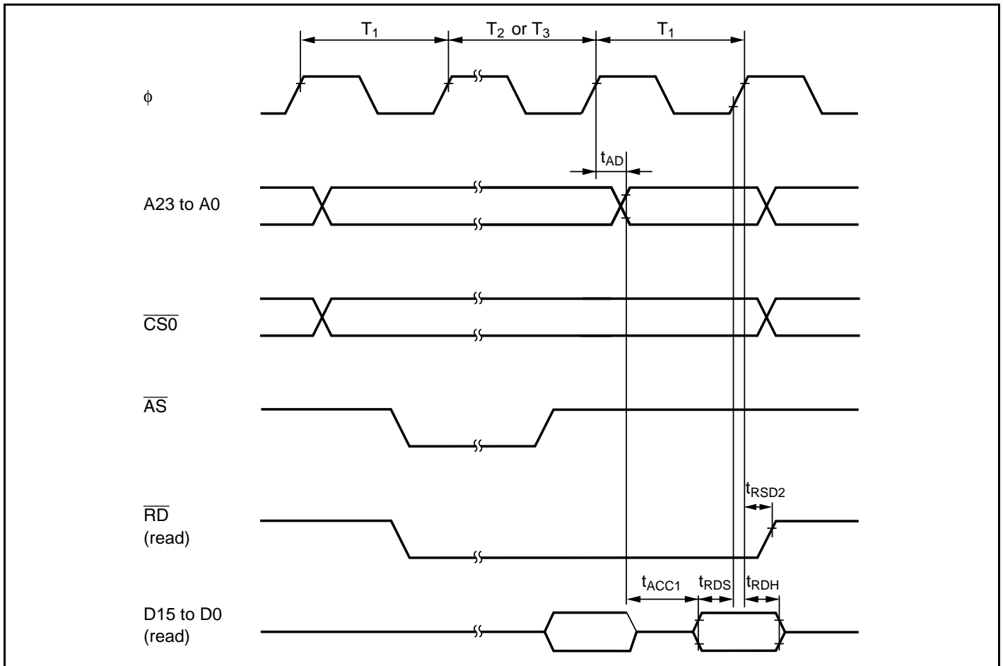
Figure 27.18 Burst ROM Access Timing (One-State Access)
