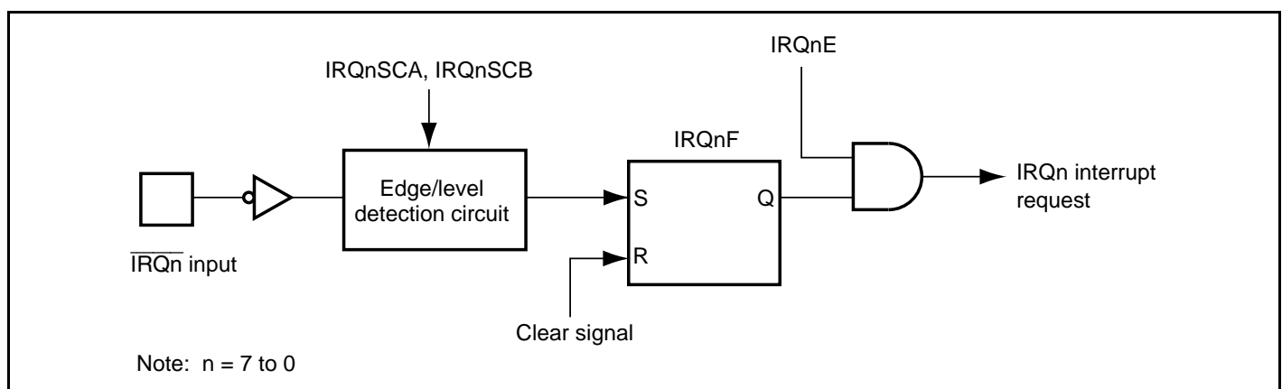
Figure 5.2 Block Diagram of IRQn Interrupts
