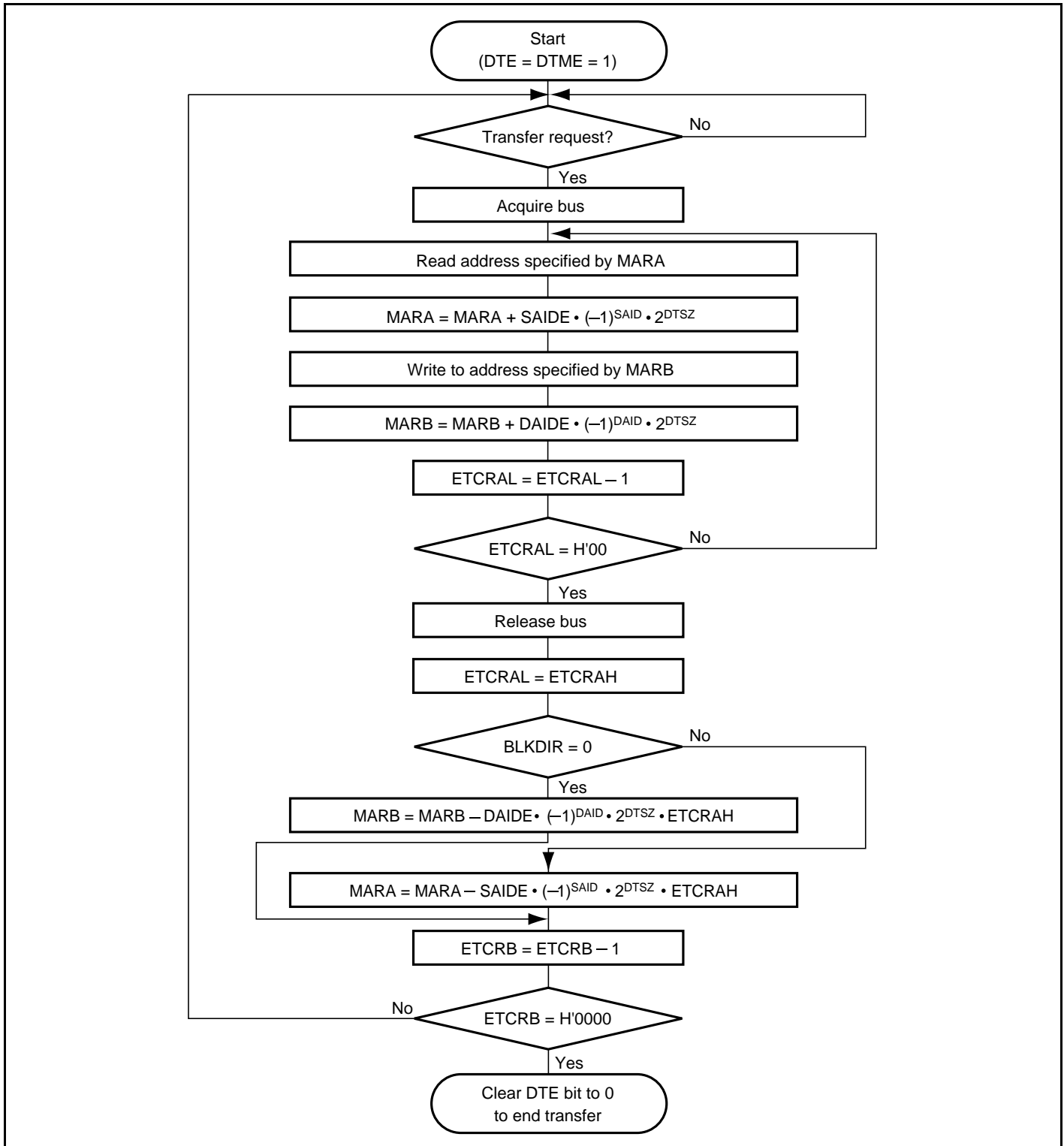
Figure 8.16 Operation Flow in Block Transfer Mode
