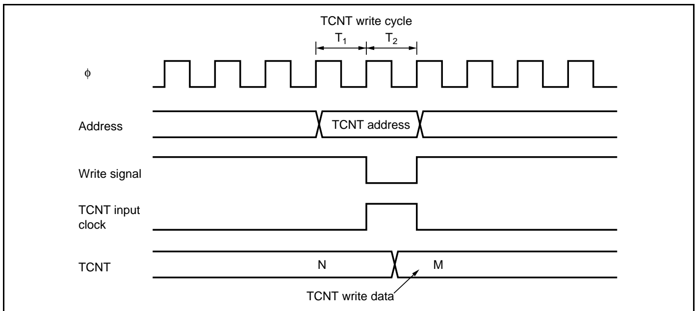
Figure 11.47 Contention between TCNT Write and Increment Operations
