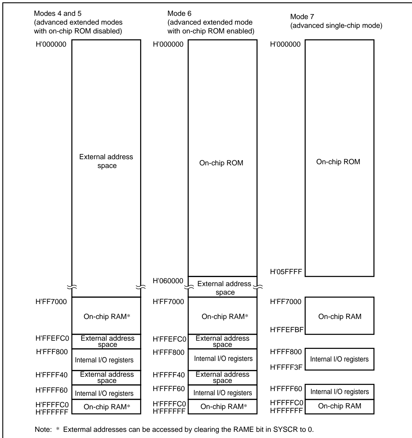
Figure 3.3 H8S/2239 Memory Map in Each Operating Mode
