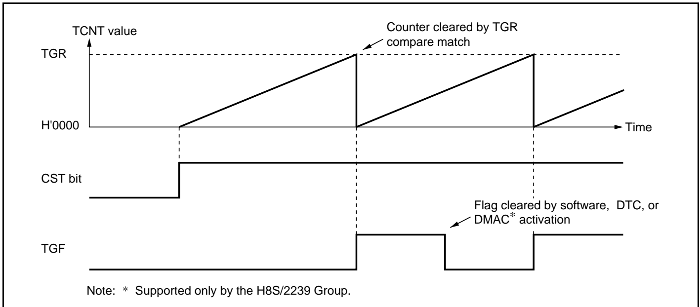
Figure 11.5 Periodic Counter Operation
