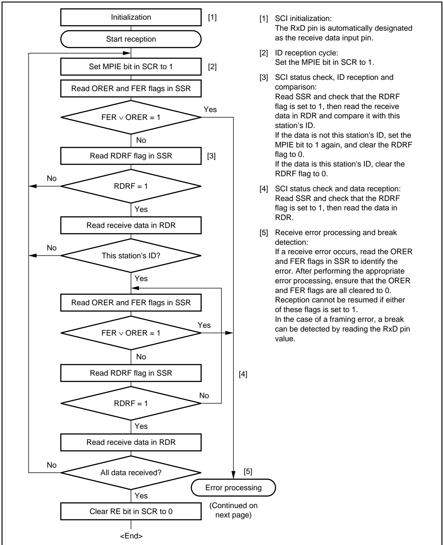
Figure 15.16 Sample Multiprocessor Serial Reception Flowchart (1)
