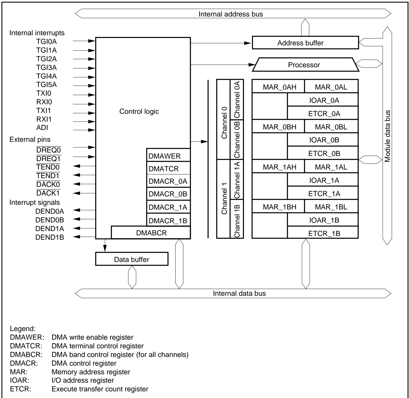
Figure 8.1 Block Diagram of DMAC
