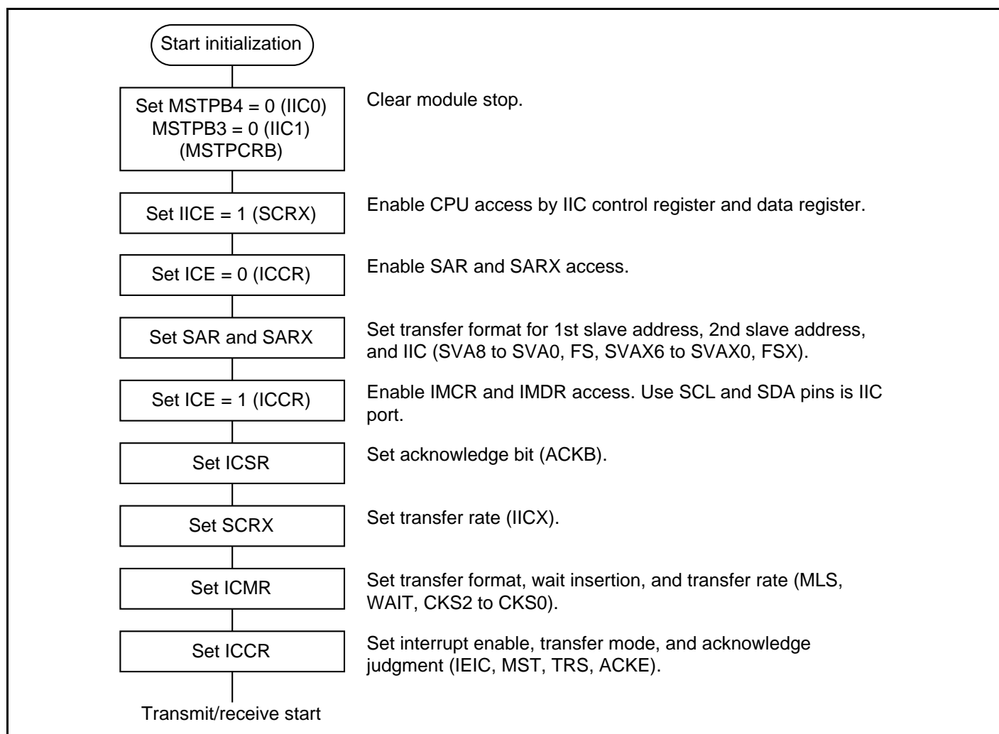
Figure 16.6 Flowchart for IIC Initialization (Example)
