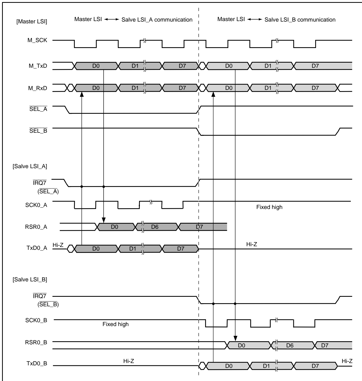
Figure 15.37 Summary of SCI Select Function Operation
