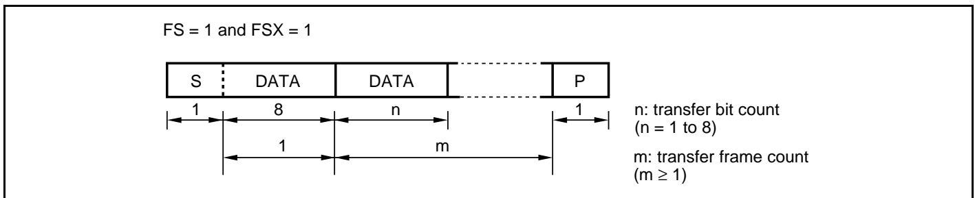
Figure 16.4 I 2 C Bus Data Format (Serial Format)
