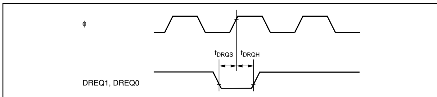
Figure 27.23 DMAC DREQ Input Timing
