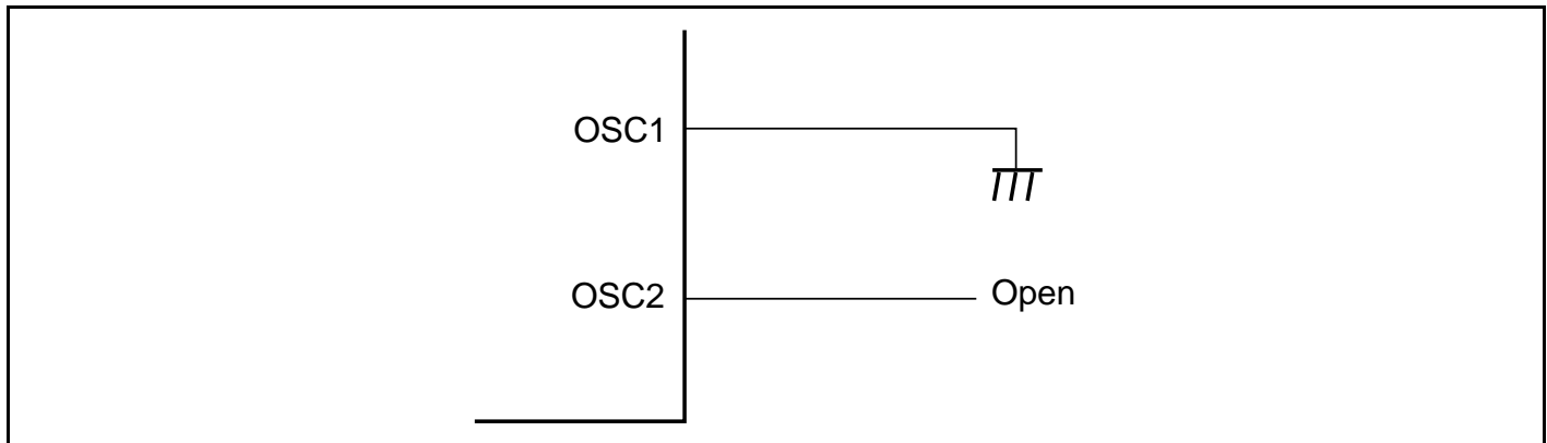
Figure 23.10 Pin Handling when Subclock Not Required
