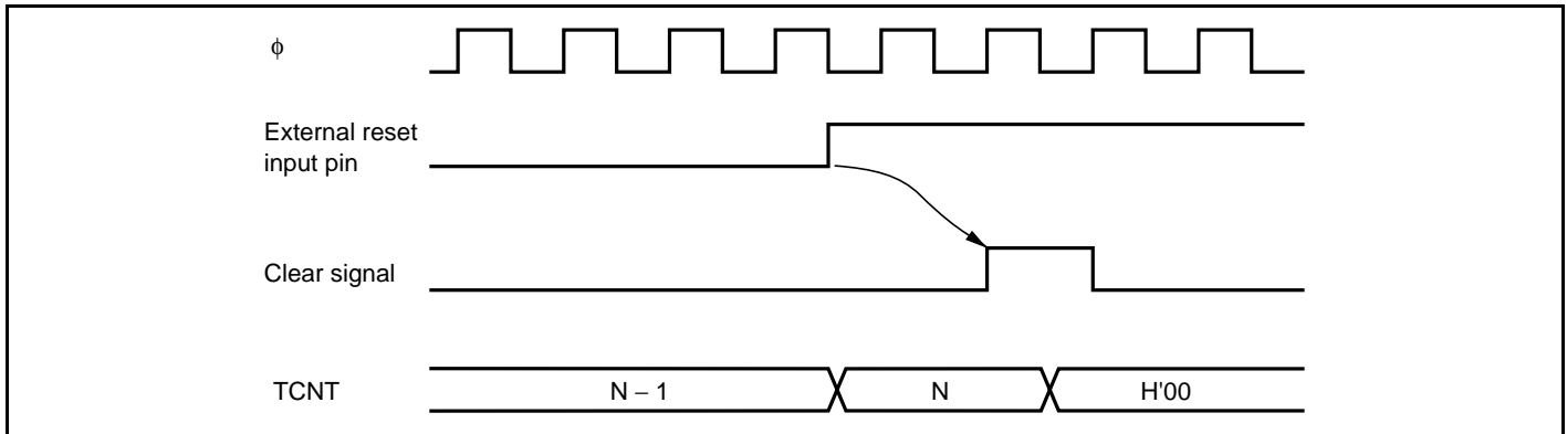
Figure 12.8 Timing of Clearing by External Reset Input
