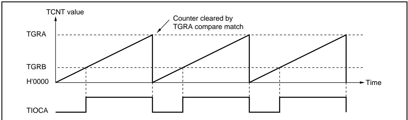
Figure 11.22 Example of PWM Mode Operation (1)
