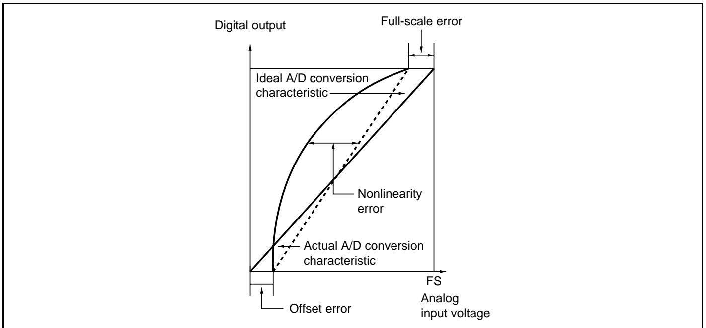
Figure 17.8 A/D Conversion Accuracy Definitions
