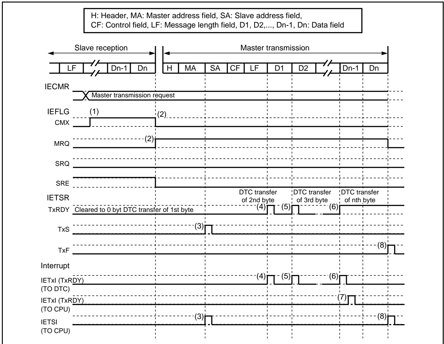
Figure 14.8 Master Transmit Operation Timing
