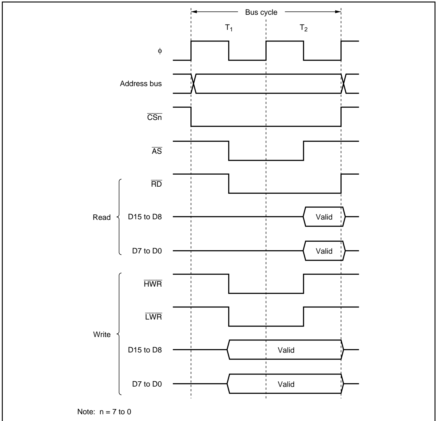
Figure 7.14 Bus Timing for 16-Bit 2-State Access Space (3) (Word Access)
