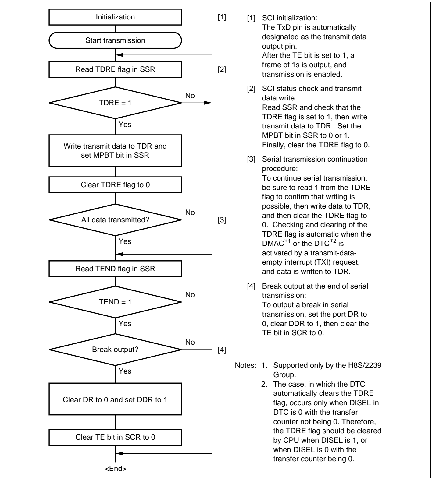
Figure 15.14 Sample Multiprocessor Serial Transmission Flowchart
