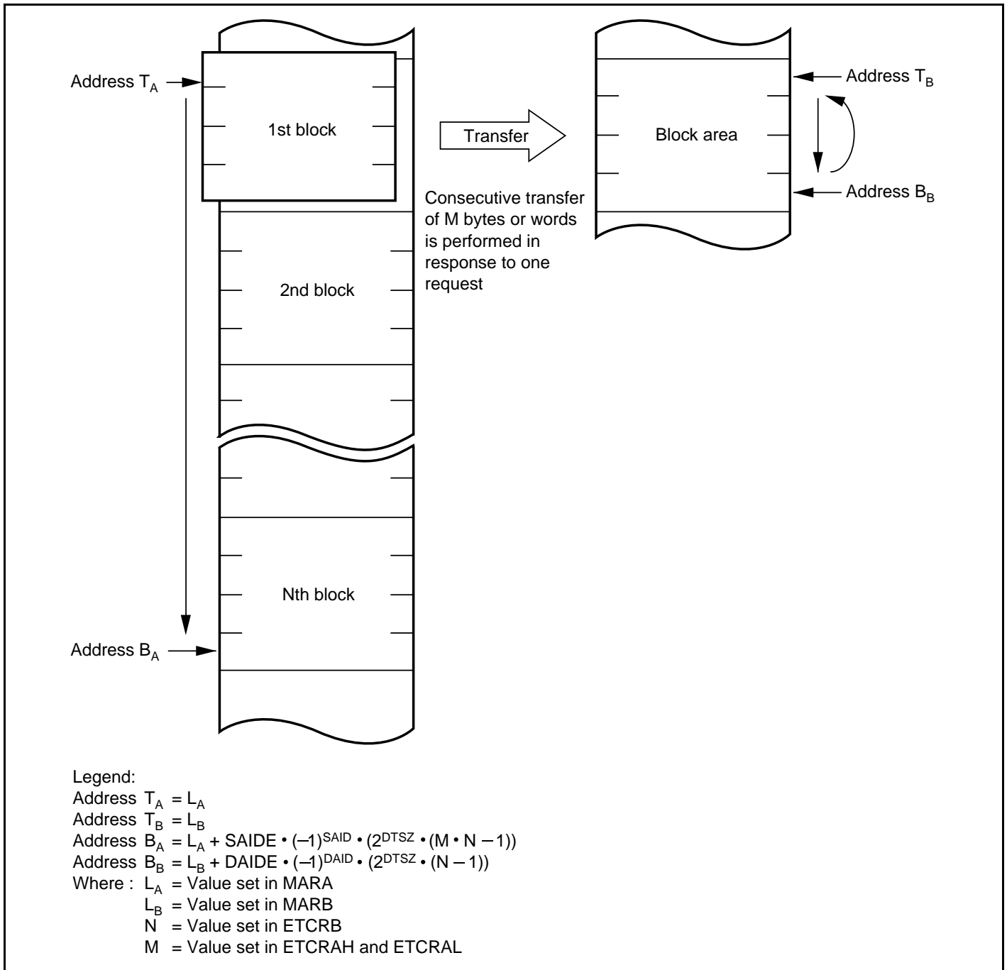
Figure 8.14 Operation in Block Transfer Mode (BLKDIR = 0)
