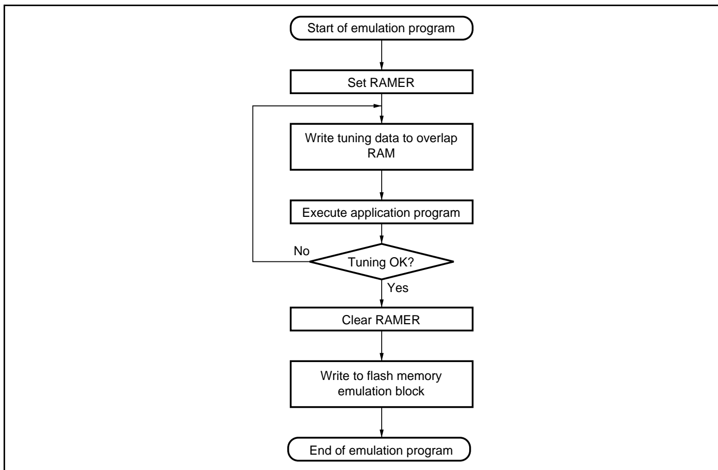
Figure 20.9 Flowchart for Flash Memory Emulation in RAM
