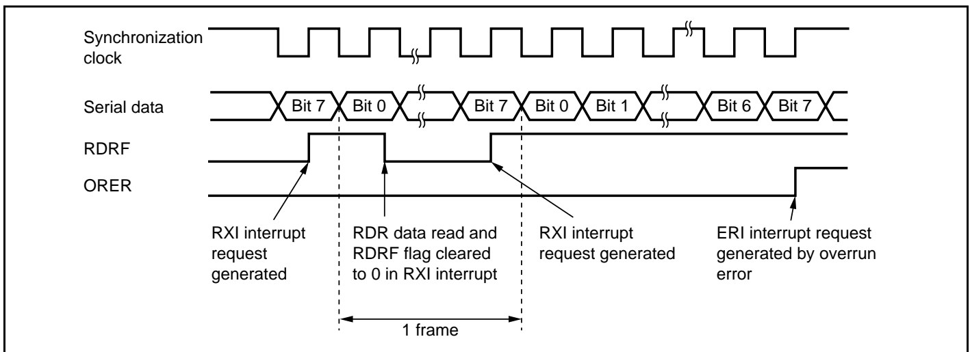
Figure 15.21 Example of SCI Operation in Reception
