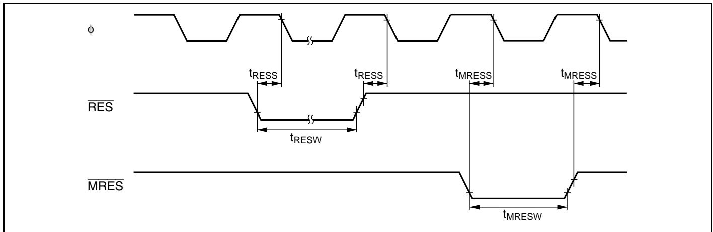
Figure 27.12 Reset Input Timing
