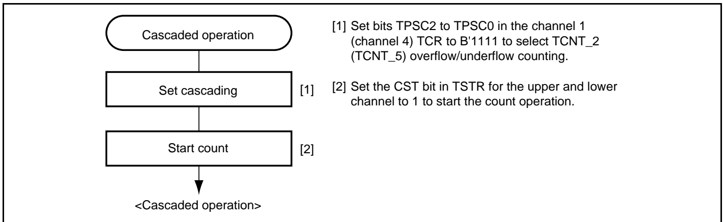
Figure 11.18 Cascaded Operation Setting Procedure
