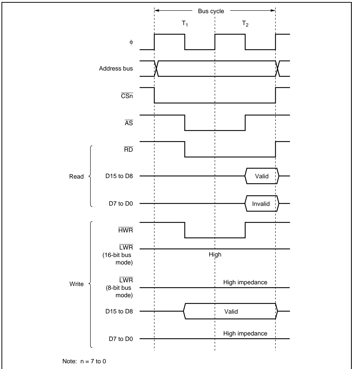
Figure 7.10 Bus Timing for 8-Bit 2-State Access Space
