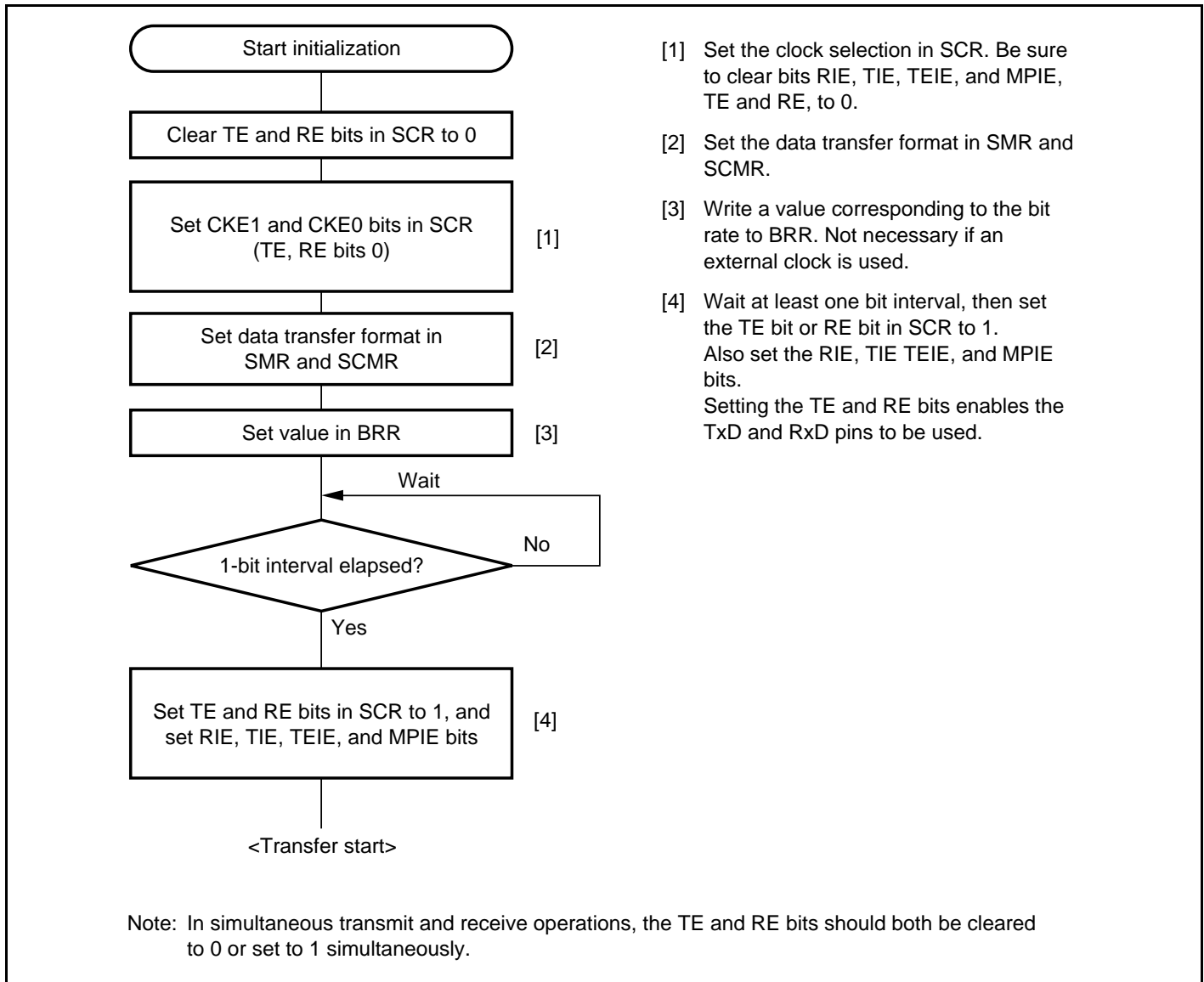
Figure 15.18 Sample SCI Initialization Flowchart
