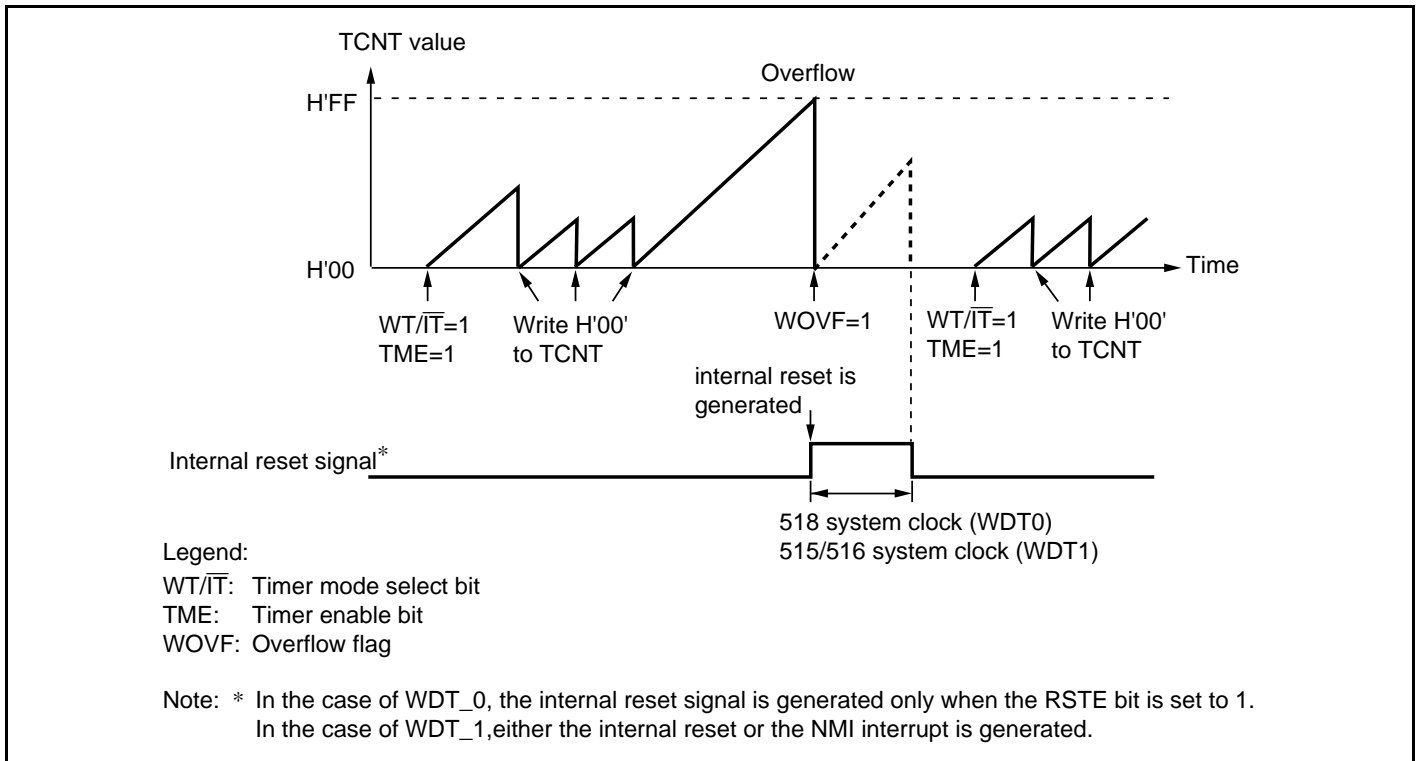
Figure 13.2 Watchdog Timer Mode Operation
