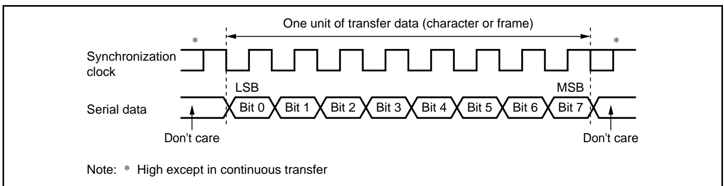
Figure 15.17 Data Format in Synchronous Communication (For LSB-First)
