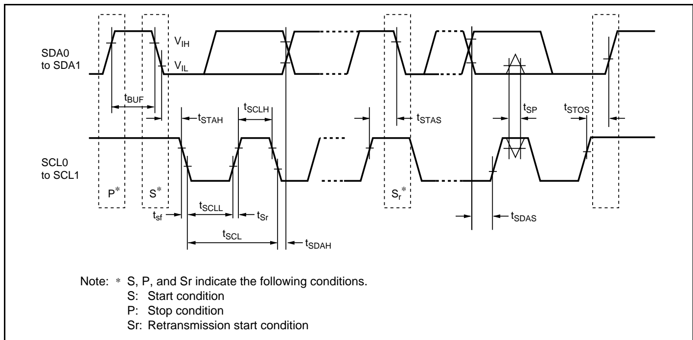
Figure 27.7 I 2 C Bus Interface Input/Output Timing (Optional)
