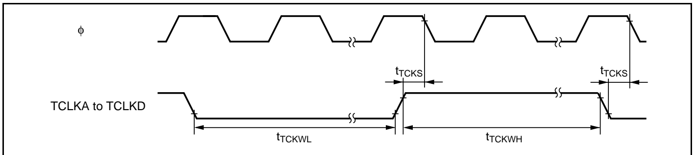
Figure 27.26 TPU Clock Input Timing
