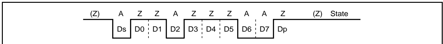
Figure 15.26 Direct Convention (SDIR = SINV = O/\bar{E} = 0 )
