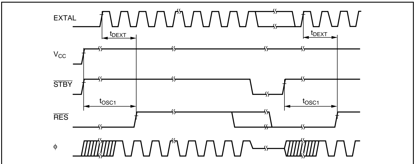
Figure 27.11 Oscillation Stabilization Timing
