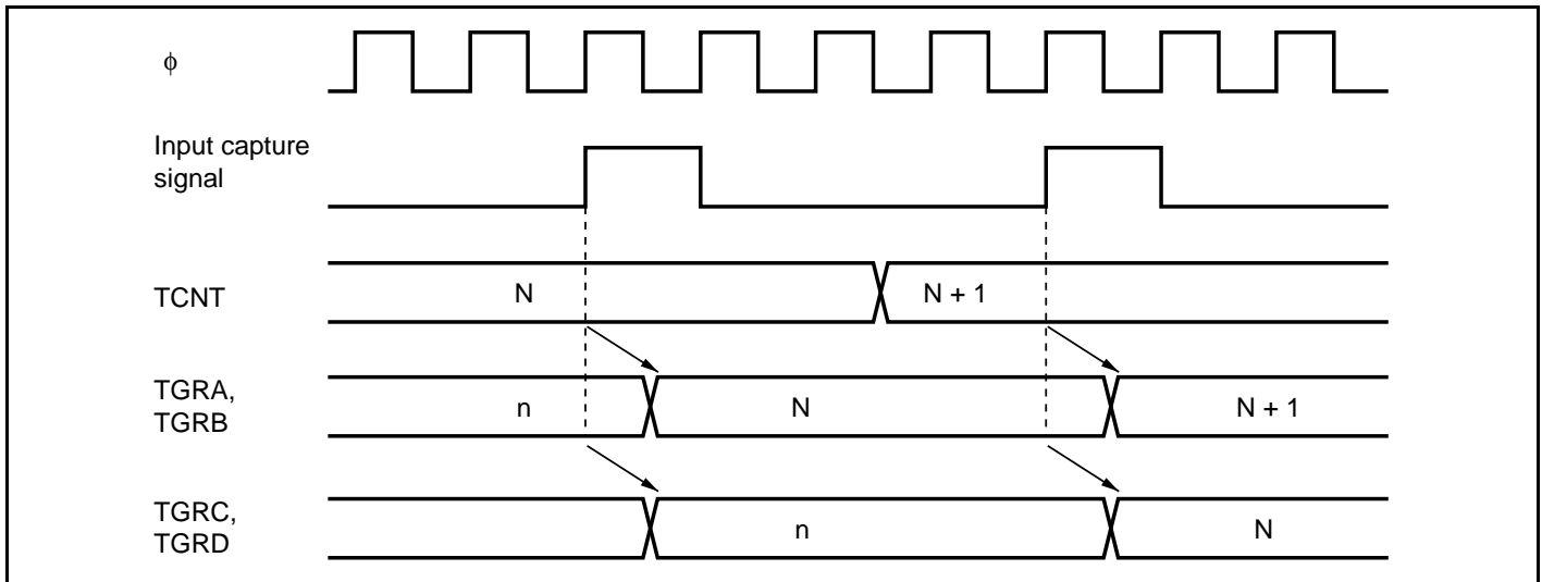
Figure 11.38 Buffer Operation Timing (Input Capture)
