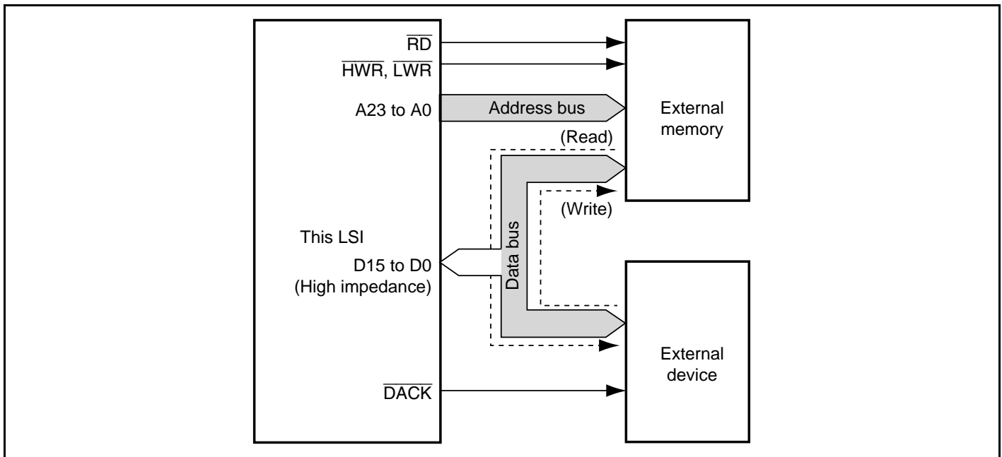
Figure 8.9 Data Bus in Single Address Mode
