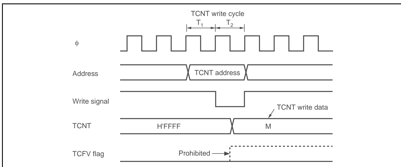
Figure 11.54 Contention between TCNT Write and Overflow
