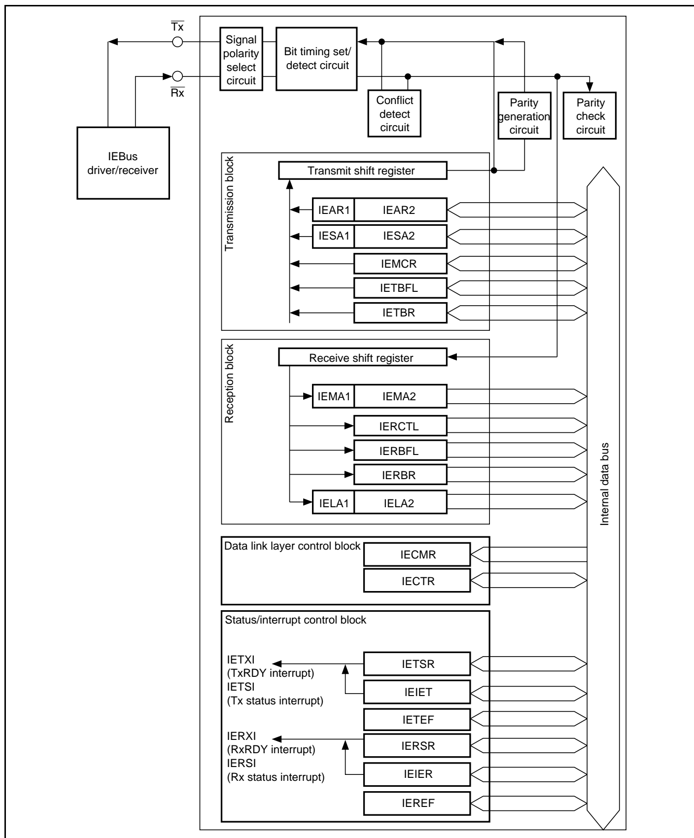
Figure 14.1 Block Diagram of IEB
