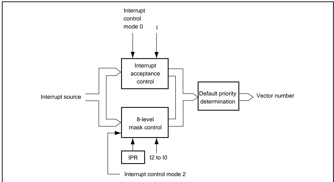
Figure 5.4 Block Diagram of Interrupt Control Operation
