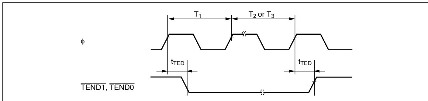
Figure 27.22 DMAC TEND Output Timing
