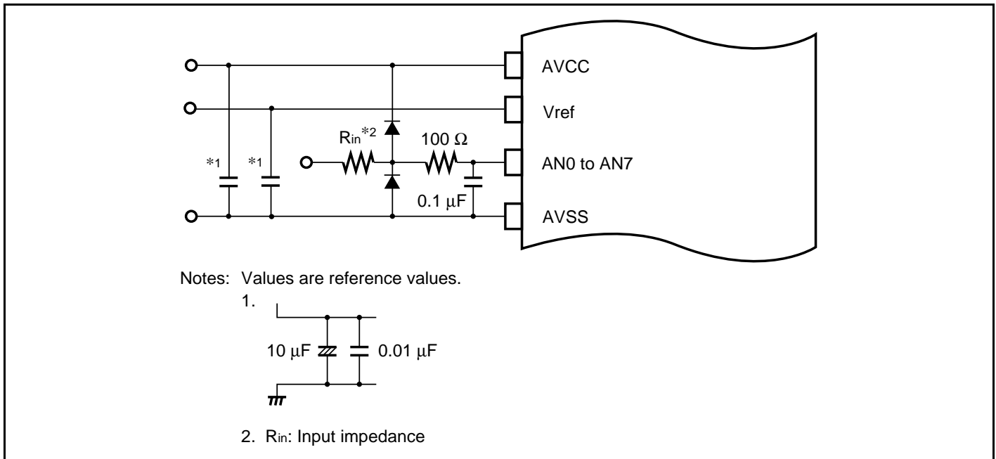
Figure 17.10 Example of Analog Input Protection Circuit
