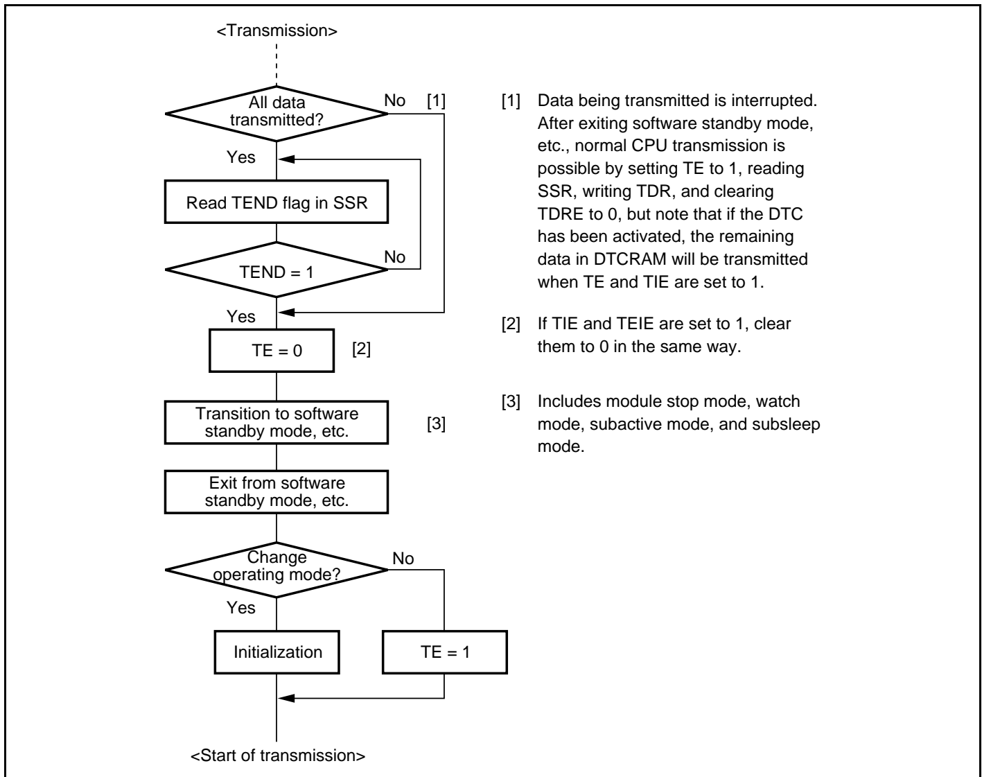
Figure 15.39 Sample Flowchart for Mode Transition during Transmission
