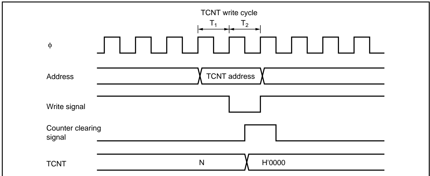
Figure 11.46 Contention between TCNT Write and Clear Operations
