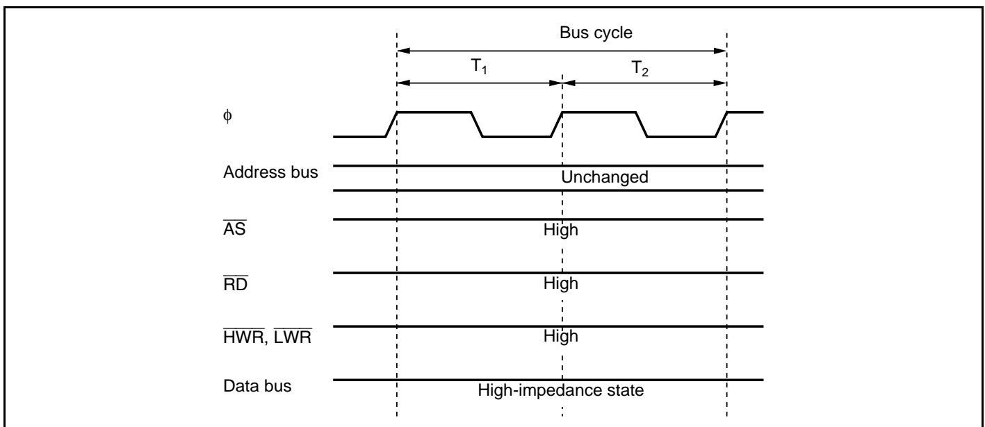
Figure 7.7 Pin States during On-Chip Peripheral Module Access
