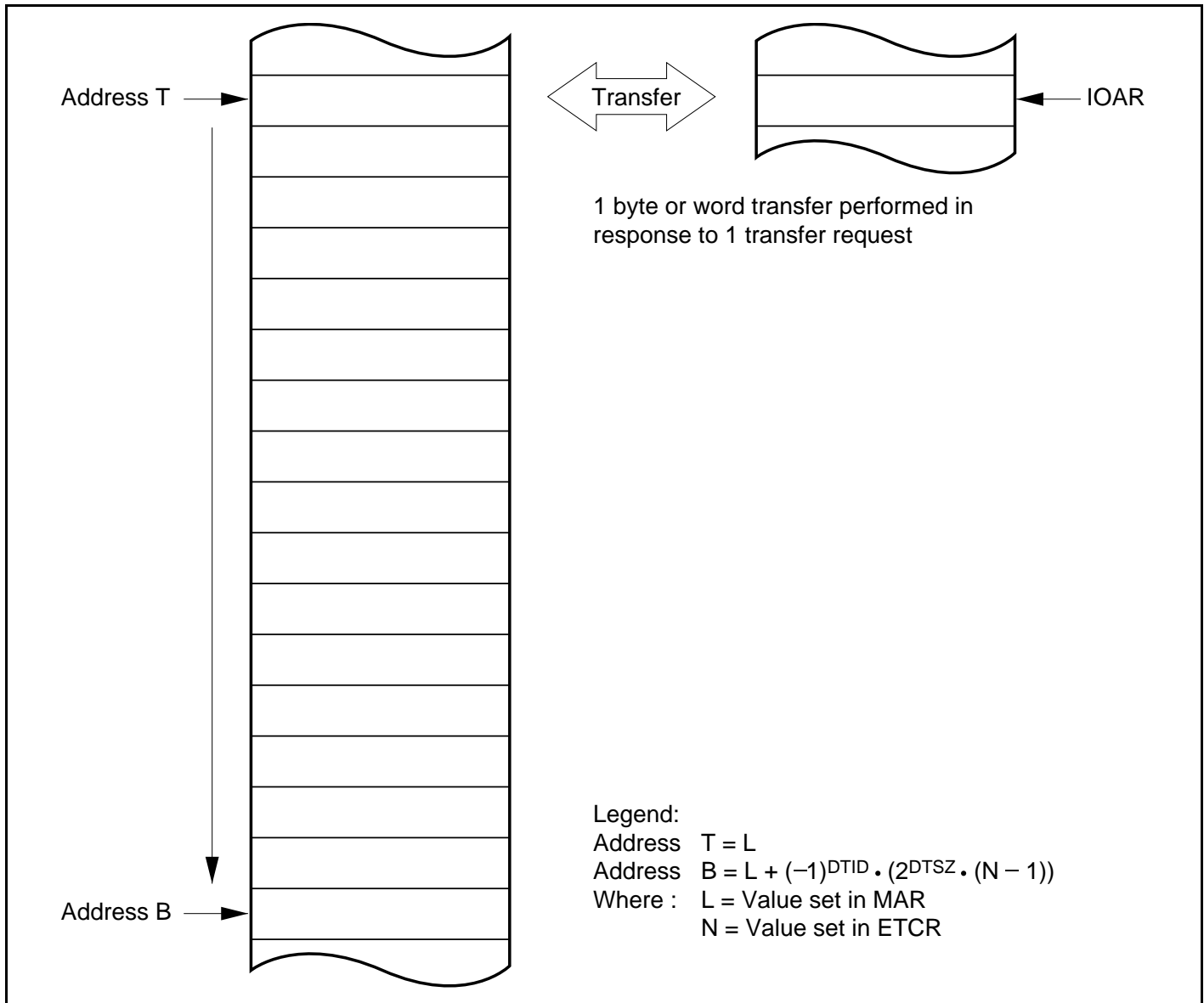
Figure 8.3 Operation in Sequential Mode
