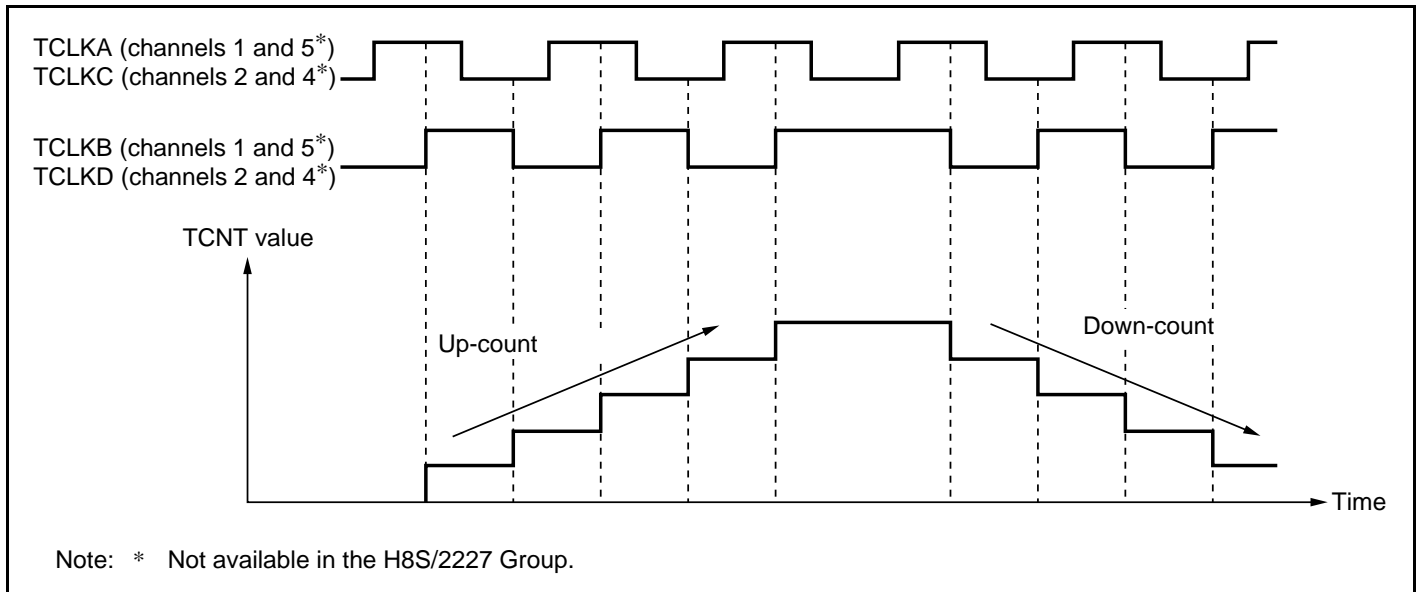
Figure 11.29 Example of Phase Counting Mode 4 Operation
