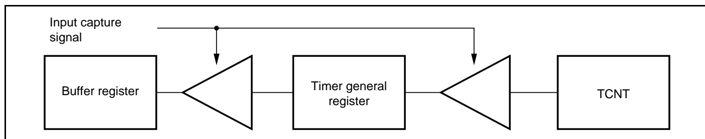
Figure 11.14 Input Capture Buffer Operation
