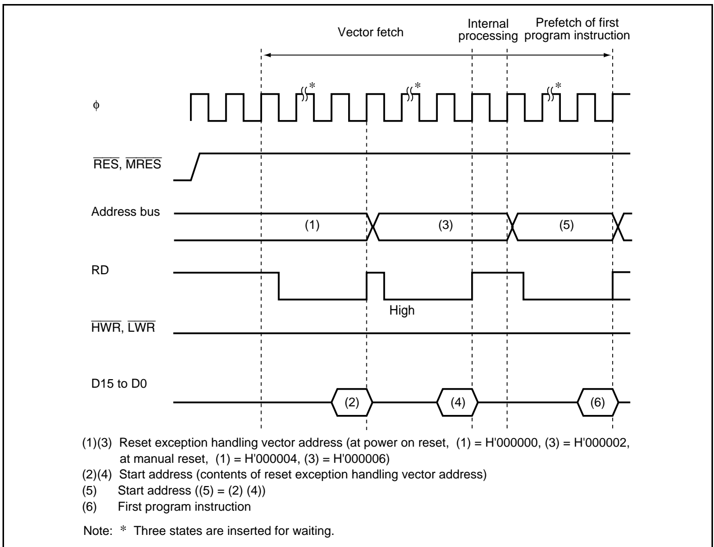
Figure 4.1 Reset Sequence (Mode 4)
