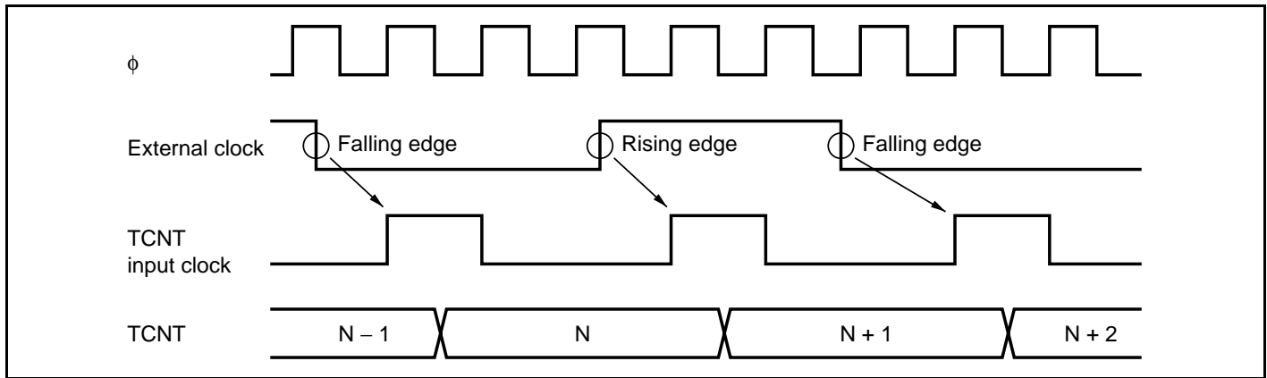
Figure 11.32 Count Timing in External Clock Operation
