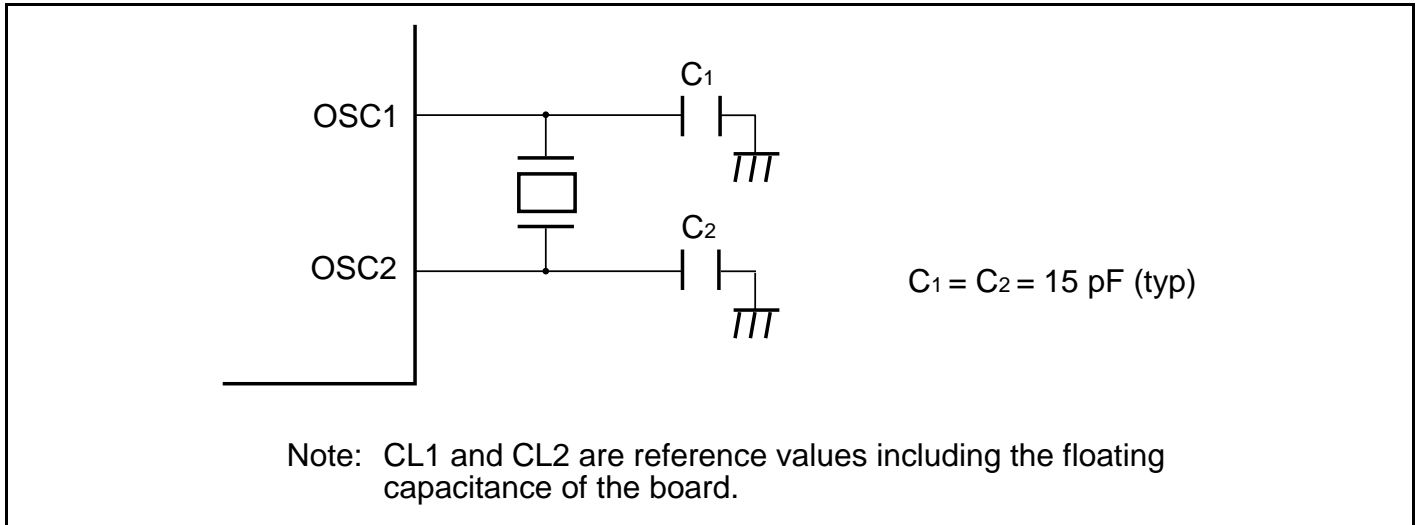
Figure 23.8 Connection Example of 32.768-kHz Quartz Oscillator
