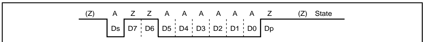
Figure 15.27 Inverse Convention (SDIR = SINV = O/\bar{E} = 1 )
