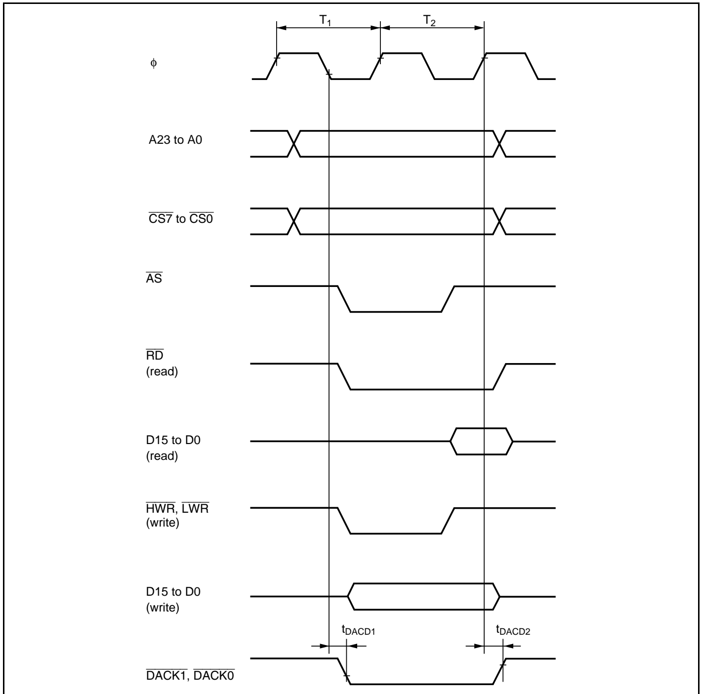
Figure 27.20 DMAC Single Address Transfer Timing (Two-State Access)
