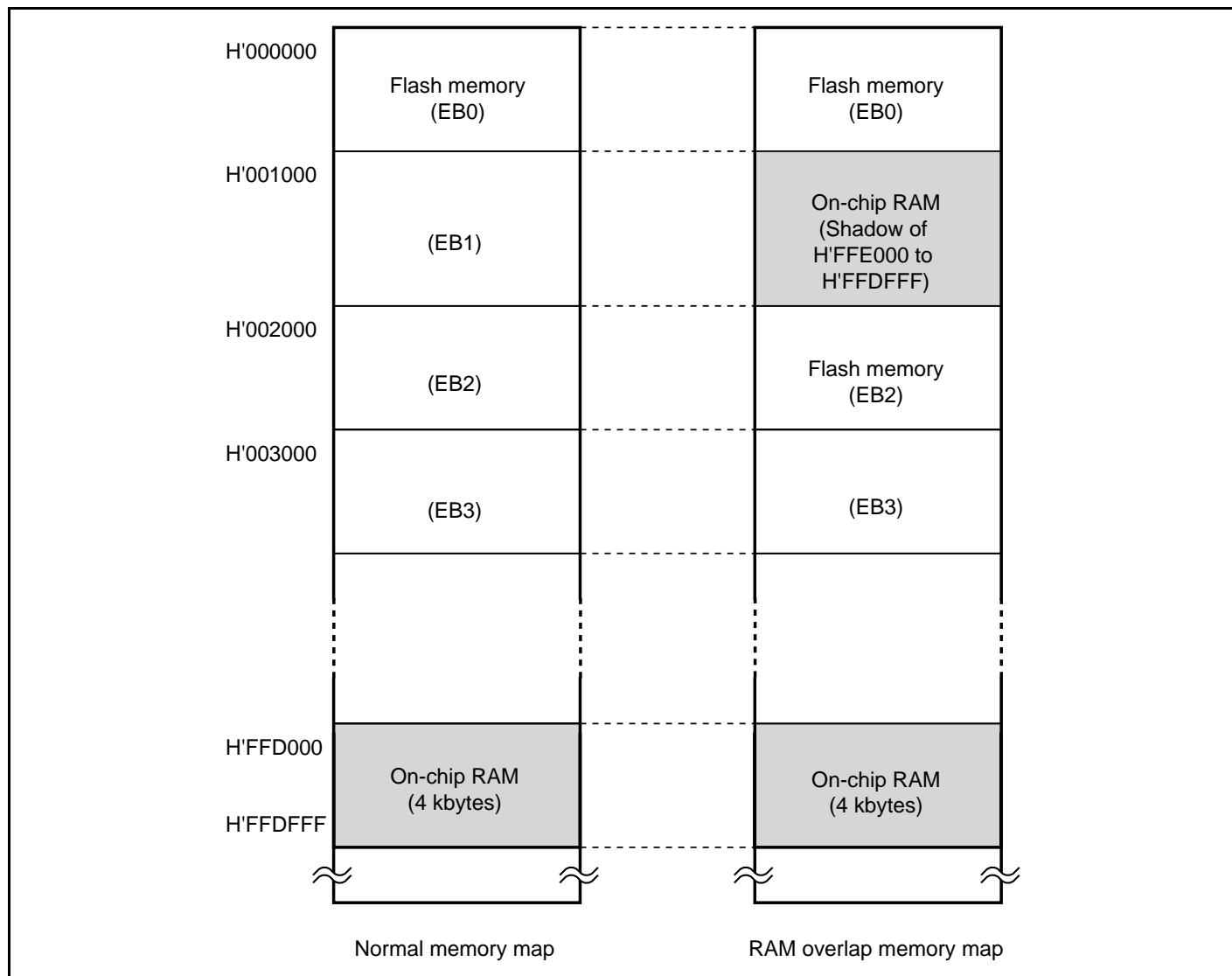
Figure 20.10 Example of RAM Overlap Operation
