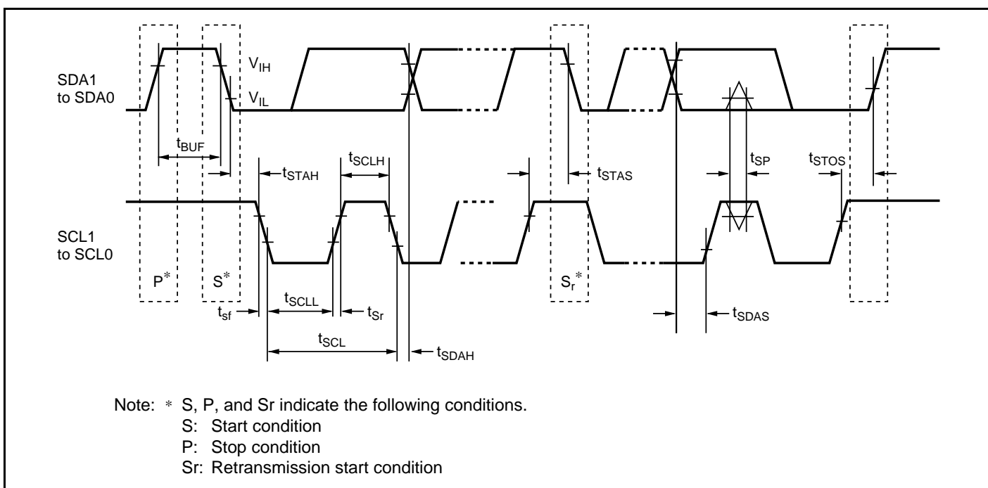
Figure 27.34 I 2 C Bus Interface Input/Output Timing (Optional)
