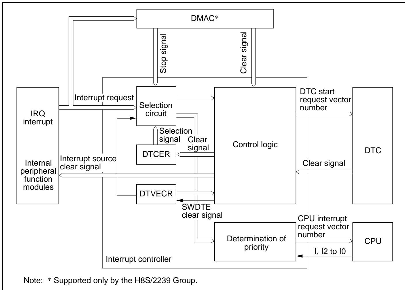
Figure 5.8 DTC and DMAC* Interrupt Control
