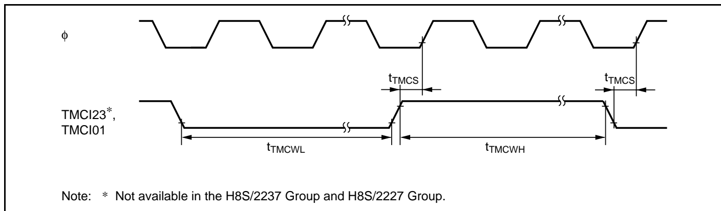
Figure 27.28 8-Bit Timer Clock Input Timing
