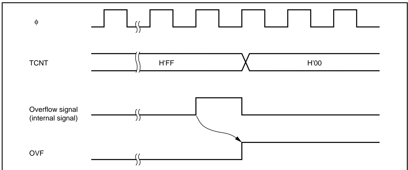
Figure 13.4 Timing of OVF Setting
