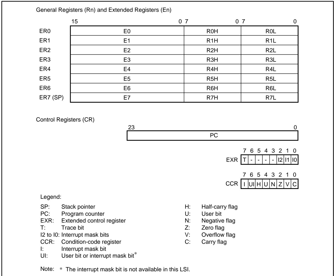
Figure 2.6 CPU Registers
