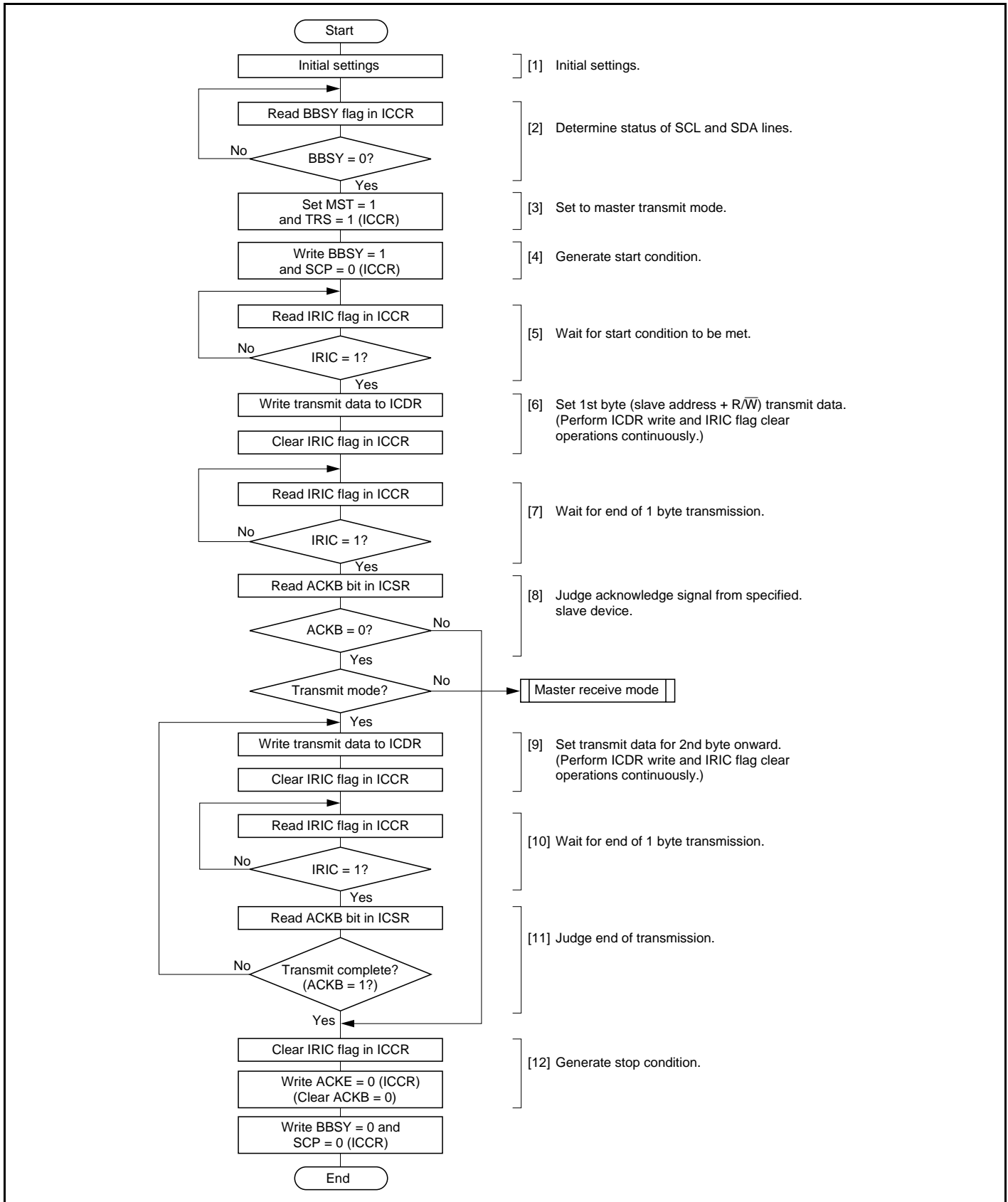
Figure 16.7 Flowchart for Master Transmit Mode (Example)
