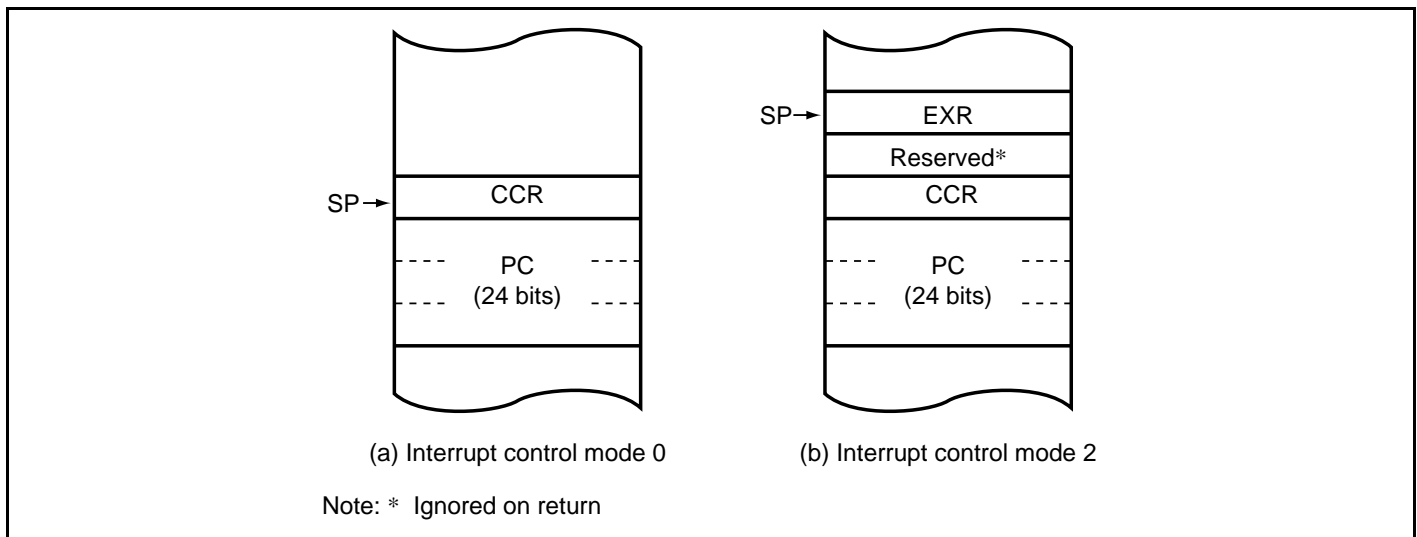
Figure 4.2 Stack Status after Exception Handling (Advanced Mode)
