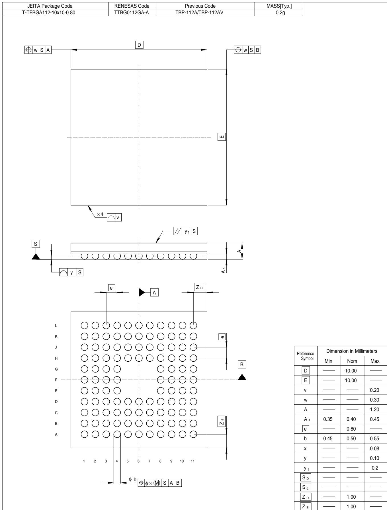
Figure C.6 TBP-112A, TBP-112AV Package Dimensions
