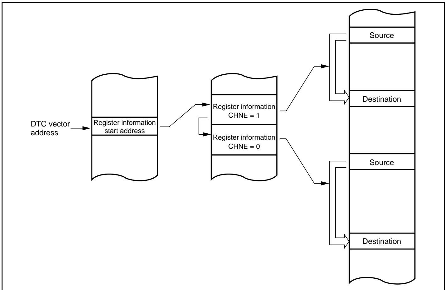
Figure 9.9 Chain Transfer Operation
