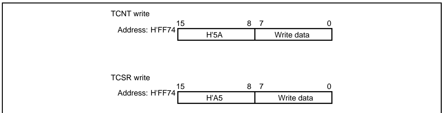
Figure 13.6 Writing to TCNT, TCSR
