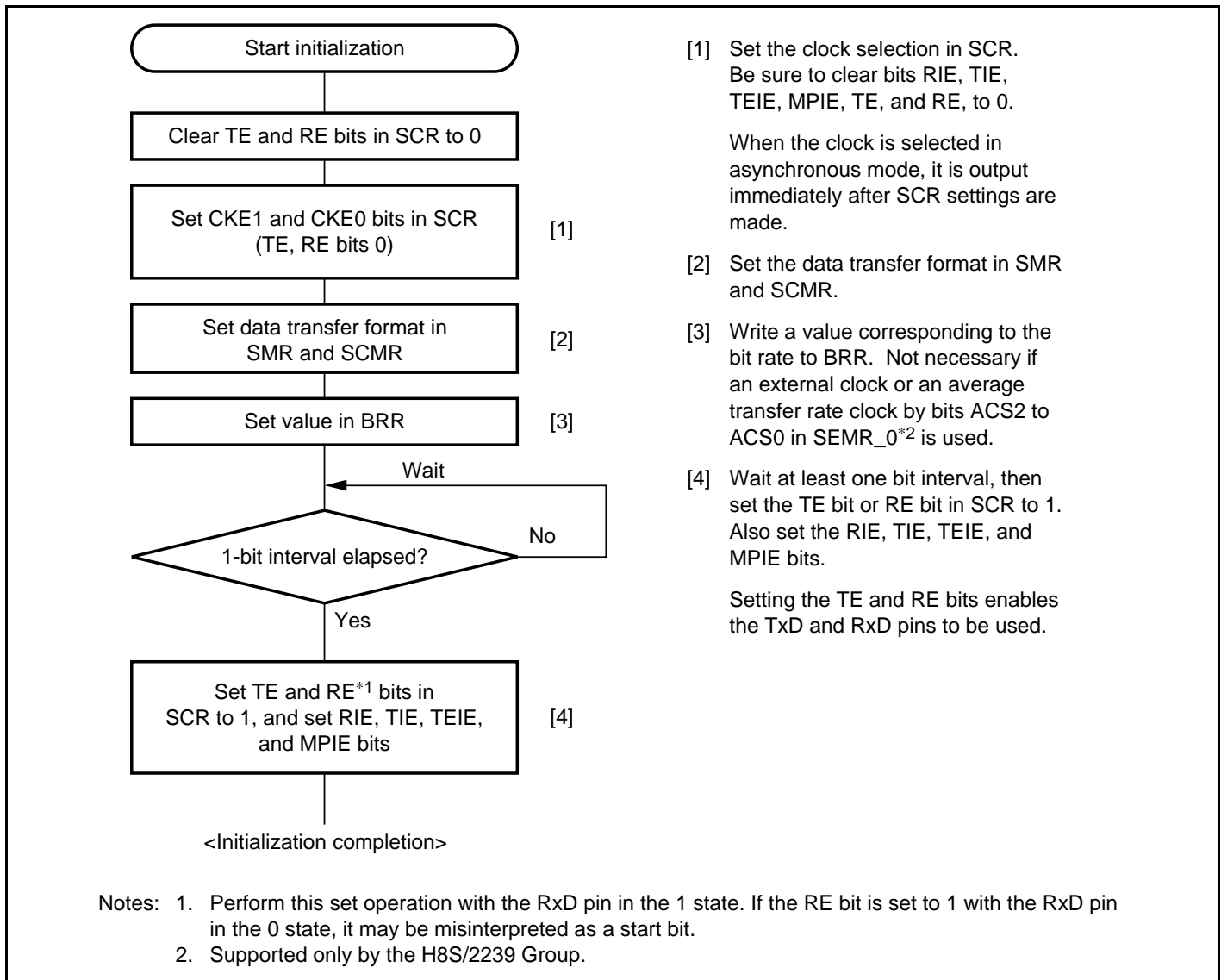
Figure 15.8 Sample SCI Initialization Flowchart
