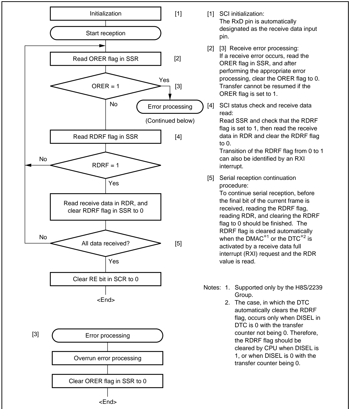
Figure 15.22 Sample Serial Reception Flowchart
