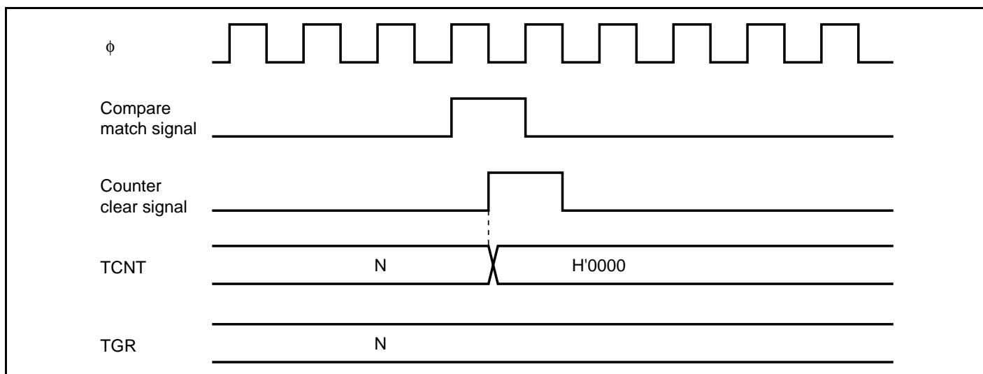
Figure 11.35 Counter Clear Timing (Compare Match)
