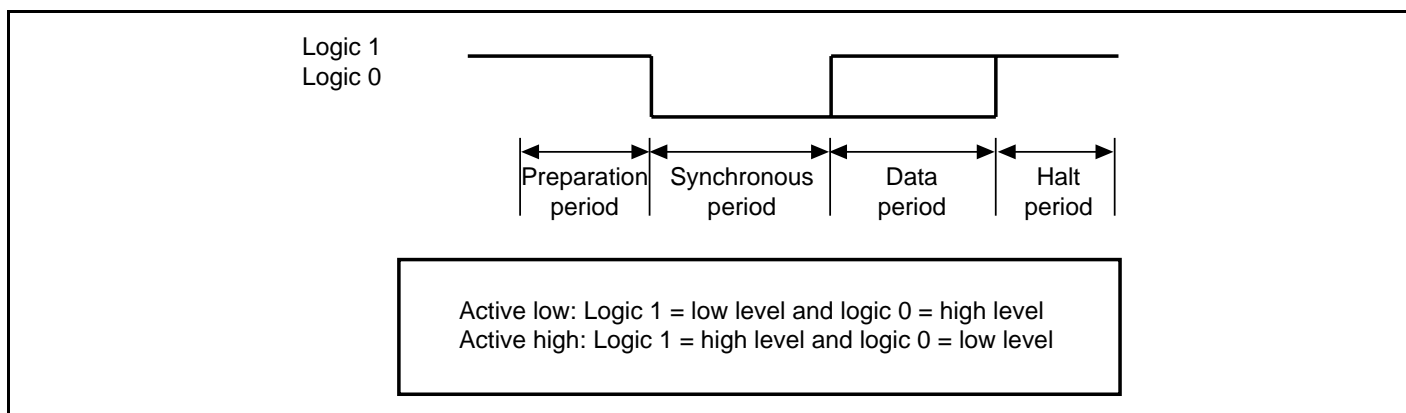
Figure 14.5 IEBus Bit Format (Conceptual Diagram)
