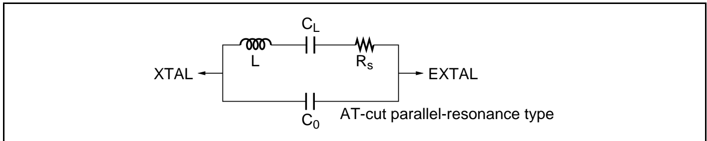
Figure 23.3 Crystal Resonator Equivalent Circuit
