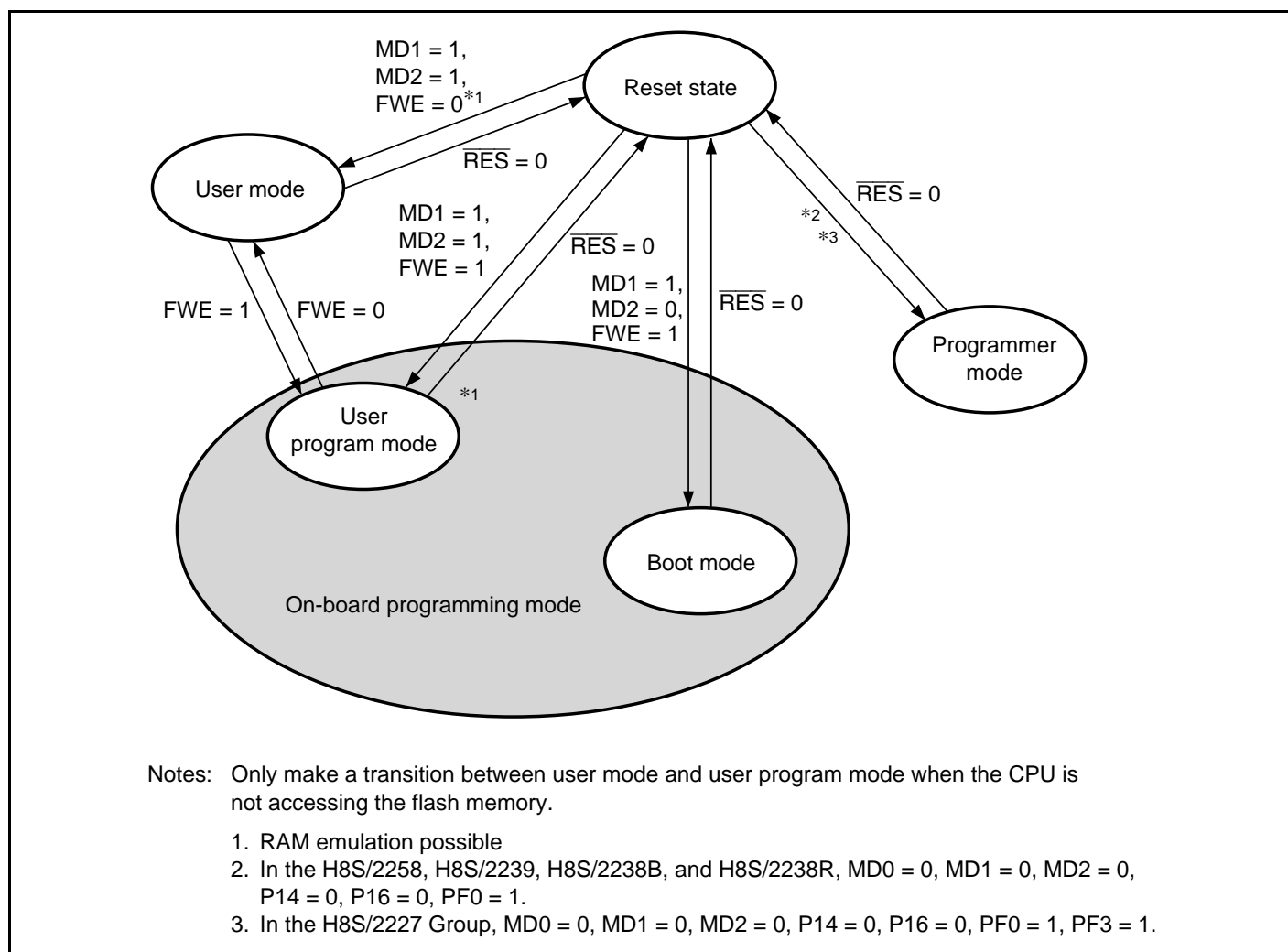
Figure 20.2 Flash Memory State Transitions
