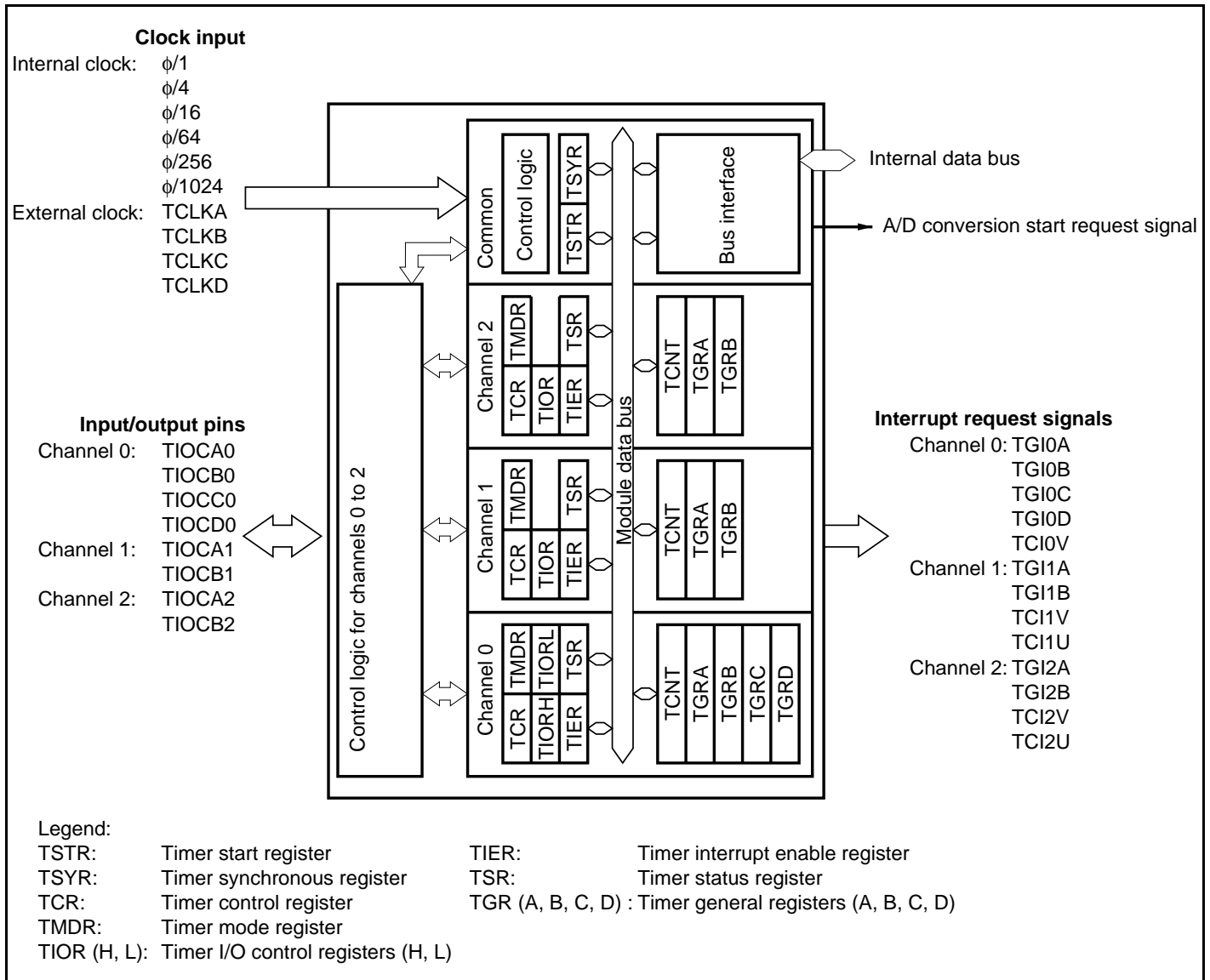
Figure 11.2 Block Diagram of TPU (H8S/2227 Group)
