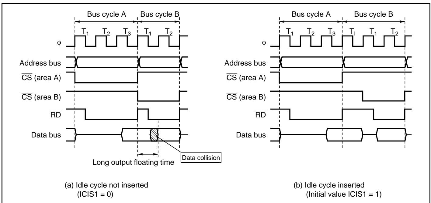
Figure 7.21 Example of Idle Cycle Operation (1)
