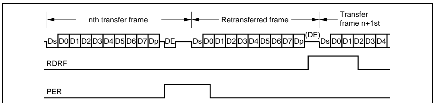
Figure 15.32 Retransfer Operation in SCI Receive Mode
