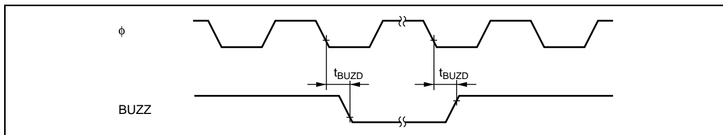
Figure 27.30 WDT_1 Output Timing
