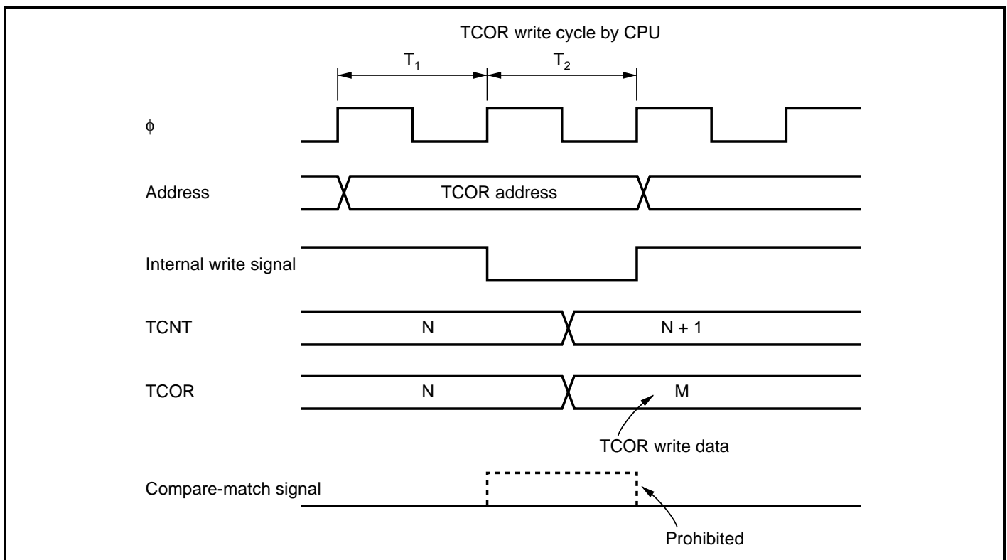
Figure 12.12 Contention between TCOR Write and Compare-Match
