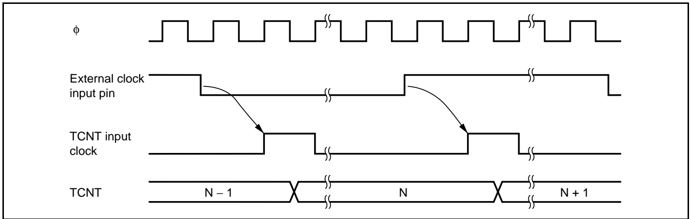
Figure 12.4 Count Timing for External Clock Input
