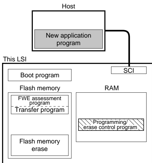
Figure 20.4 User Program Mode (Example)
