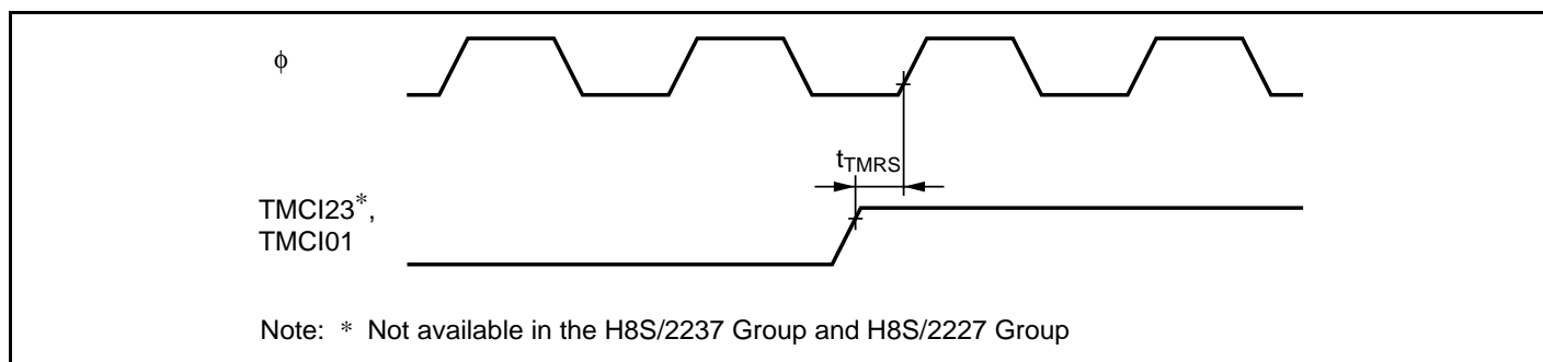
Figure 27.29 8-Bit Timer Reset Input Timing
