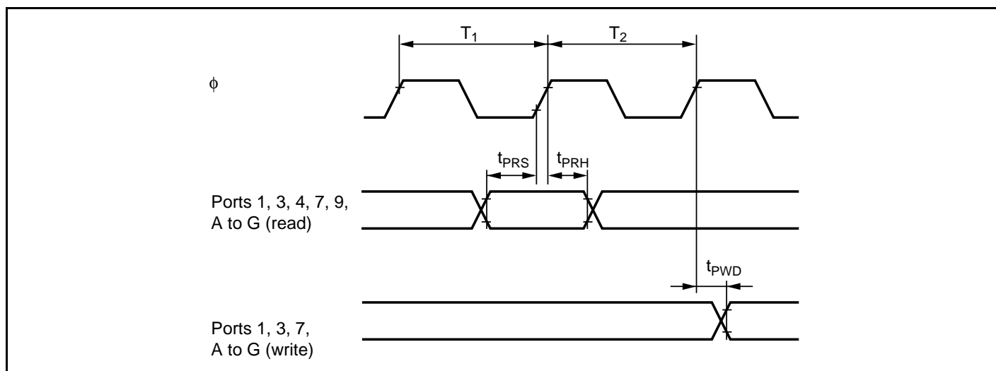
Figure 27.24 I/O Port Input/Output Timing
