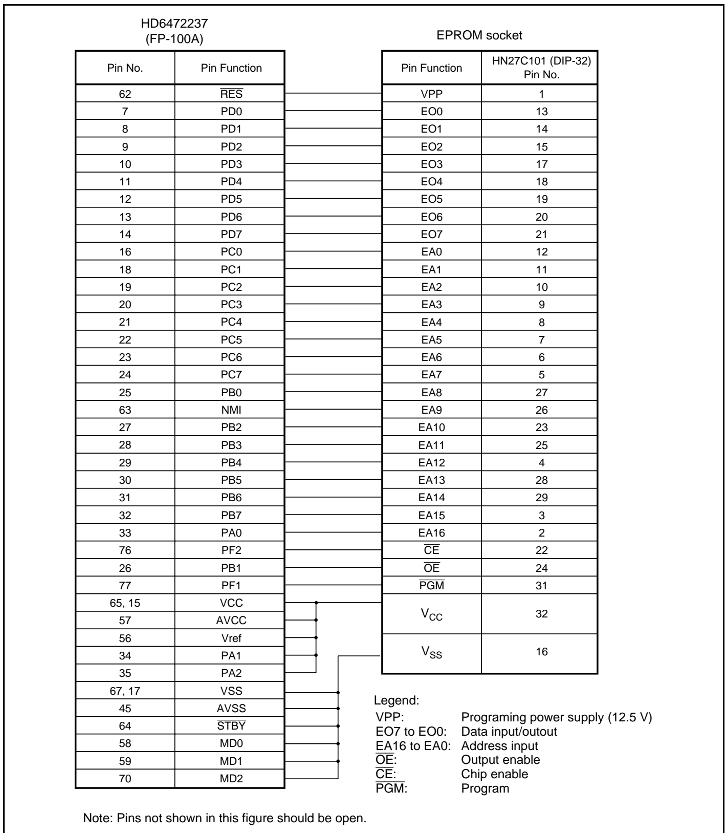
Figure 22.2 HD6472237 Socket Adapter Pin Correspondence Diagram (FP-100A)
