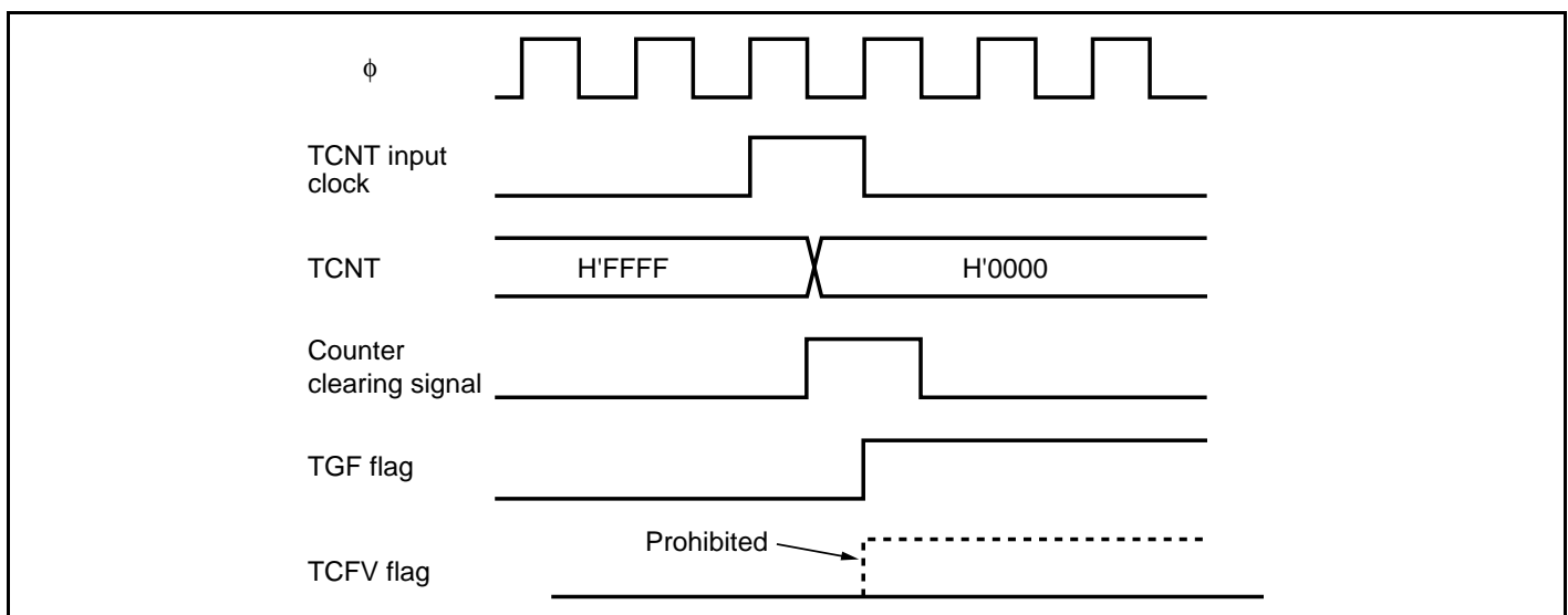
Figure 11.53 Contention between Overflow and Counter Clearing
