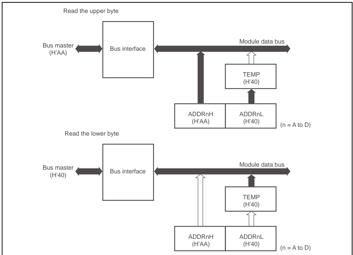
Figure 17.2 Access to ADDR (When Reading H'AA40)
