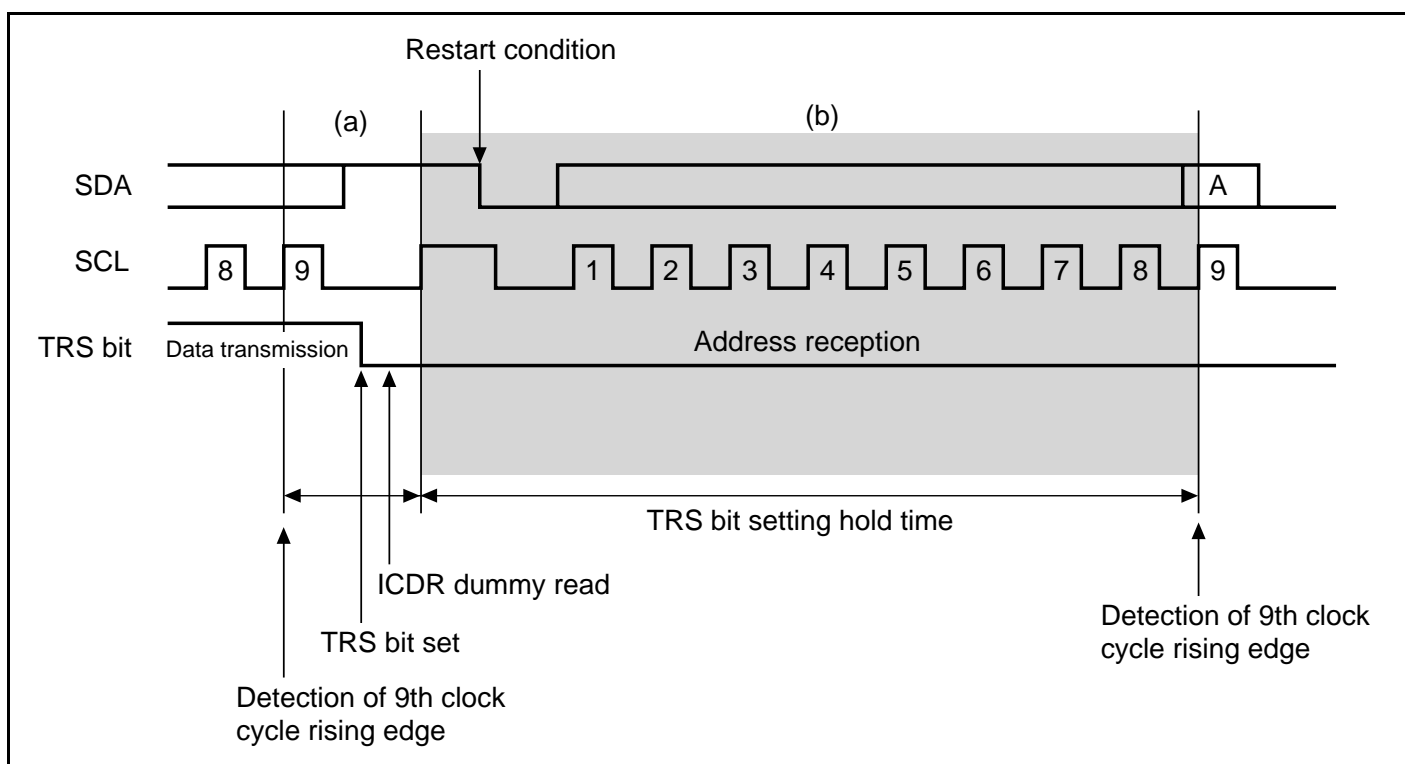
Figure 16.26 TRS Bit Setting Timing in Slave Mode
