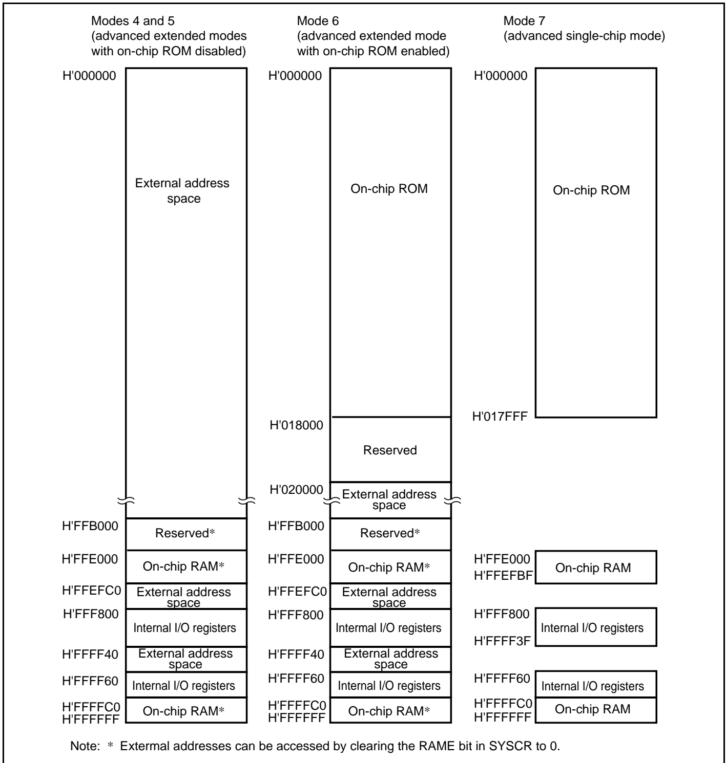
Figure 3.8 H8S/2224 Memory Map in Each Operating Mode
