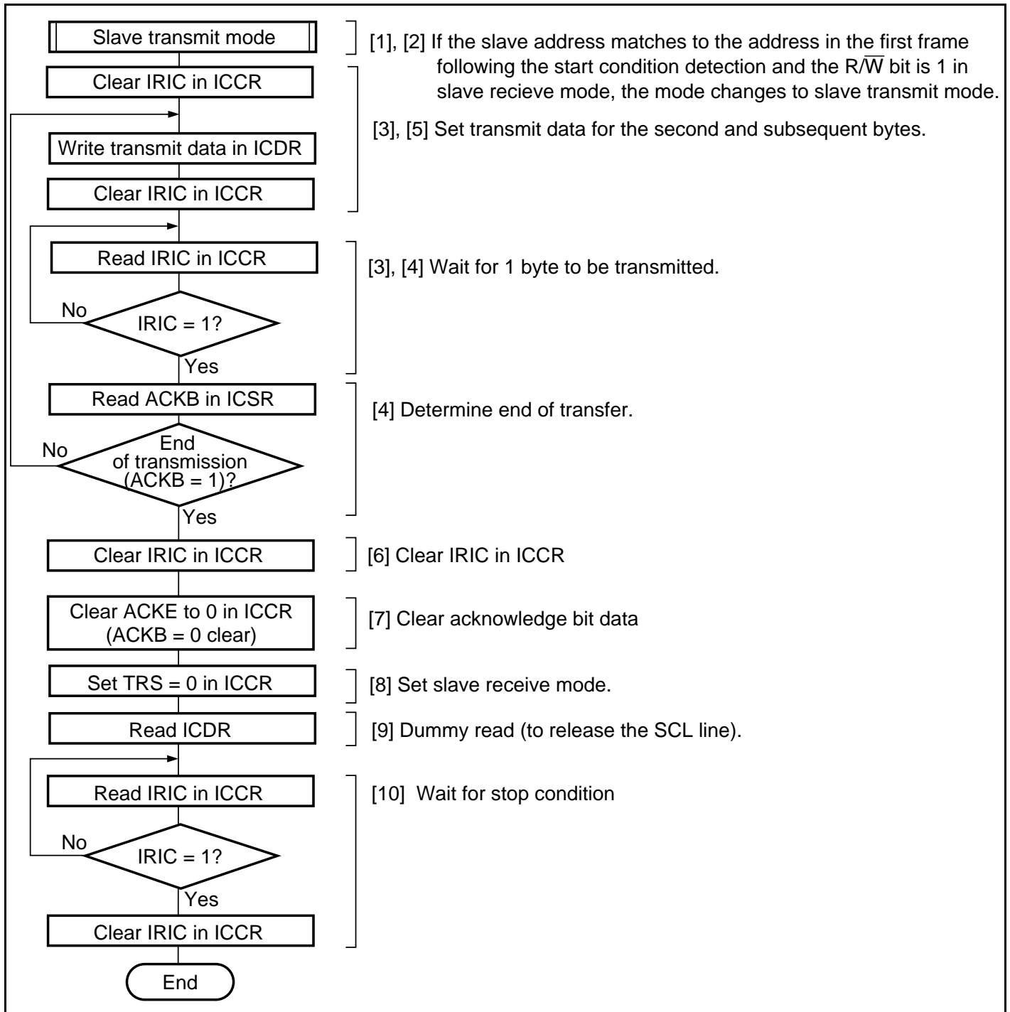
Figure 16.17 Sample Flowchart for Slave Transmit Mode
