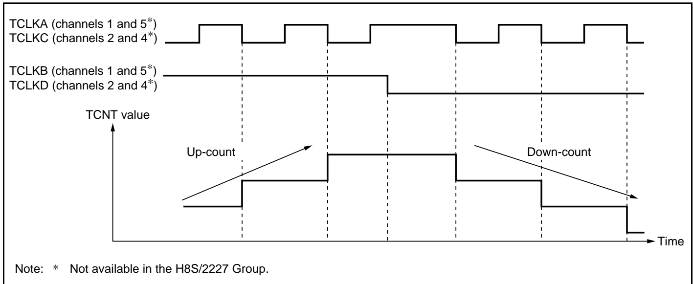
Figure 11.27 Example of Phase Counting Mode 2 Operation
