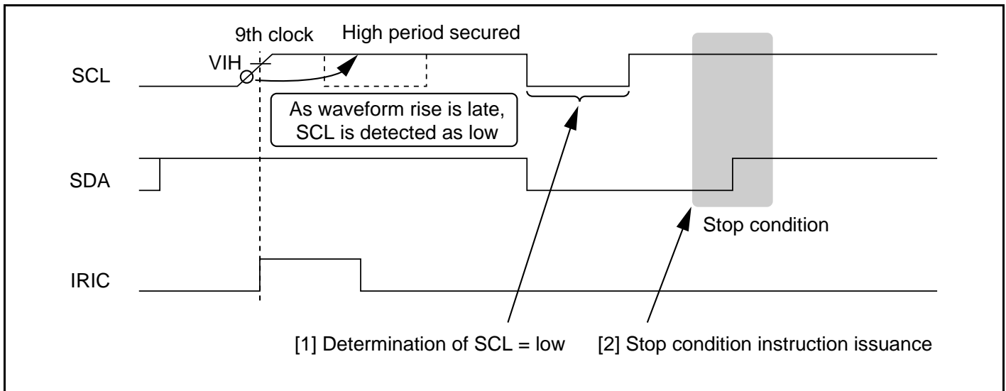
Figure 16.23 Timing of Stop Condition Issuance
