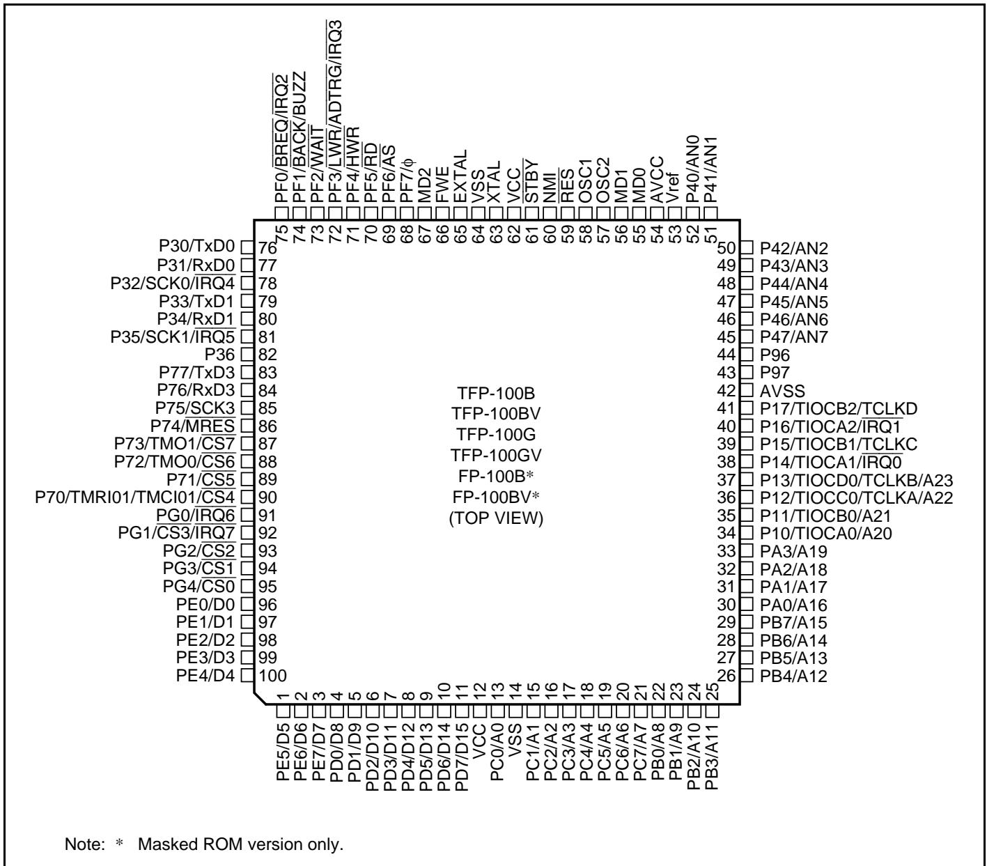
Figure 1.15 Pin Arrangement of H8S/2227 Group (TFP-100B, TFP-100BV, TFP-100G, TFP-100GV, FP-100B*, FP-100BV*: Top View)
