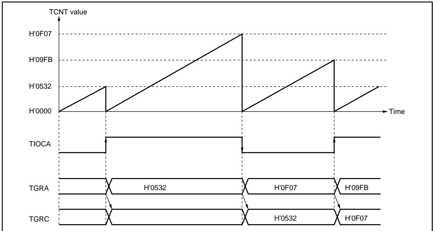
Figure 11.17 Example of Buffer Operation (2)
