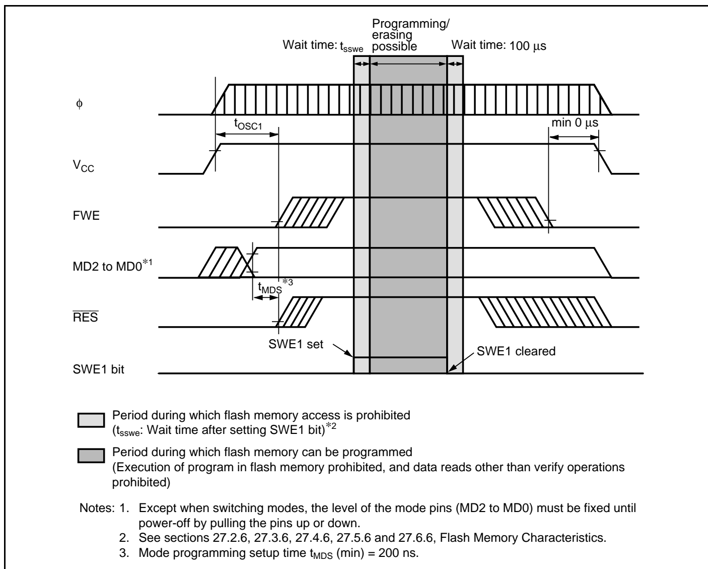
Figure 20.15 Power-On/Off Timing (User Program Mode)
