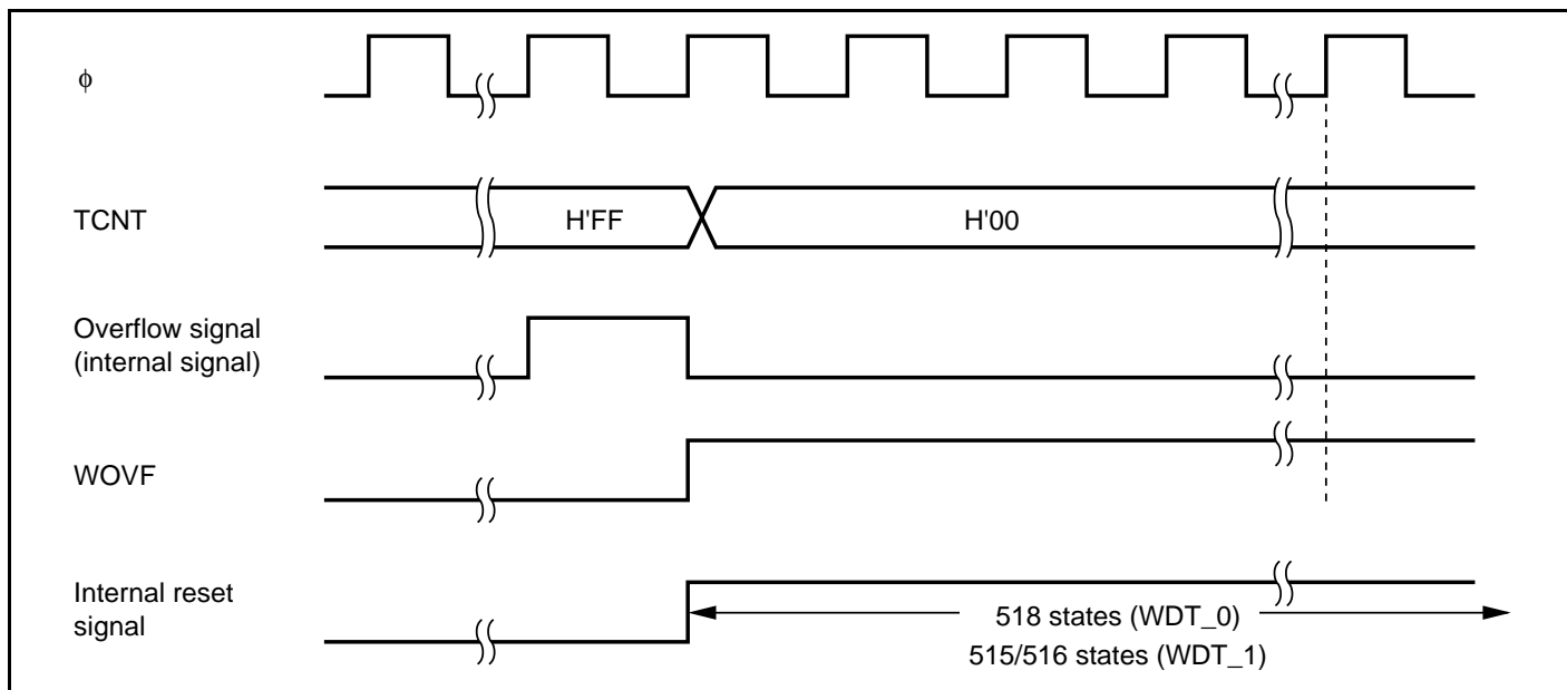
Figure 13.5 Timing of WOVF Setting
