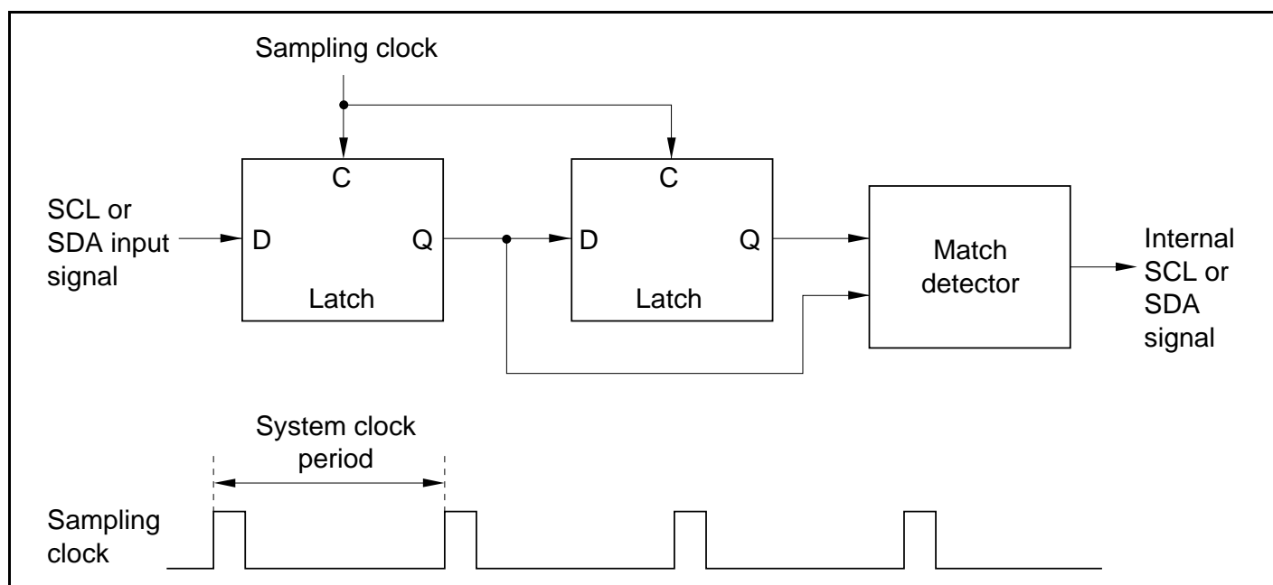
Figure 16.20 Block Diagram of Noise Canceler
