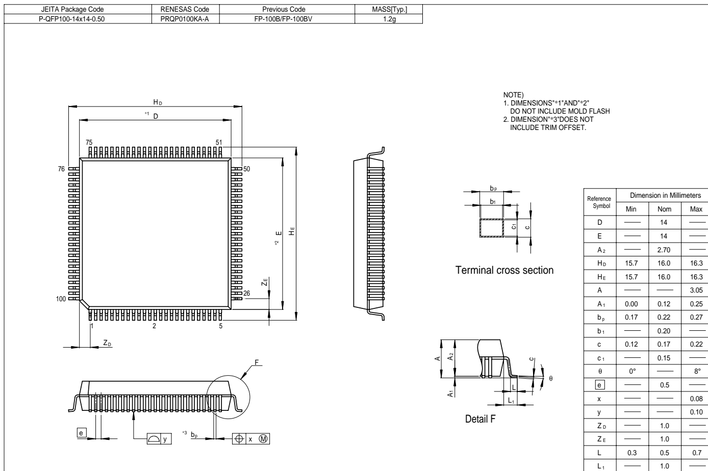
Figure C.4 FP-100B Package Dimensions
