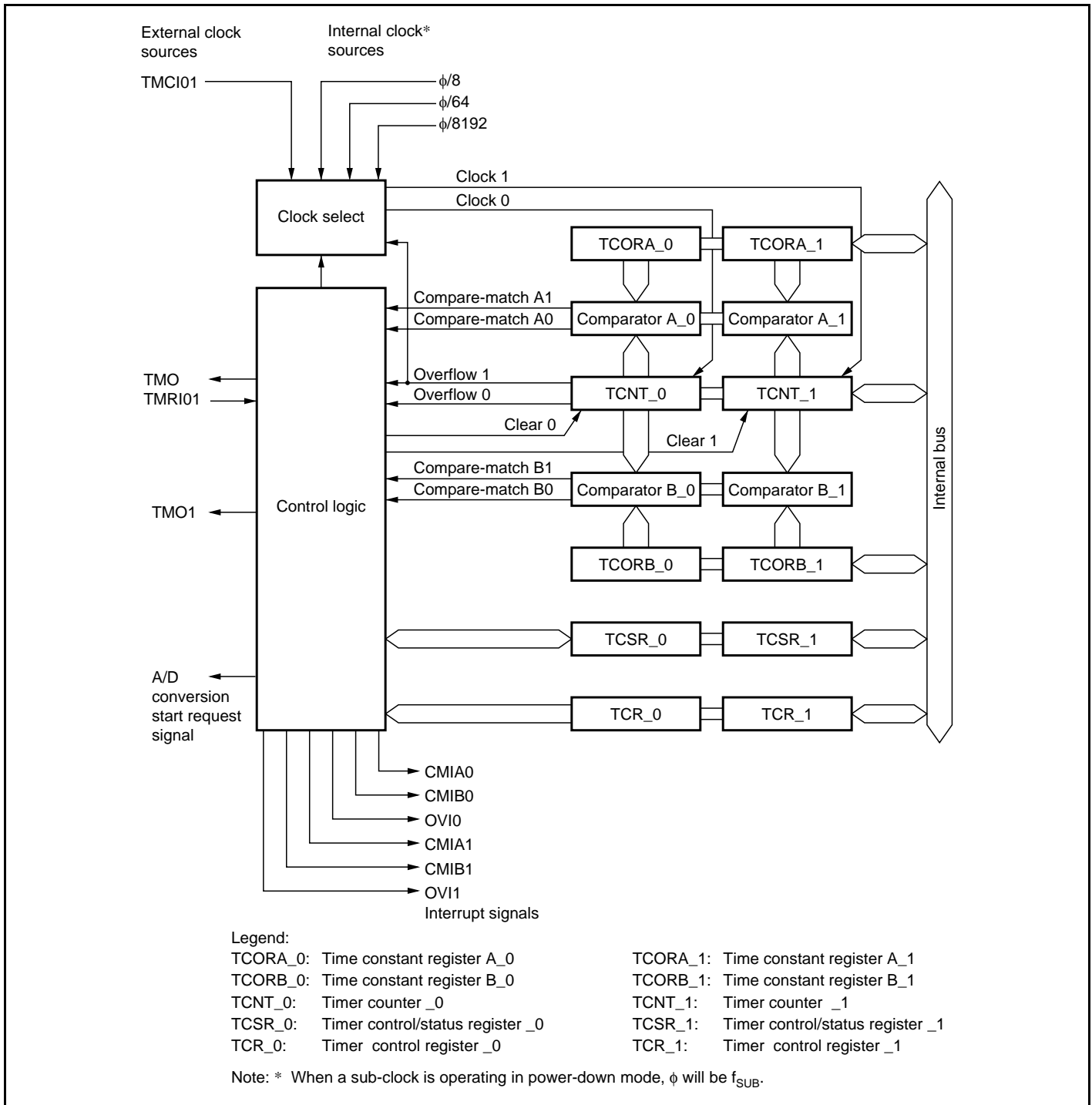
Figure 12.1 Block Diagram of 8-Bit Timer Module
