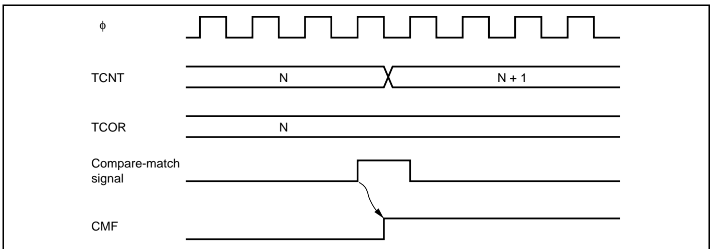
Figure 12.5 Timing of CMF Setting
