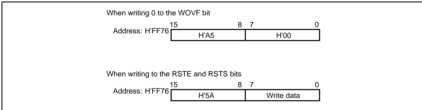
Figure 13.7 Writing to RSTCSR
