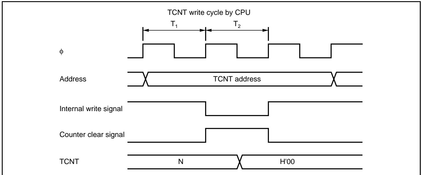
Figure 12.10 Contention between TCNT Write and Clear
