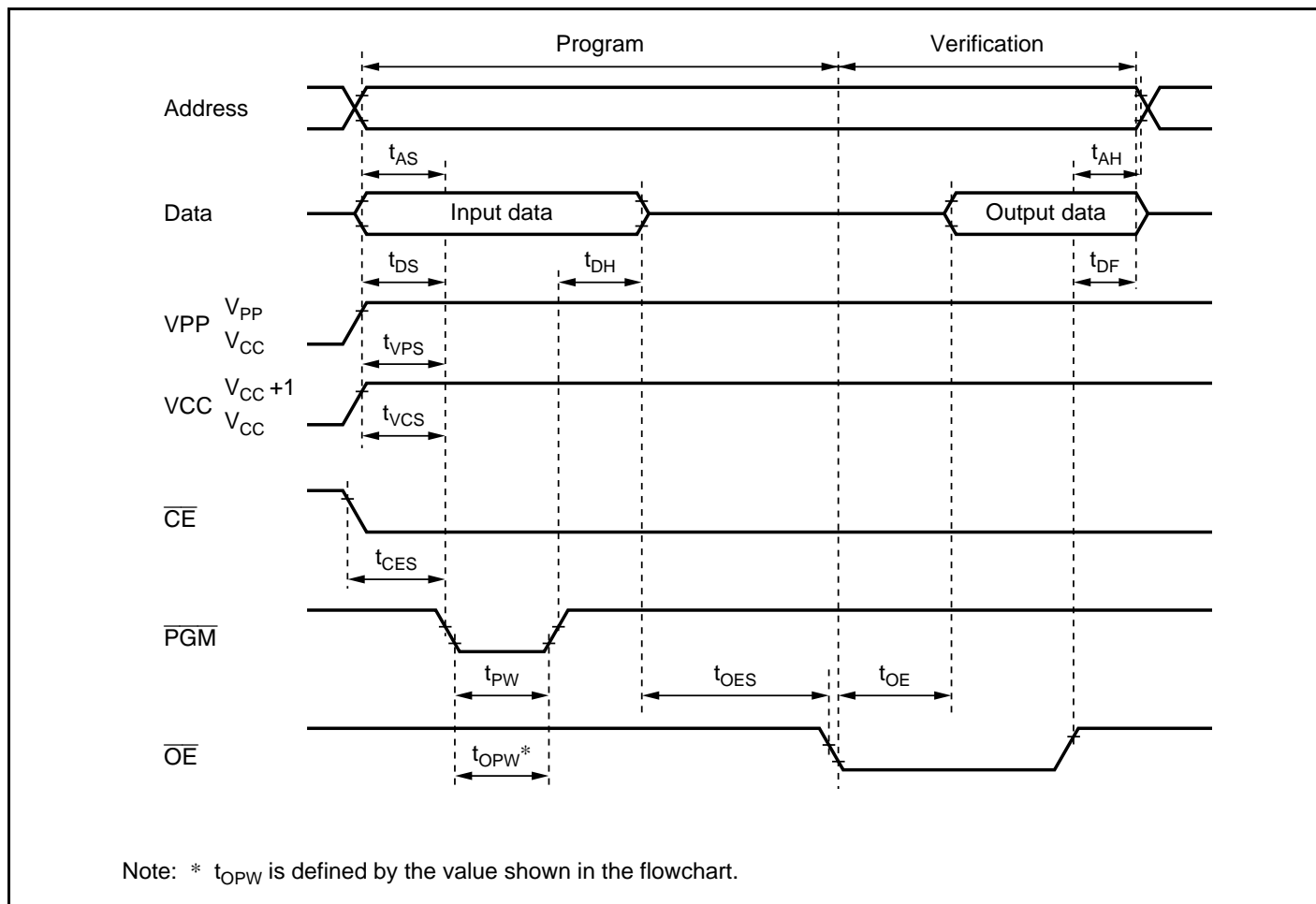
Figure 22.5 PROM Programming/Verification Timing
