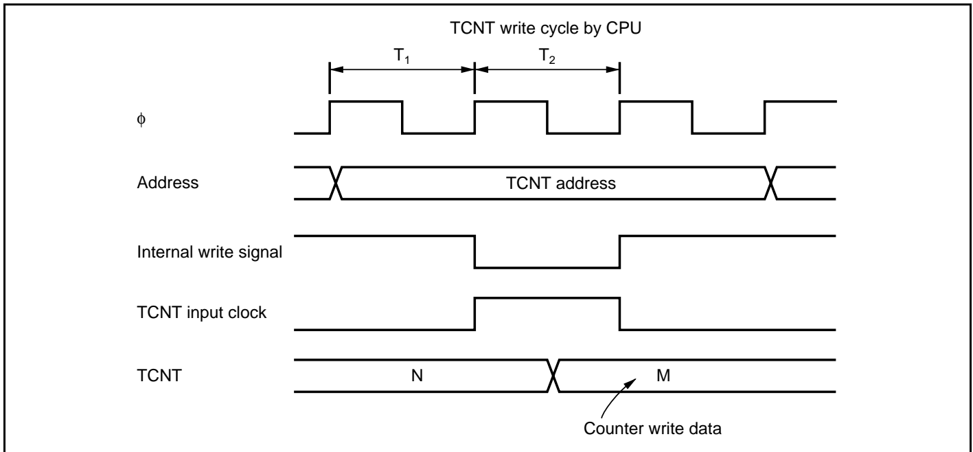
Figure 12.11 Contention between TCNT Write and Increment
