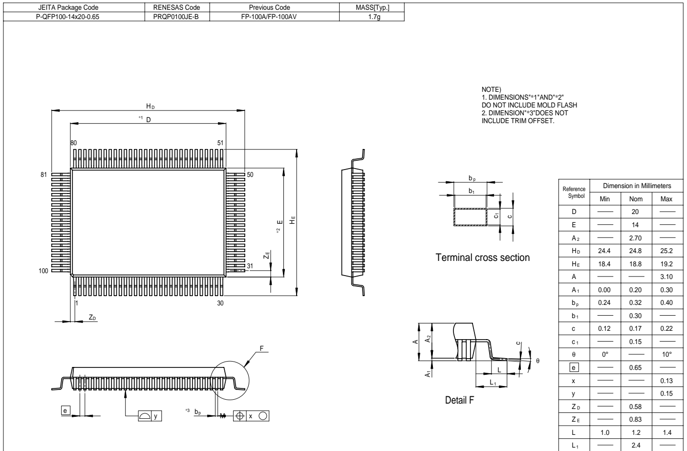
Figure C.3 FP-100A Package Dimensions
