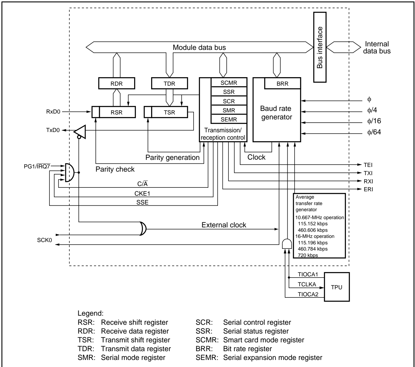
Figure 15.2 Block Diagram of SCI_0 of H8S/2239 Group
