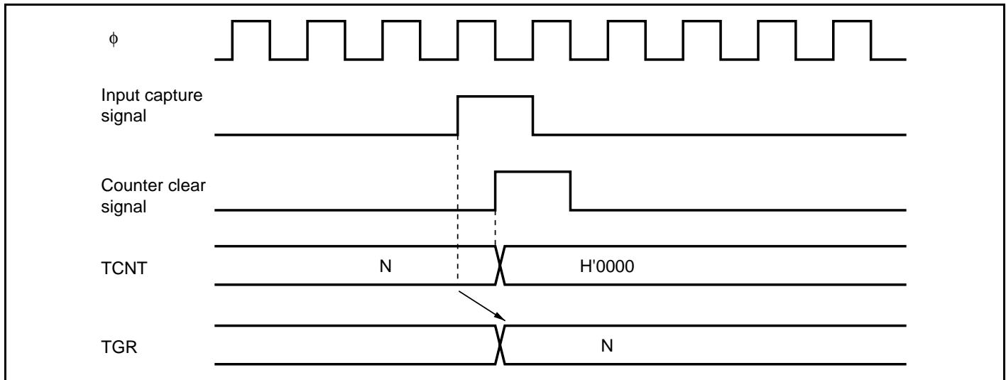
Figure 11.36 Counter Clear Timing (Input Capture)
