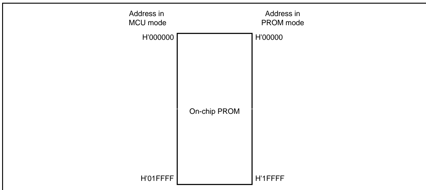
Figure 22.3 Memory Map in PROM Mode
