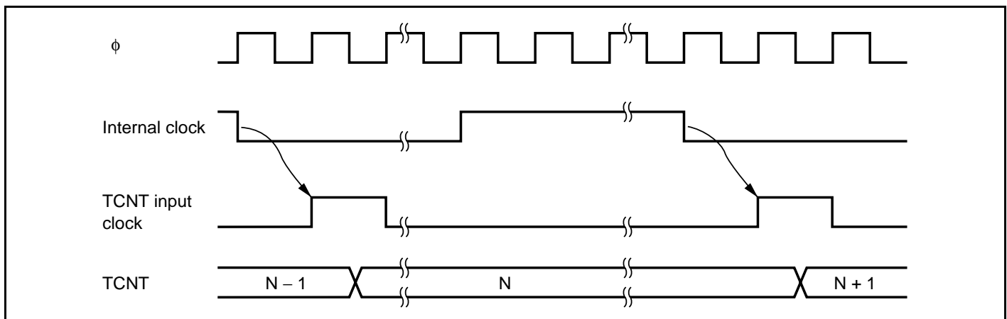
Figure 12.3 Count Timing for Internal Clock Input
