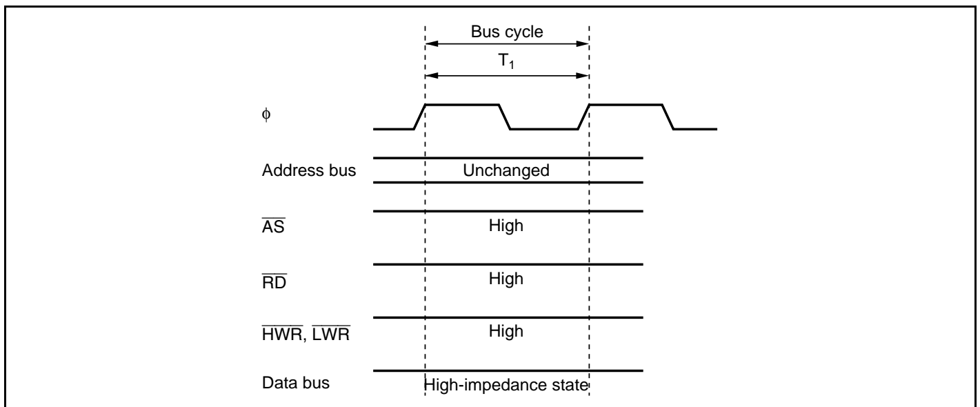
Figure 7.5 Pin States during On-Chip Memory Access
