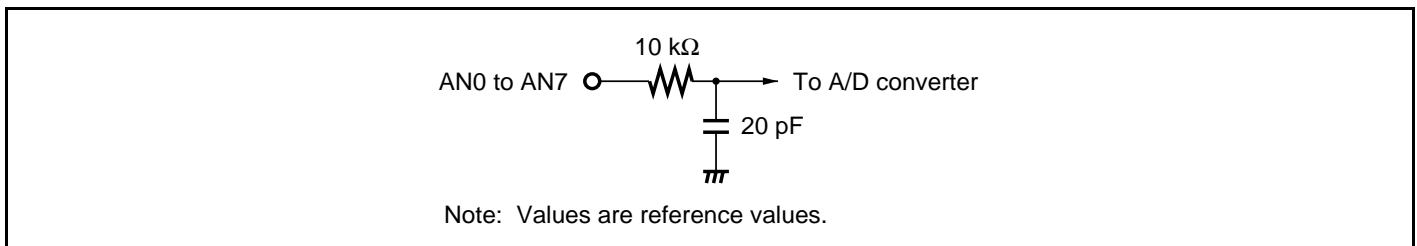
Figure 17.11 Analog Input Pin Equivalent Circuit
