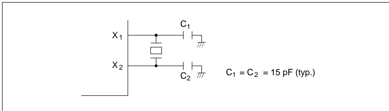
Figure 4-7 Typical Connection to 32.768-kHz Crystal Oscillator
