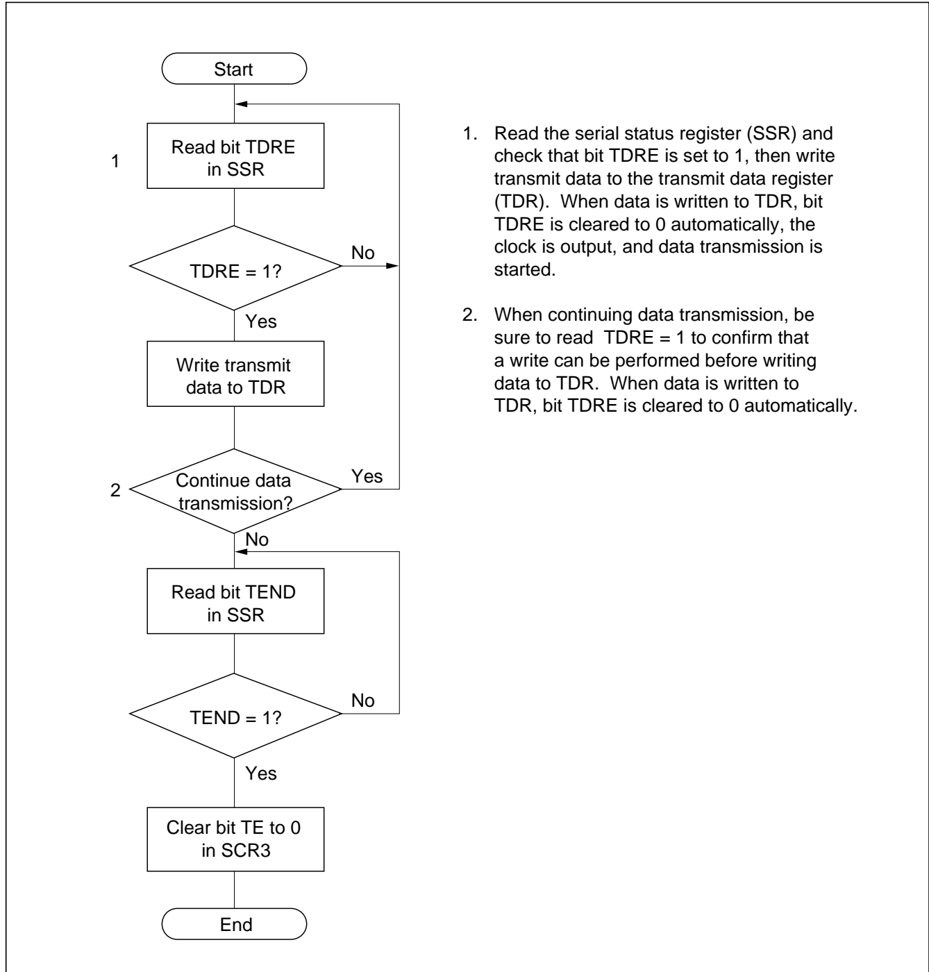
Figure 10-16 Example of Data Transmission Flowchart (Synchronous Mode)
