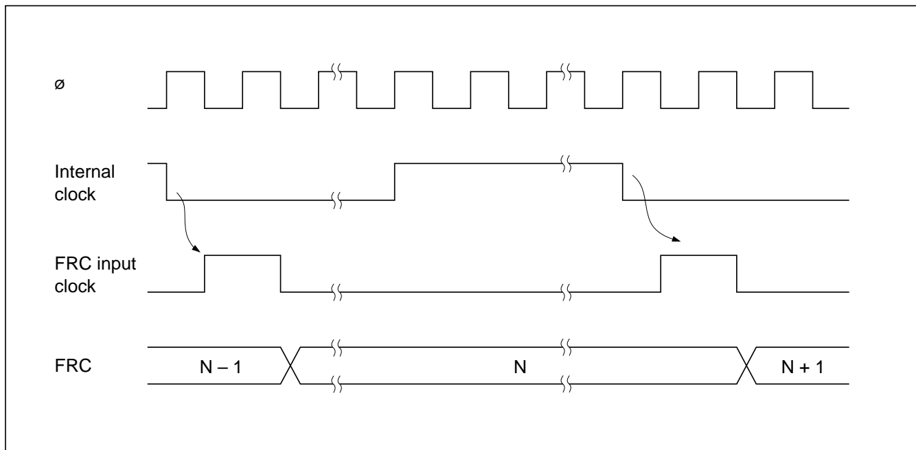
Figure 9-20 Increment Timing with Internal Clock
