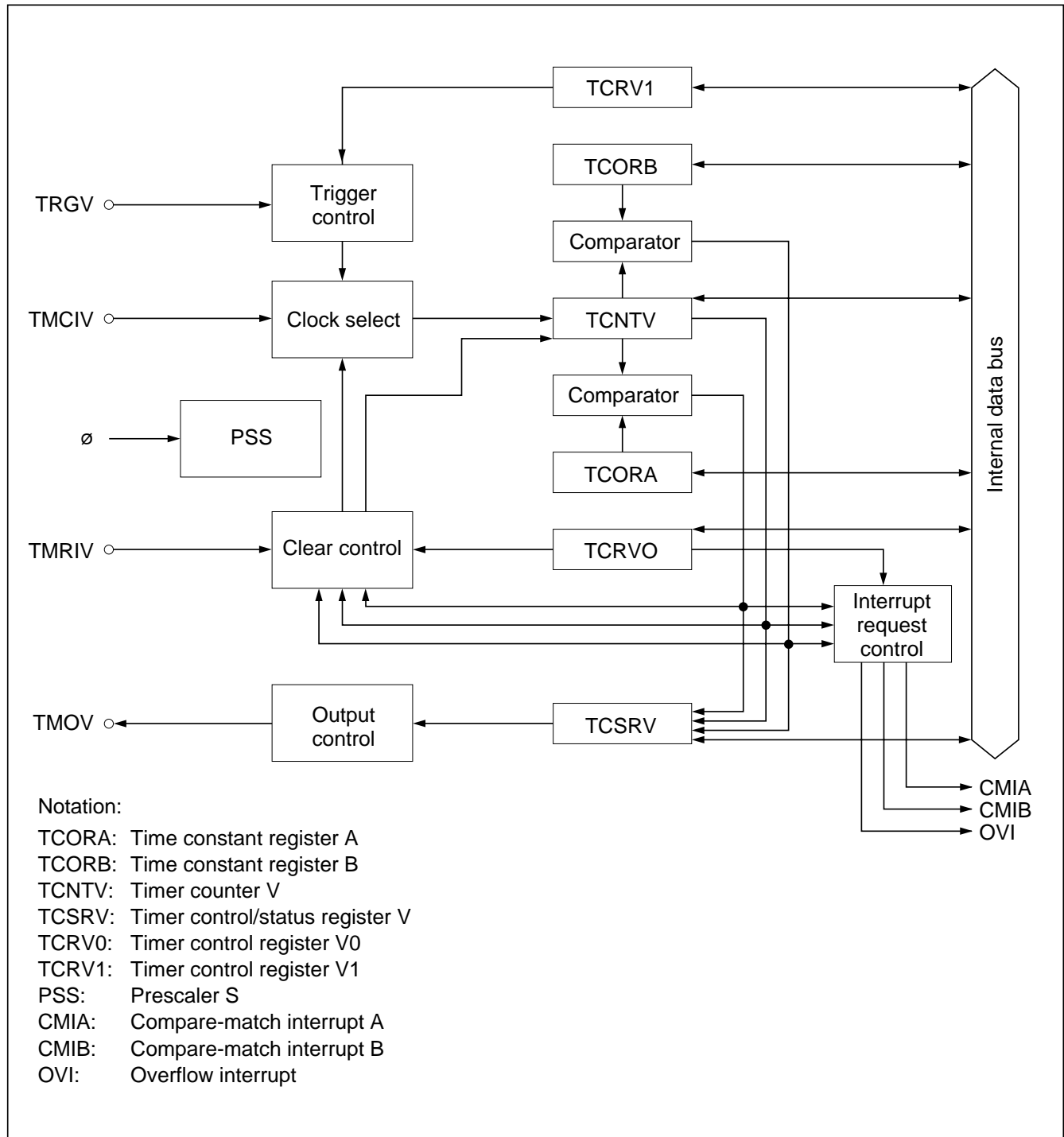
Figure 9-3 Block Diagram of Timer V
