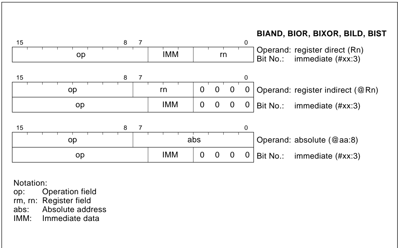
Figure 2-7 Bit Manipulation Instruction Codes (cont)
