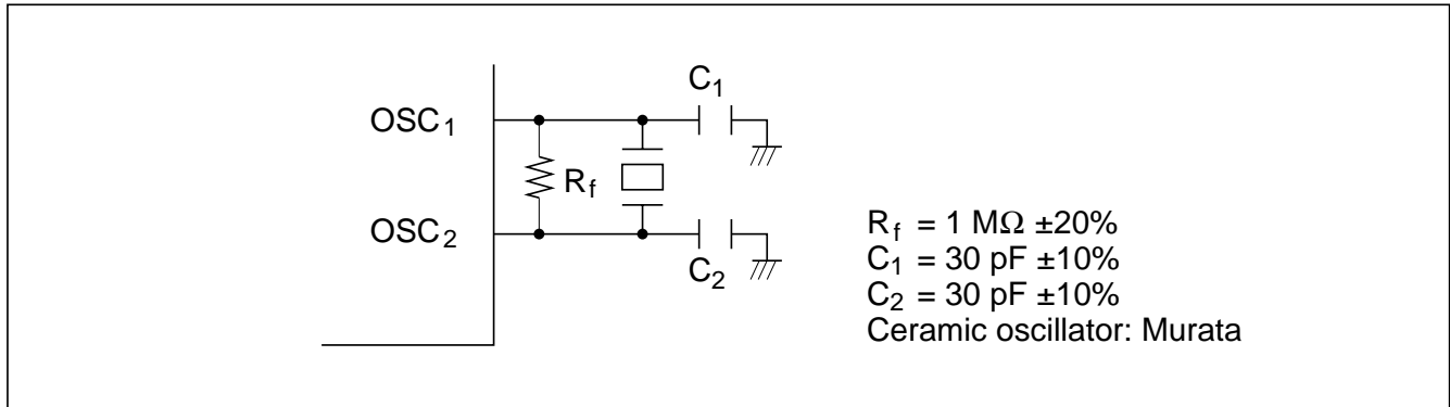
Figure 4-4 Typical Connection to Ceramic Oscillator
