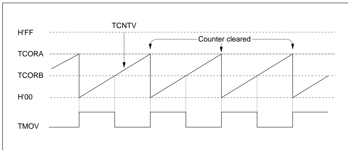
Figure 9-11 Pulse Output Example
