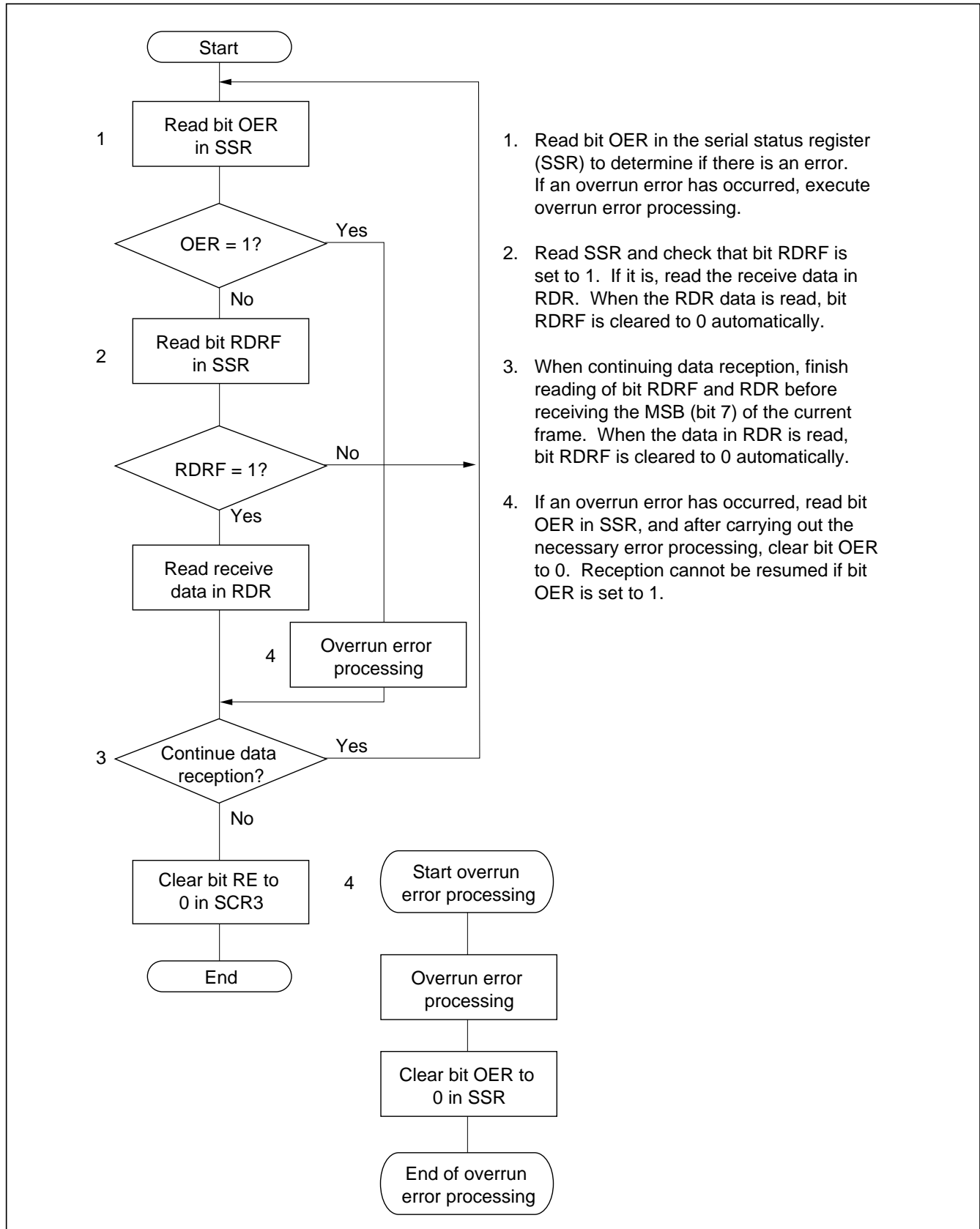
Figure 10-18 Example of Data Reception Flowchart (Synchronous Mode)
