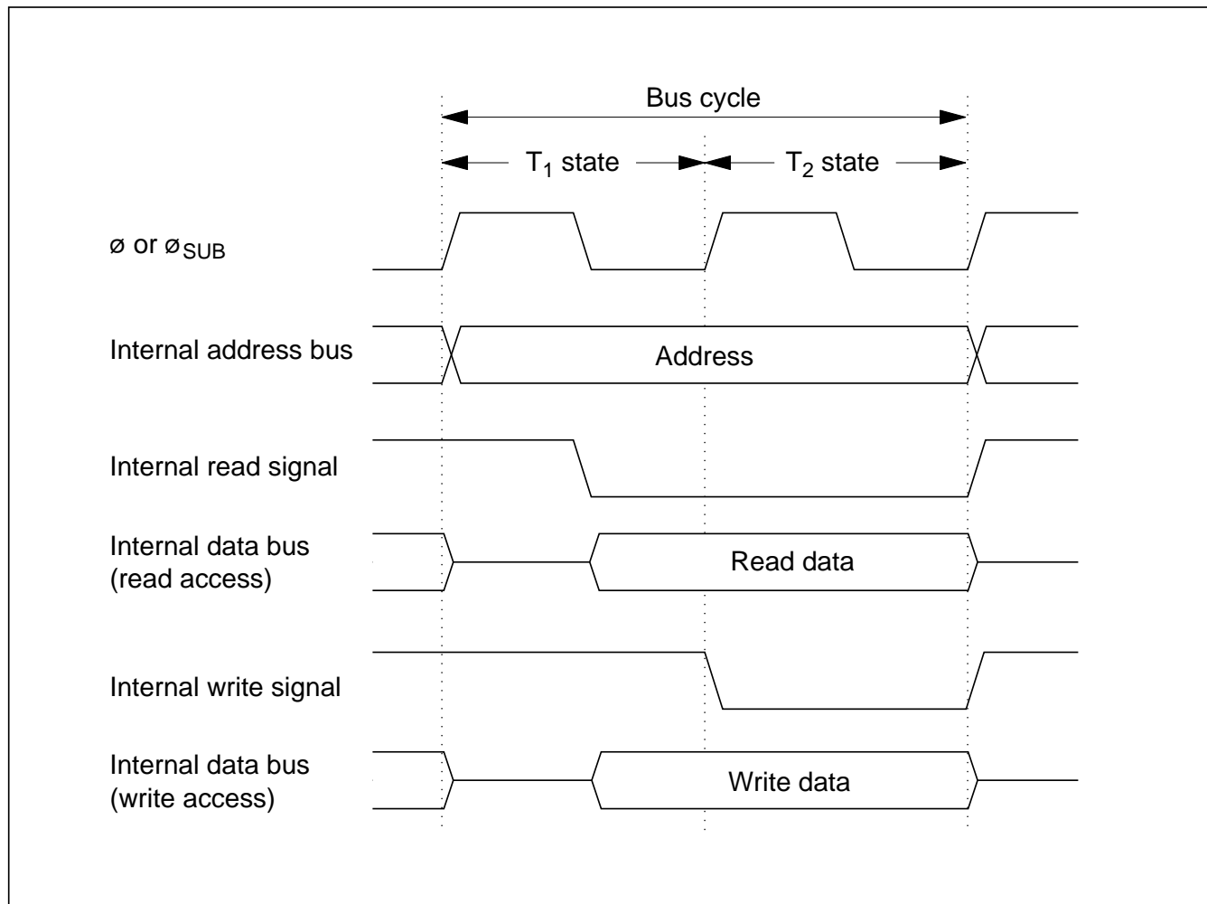
Figure 2-11 On-Chip Memory Access Cycle
