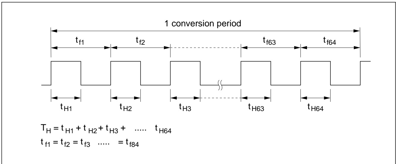
Figure 11-2 PWM Output Waveform
