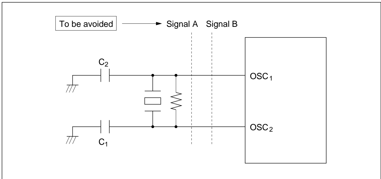
Figure 4-5 Board Design of Oscillator Circuit
