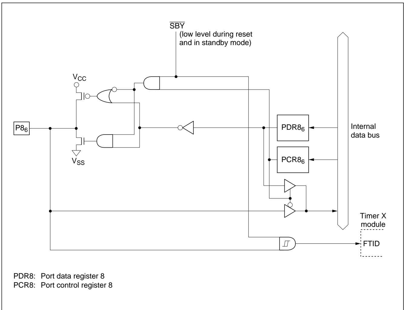
Figure C-7 (b) Port 8 Block Diagram (Pin P8 6 )
