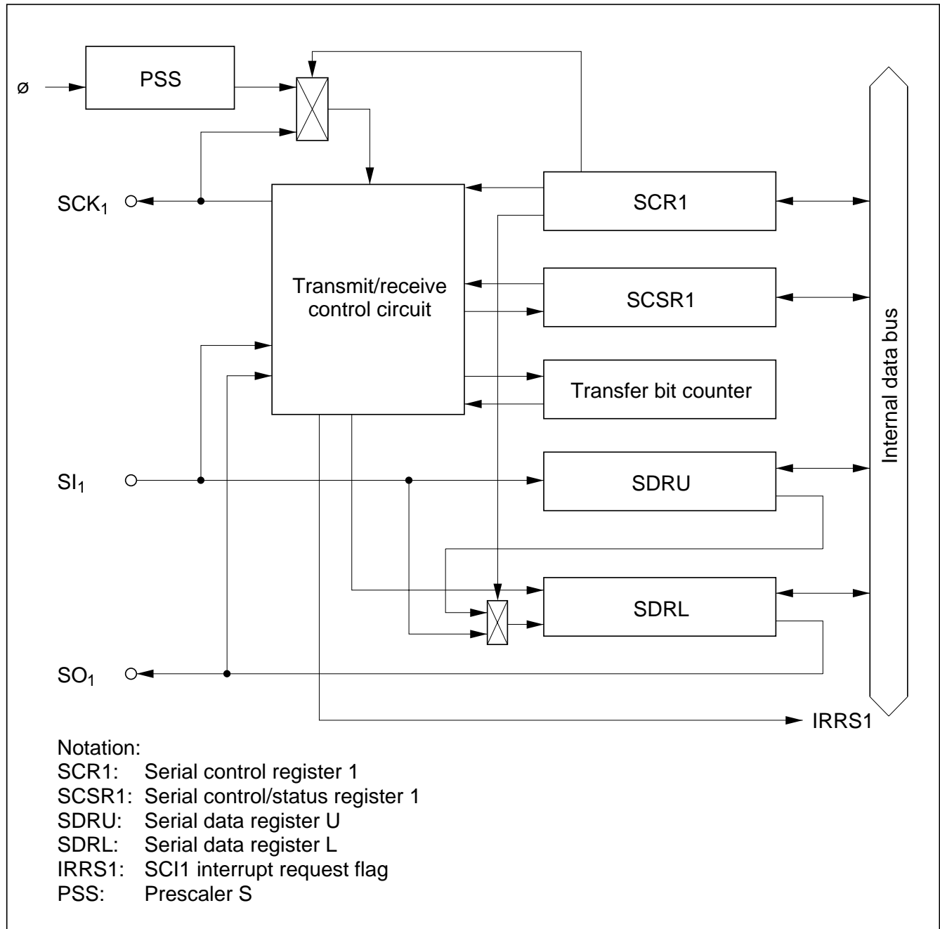
Figure 10-1 SCI1 Block Diagram
