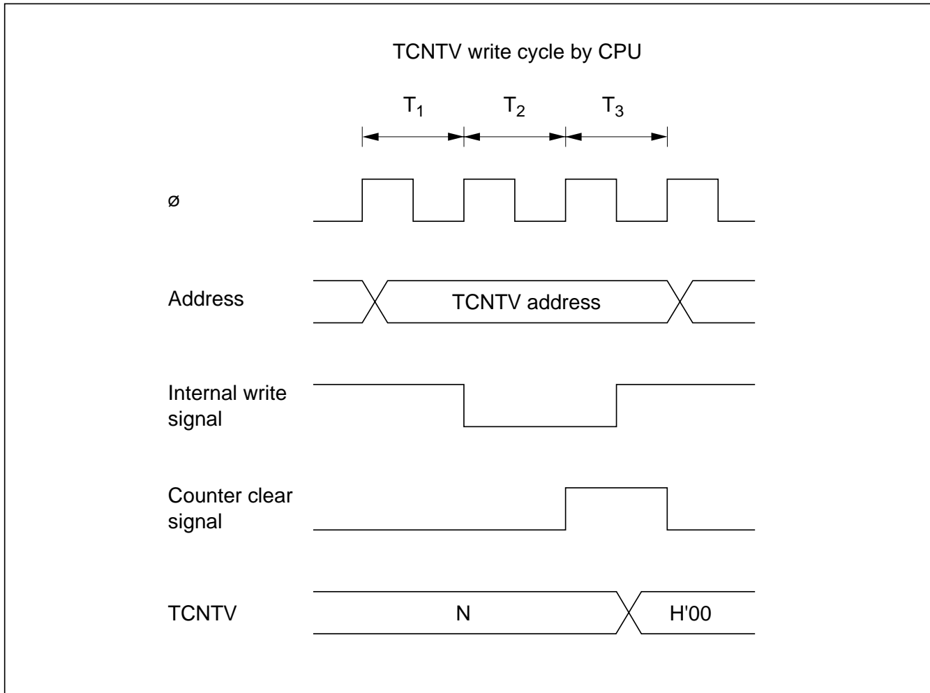
Figure 9-13 Contention between TCNTV Write and Clear
