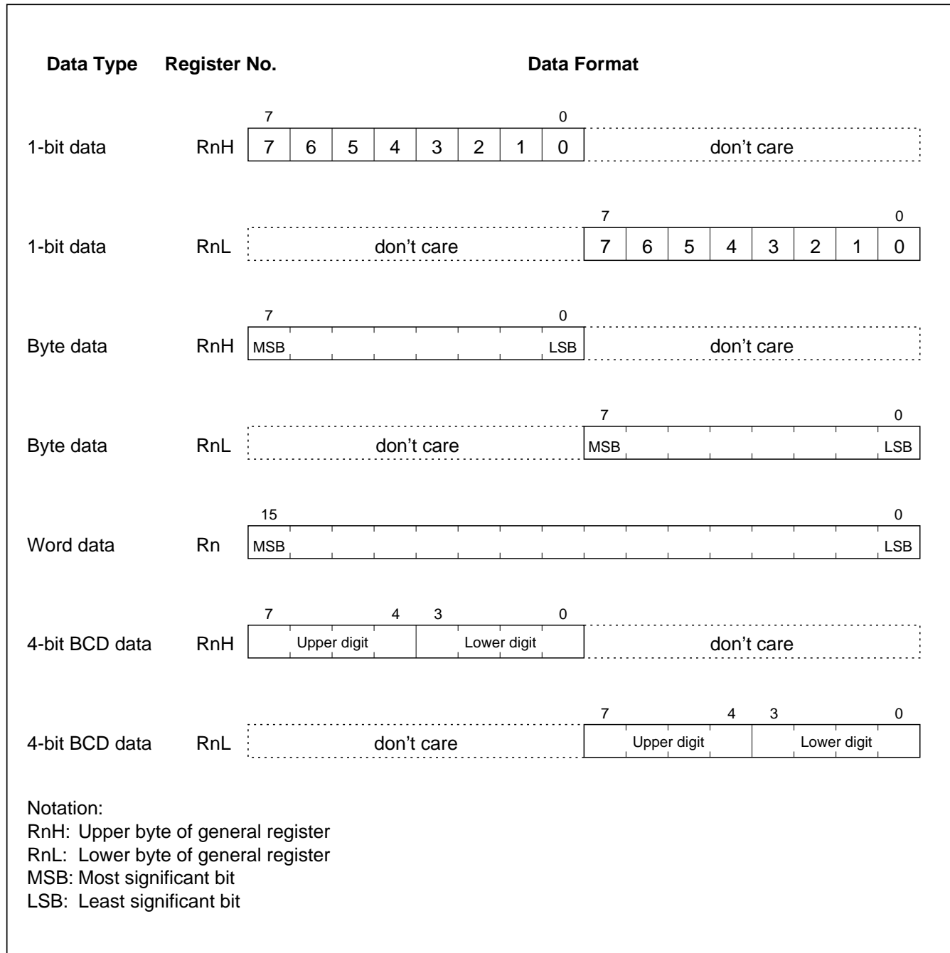
Figure 2-3 Register Data Formats
