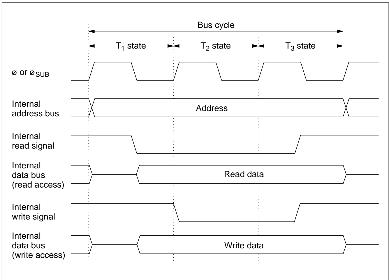
Figure 2-13 On-Chip Peripheral Module Access Cycle (3-State Access)
