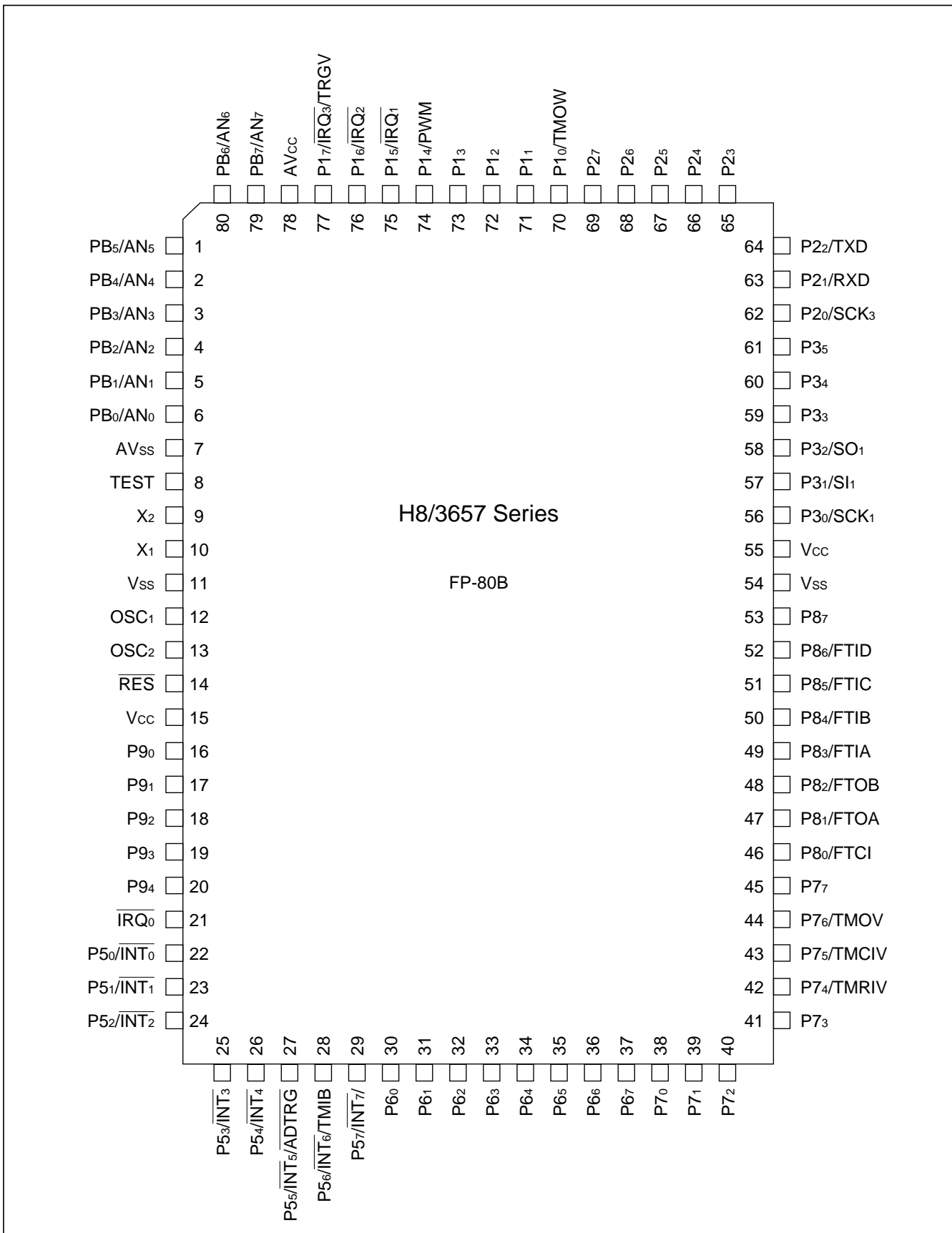
Figure 1-3 Pin Arrangement (FP-80B: Top View)
