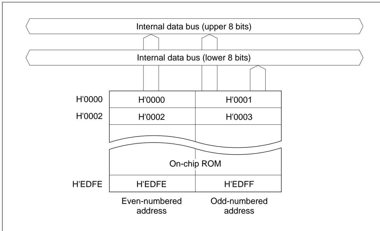
Figure 6-1 ROM Block Diagram (H8/3657)
