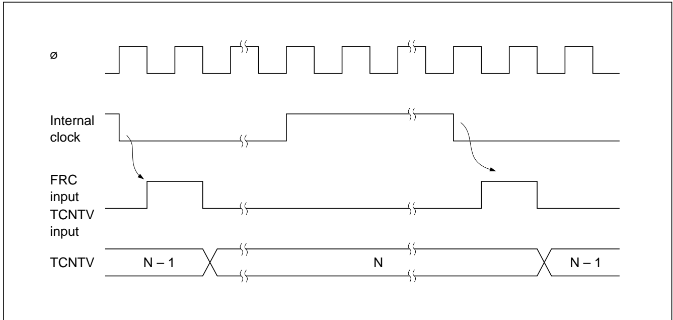
Figure 9-4 Increment Timing with Internal Clock
