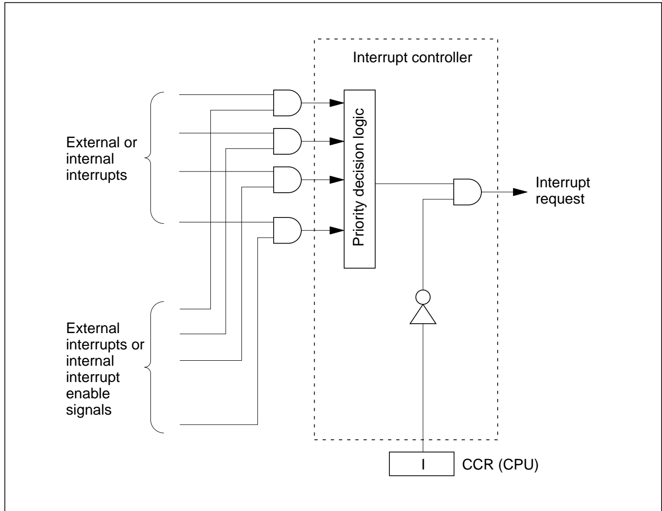
Figure 3-2 Block Diagram of Interrupt Controller
