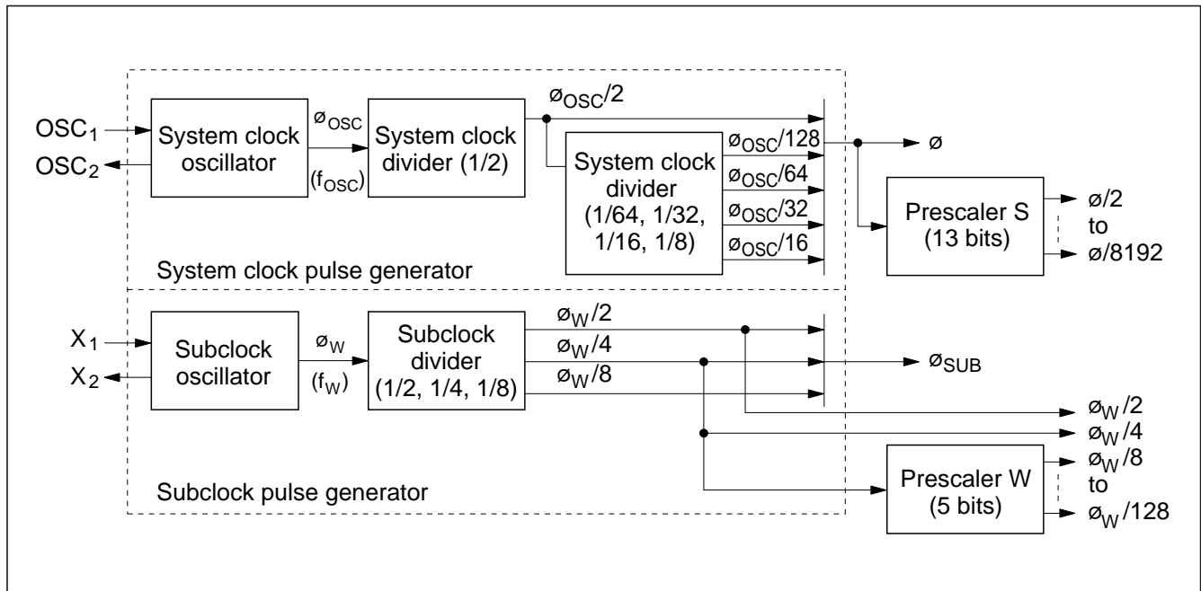
Figure 4-1 Block Diagram of Clock Pulse Generators
