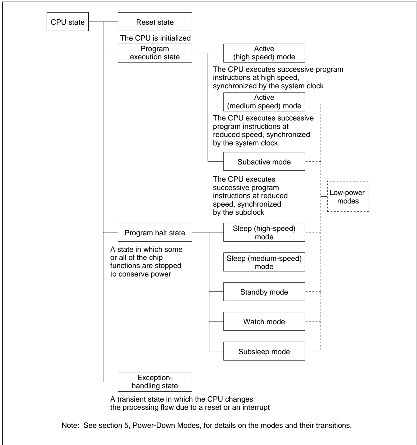
Figure 2-14 CPU Operation States
