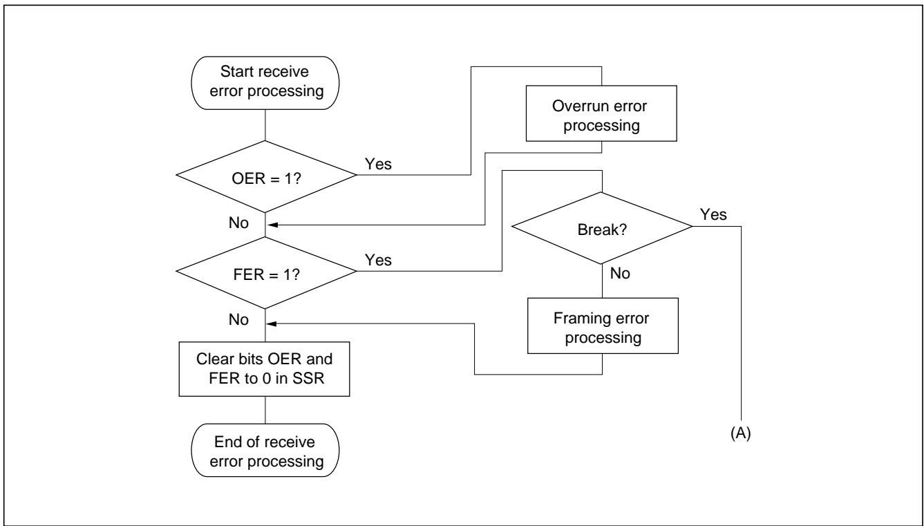
Figure 10-24 Example of Multiprocessor Data Reception Flowchart (cont)
