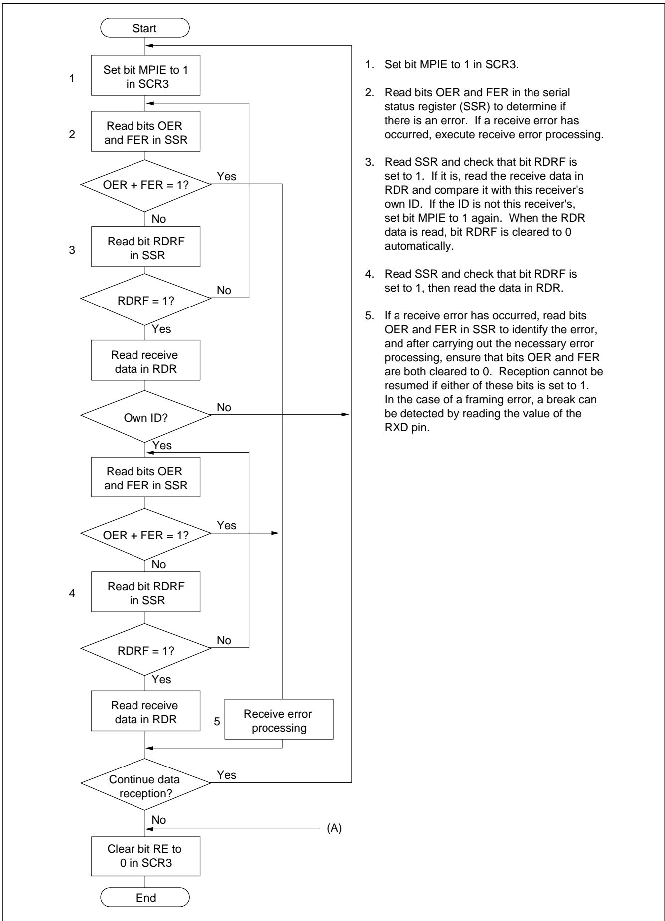
Figure 10-24 Example of Multiprocessor Data Reception Flowchart
