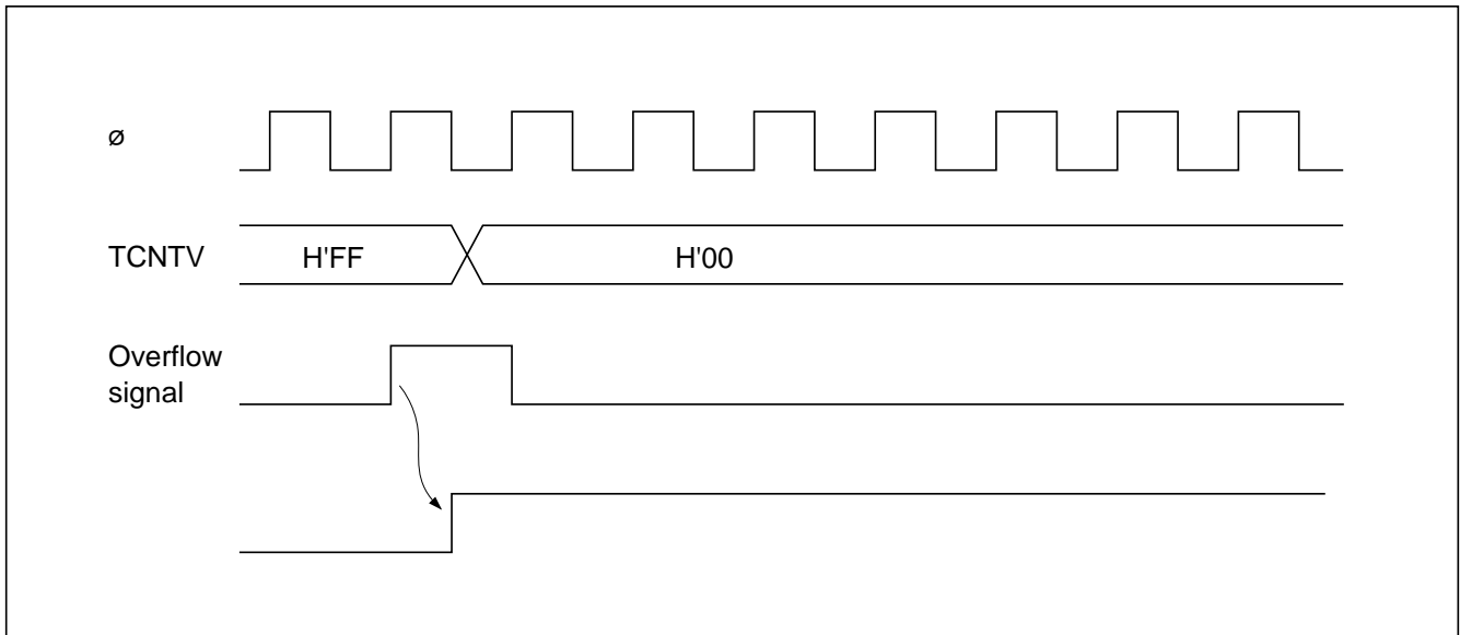
Figure 9-6 OVF Set Timing
