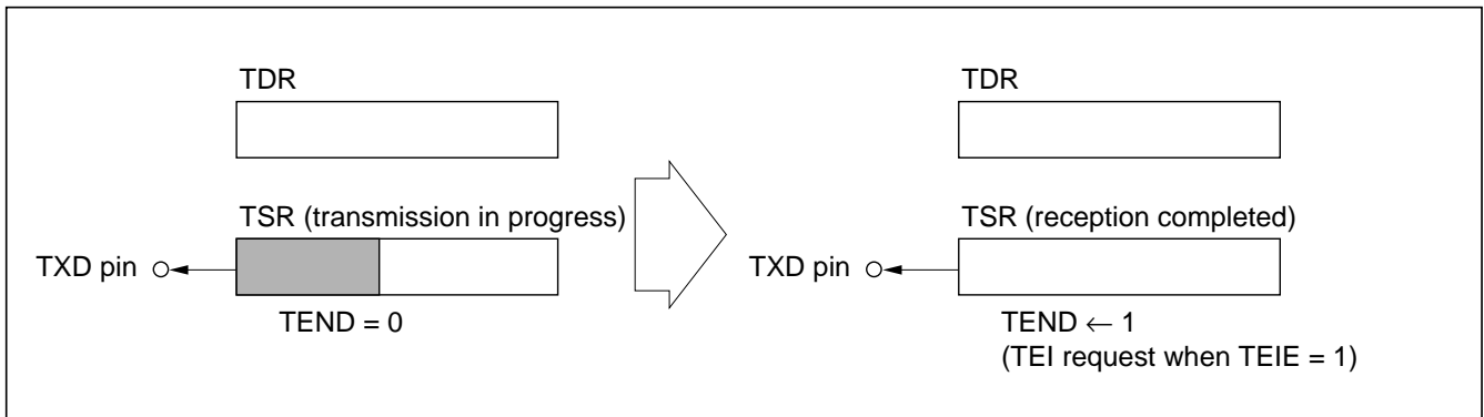
Figure 10-7 (c) TEND Setting and TEI Interrupt
