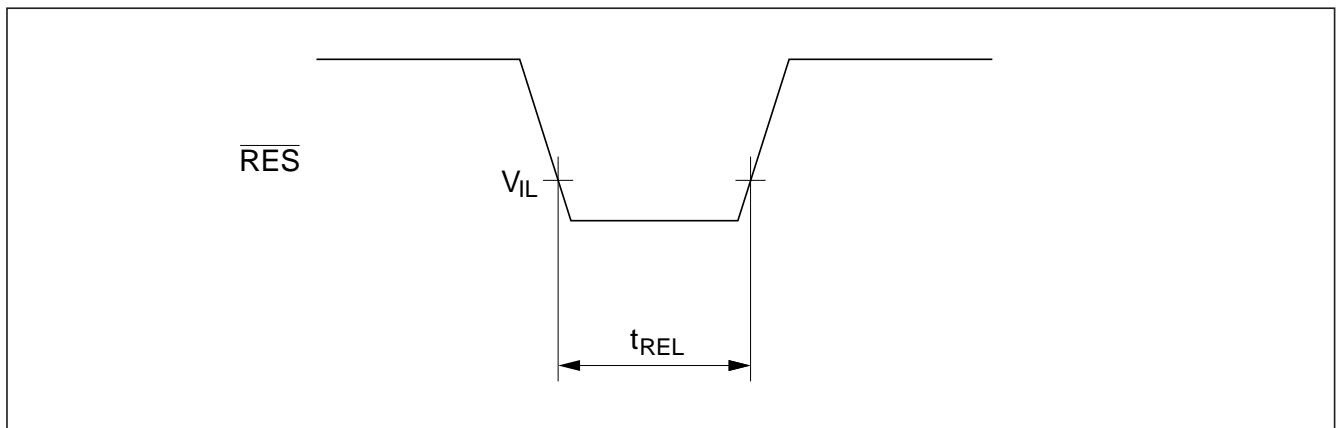
Figure 13-2 \overline{RES} Low Width Timing
