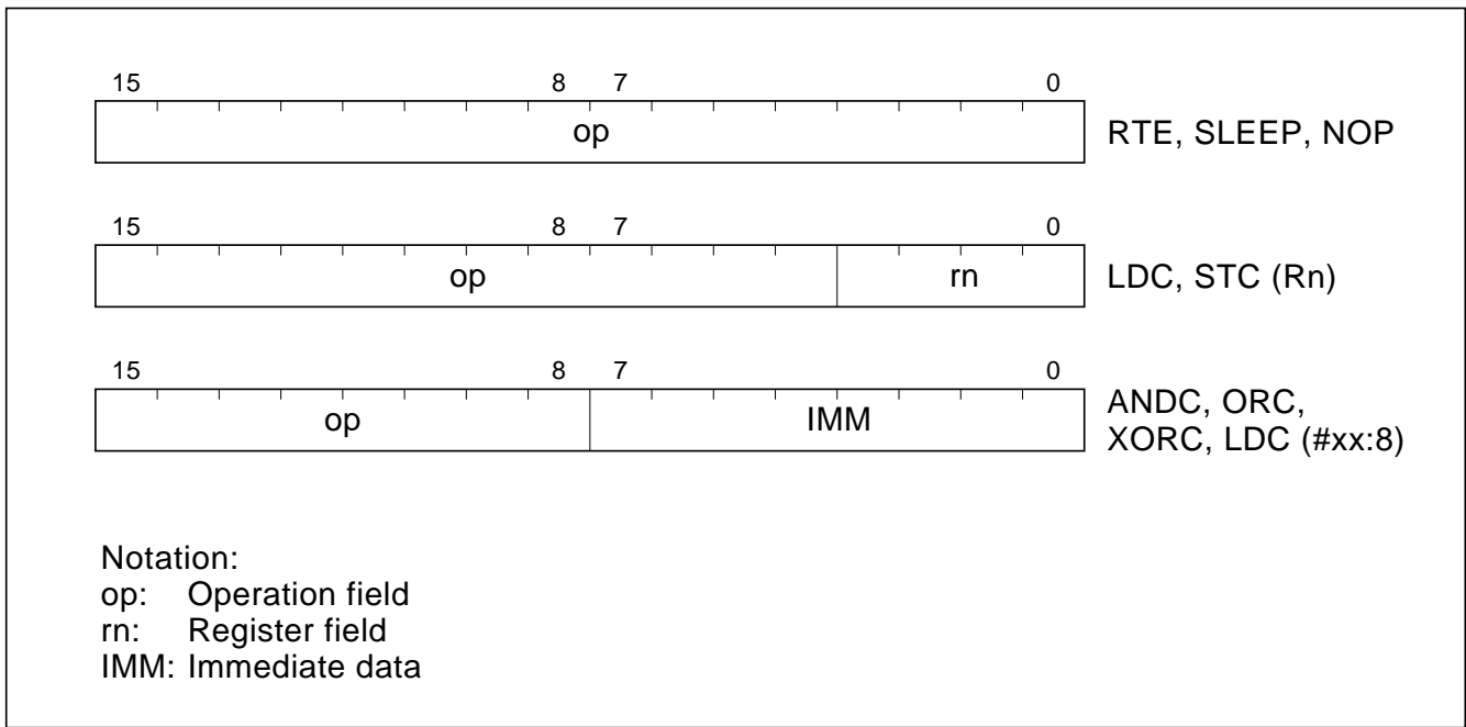
Figure 2-9 System Control Instruction Codes
