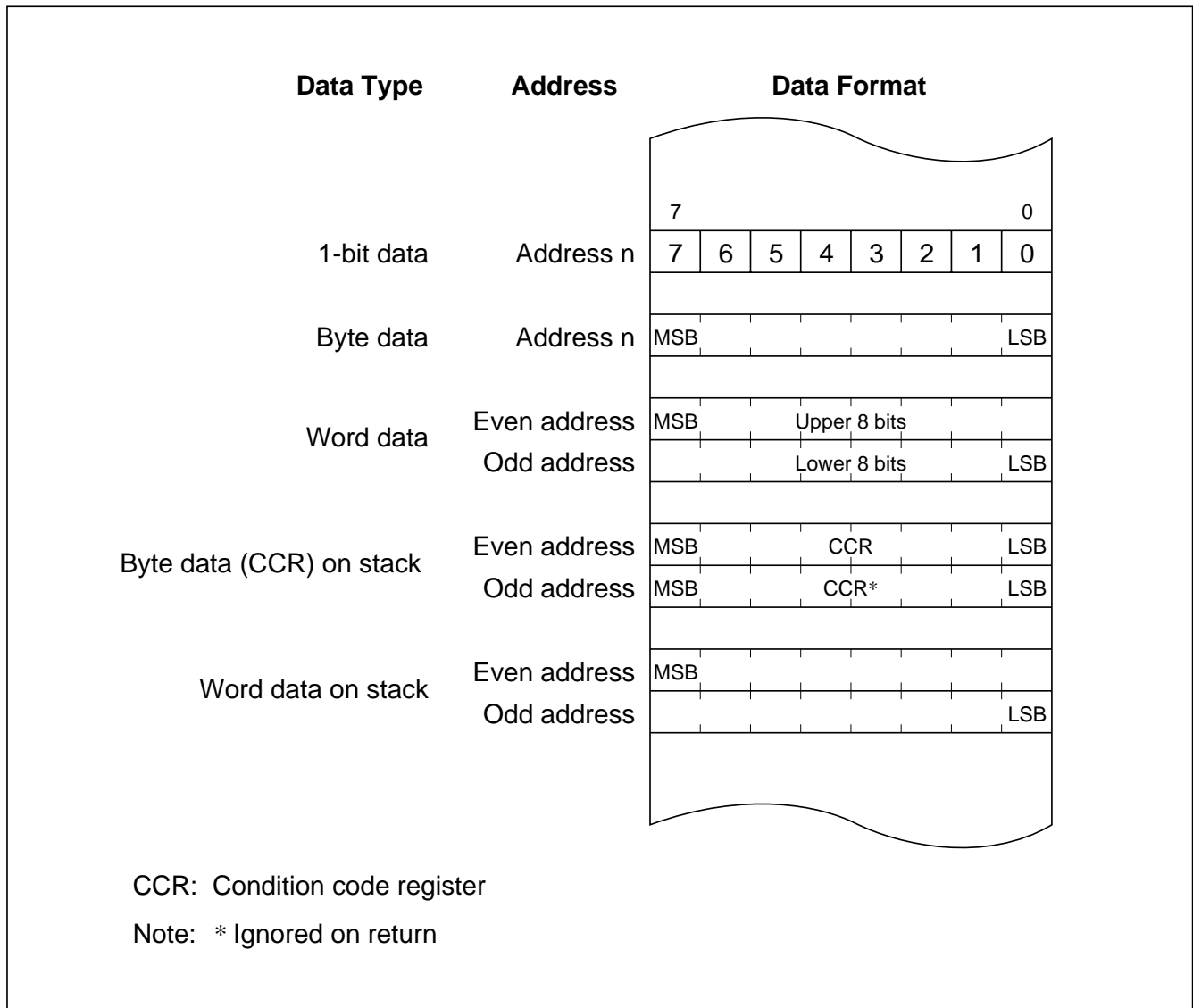
Figure 2-4 Memory Data Formats
