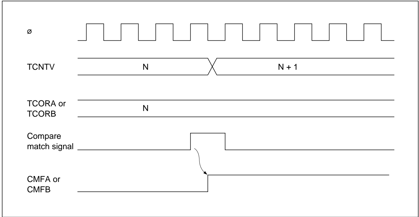
Figure 9-7 CMFA and CMFB Set Timing
