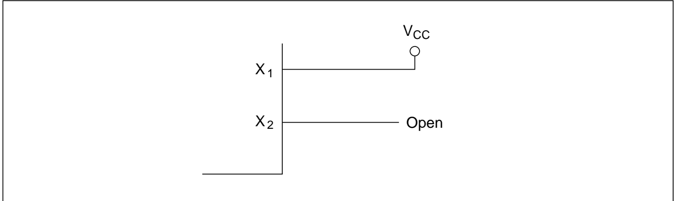
Figure 4-9 Pin Connection when not Using Subclock
