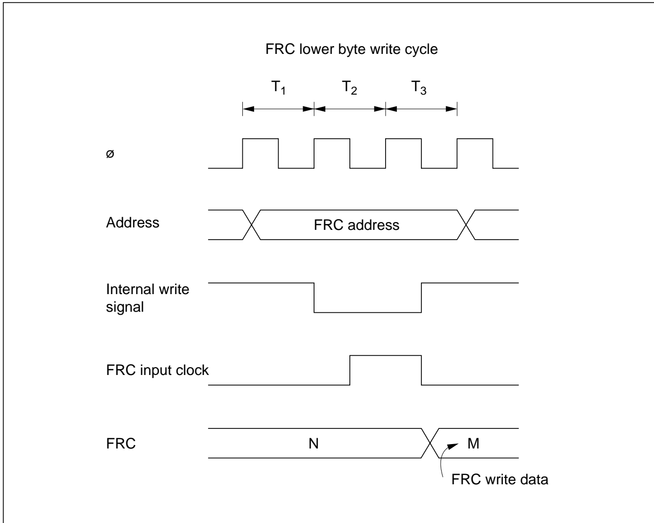
Figure 9-33 Contention between FRC Write and Increment
