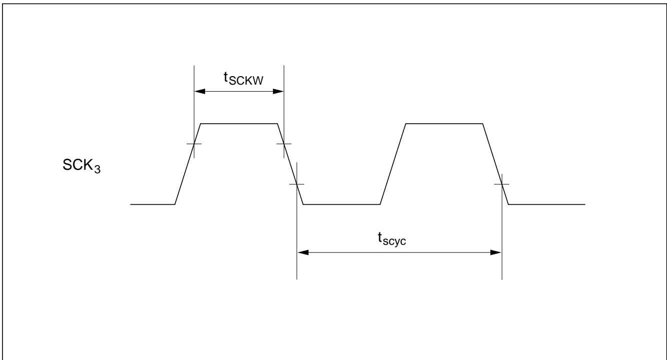
Figure 13-5 SCK 3 Input Clock Timing
