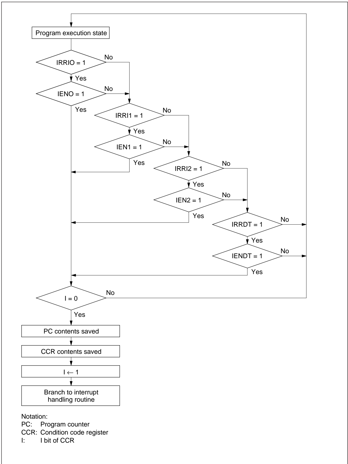
Figure 3-3 Flow up to Interrupt Acceptance
