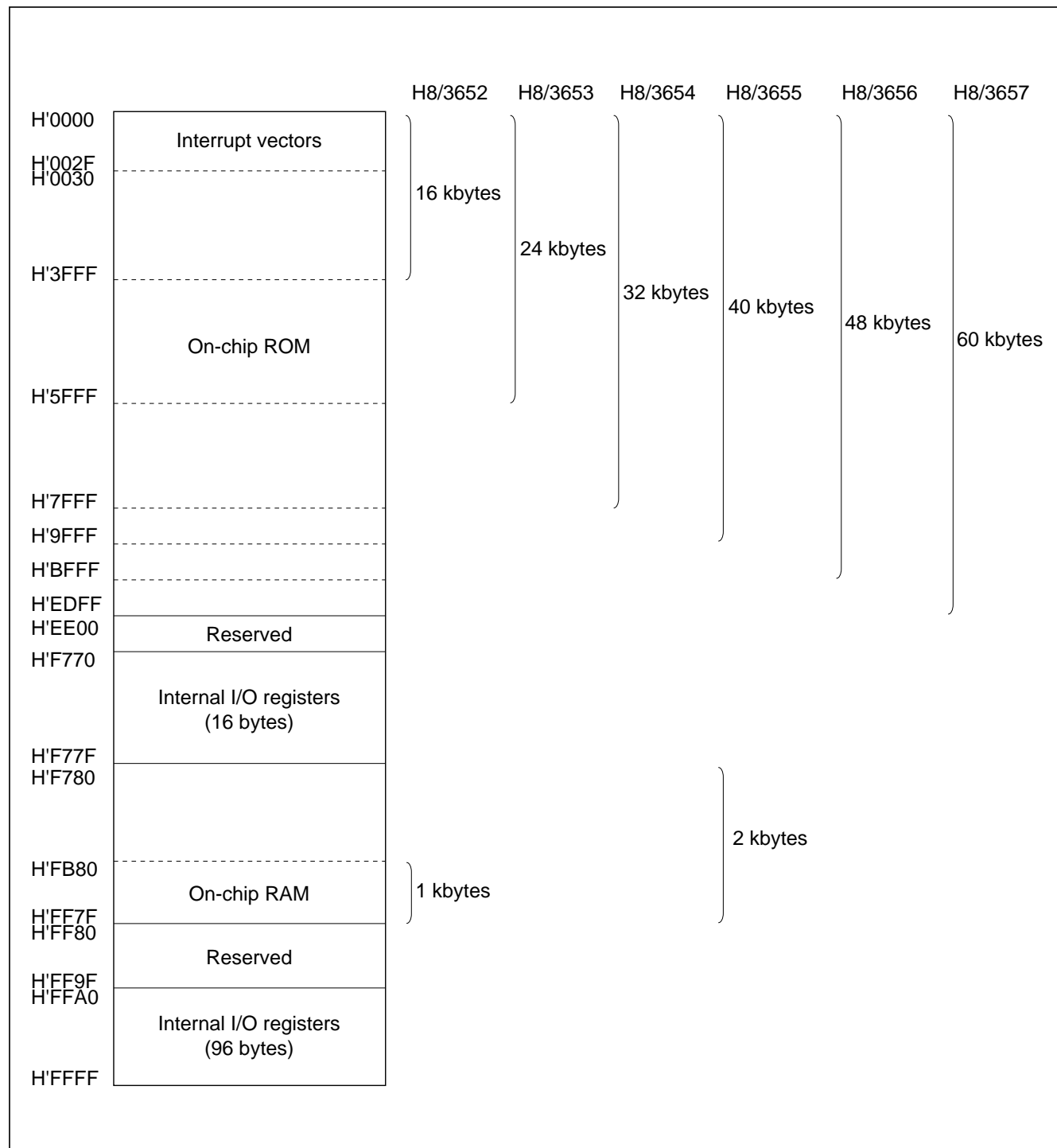
Figure 2-16 H8/3657 Series Memory Map
