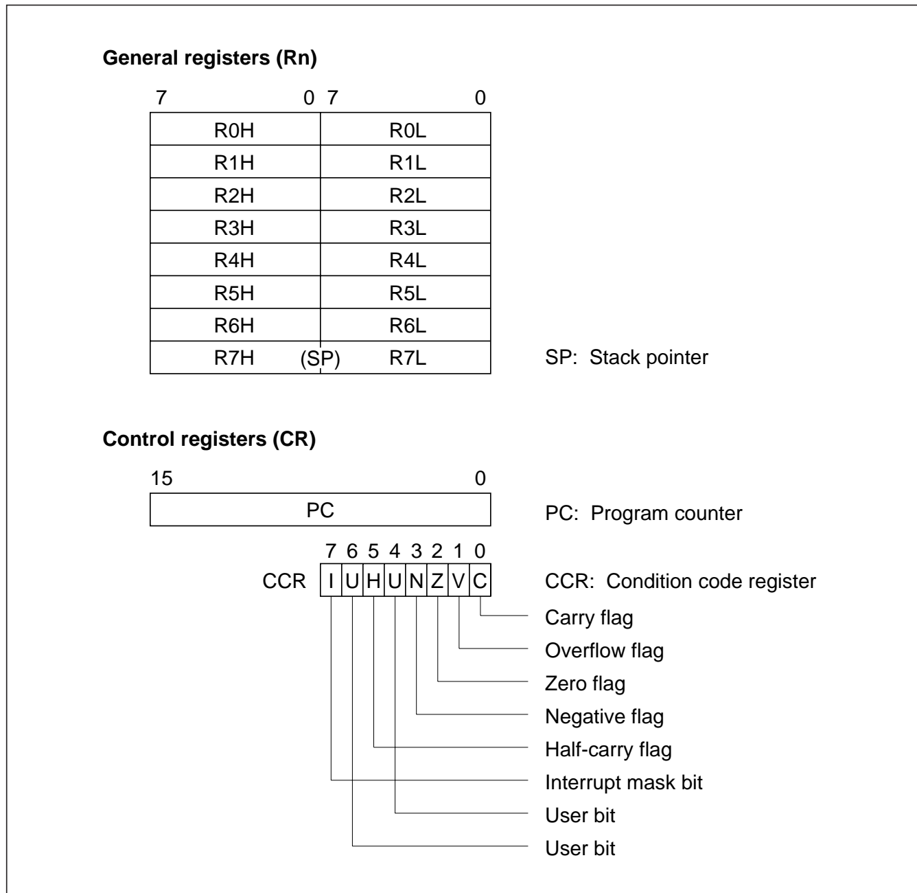
Figure 2-1 CPU Registers
