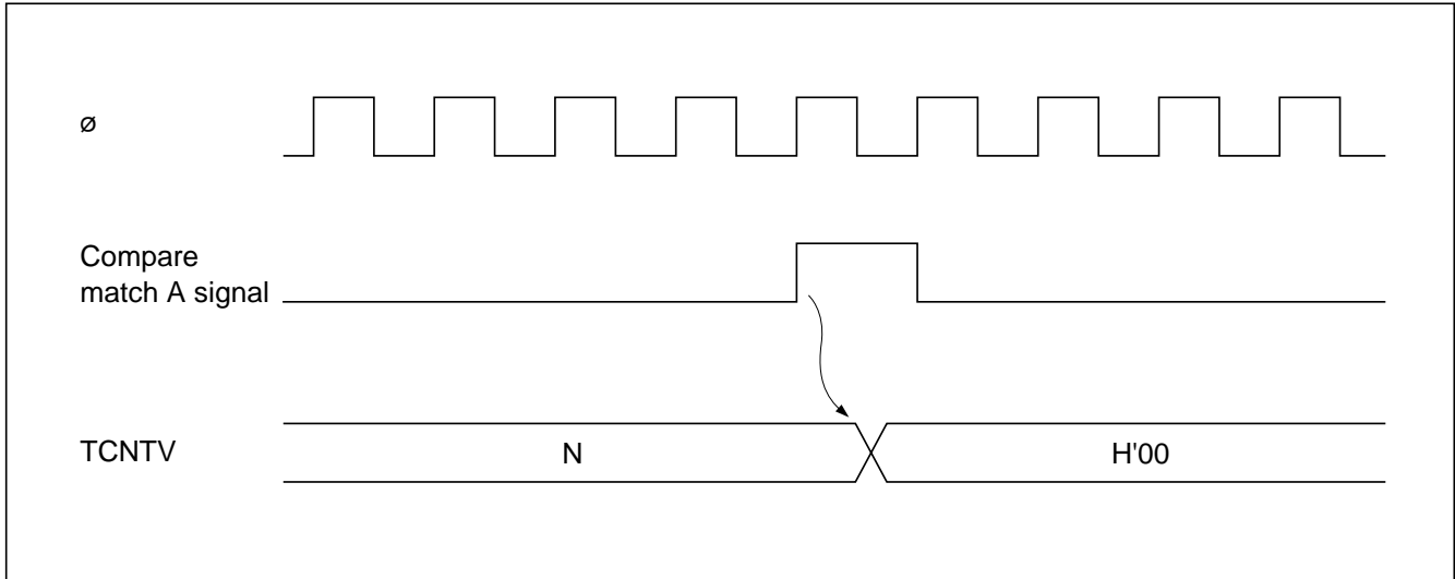
Figure 9-9 Clear Timing by Compare Match
