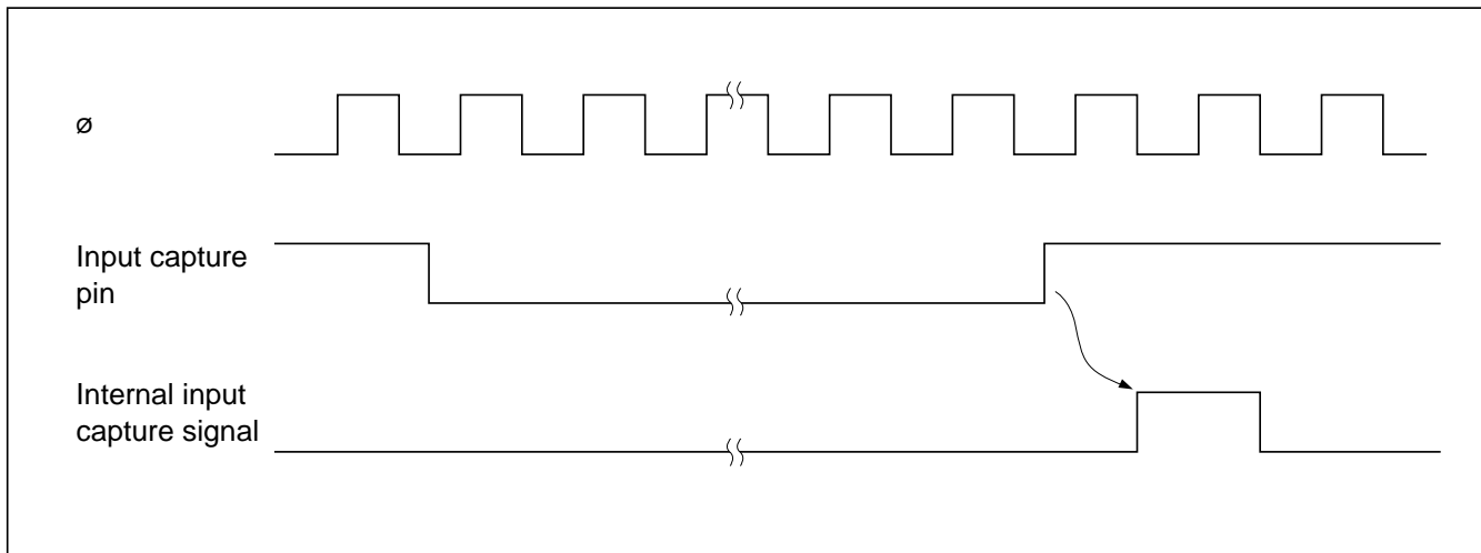
Figure 9-24 Input Capture Signal Timing (Normal Case)
