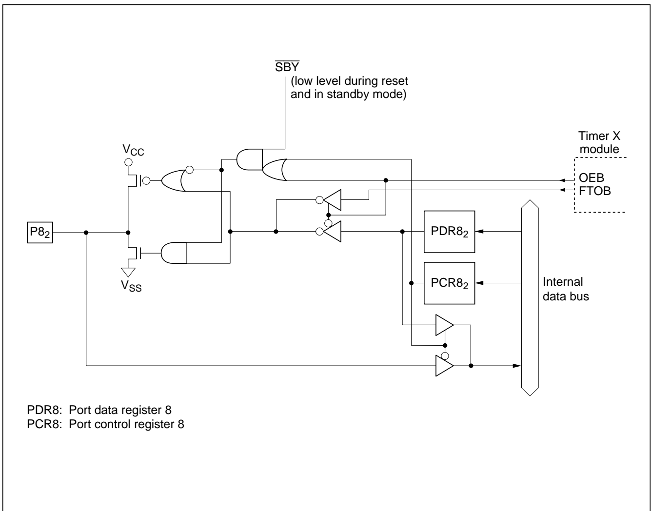
Figure C-7 (f) Port 8 Block Diagram (Pin P8 2 )
