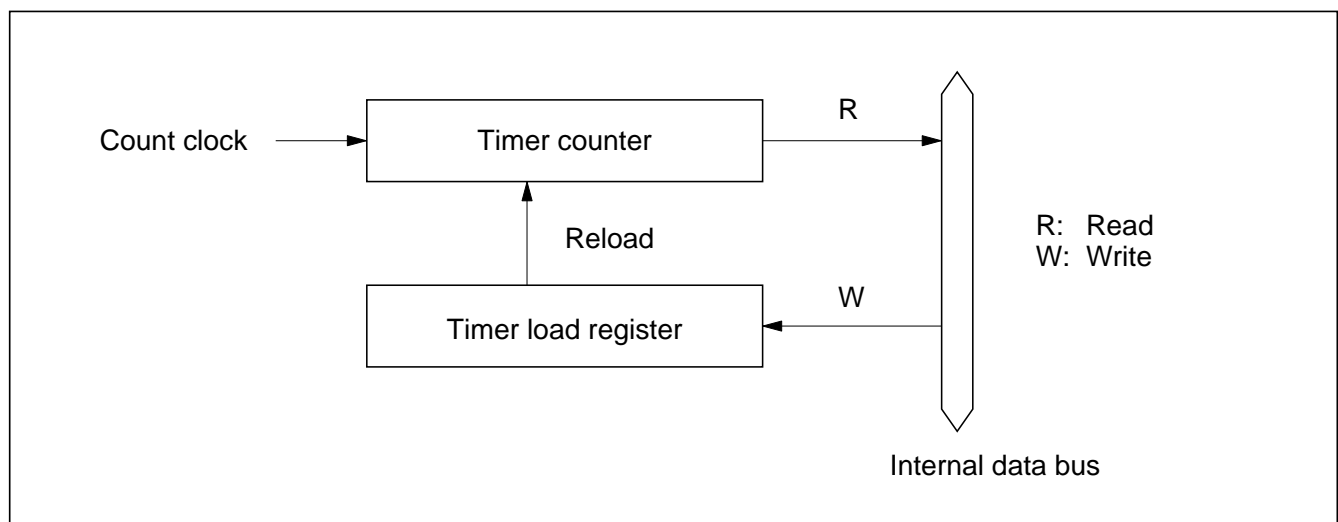
Figure 2-18 Timer Configuration Example
