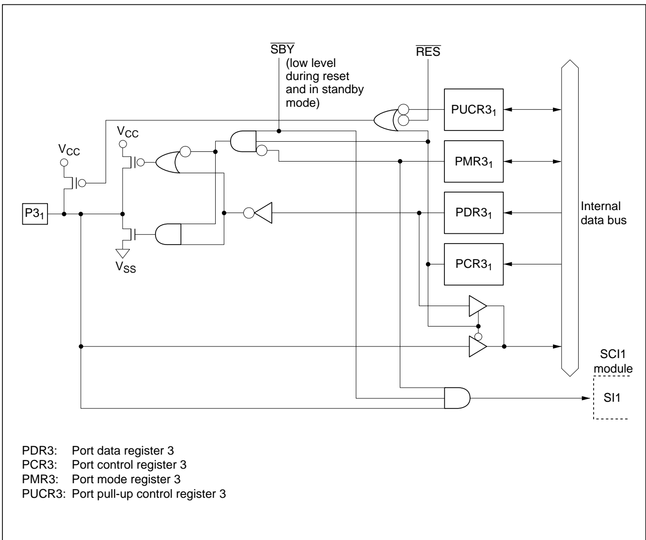
Figure C-3 (c) Port 3 Block Diagram (Pin P3 1 )
