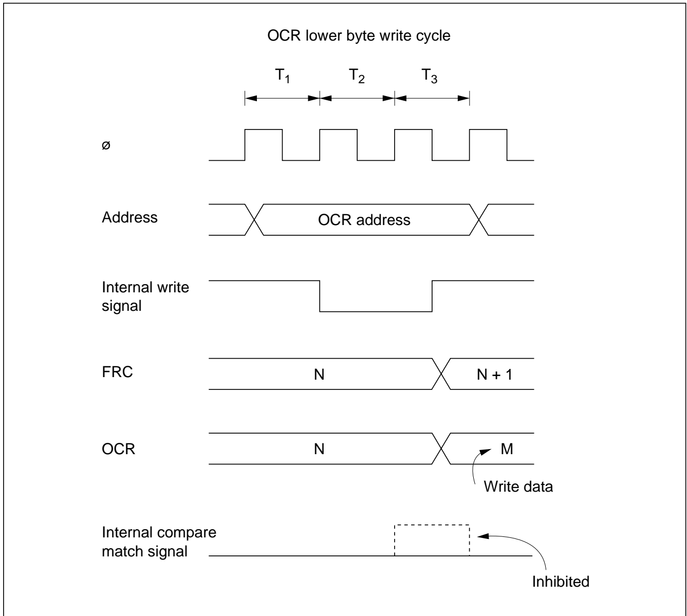
Figure 9-34 Contention between OCR Write and Compare Match
