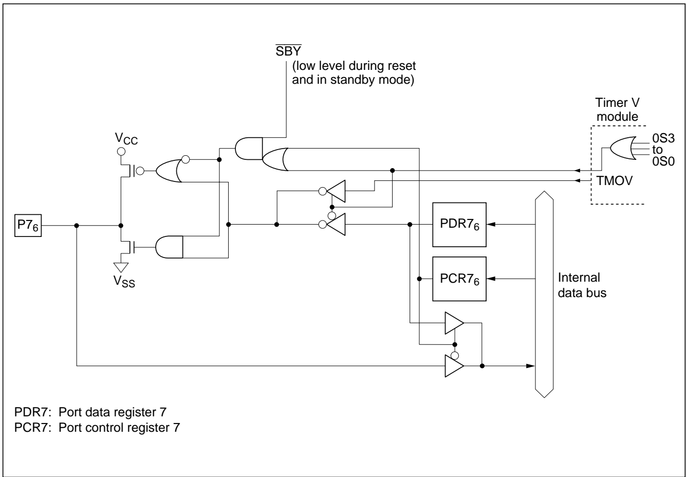
Figure C-6 (b) Port 7 Block Diagram (Pin P7 6 )
