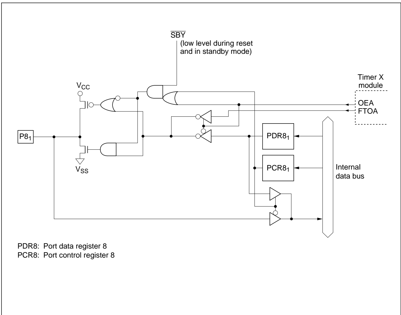
Figure C-7 (g) Port 8 Block Diagram (Pin P8 1 )
