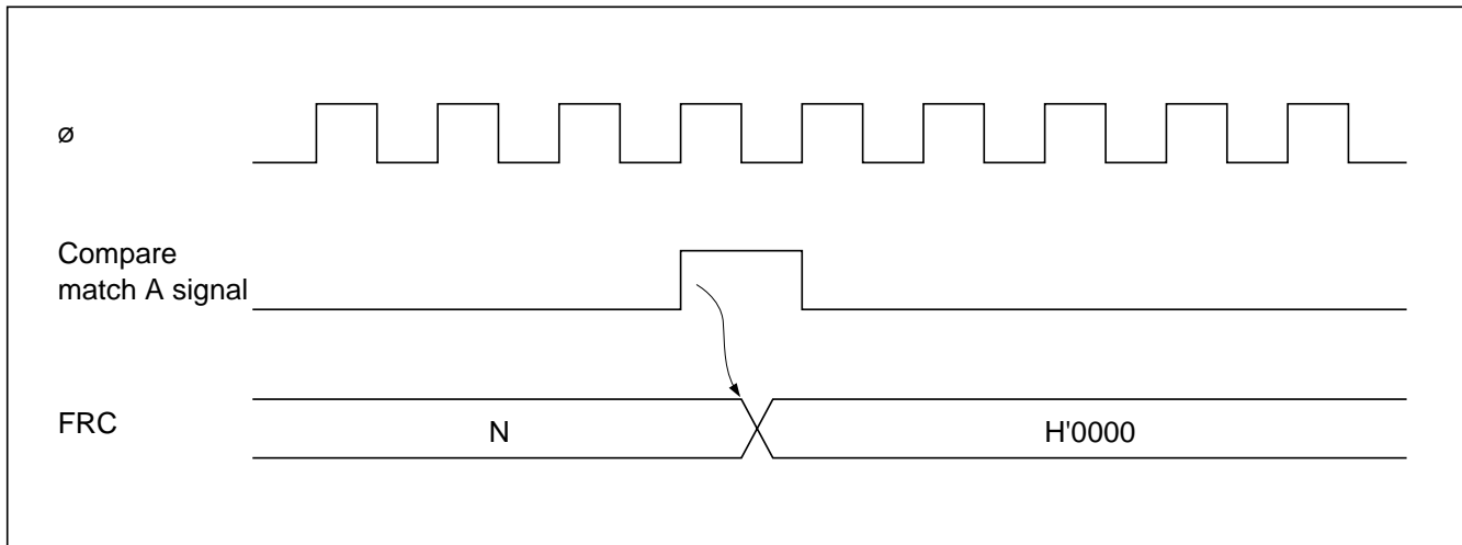
Figure 9-23 Clear Timing by Compare Match A
