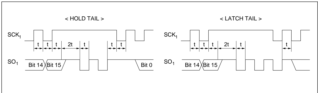
Figure 10-5 HOLD TAIL and LATCH TAIL Waveforms
