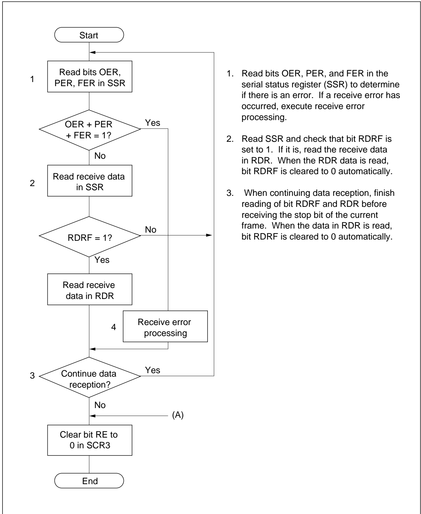
Figure 10-13 Example of Data Reception Flowchart (Asynchronous Mode)
