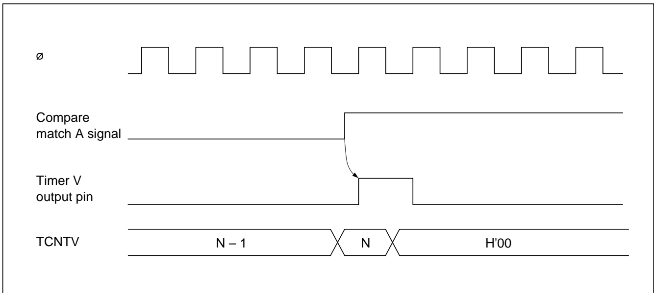
Figure 9-10 Clear Timing by TMRIV Input
