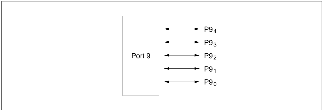
Figure 8-8 Port 9 Pin Configuration
