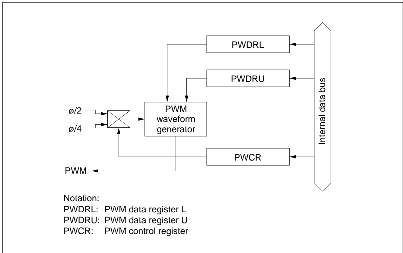
Figure 11-1 Block Diagram of the 14 bit PWM
