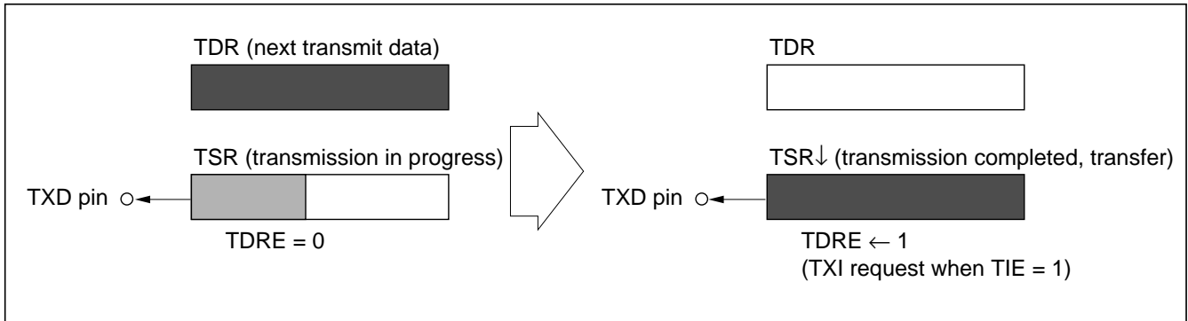
Figure 10-7 (b) TDRE Setting and TXI Interrupt
