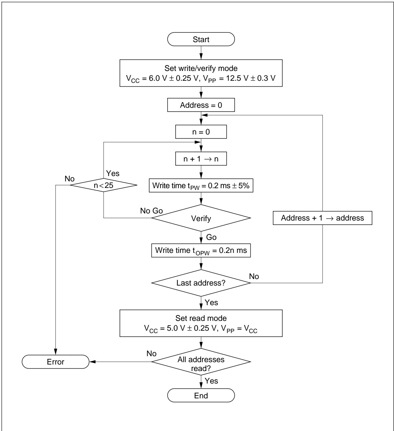
Figure 6-4 High-Speed, High-Reliability Programming Flow Chart
