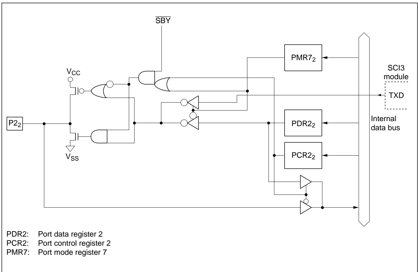
Figure C-2 (b) Port 2 Block Diagram (Pin P2 2 )
