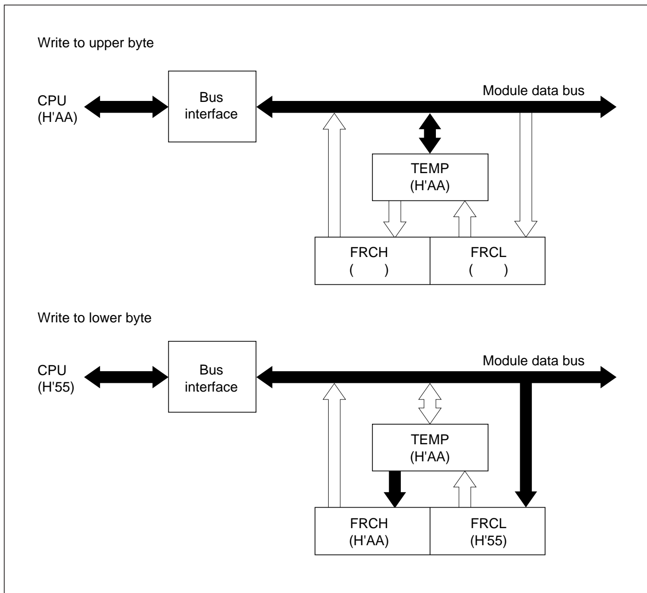
Figure 9-18 Write Access to FRC (CPU → FRC)
