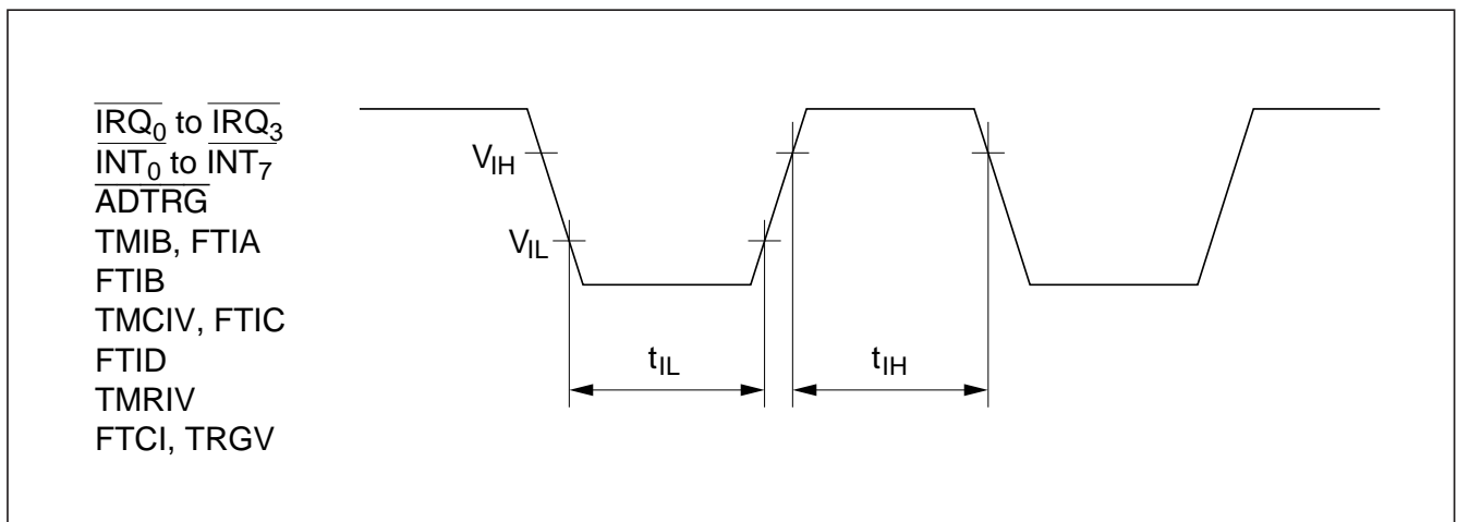
Figure 13-3 Input Timing
