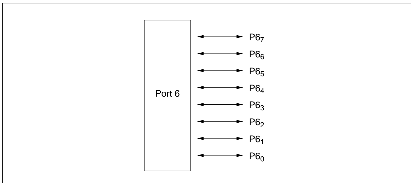
Figure 8-5 Port 6 Pin Configuration
