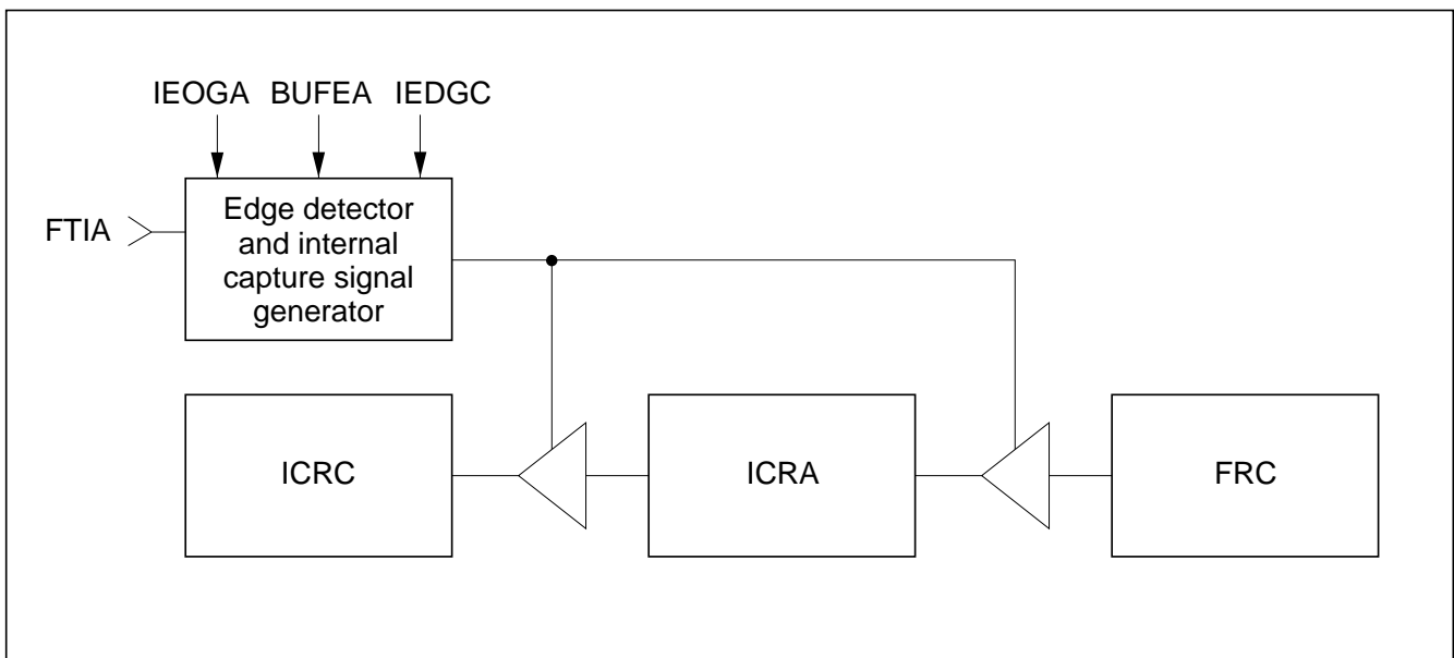
Figure 9-17 Buffer Operation (Example)
