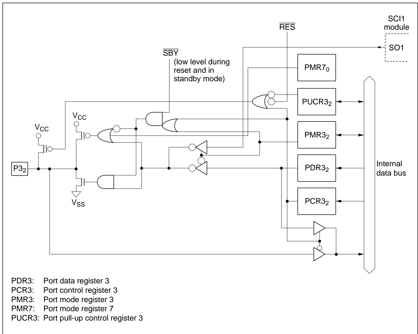
Figure C-3 (b) Port 3 Block Diagram (Pin P3 2 )
