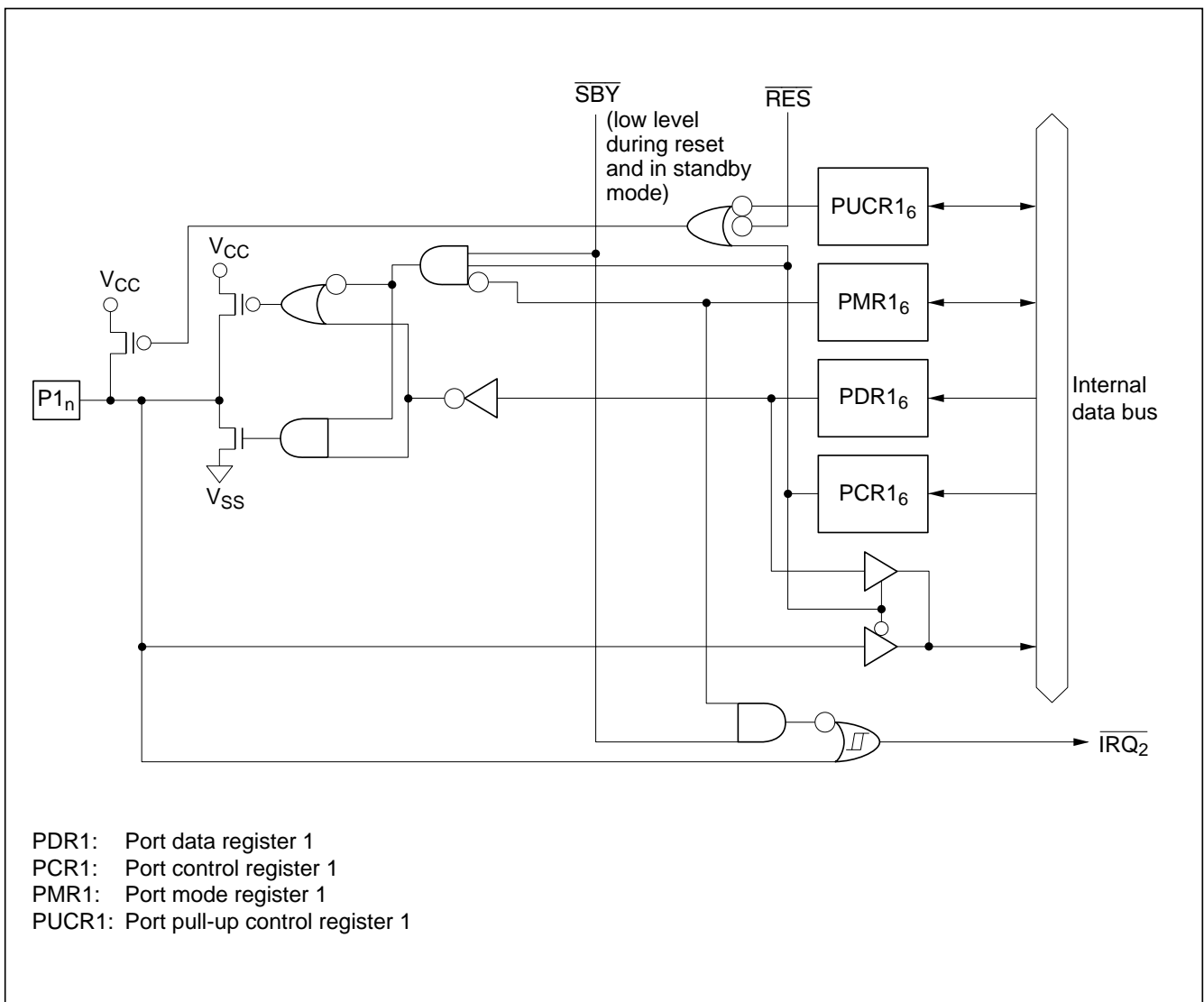
Figure C-1 (b) Port 1 Block Diagram (Pin P1 6 )
