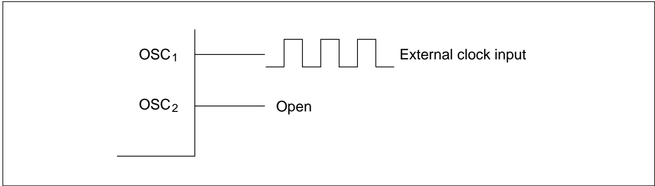
Figure 4-6 External Clock Input (Example)
