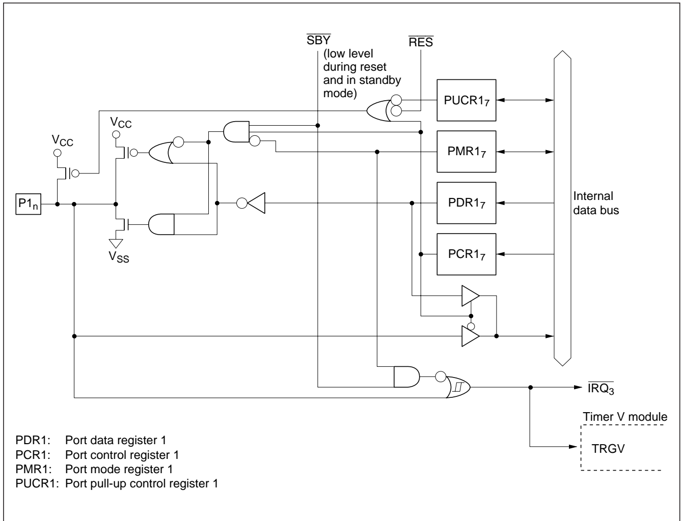
Figure C-1 (a) Port 1 Block Diagram (Pin P1 7 )
