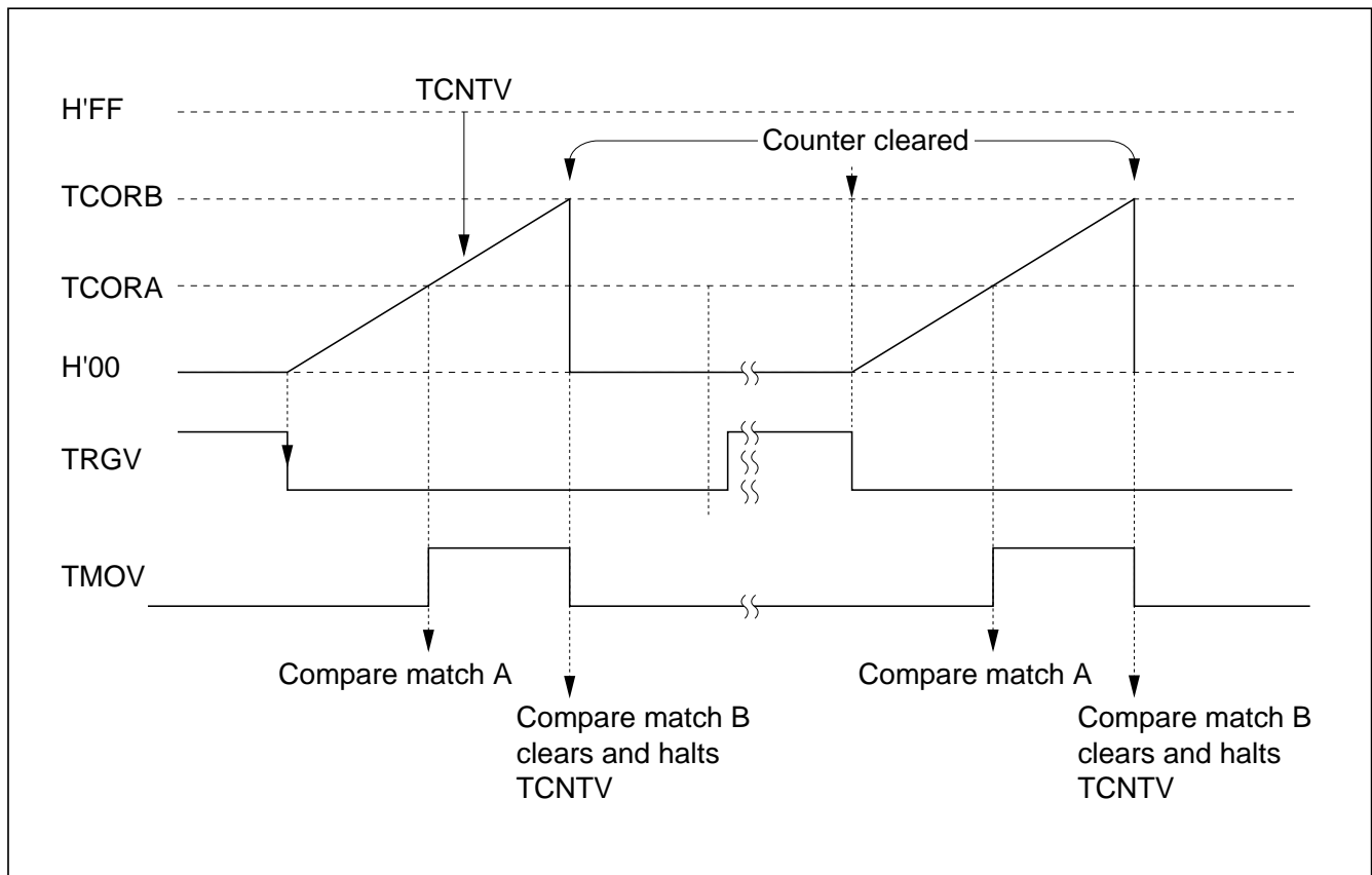
Figure 9-12 Pulse Output Synchronized to TRGV Input
