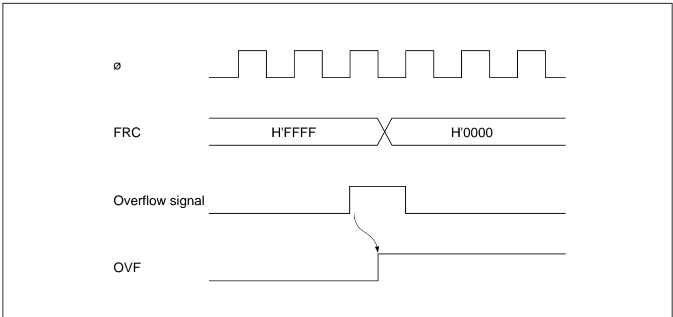
Figure 9-30 OVF Set Timing
