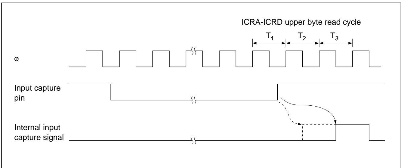
Figure 9-25 Input Capture Signal Timing (during ICRA-ICRD Read)
