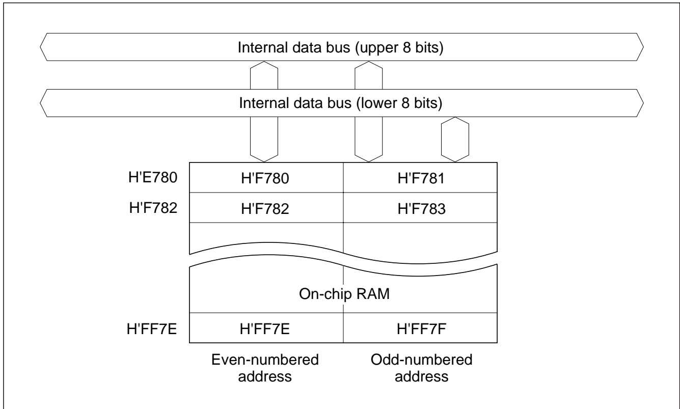
Figure 7-1 RAM Block Diagram (Example of 2 kbytes ROM)
