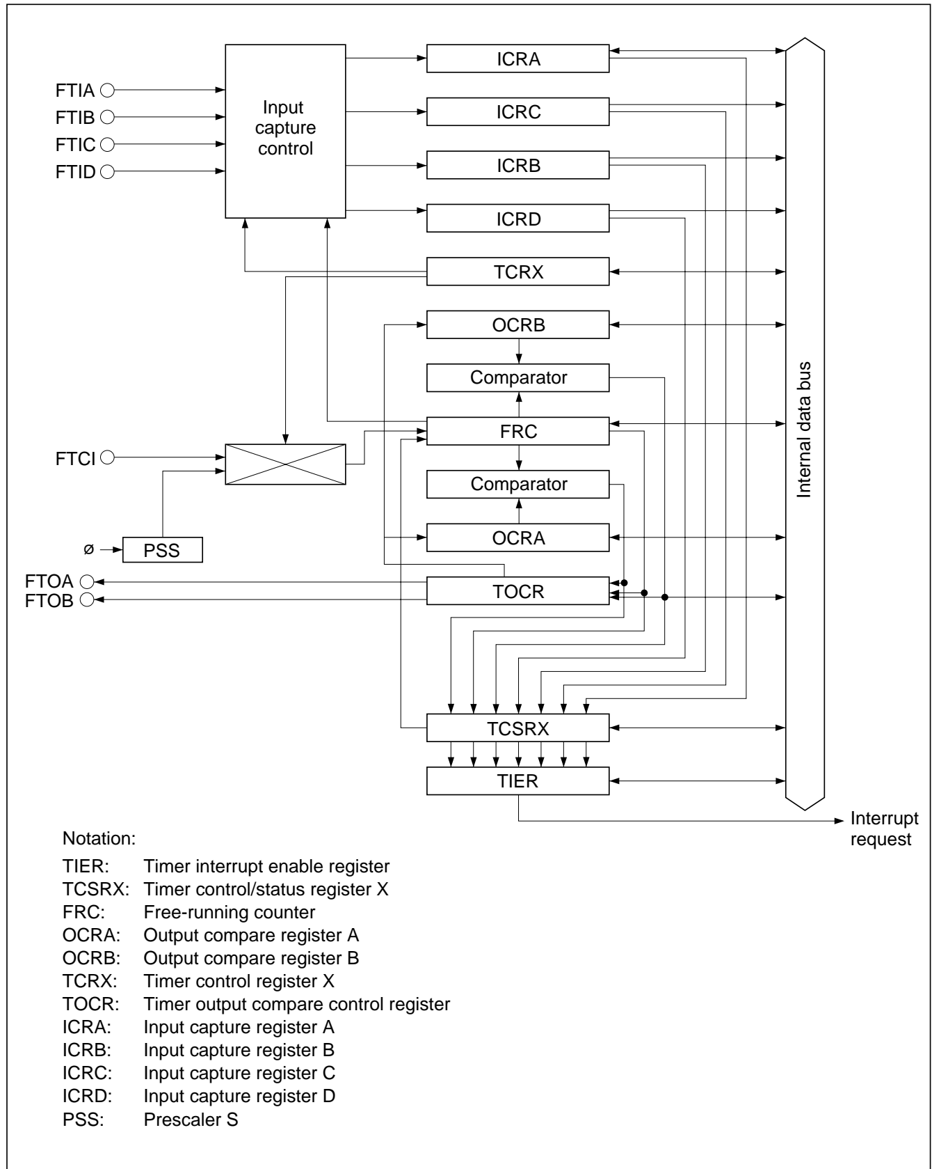
Figure 9-16 Block Diagram of Timer X
