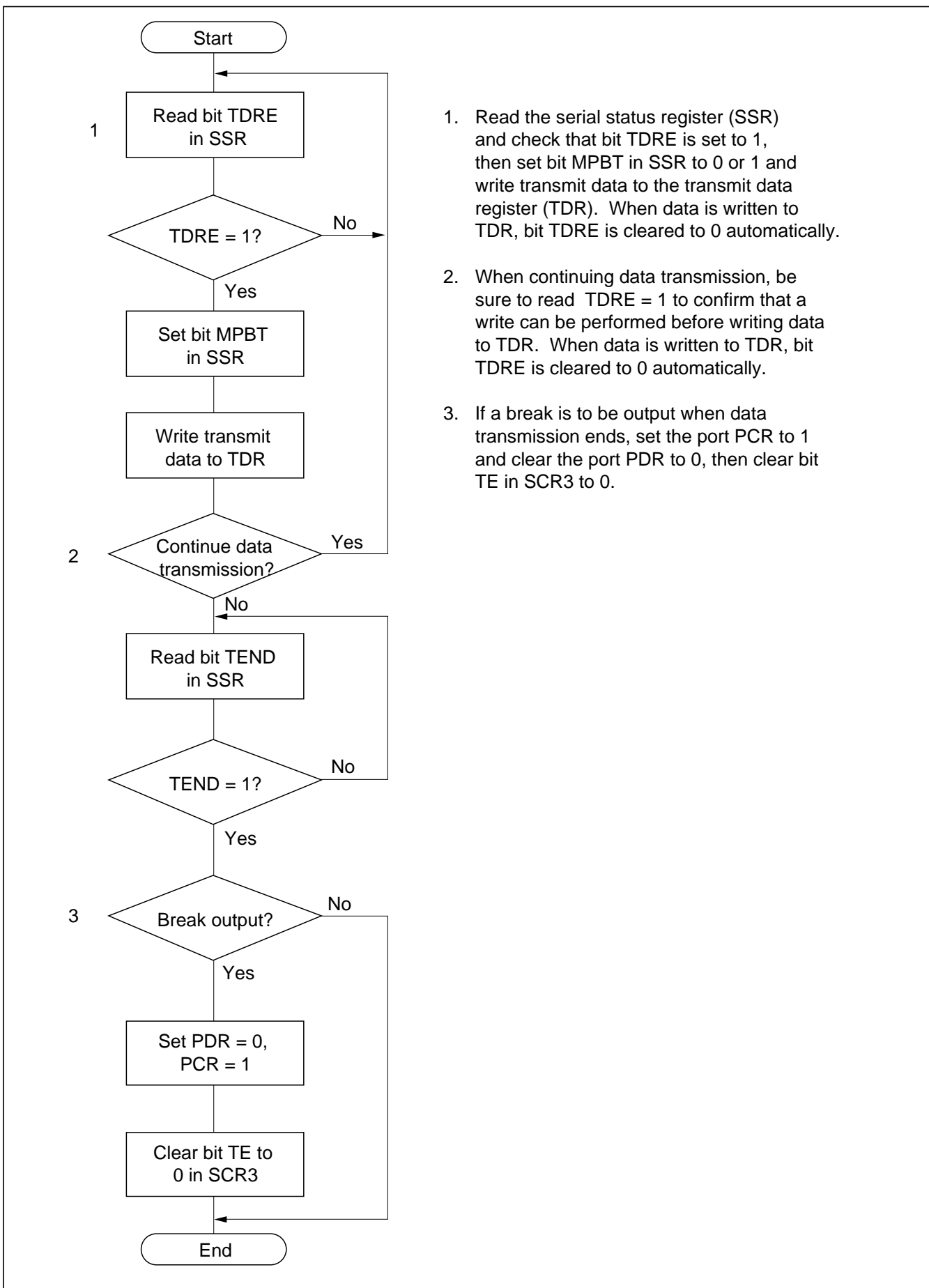
Figure 10-22 Example of Multiprocessor Data Transmission Flowchart
