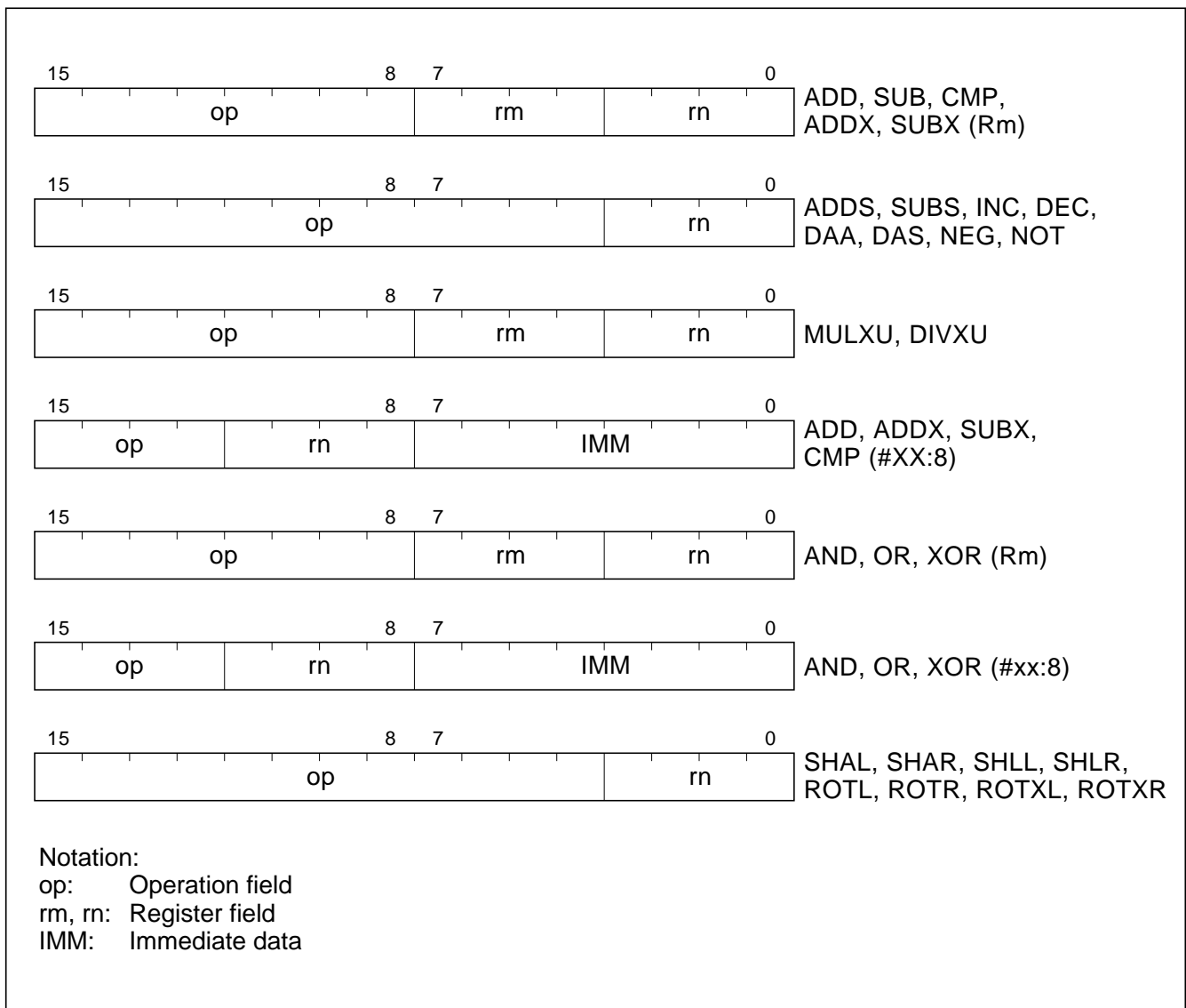
Figure 2-6 Arithmetic, Logic, and Shift Instruction Codes
