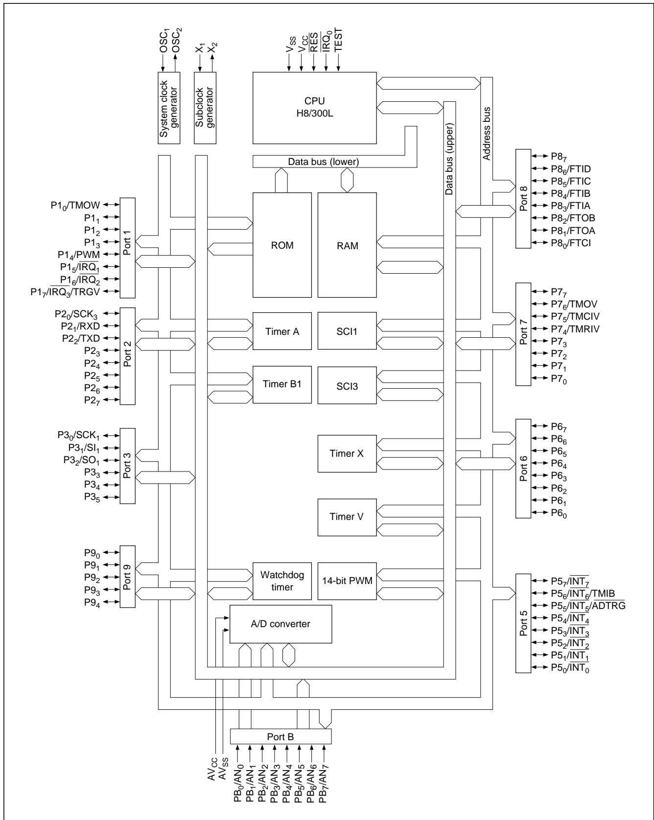
Figure 1-1 Block Diagram
