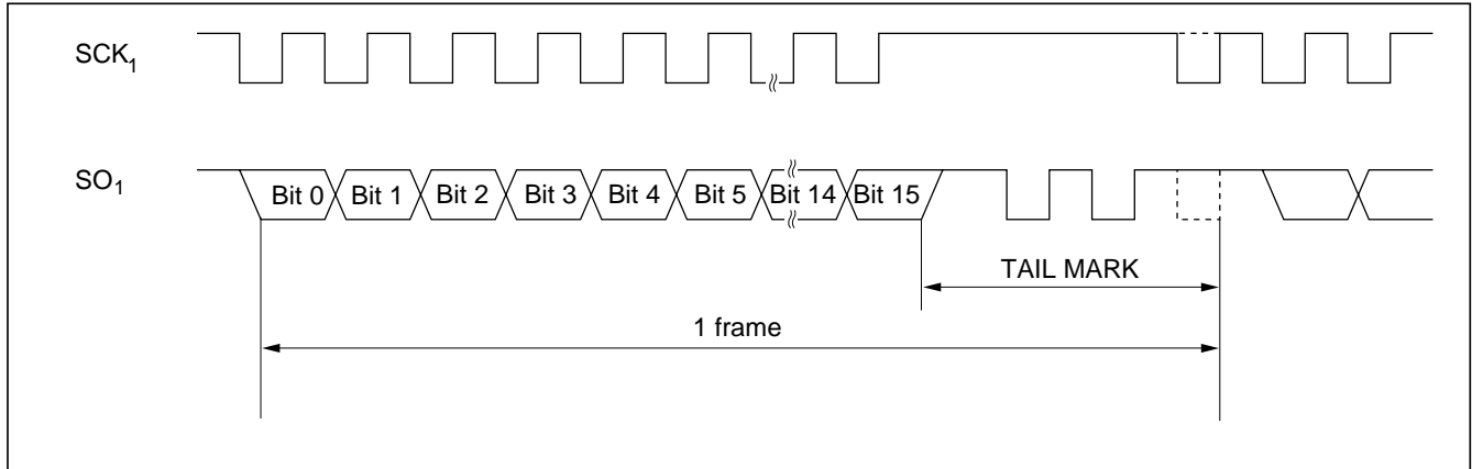
Figure 10-4 Transfer Format (When SNC1 = 0, SNC0 = 1, MRKON = 1)
