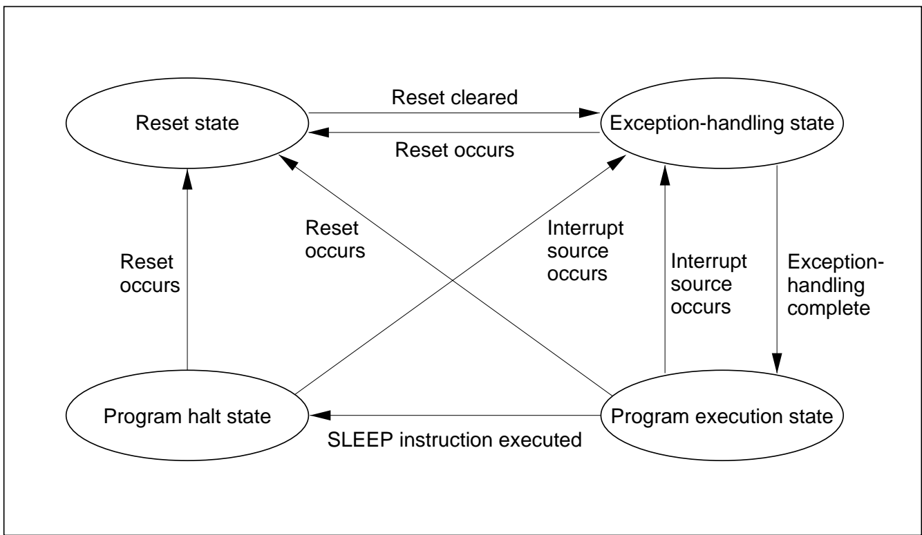
Figure 2-15 State Transitions
