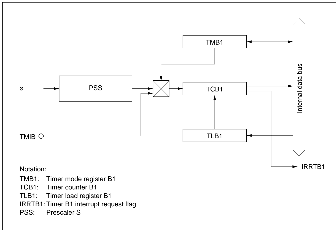
Figure 9-2 Block Diagram of Timer B1
