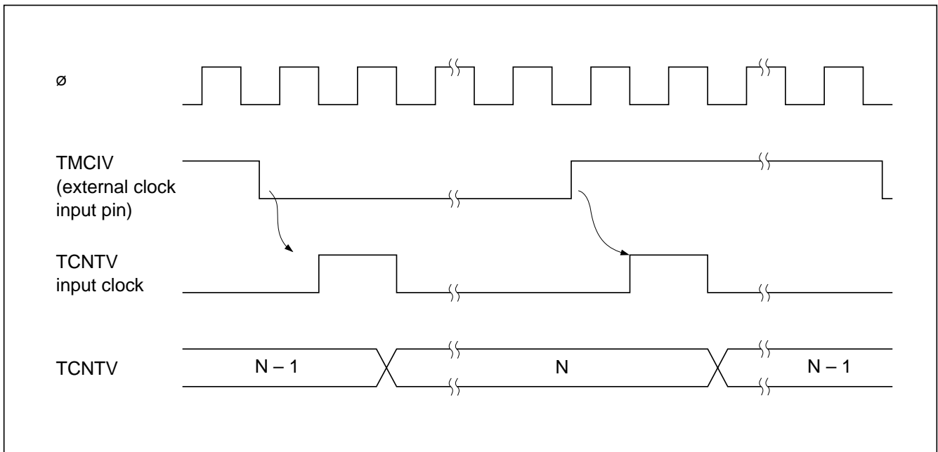
Figure 9-5 Increment Timing with External Clock
