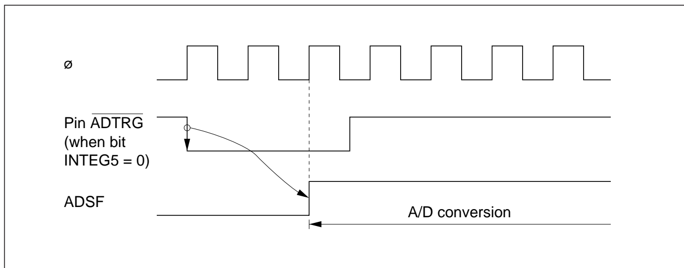
Figure 12-2 External Trigger Input Timing
