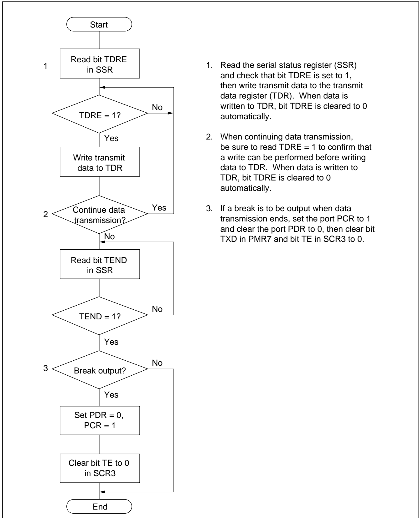
Figure 10-11 Example of Data Transmission Flowchart (Asynchronous Mode)
