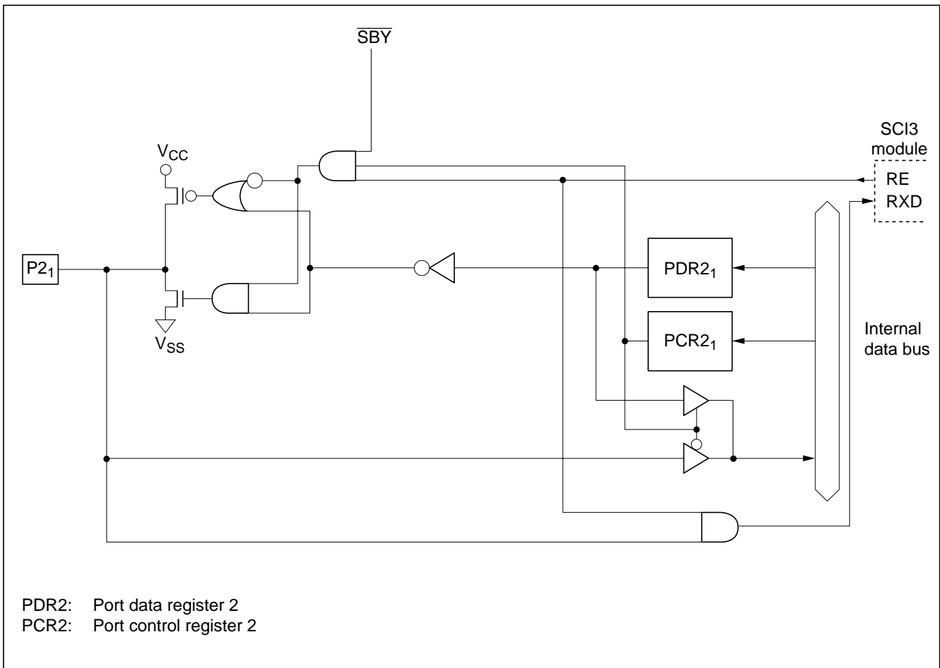
Figure C-2 (c) Port 2 Block Diagram (Pin P2 1 )
