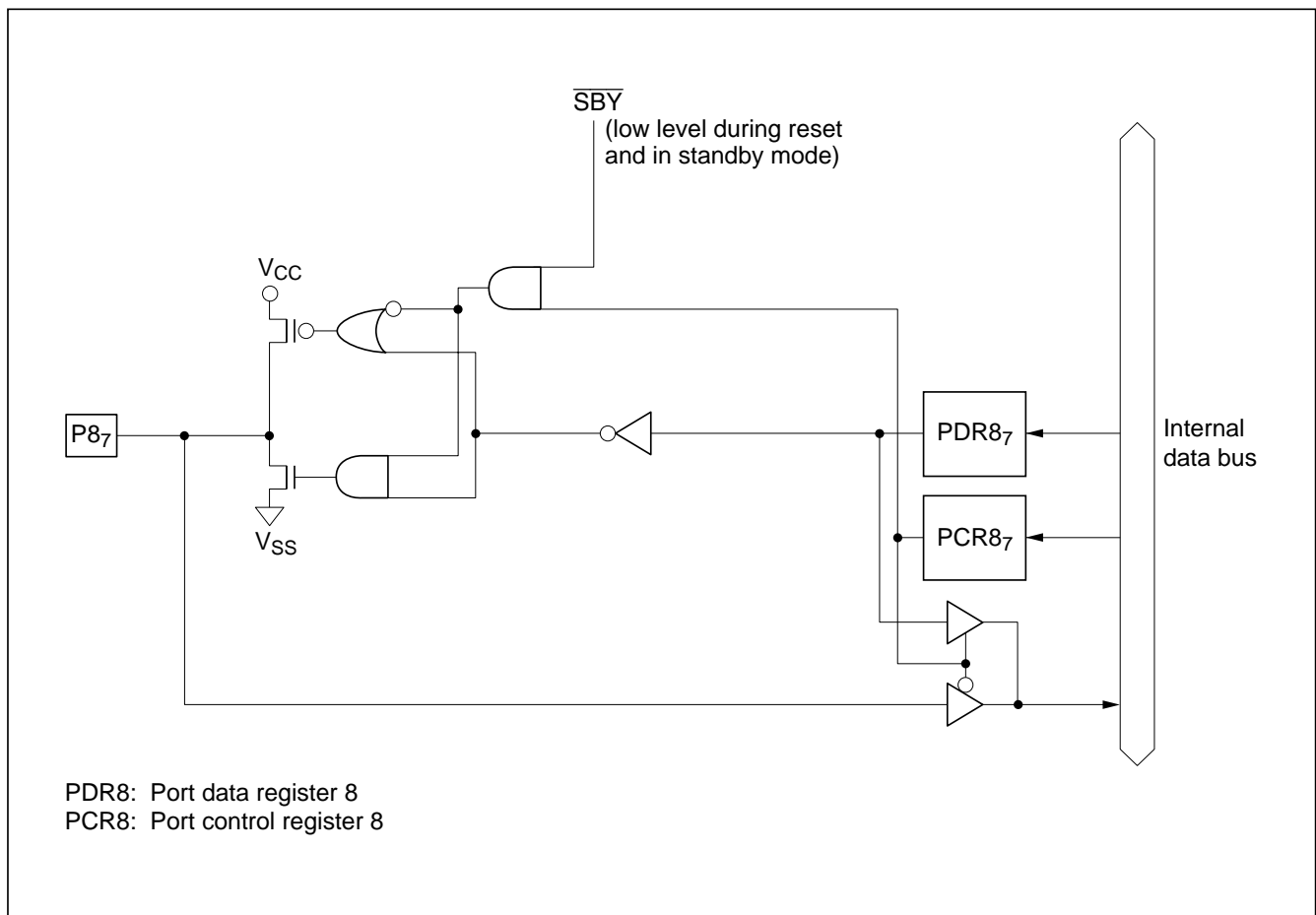
Figure C-7 (a) Port 8 Block Diagram (Pin P8 7 )
