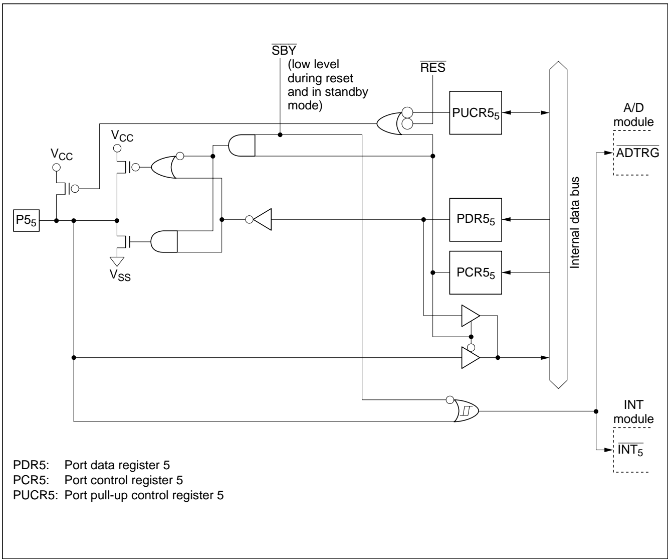
Figure C-4 (c) Port 5 Block Diagram (Pin P5 5 )
