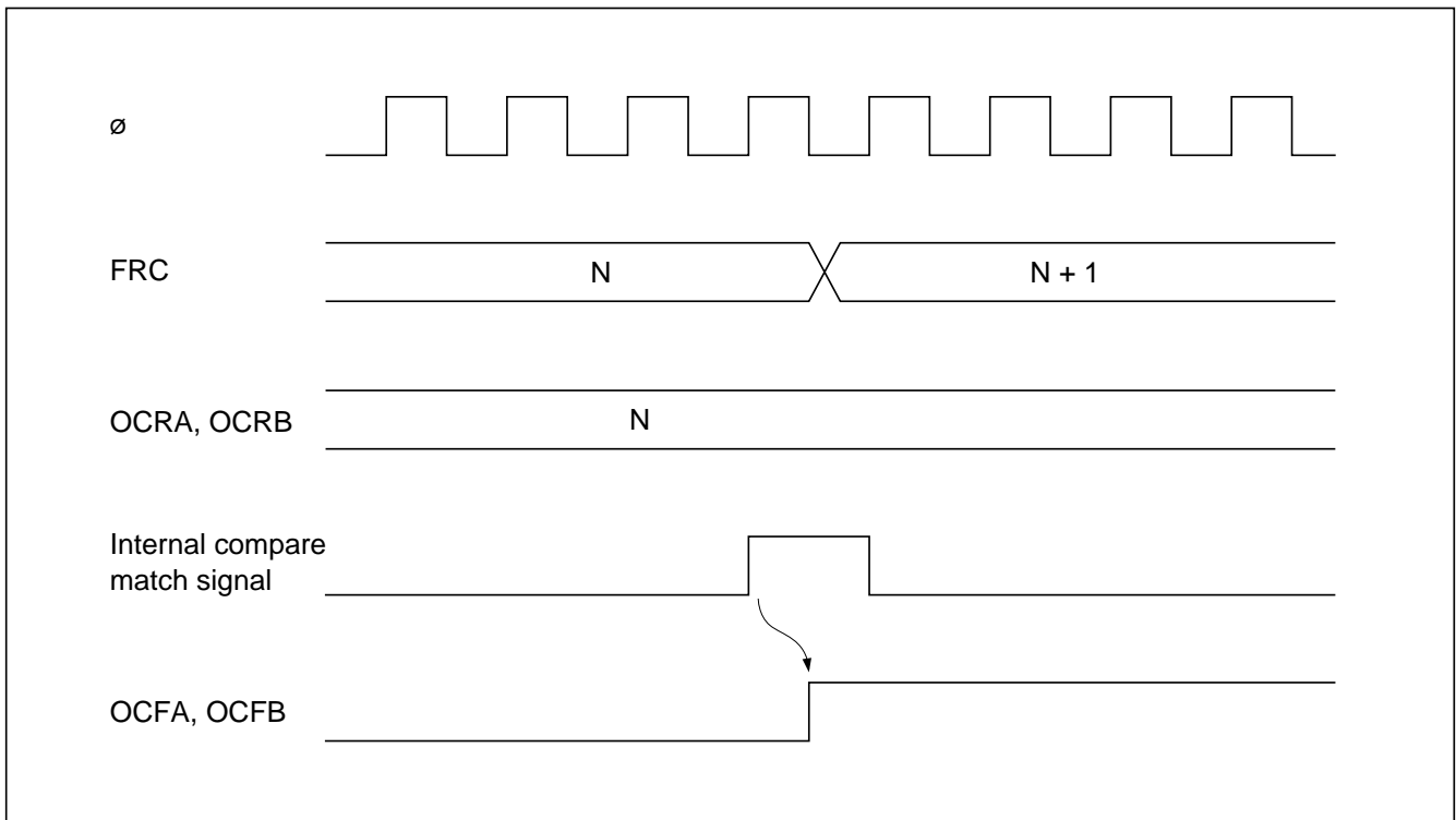
Figure 9-29 OCFA and OCFB Set Timing
