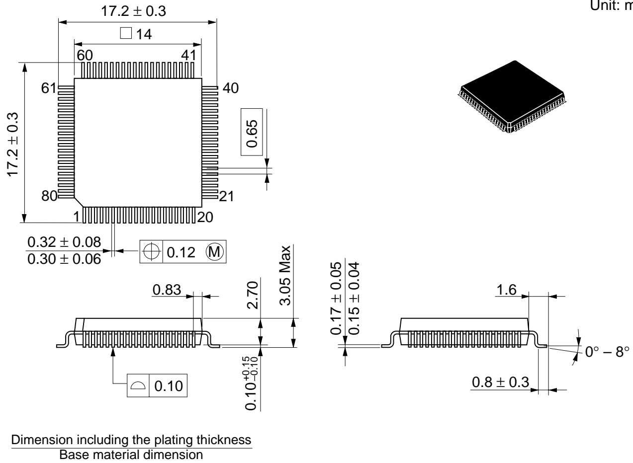
Figure F-3 FP-80A Package Dimensions
