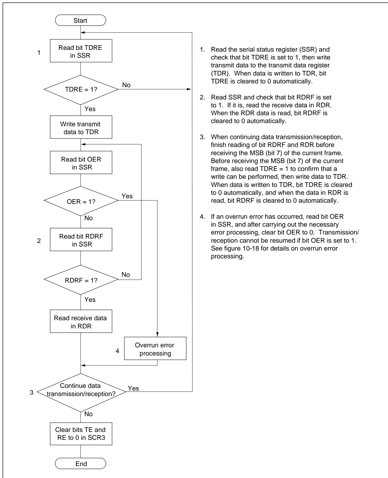
Figure 10-20 Example of Simultaneous Data Transmission/Reception Flowchart(Synchronous Mode)
