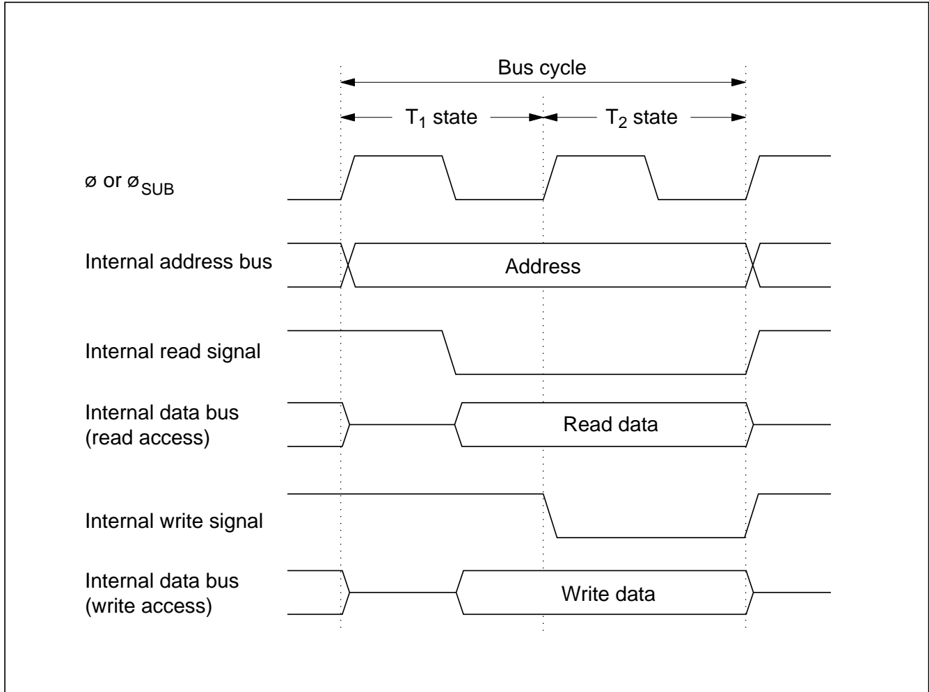
Figure 2-12 On-Chip Peripheral Module Access Cycle (2-State Access)
