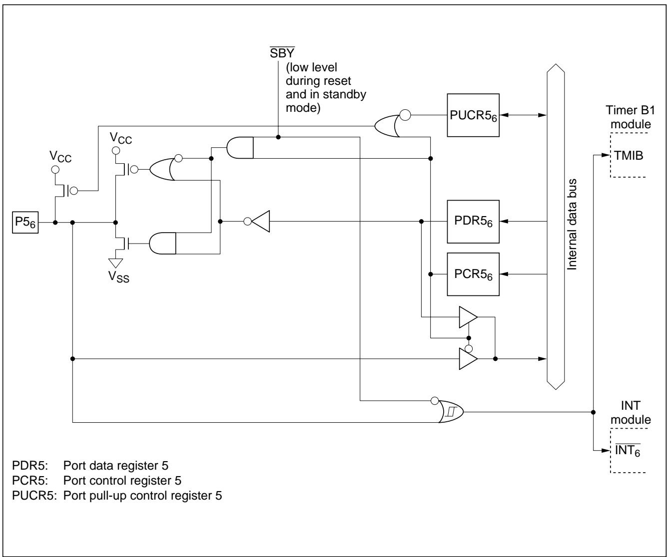
Figure C-4 (b) Port 5 Block Diagram (Pin P5 6 )
