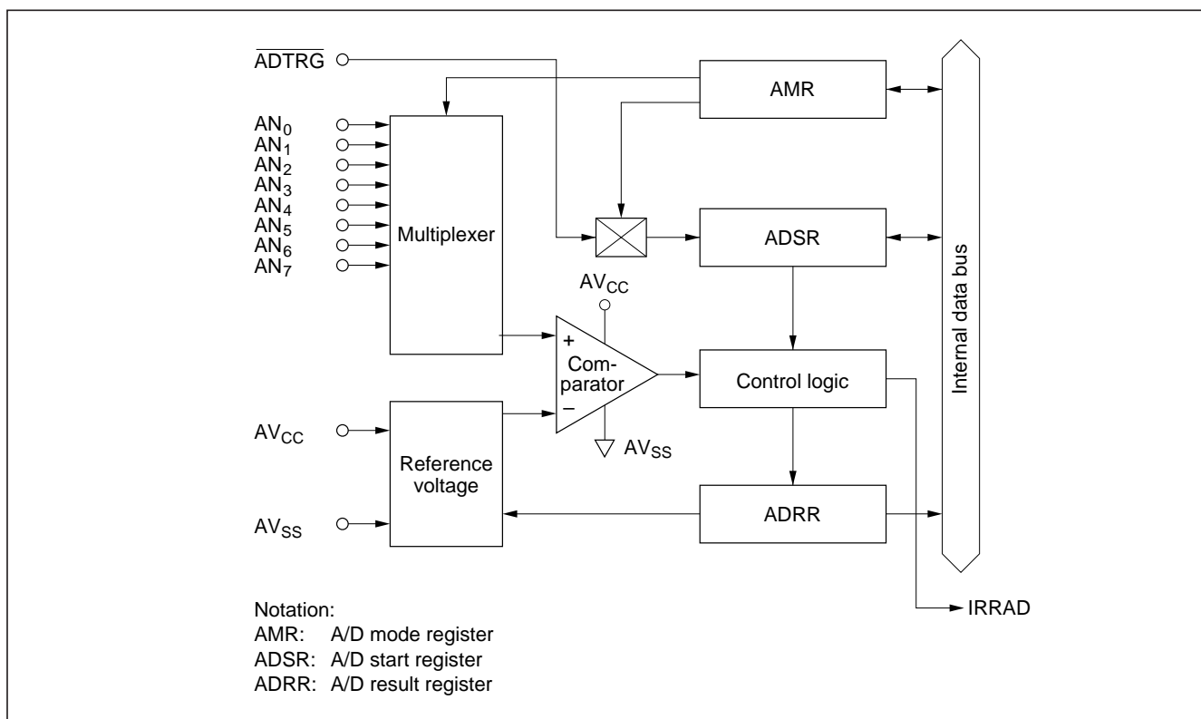
Figure 12-1 Block Diagram of the A/D Converter
