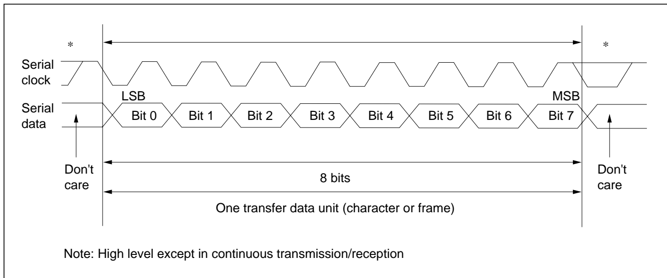
Figure 10-15 Data Format in Synchronous Communication
