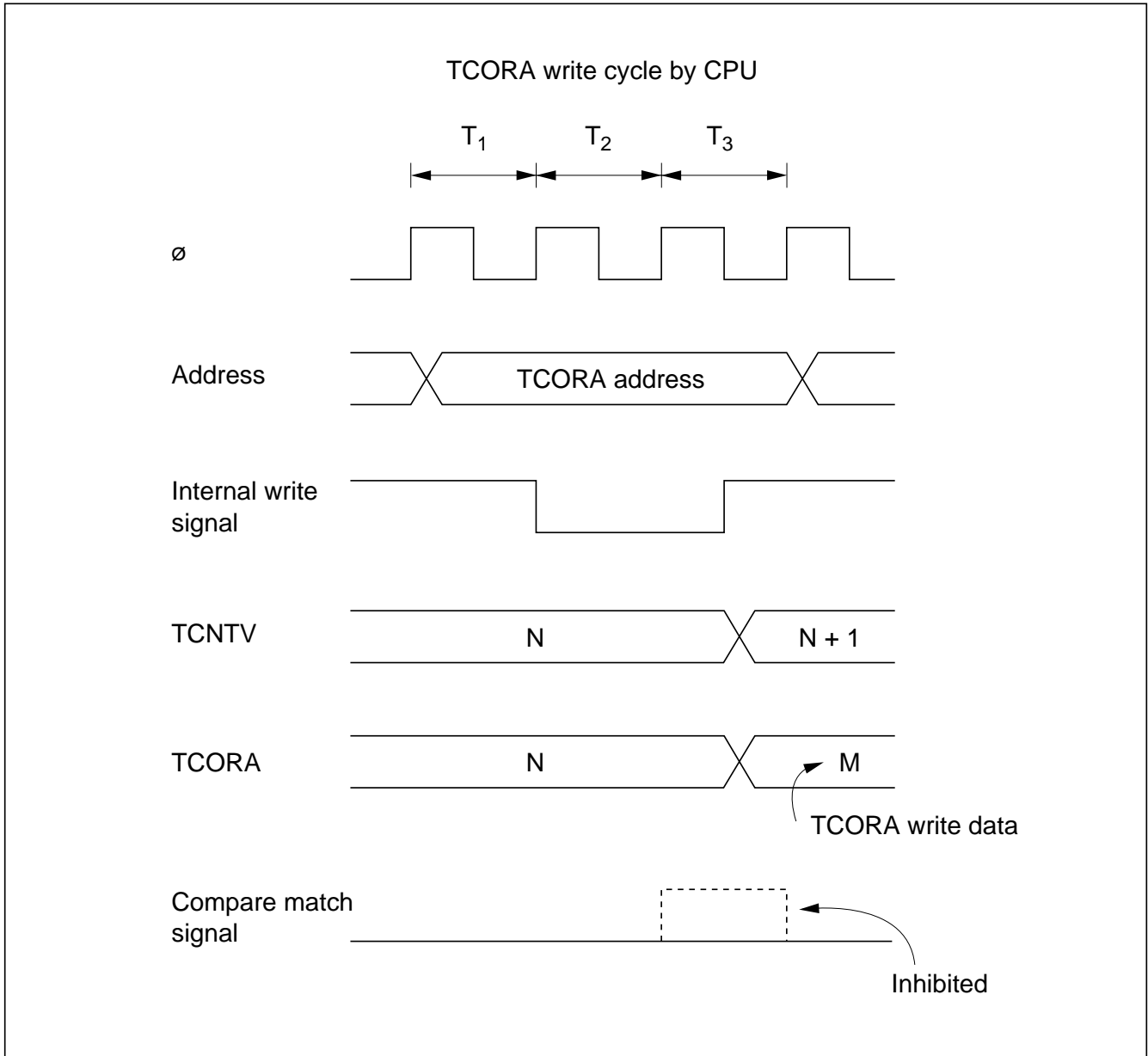
Figure 9-15 Contention between TCORA Write and Compare Match
