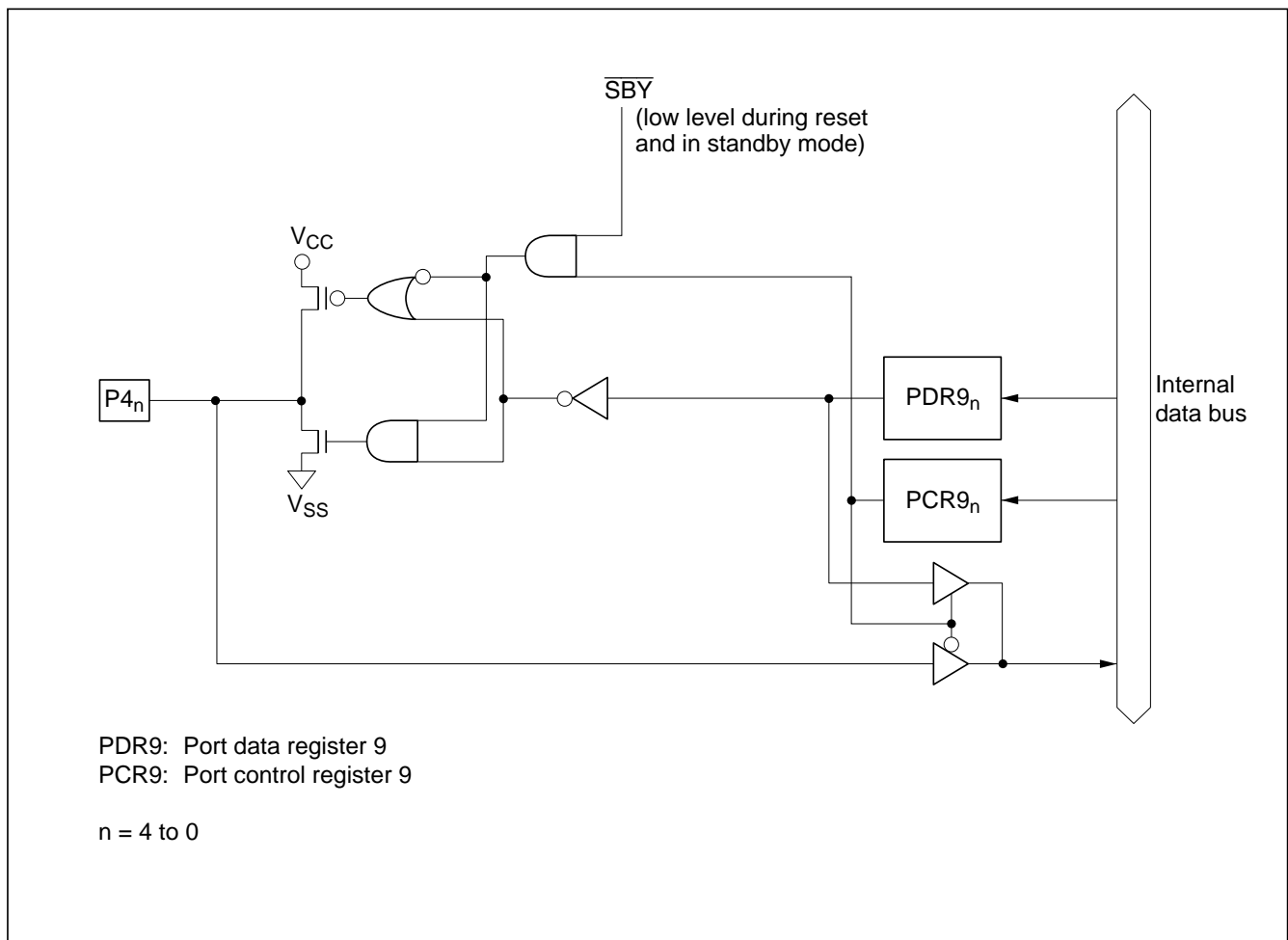
Figure C-8 Port 9 Block Diagram (Pins P9 4 to P9 0 )
