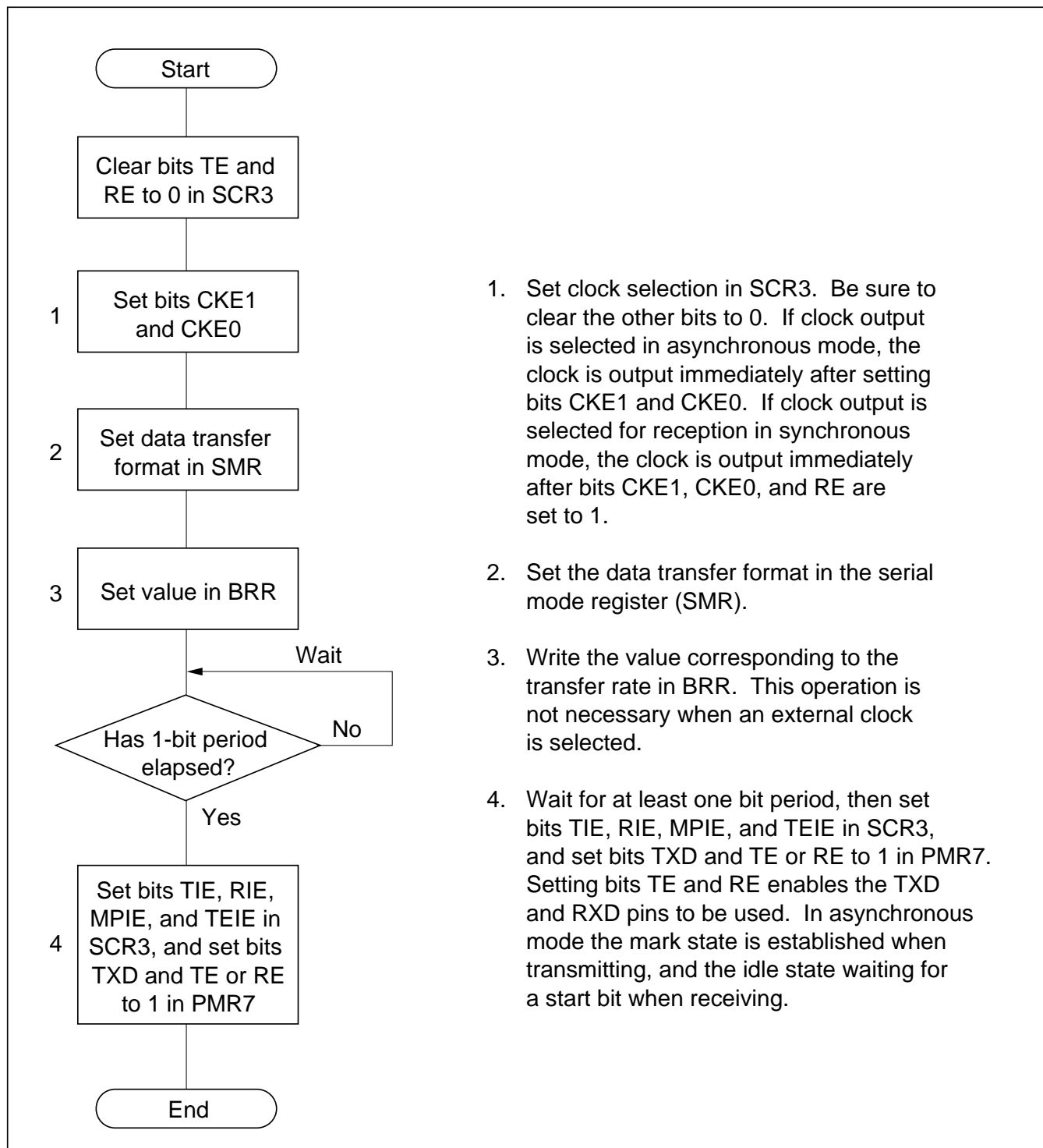
Figure 10-10 Example of SCI3 Initialization Flowchart
