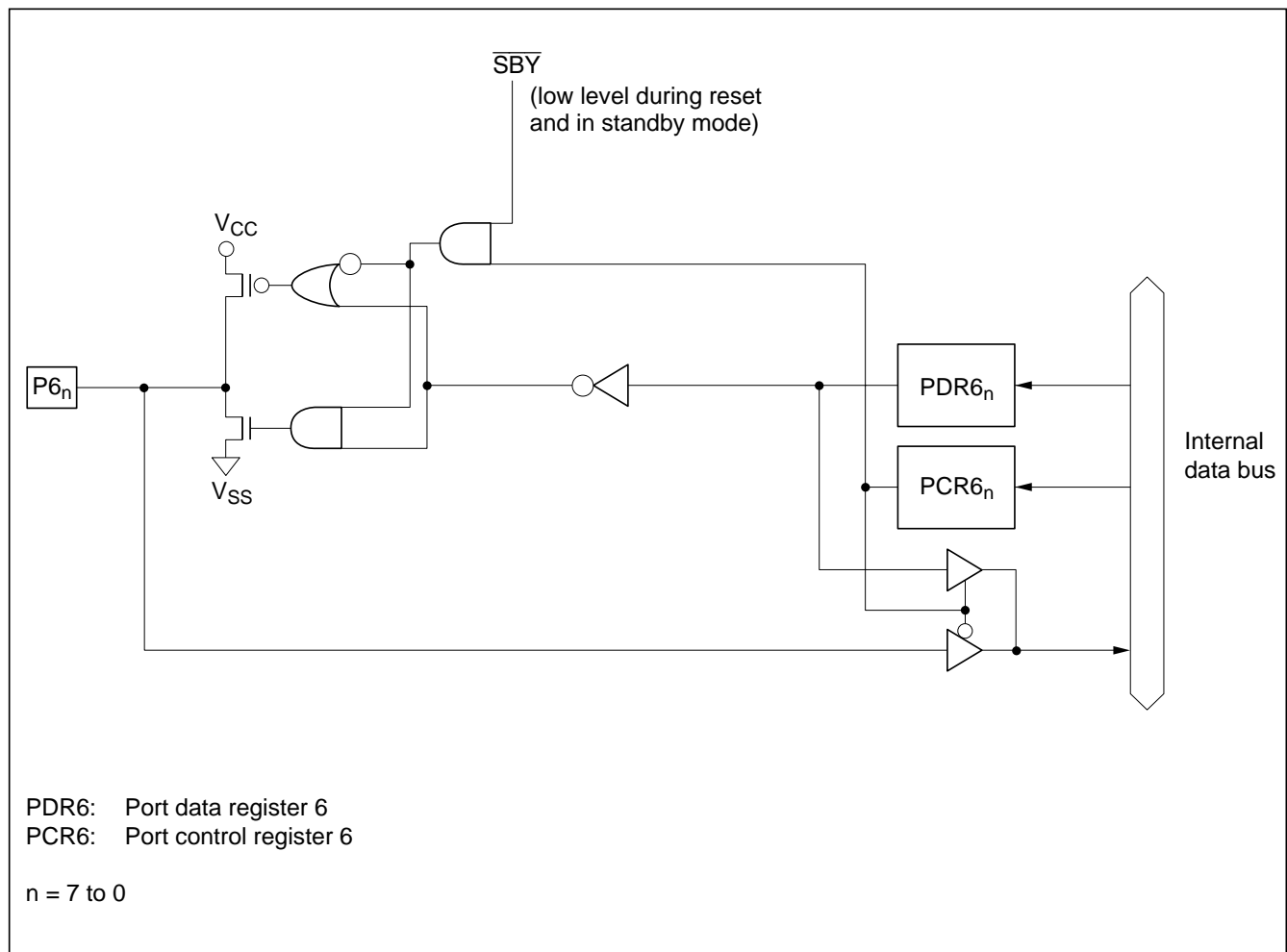
Figure C-5 Port 6 Block Diagram (Pins P6_7 to P6_0 )
