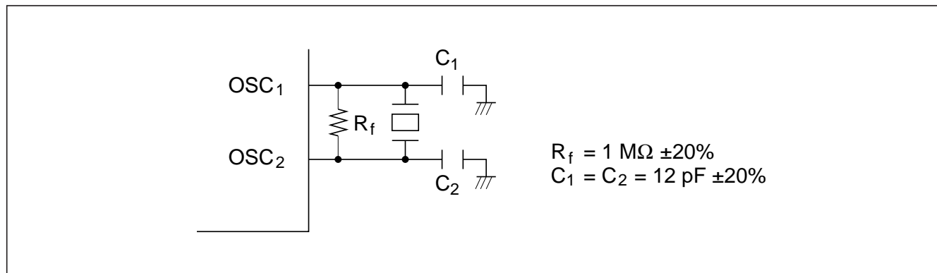
Figure 4-2 Typical Connection to Crystal Oscillator
