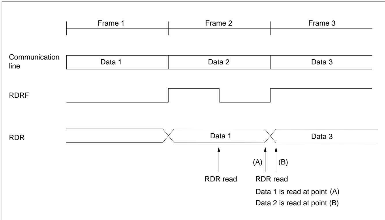
Figure 10-27 Relation between RDR Read Timing and Data
