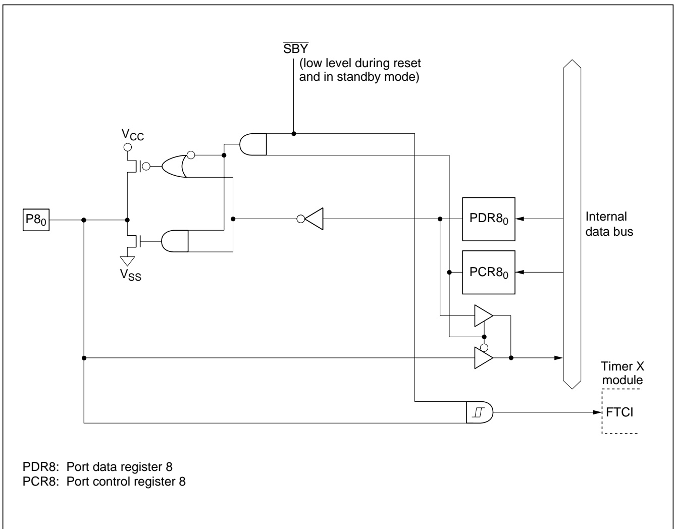
Figure C-7 (h) Port 8 Block Diagram (Pin P8 0 )
