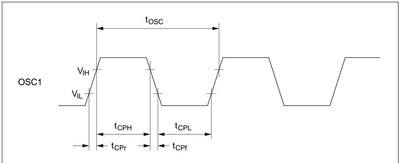
Figure 13-1 System Clock Input Timing
