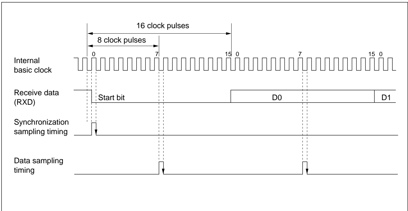
Figure 10-26 Receive Data Sampling Timing in Asynchronous Mode
