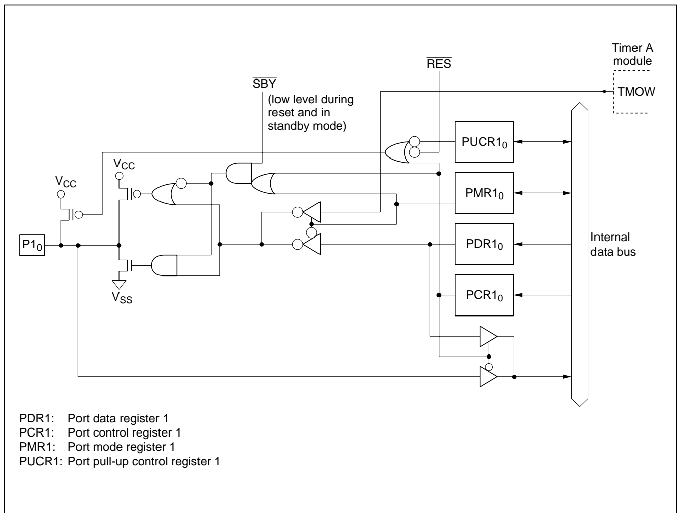
Figure C-1 (f) Port 1 Block Diagram (Pin P1 0 )
