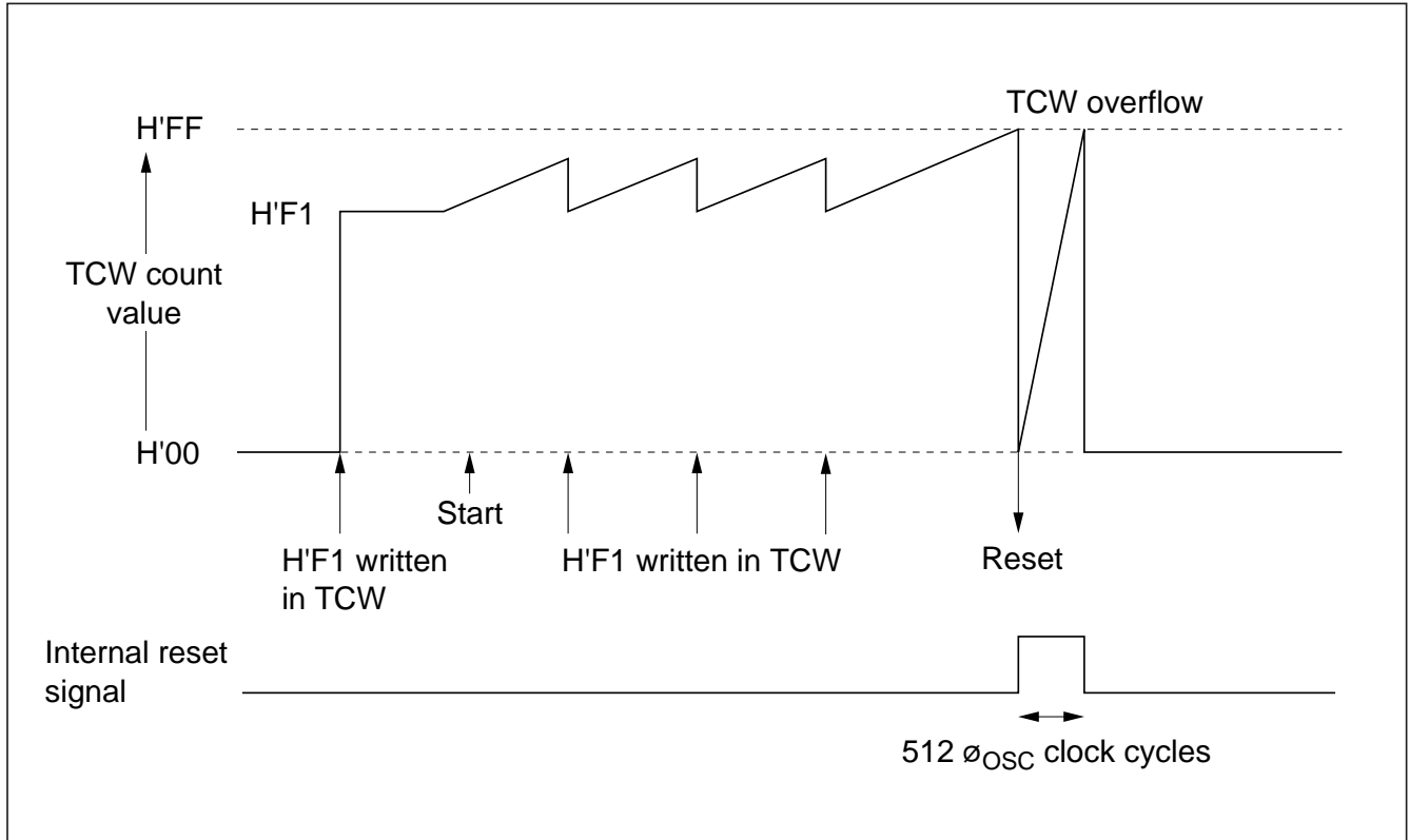
Figure 9-36 Typical Watchdog Timer Operations (Example)
