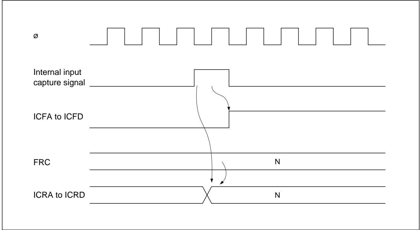
Figure 9-28 ICFA to ICFD Set Timing
