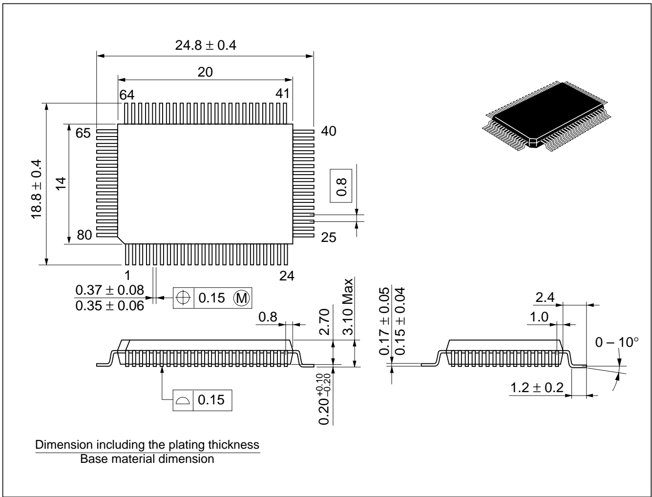
Figure F-4 FP-80B Package Dimensions
