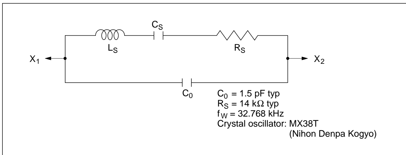
Figure 4-8 Equivalent Circuit of 32.768-kHz Crystal Oscillator
