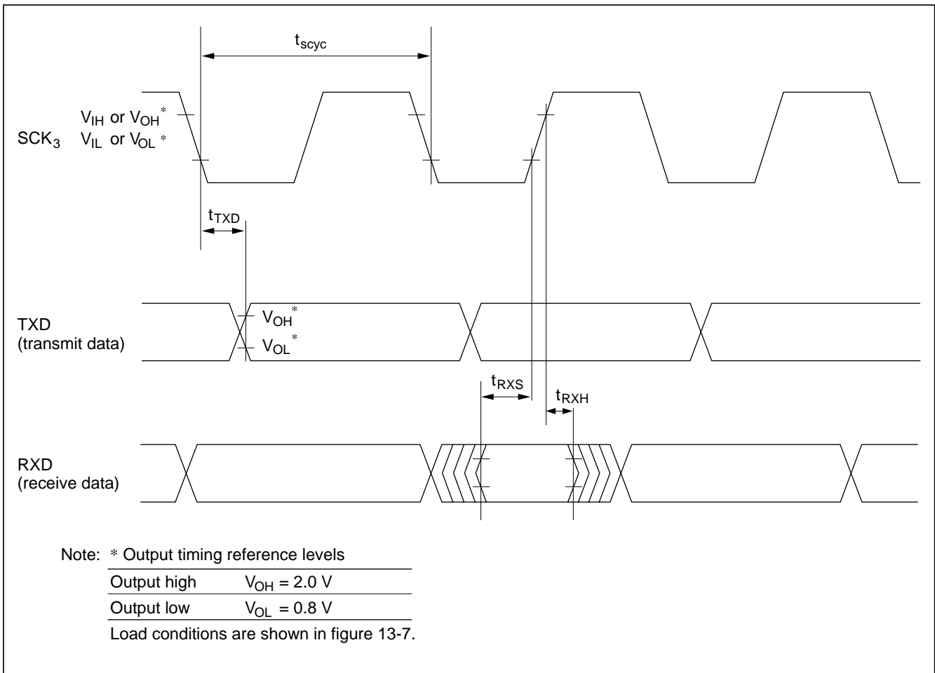
Figure 13-6 Serial Interface 3 Synchronous Mode Input Output Timing
