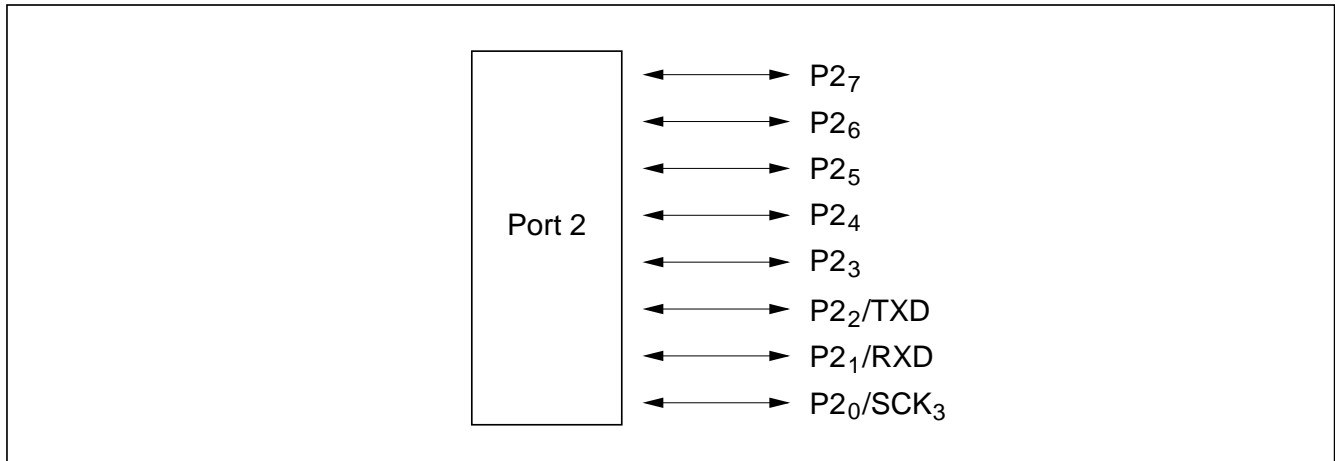
Figure 8-2 Port 2 Pin Configuration
