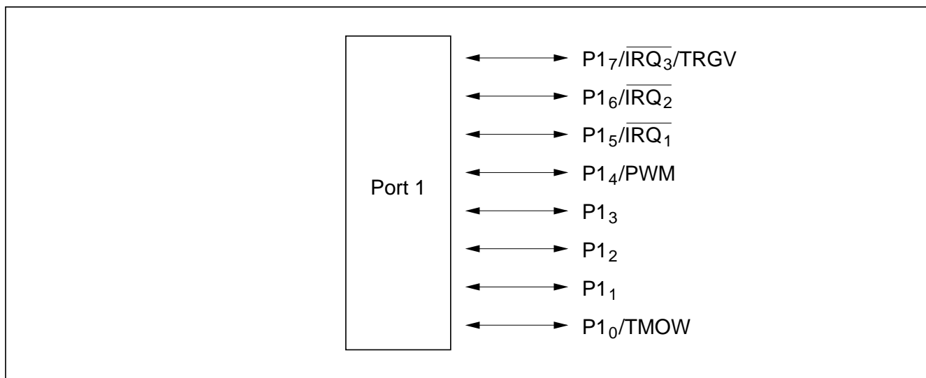
Figure 8-1 Port 1 Pin Configuration
