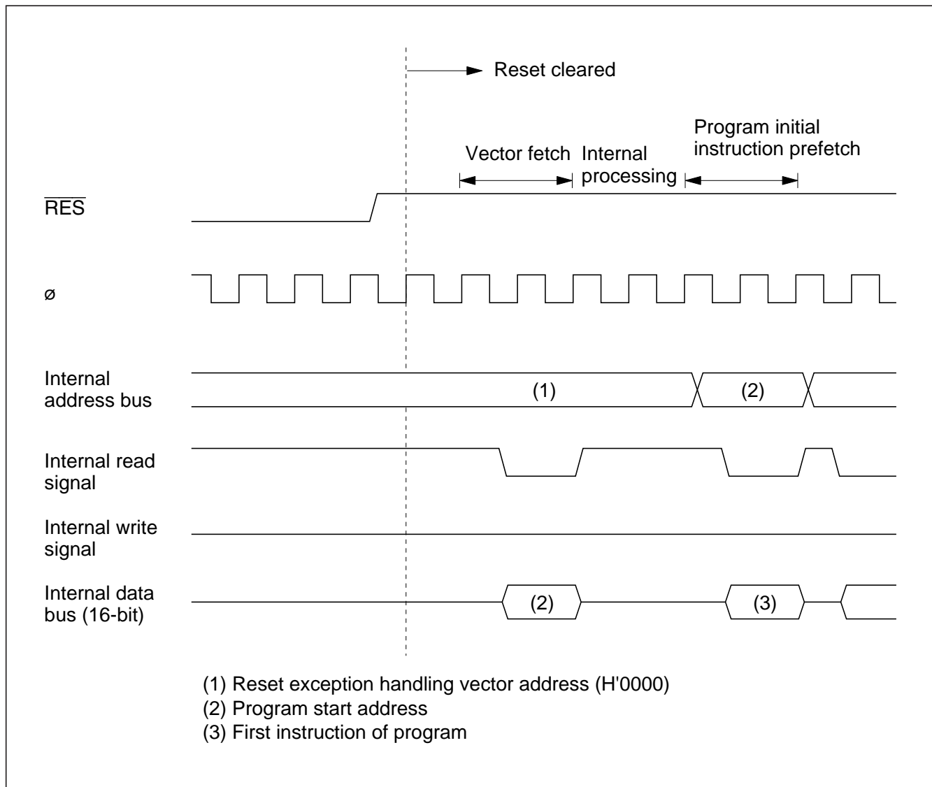
Figure 3-1 Reset Sequence
