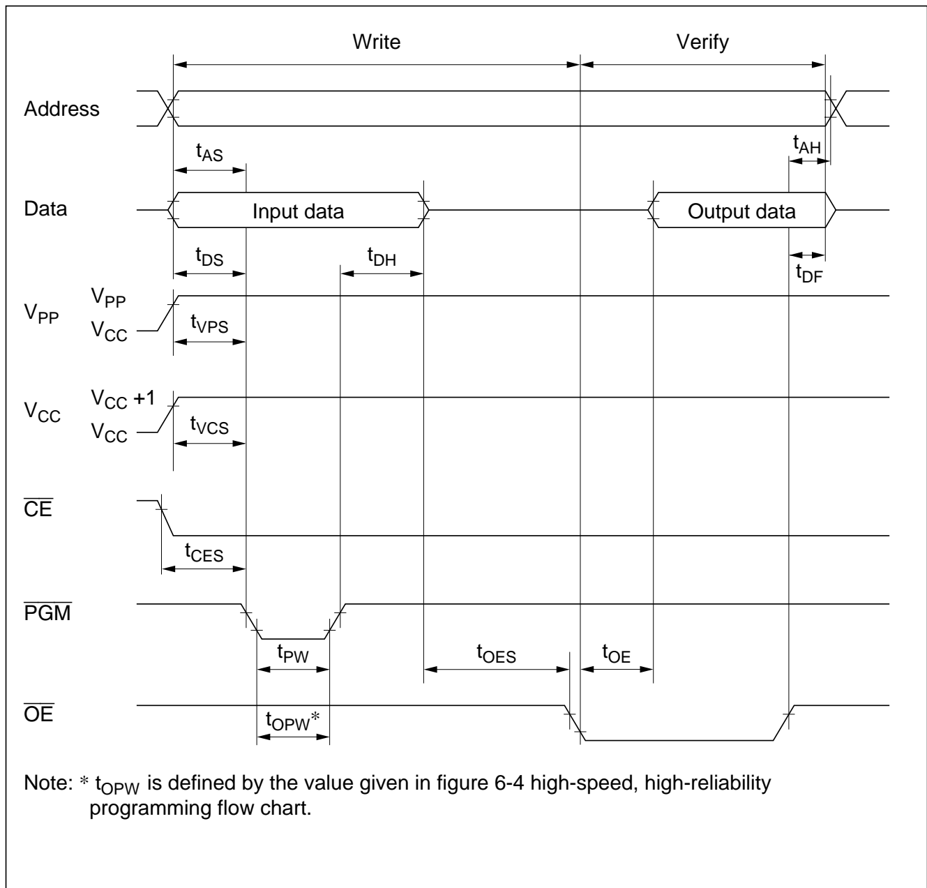
Figure 6-5 PROM Write/Verify Timing
