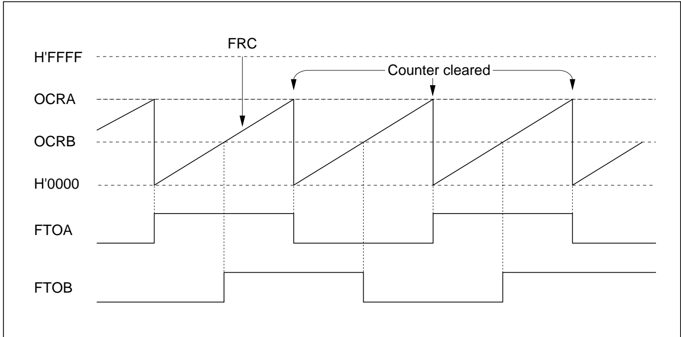
Figure 9-31 Pulse Output Example
