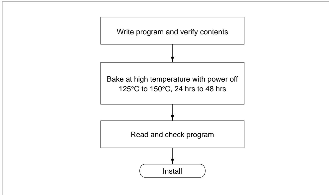
Figure 6-6 Recommended Screening Procedure
