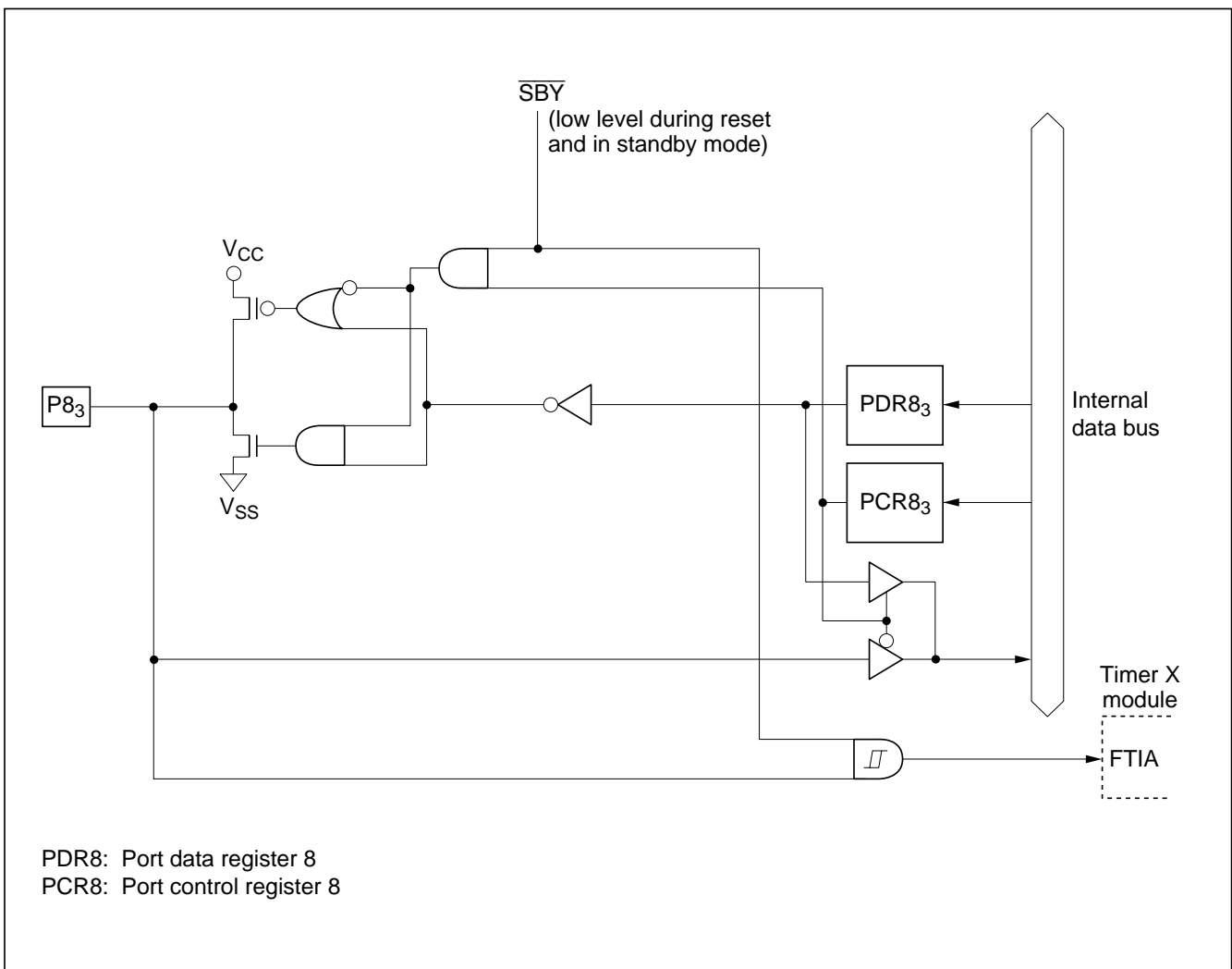
Figure C-7 (e) Port 8 Block Diagram (Pin P8 3 )
