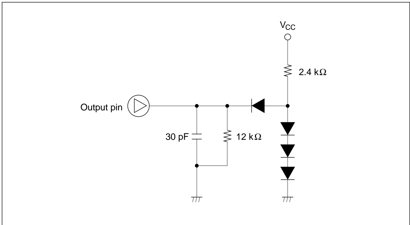
Figure 13-7 Output Load Condition
