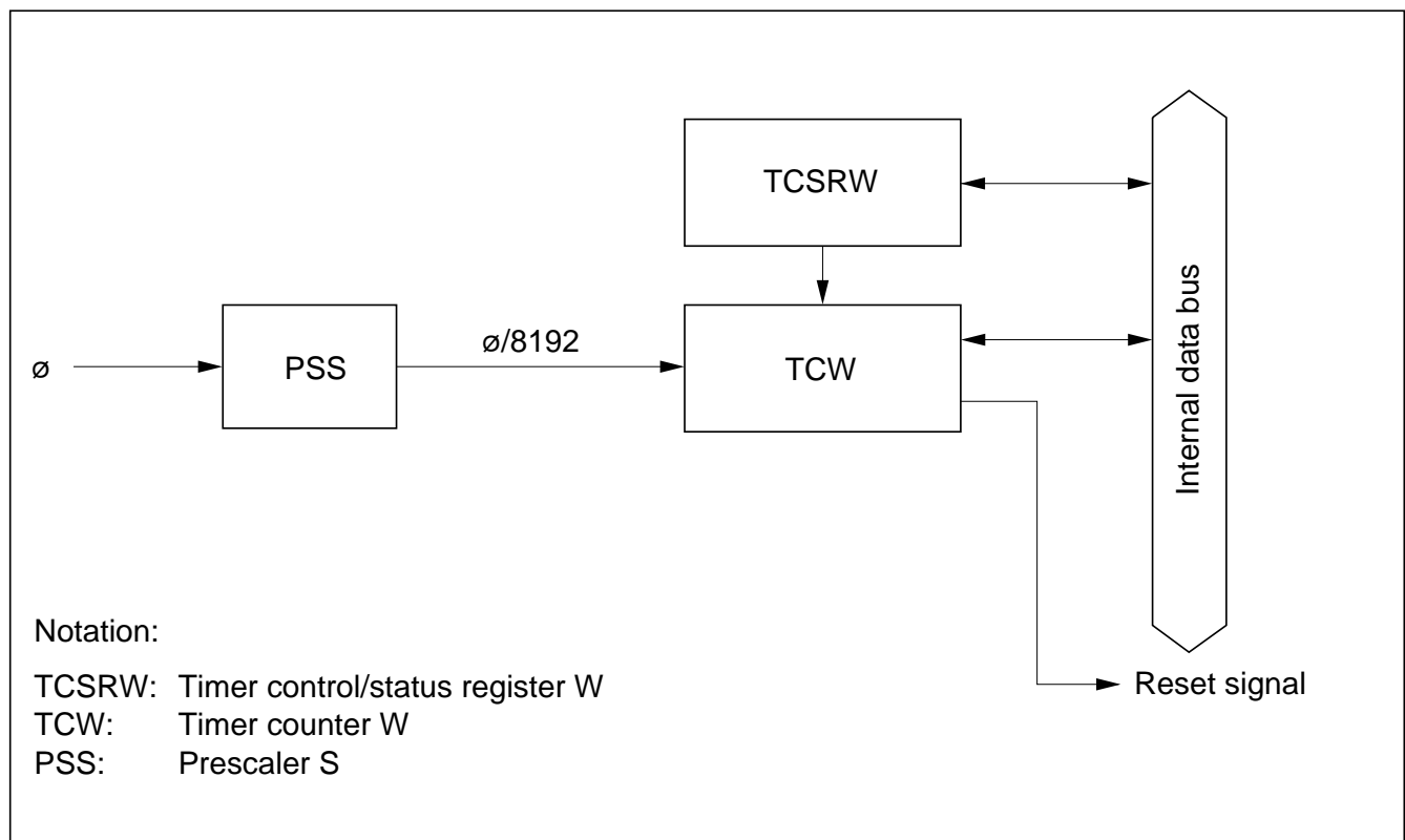
Figure 9-35 Block Diagram of Watchdog Timer
