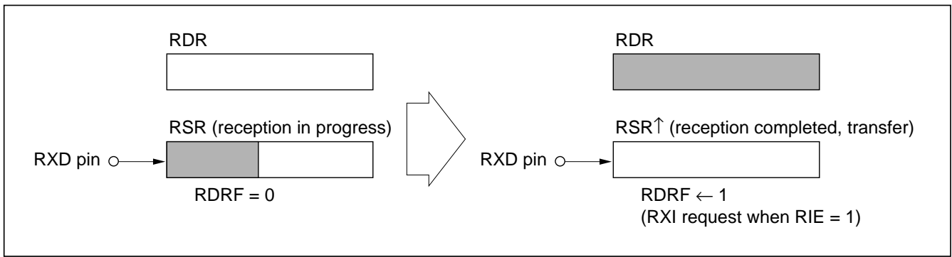
Figure 10-7 (a) RDRF Setting and RXI Interrupt
