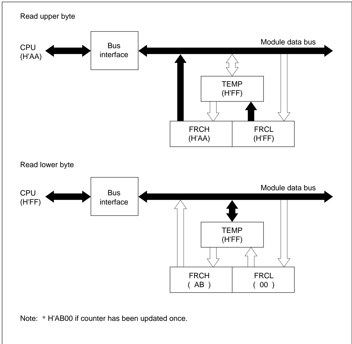
Figure 9-19 Read Access to FRC (FRC → CPU)
