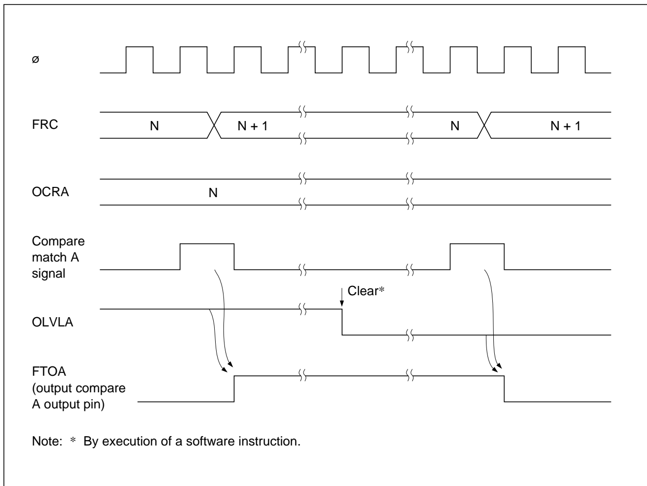
Figure 9-22 Output Compare A Output Timing
