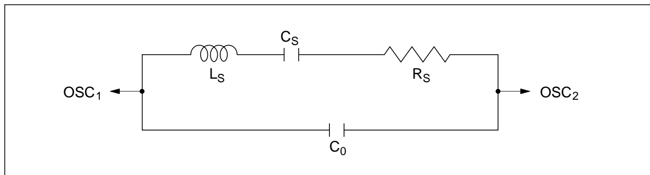
Figure 4-3 Equivalent Circuit of Crystal Oscillator
