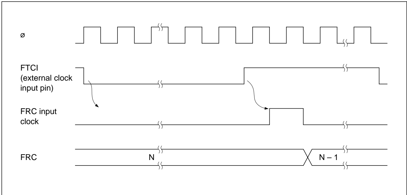
Figure 9-21 Increment Timing with External Clock
