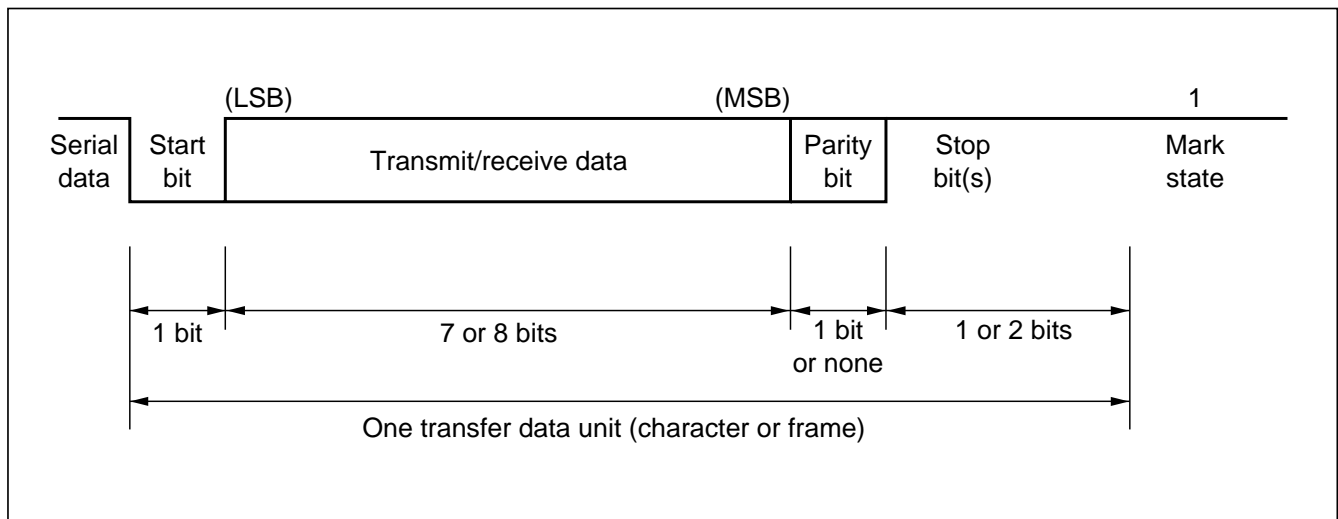
Figure 10-8 Data Format in Asynchronous Communication
