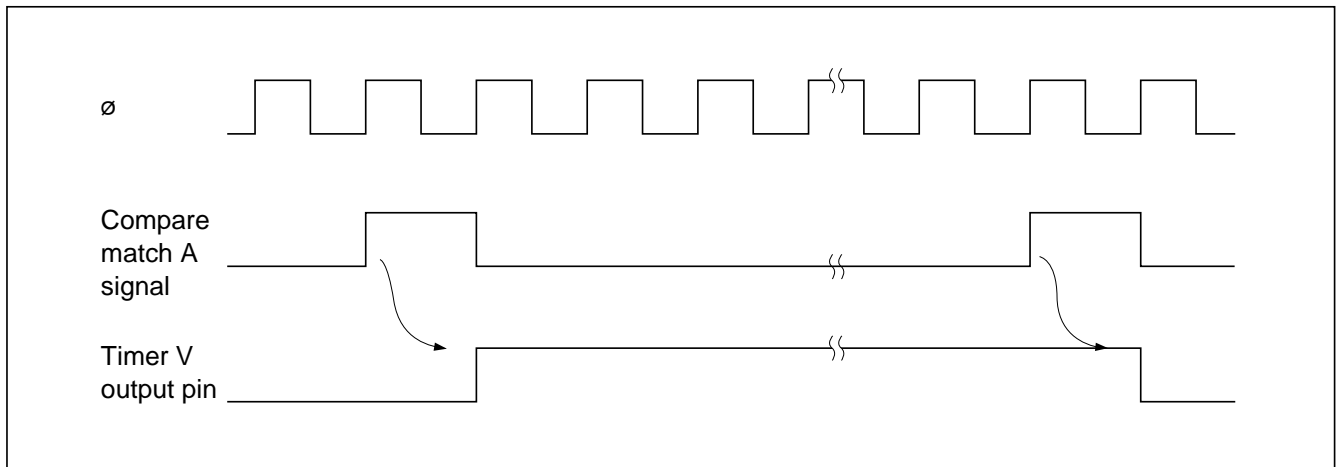
Figure 9-8 TMOV Output Timing
