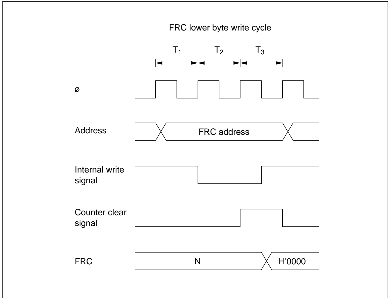
Figure 9-32 Contention between FRC Write and Clear
