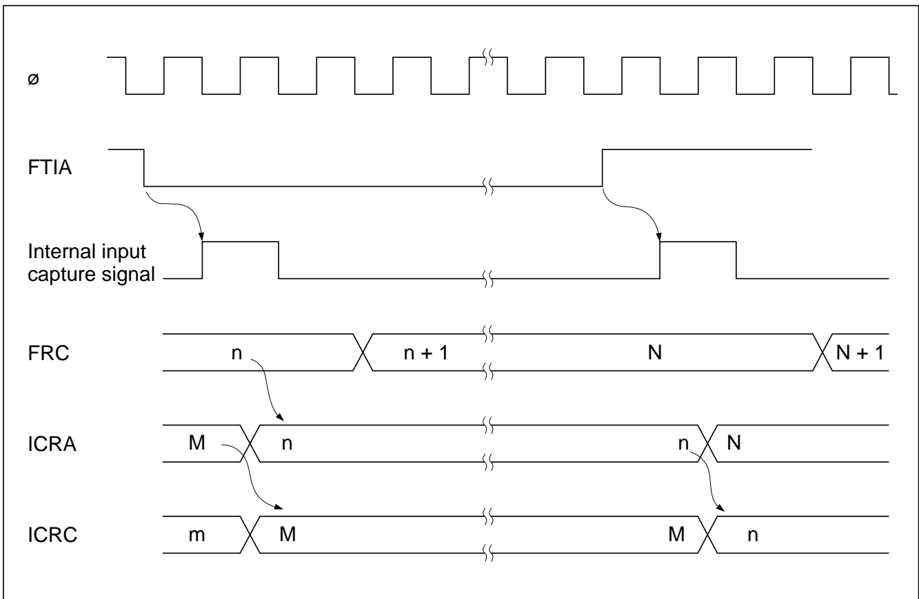
Figure 9-26 Buffered Input Capture Timing (Normal Case)
