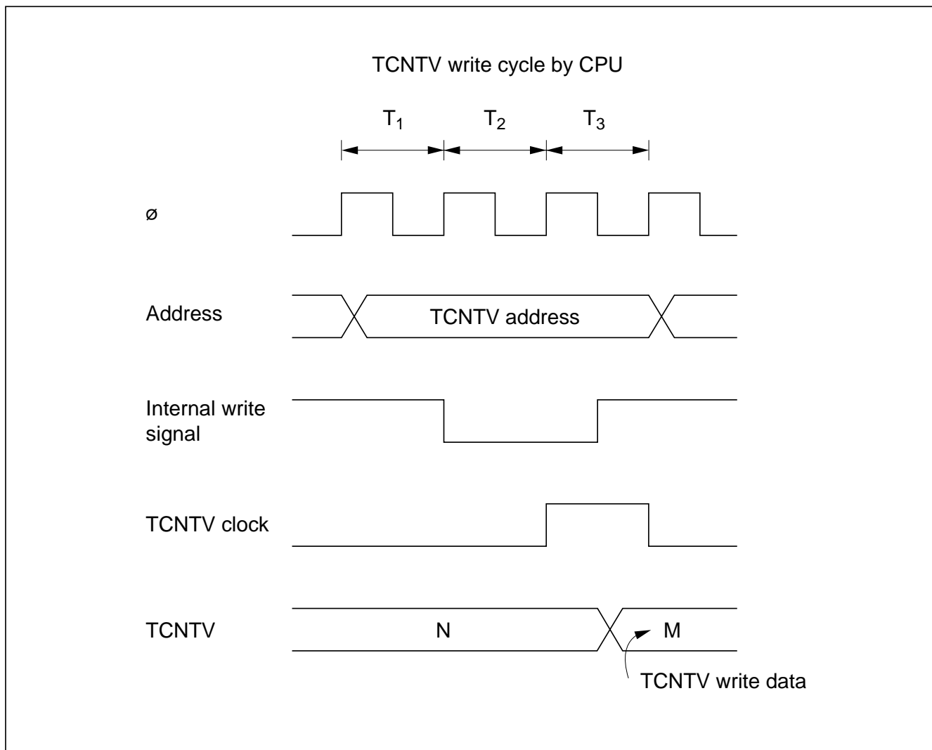
Figure 9-14 Contention between TCNTV Write and Increment
