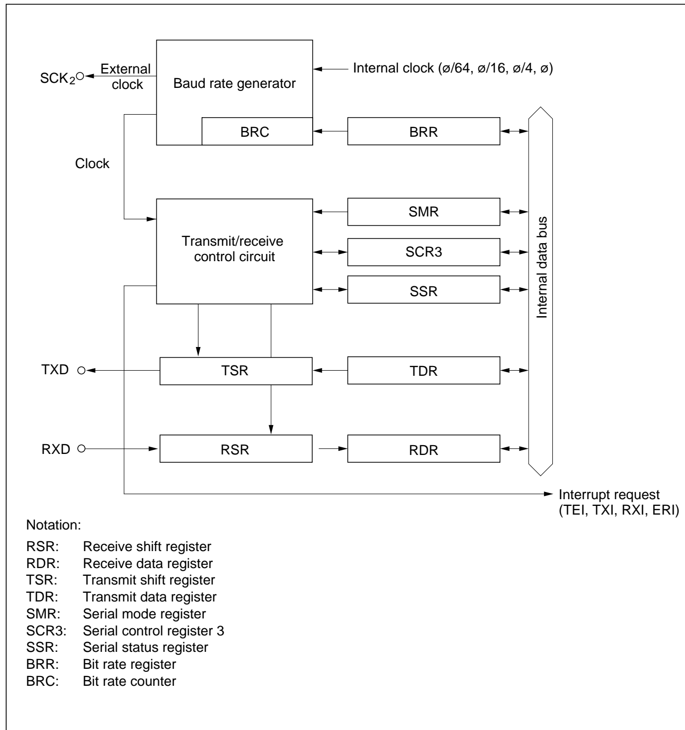
Figure 10-6 SCI3 Block Diagram
