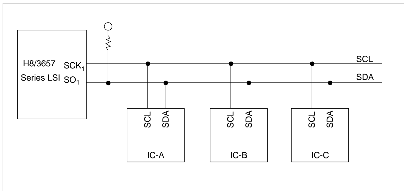
Figure 10-3 Example of SSB Connection
