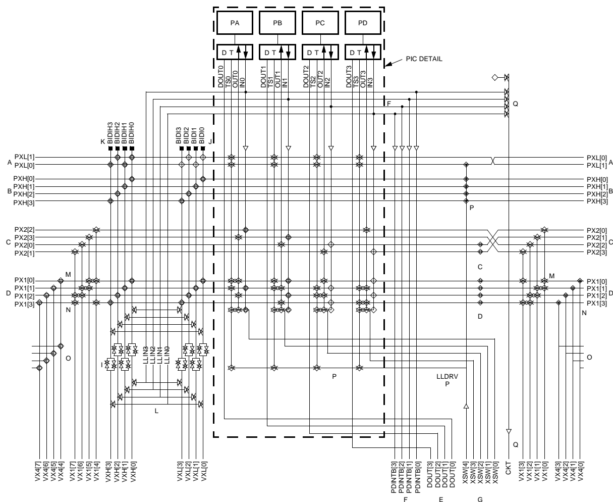
Figure 26. PIC Architecture
