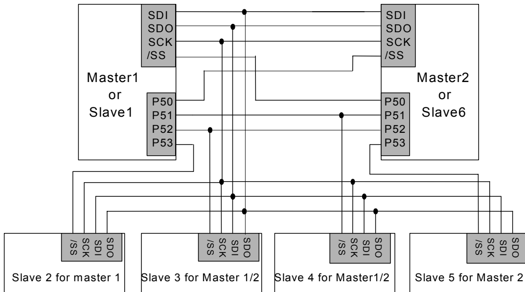
Fig. 10 The SPI Configuration of Single-Master and Multi-Slave
