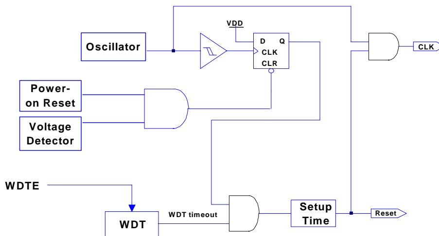
Fig. 16 Block Diagram of Reset
