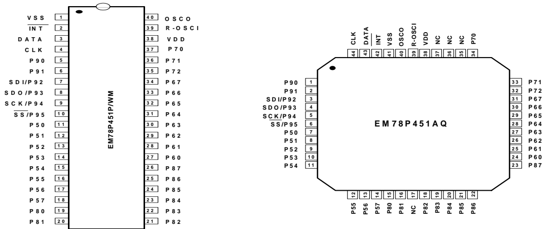
Fig. 1 Pin Assignment
