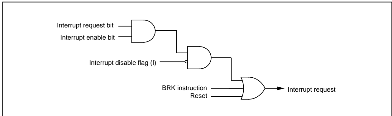
Fig. 15 Interrupt control
