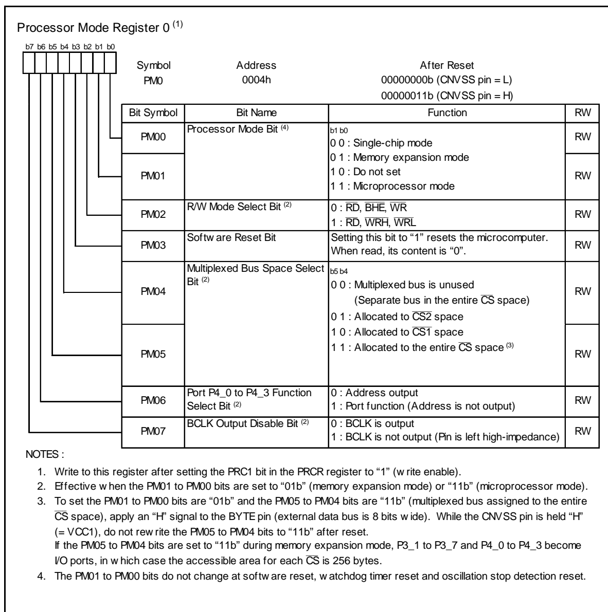
Figure 7.1 PM0 Register
