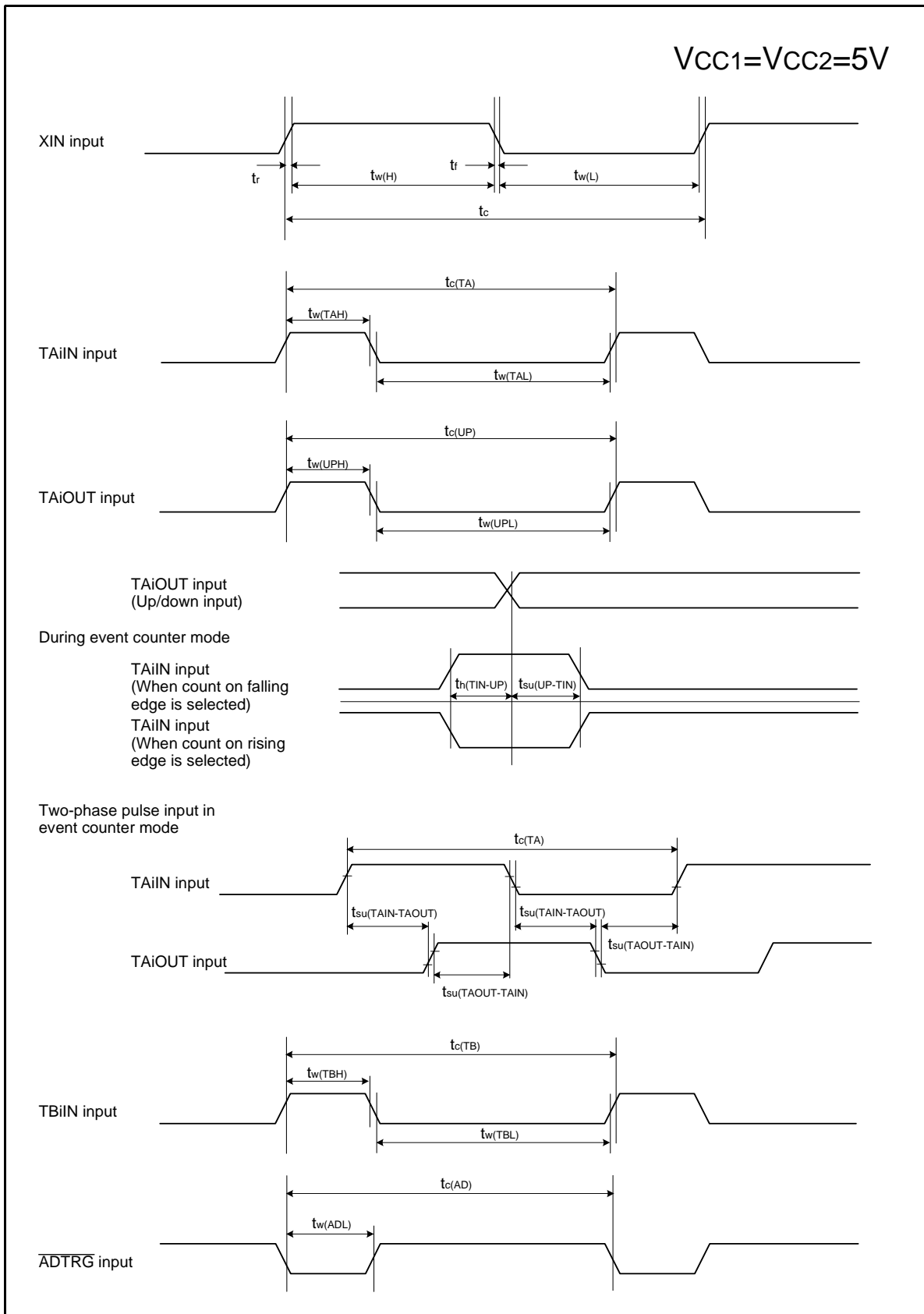
Figure 23.24 Timing Diagram (1)
