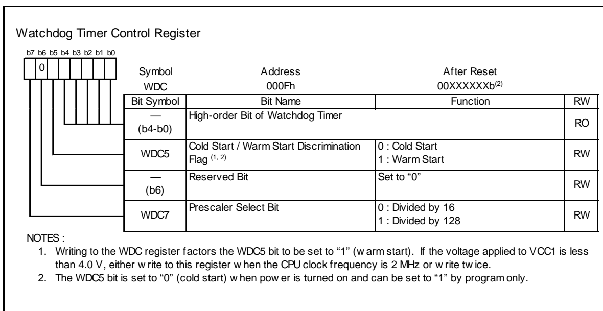
Figure 6.9 WDC Register
