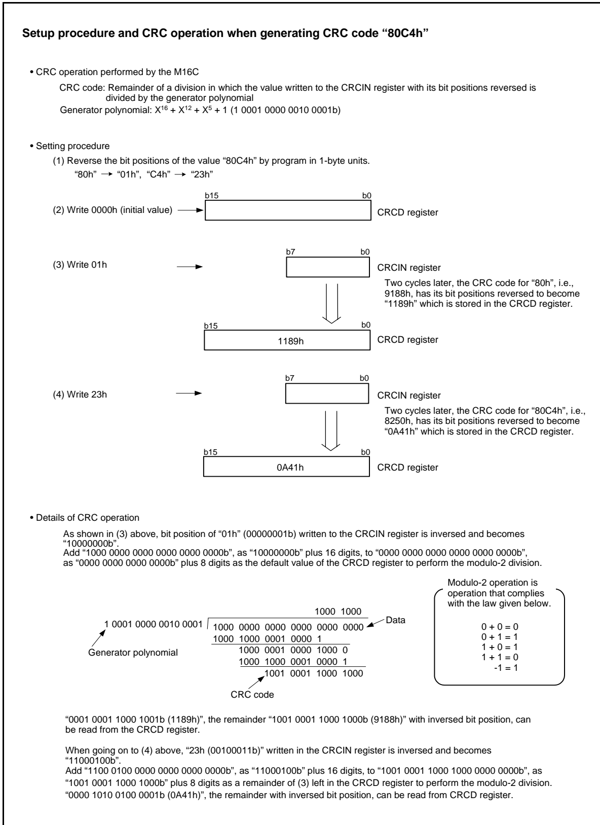
Figure 20.3 CRC Calculation
