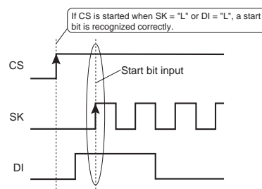
Fig. 40 Normal action timing
