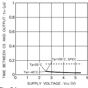
Fig. 24 Time from CS to output establishment t_{sv}
