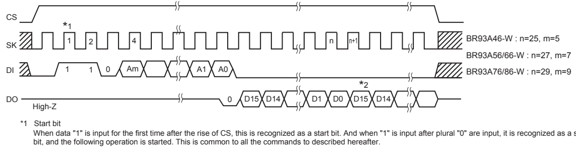
Fig. 30 Read cycle
