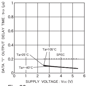
Fig. 23 Output data "1" delay time t_{PD1}
