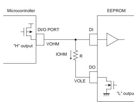
Fig. 54 Circuit at DI, DO direct connection (Microcontroller DI/O "H" output, EEPROM "L" output)
