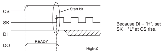
Fig. 53 Start bit input timing at DI, DO direct connection
