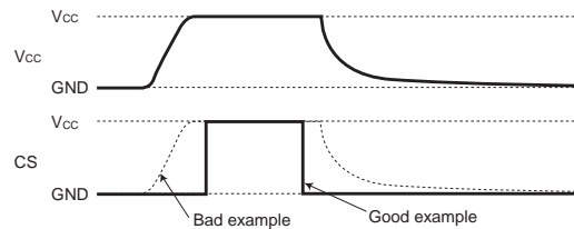
Fig. 56 Timing at power ON/OFF
