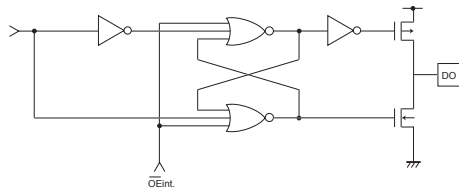
Fig. 41 Output circuit (DO)
