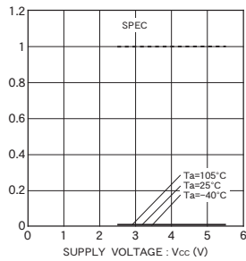
Fig. 8 Input leak current I_i (CS,SK,DI)
