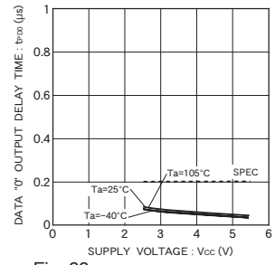
Fig. 22 Data "0" output delay time t_{PD0}
