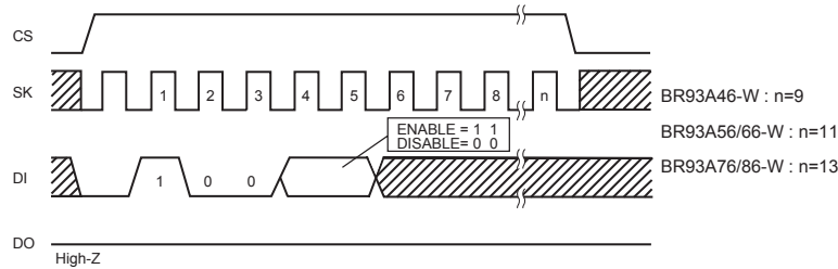
Fig. 33 Write enable (WEN) / disable (WDS) cycle
