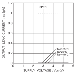
Fig. 9 Output leak current I_{LO} (DO)
