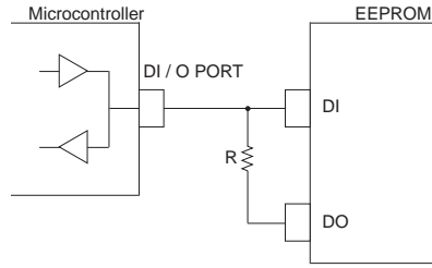
Fig. 50 DI, DO control line common connection
