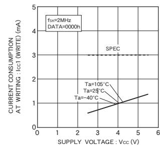
Fig. 10 Current consumption at WRITE action I_{CC1}(WRITE, f_{SK}=2MHz)
