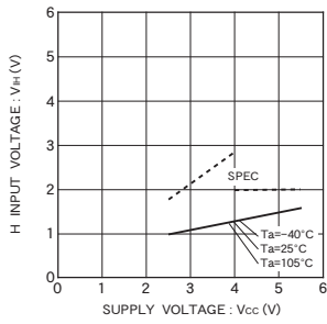
Fig. 2 H input voltage V_{IH} (CS,SK,DI)
