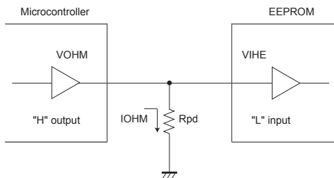
Fig. 45 CS pull down resistance
