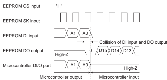
Fig. 51 Collision timing at read data output at DI, DO direct connection
