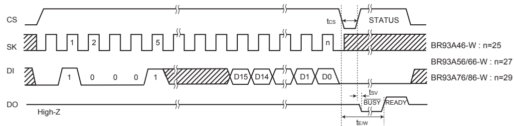
Fig. 32 Write all cycle
