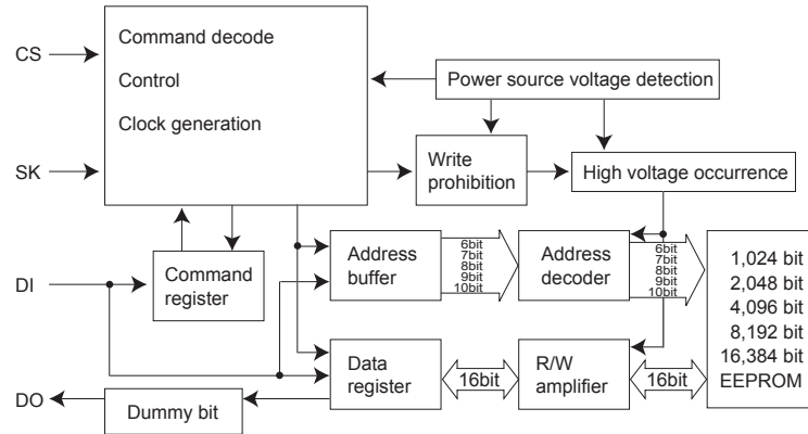
Fig. 27 Block diagram
