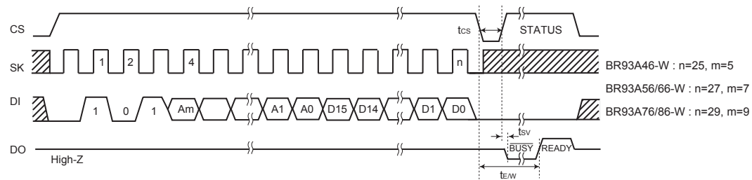
Fig. 31 Write cycle
