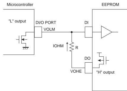
Fig. 55 Circuit at DI, DO direct connection (Microcontroller DI/O "L" output, EEPROM "H" output)
