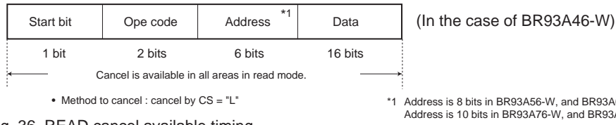
Fig. 36 READ cancel available timing
