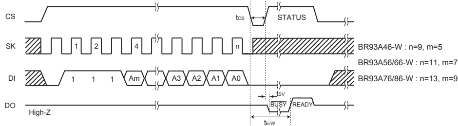
Fig. 34 Erase cycle timing
