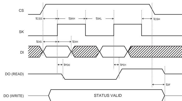
Fig.1 Sync data input / output timing
