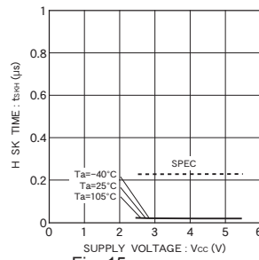
Fig. 15 SK high time t_{sKH}
