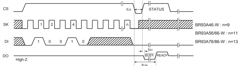
Fig. 35 Chip erase cycle timing
