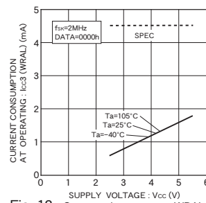
Fig. 12 Consumption current at WRAL action I_{CC3}(WRAL, f_{SK}=2MHz)
