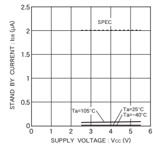
Fig. 13 Consumption current at standby action I_{SS}
