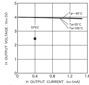
Fig. 7 H output voltage V_{OH-IOH}(V_{CC}=4.0V)
