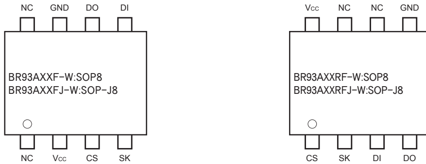
Fig. 28 Pin assignment diagram
