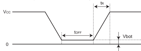
Fig. 57 Rise waveform diagram
