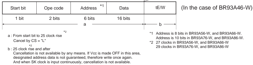
Fig. 37 WRITE, WRAL cancel available timing
