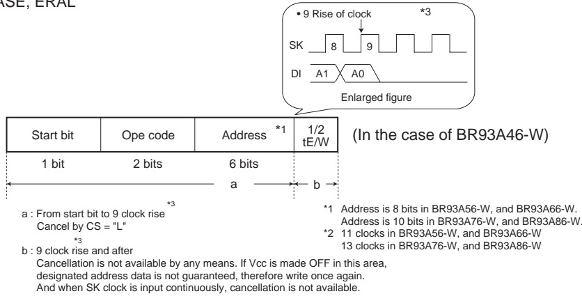
Fig. 38 ERASE, ERAL cancel available timing
