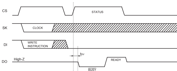
Fig. 49 \overline{RDY} status output timing chart
