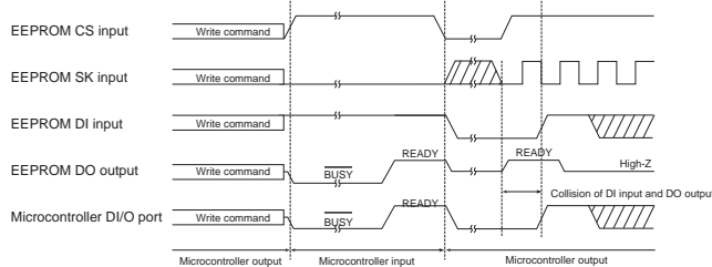
Fig. 52 Collision timing at DI, DO direct connection
