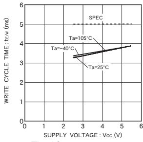
Fig. 26 Write cycle time t_{EW}
