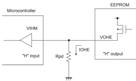
Fig. 48 DO pull down resistance
