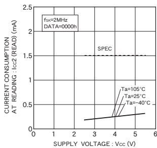
Fig. 11 Consumption current at READ action I_{CC2}(READ, f_{SK}=2MHz)
