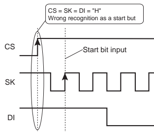
Fig. 39 Wrong action timing
