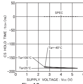
Fig. 18 CS hold time t_{cSH}
