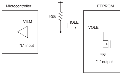
Fig. 47 DO pull up resistance
