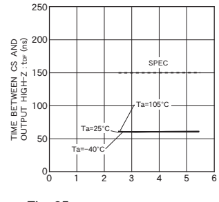
Fig. 25 Time from CS to High-Z t_{DF}
