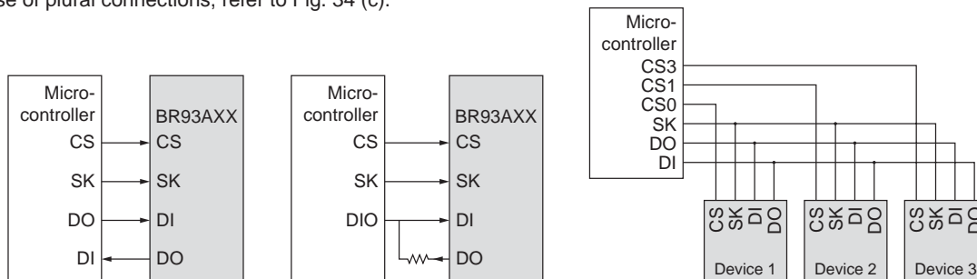
Fig. 29-(a) Connection by 4 lines
