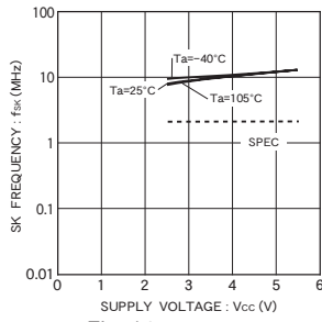
Fig. 14 SK frequency f_{sk}
