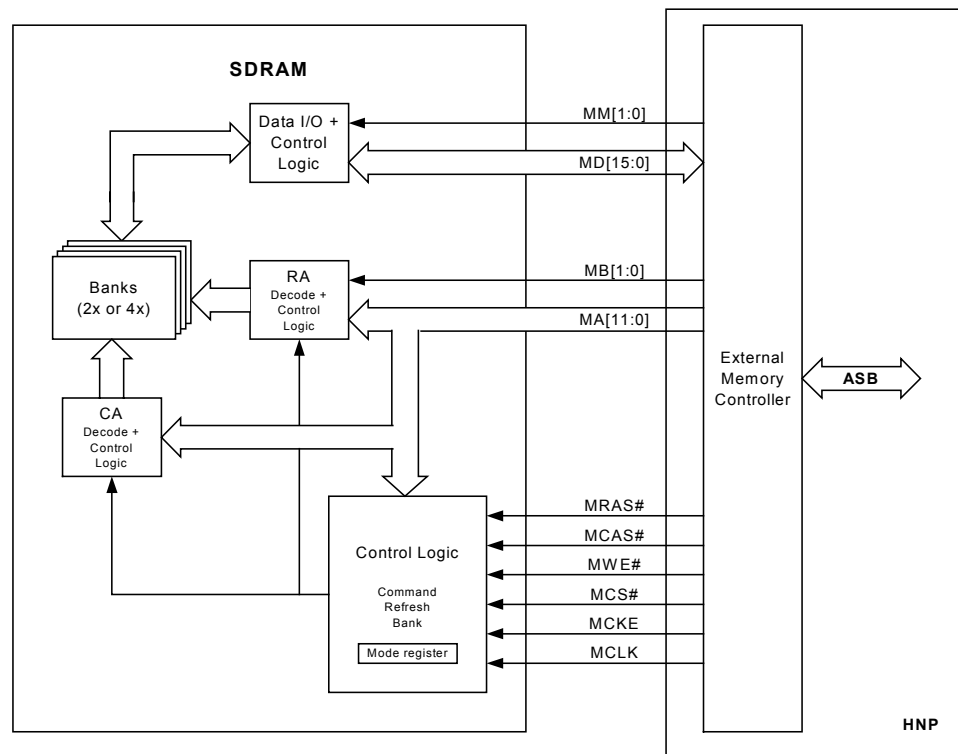
Figure 6-1. SDRAM Interface
