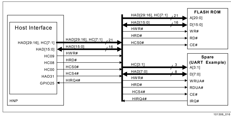
Figure 5-1. Host Master Mode Signals
