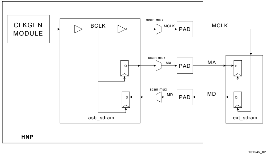
Figure 6-2. EMC Clocking Interface
