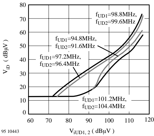
Figure 45. V_{iD} vs. V_{iUD1,2}
