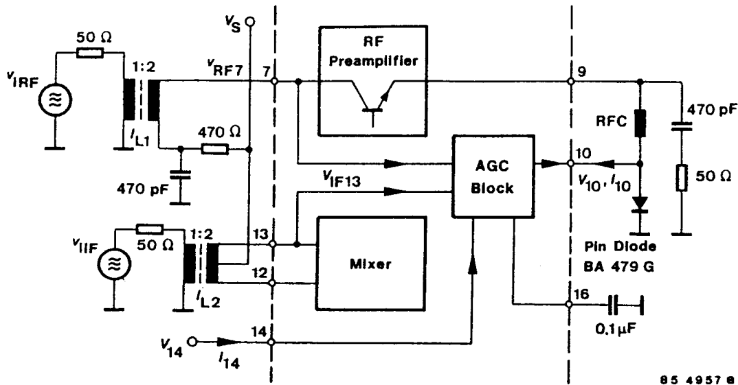
Figure 27. Test circuit
