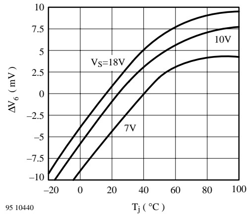
Figure 41. \Delta V_6 vs. T_j
