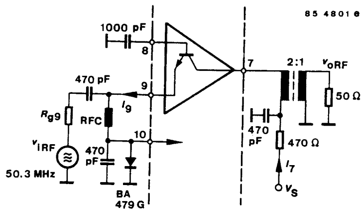
Figure 4. Test circuit
