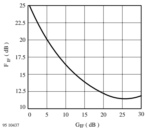
Figure 37. F_{IF} vs. G_{IF}
