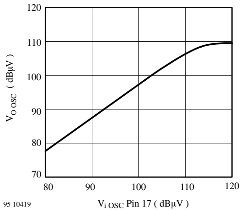
Figure 15. V_{\text{Osc}} vs. V_{i\text{ Osc}}
