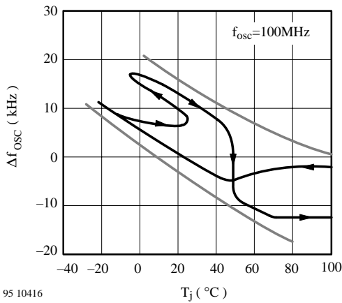
Figure 12. \Delta f_{osc} vs. T_j
