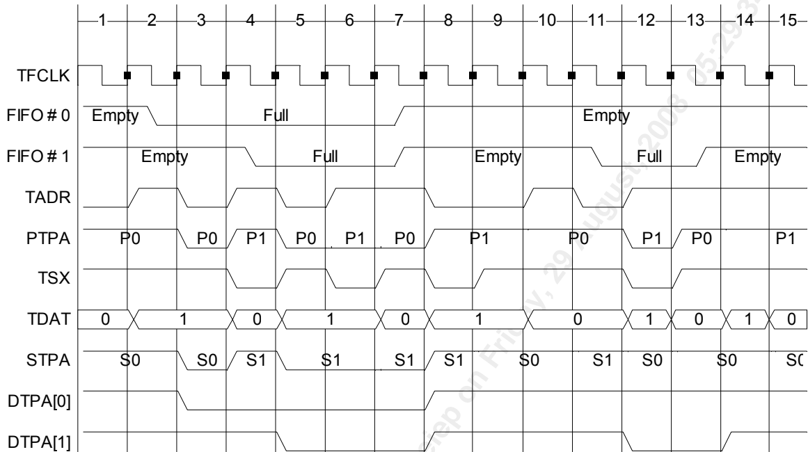
Figure 16 - PM3386 Packet-Level Transmit Polling Logical Timing
