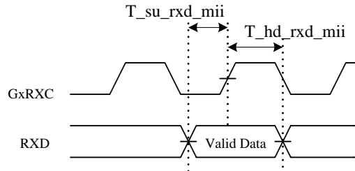
Figure 26. MII Receive Timing
