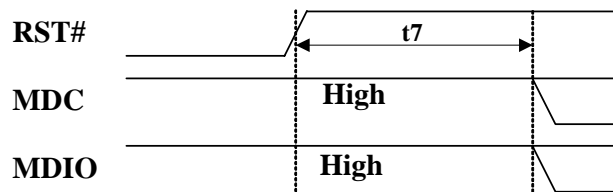
Figure 20. MDC/MDIO Reset Timing
