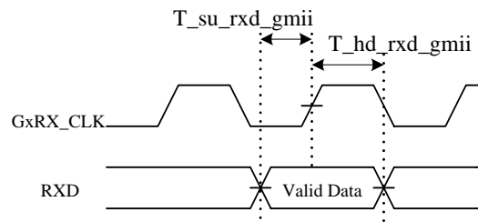
Figure 24. GMII Receive Timing
