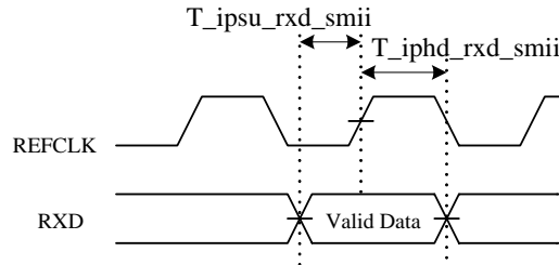
Figure 22. SMII Receive Timing
