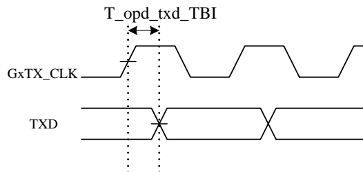
Figure 27. TBI Transmit Timing
