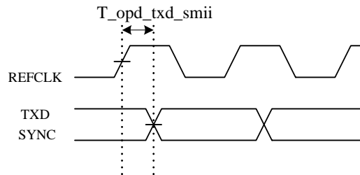
Figure 21. SMII Transmit Timing
