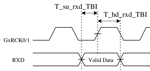
Figure 28. TBI Receive Timing
