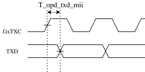
Figure 25. MII Transmit Timing
