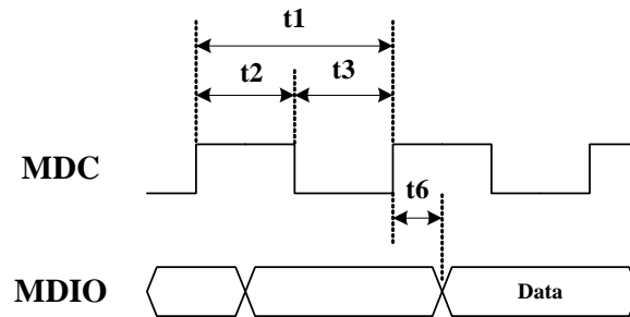
Figure 19. MDC/MDIO Read Timing
