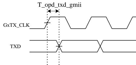
Figure 23. GMII Transmit Timing
