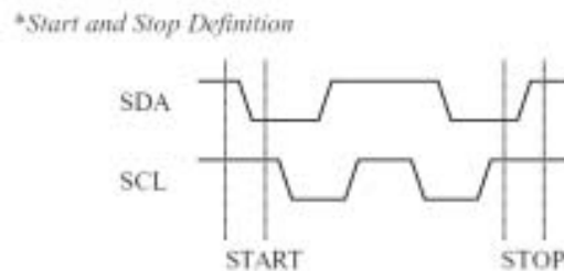
Figure 13. Start and Stop Definition
