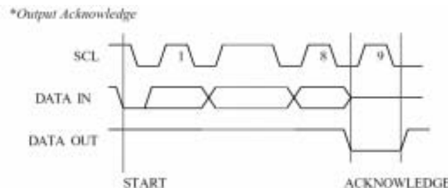
Figure 14. Output Acknowledge (ACK)
