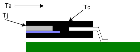
Figure 29. Cross-section of 208 PQFP
