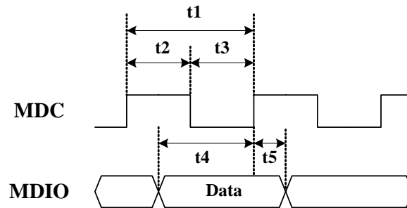
Figure 18. MDC/MDIO Write Timing
