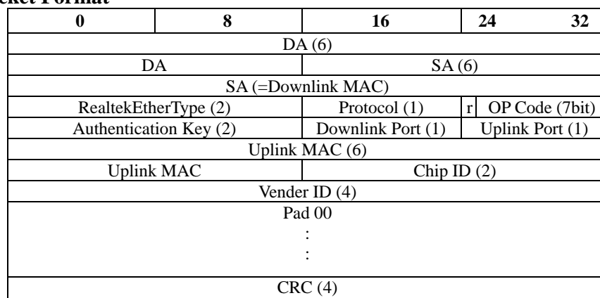
Figure 9. Hello_Reply Packet Format
