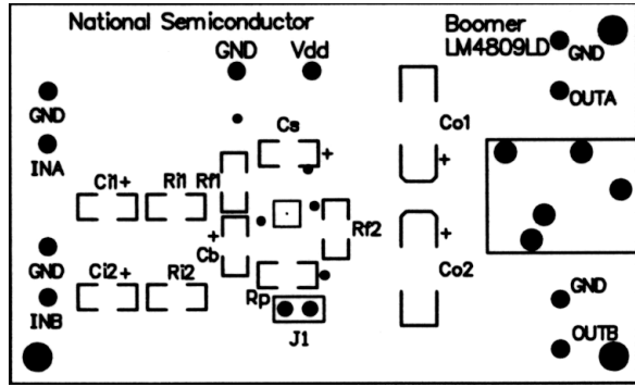
FIGURE 6. Recommended LD PC Board Layout Component-Side Silkscreen
