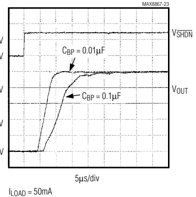
MAX886 E_K50 SHUTDOWN EXIT DELAY
