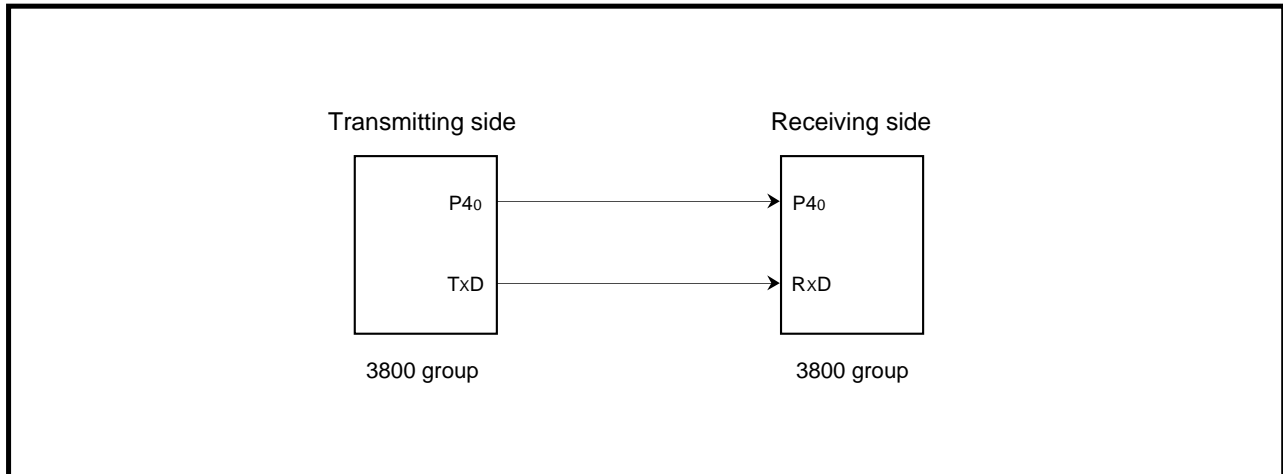
Fig. 2.3.29 Connection diagram [Communication using UART]
