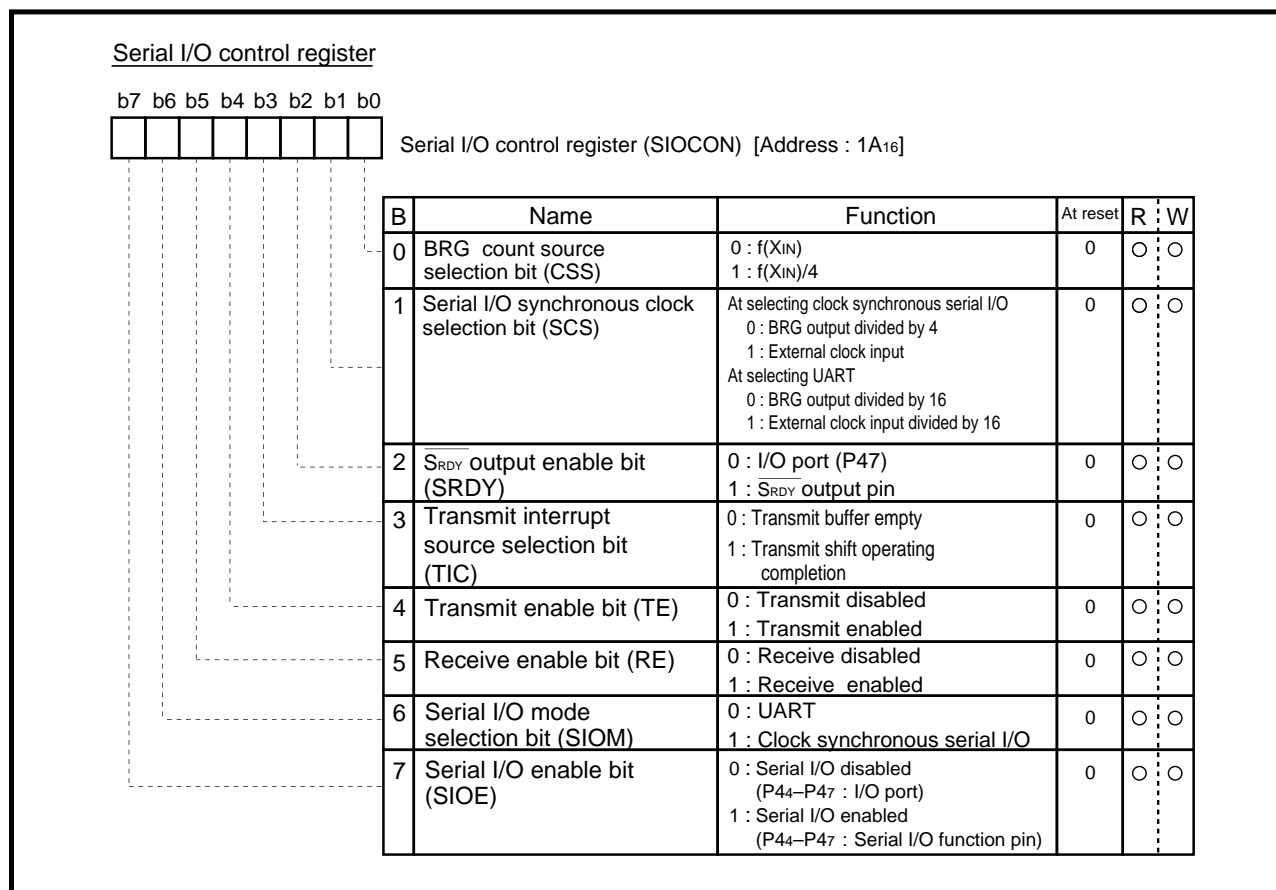
Fig. 3.5.5 Structure of Serial I/O control register
