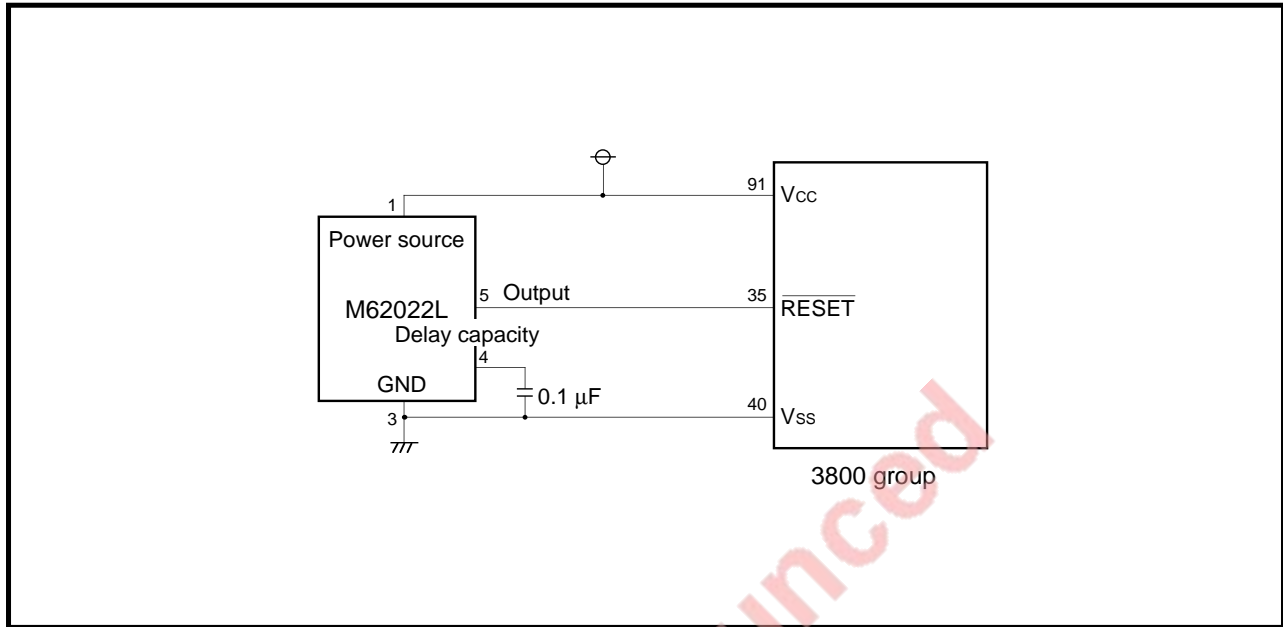
Fig. 2.5.1 Example of Poweron reset circuit
