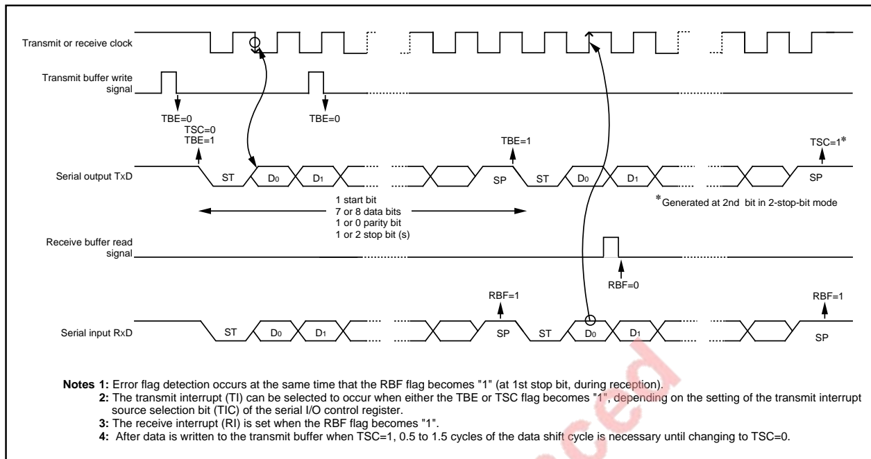
Fig. 20 Operation of UART serial I/O function
