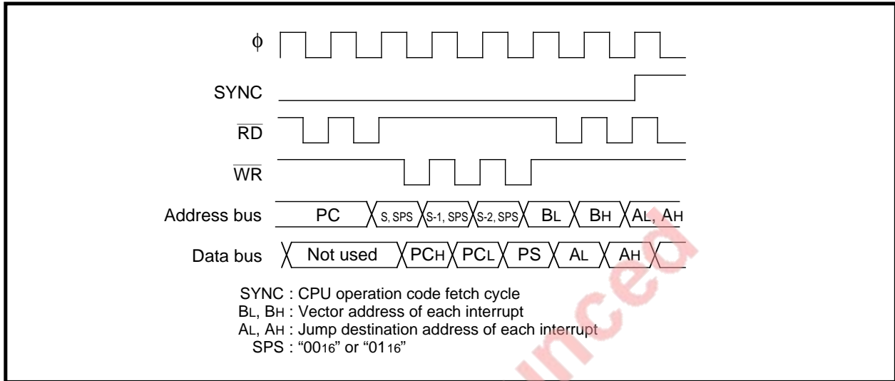
Fig. 32 Timing chart after an interrupt occurs
