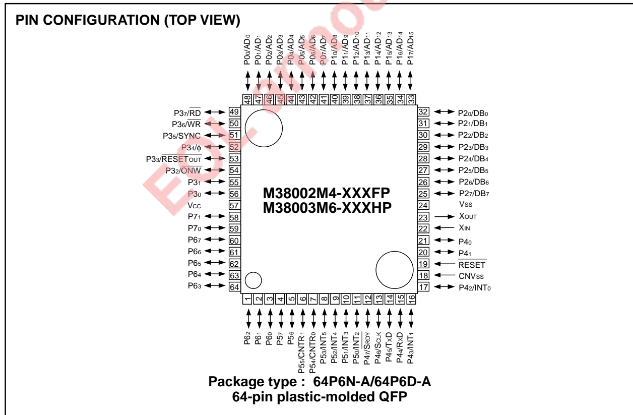
Fig. 1 Pin configuration of M38002M4-XXXFP/M38003M6-XXXHP
