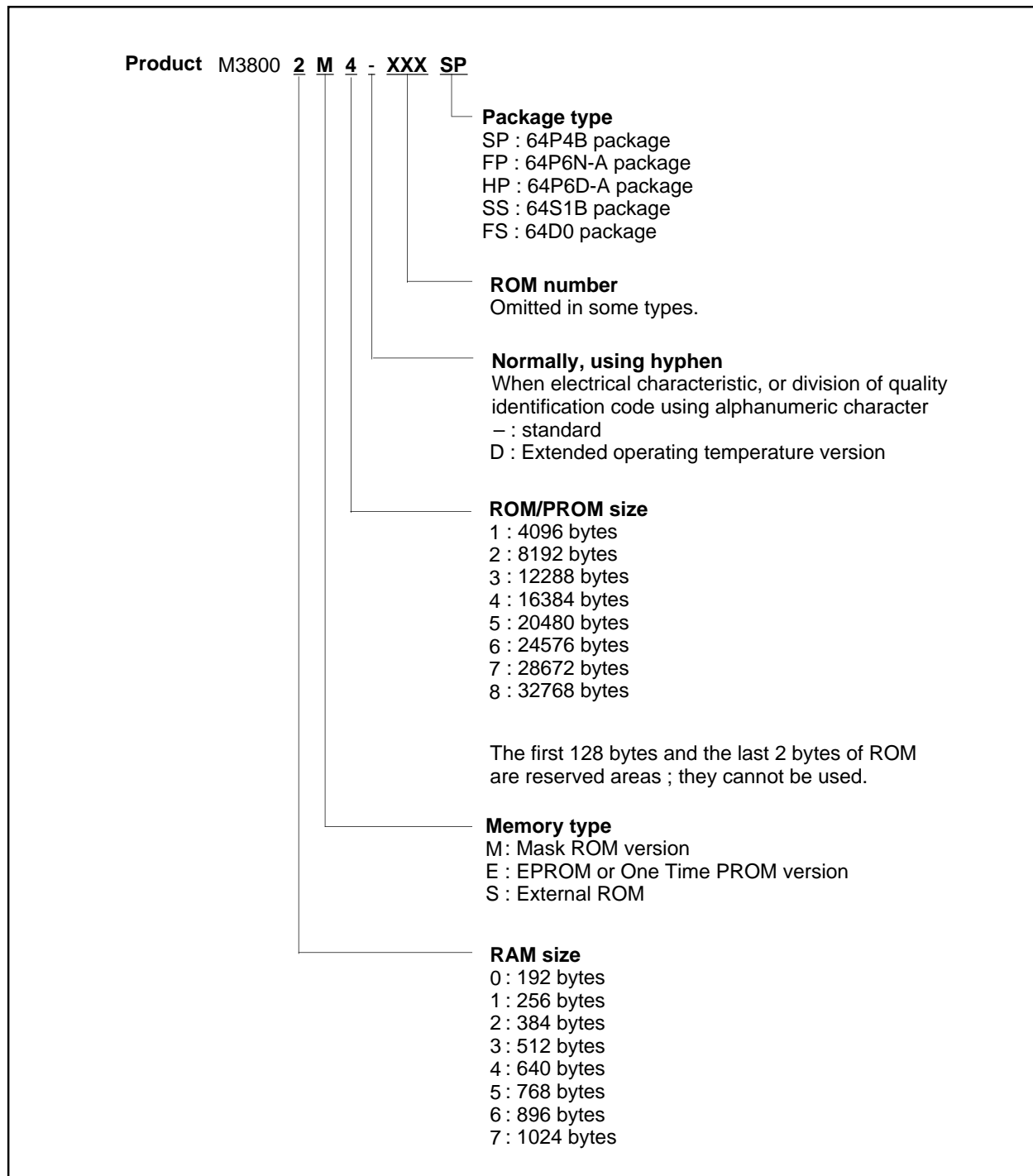
Fig. 4 Part numbering
