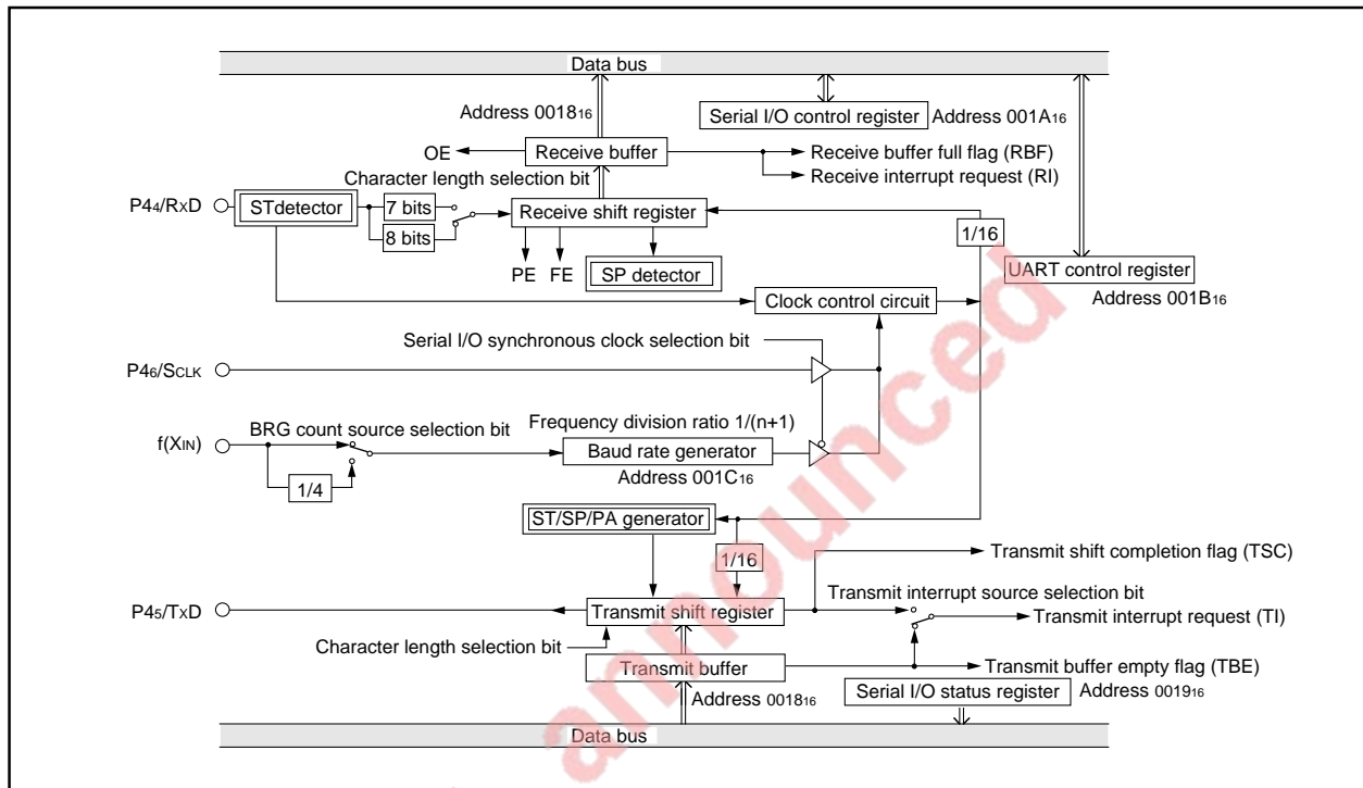
Fig. 19 Block diagram of UART serial I/O
