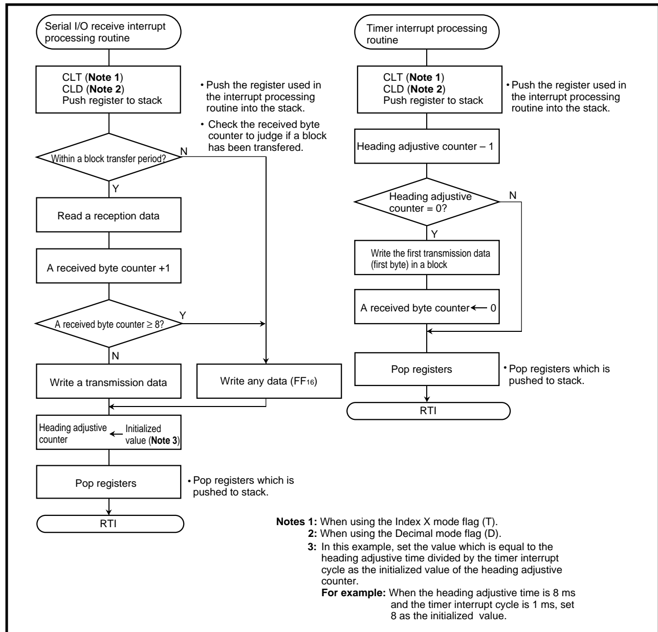
Fig. 2.3.28 Control in the slave unit
