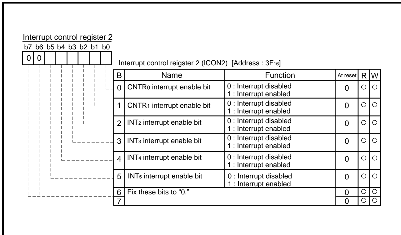
Fig. 3.5.17 Structure of Interrupt control register 2
