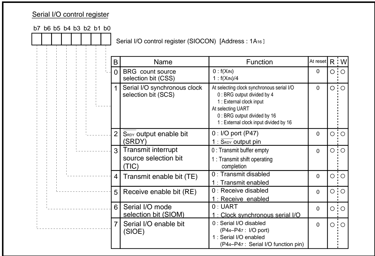
Fig. 2.3.4 Structure of Serial I/O control register
