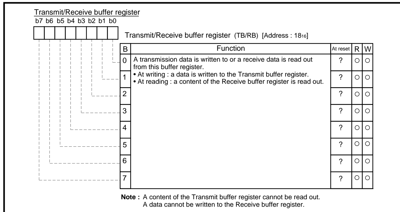
Fig. 2.3.2 Structure of Transmit/Receive buffer register
