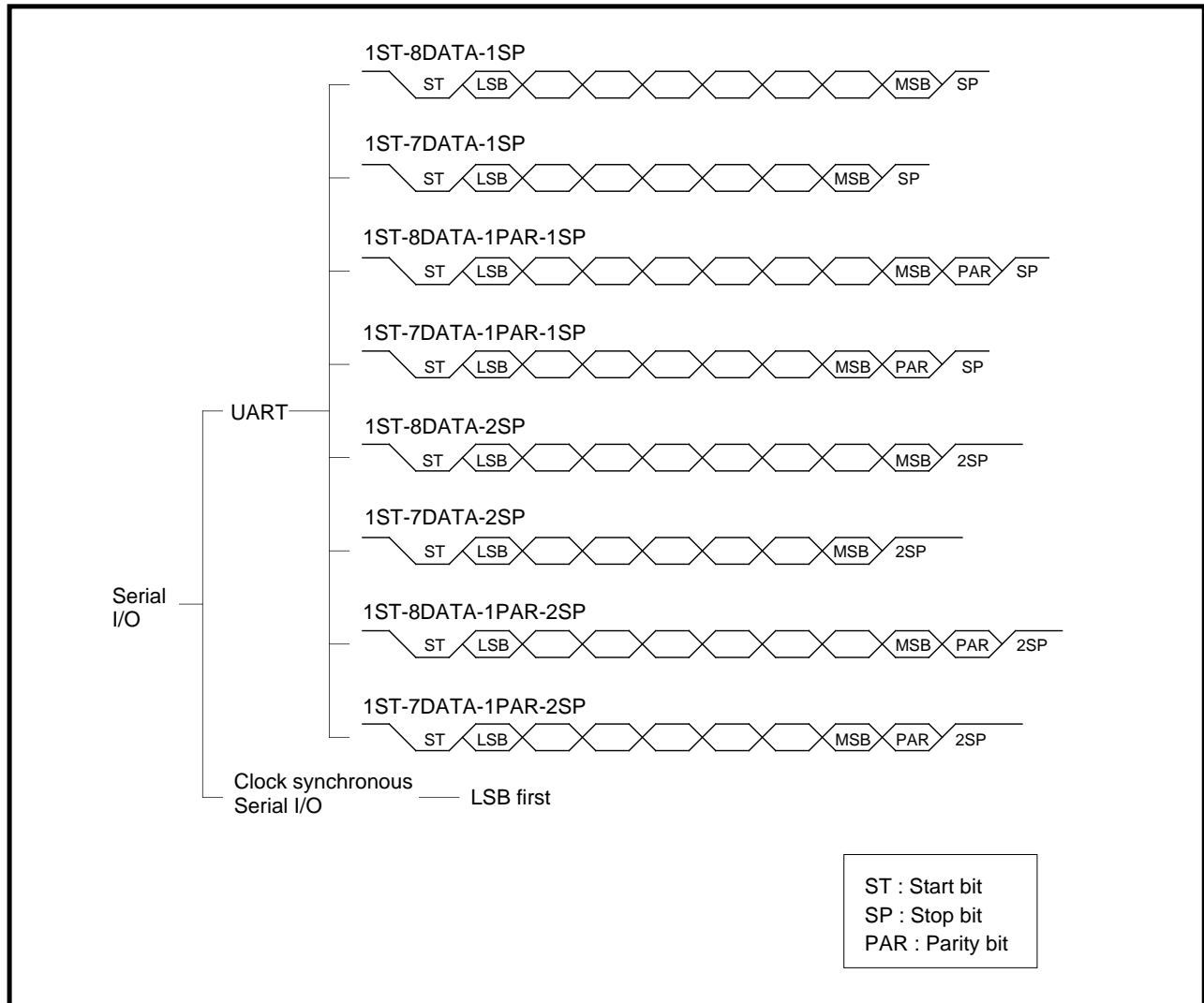
Fig. 2.3.12 Setting of Serial I/O transfer data format
