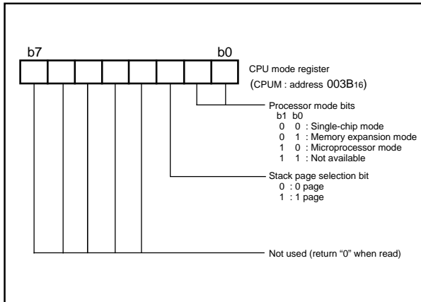
Fig. 9 Structure of CPU mode register
