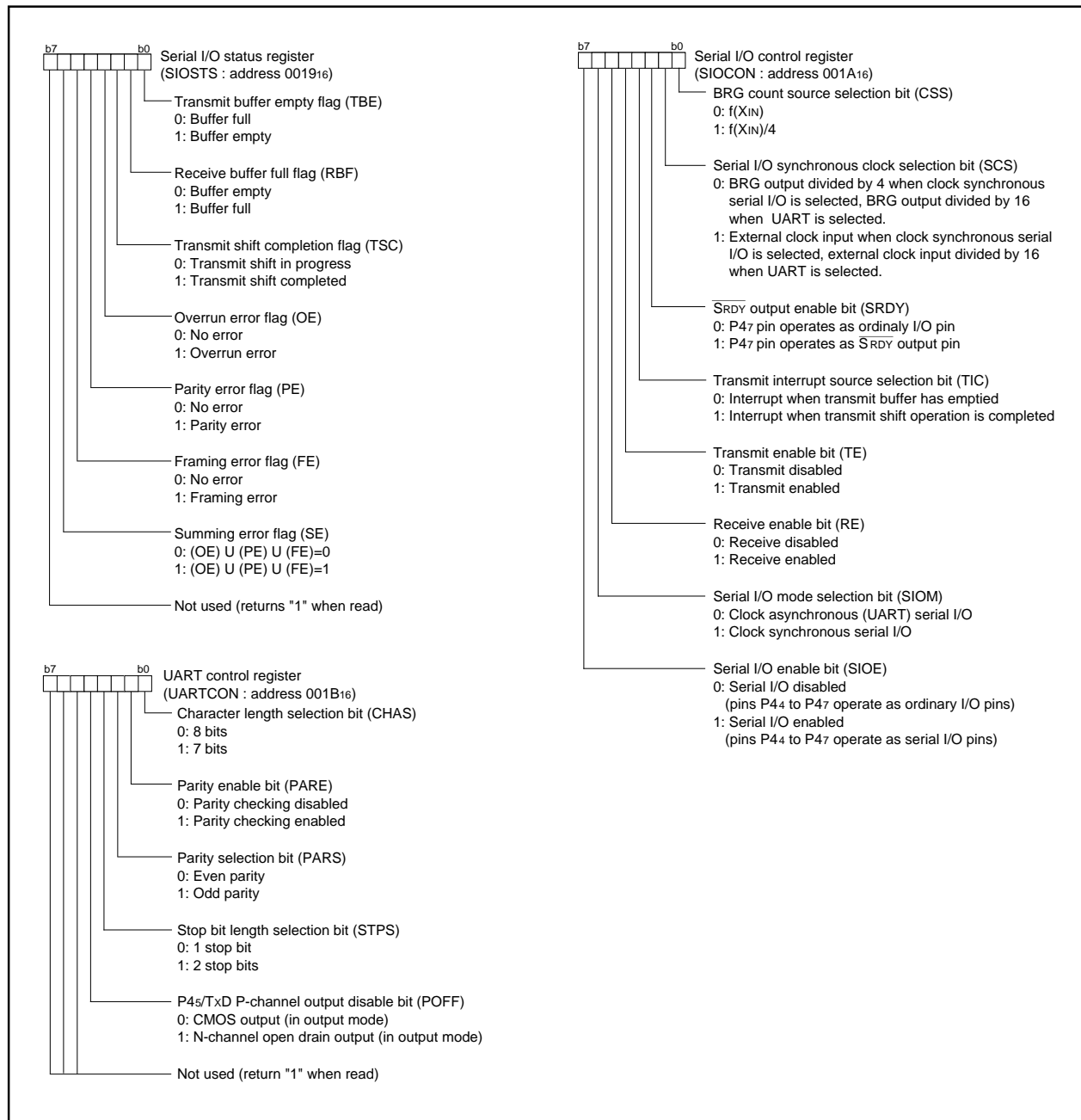
Fig. 21 Structure of serial I/O control registers
