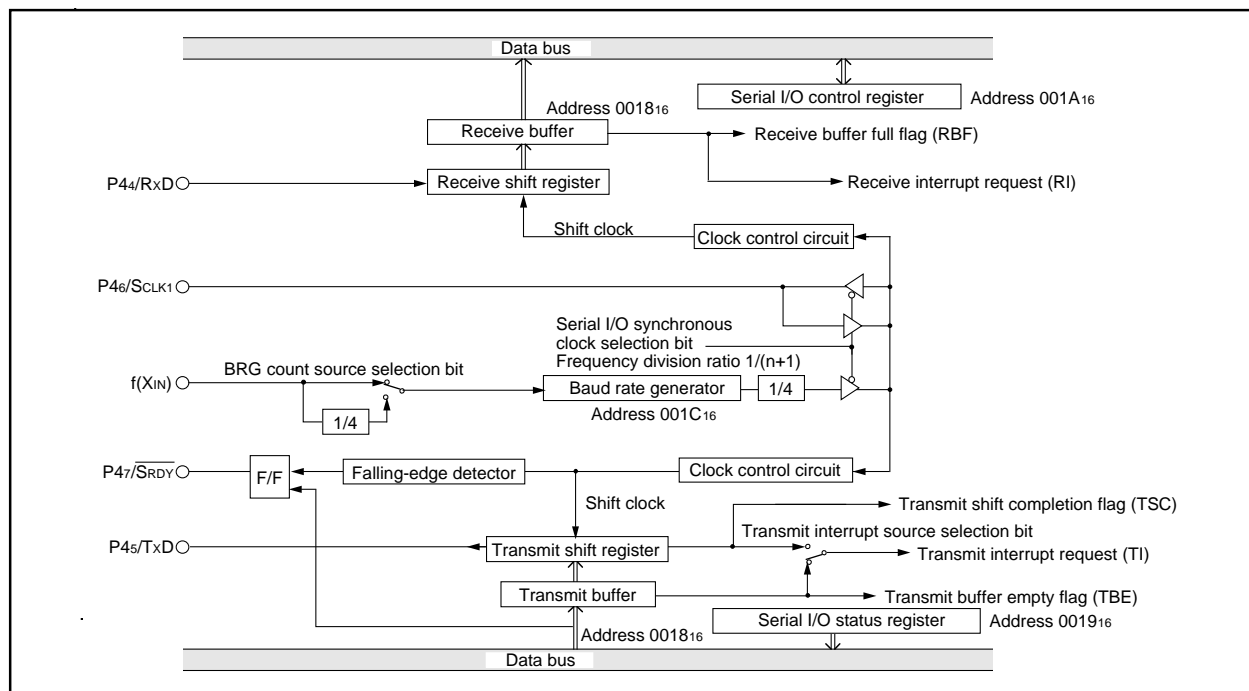
Fig. 17 Block diagram of clock synchronous serial I/O
