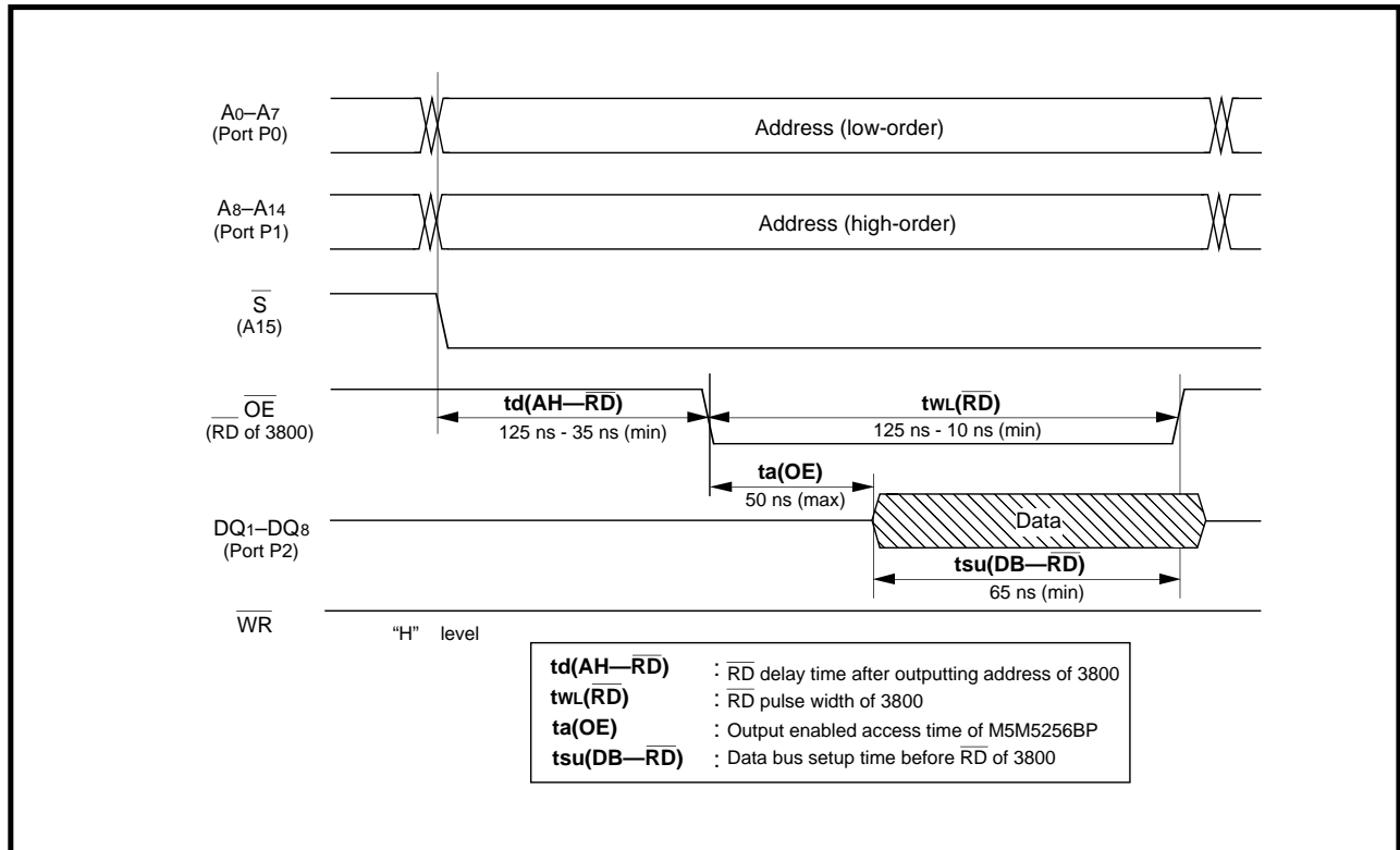
Fig. 2.4.4 Read-cycle (OE access, SRAM)
