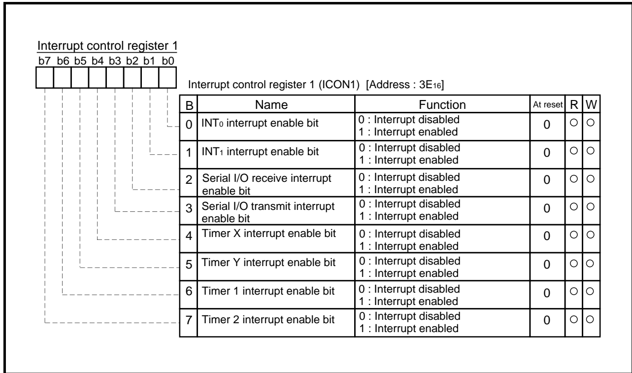
Fig. 3.5.16 Structure of Interrupt control register 1
