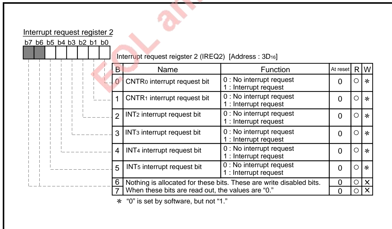
Fig. 3.5.15 Structure of Interrupt request register 2
