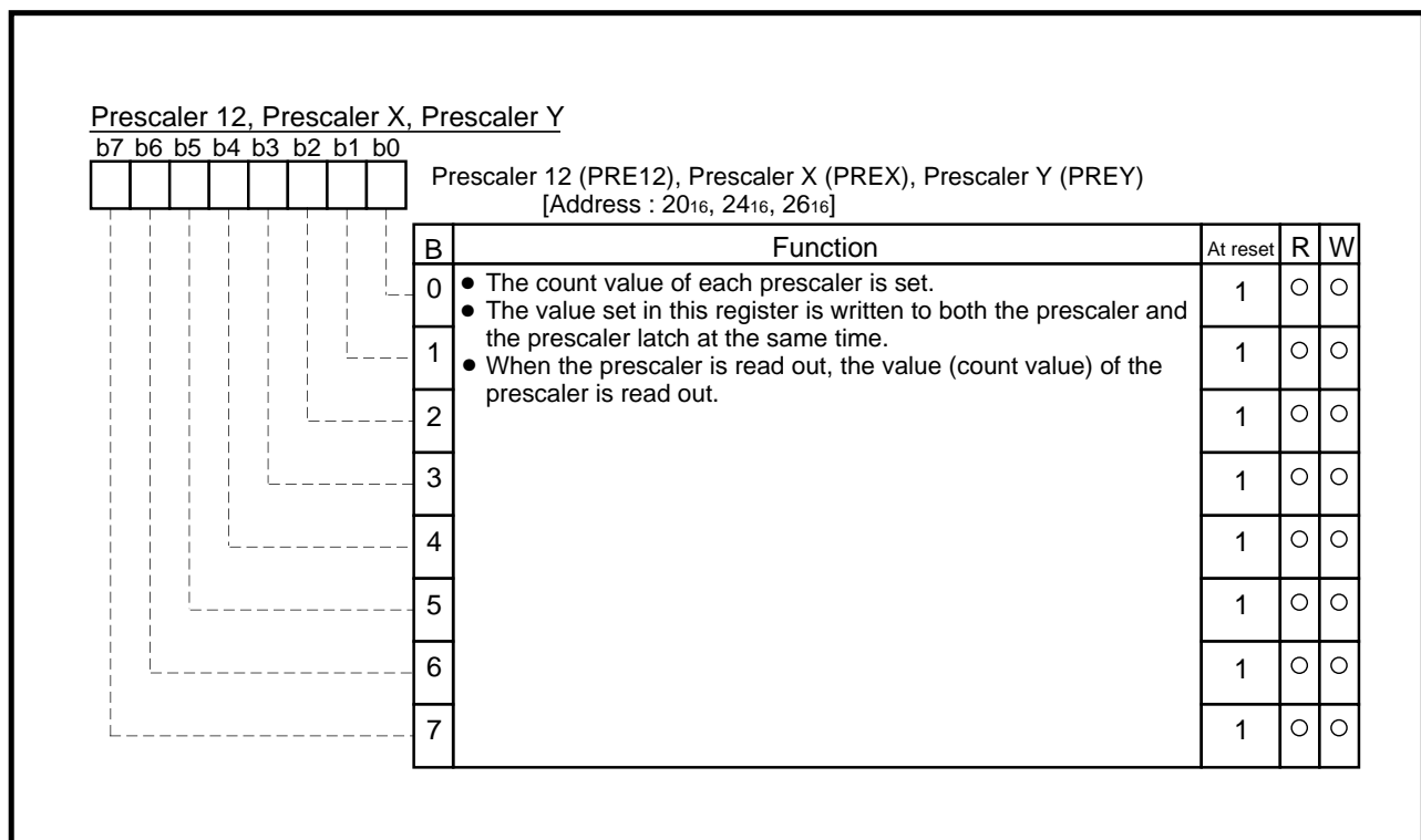
Fig. 3.5.8 Structure of Prescaler 12, Prescaler X, Prescaler Y
