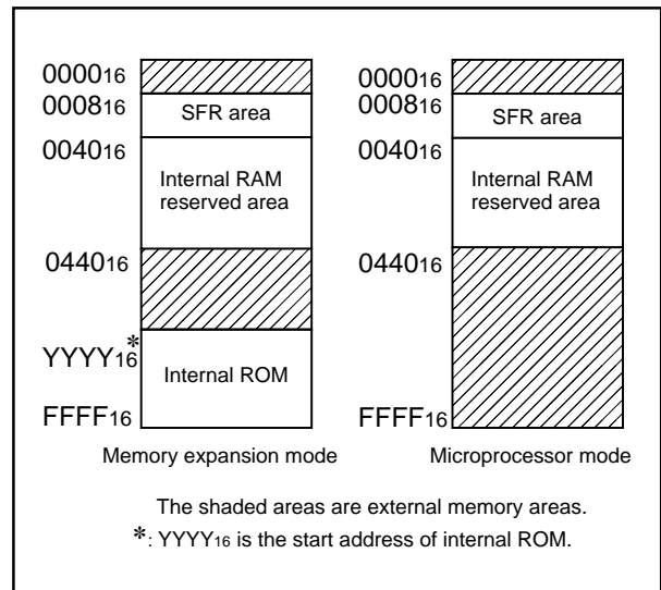
Fig. 28 Memory maps in various processor modes
