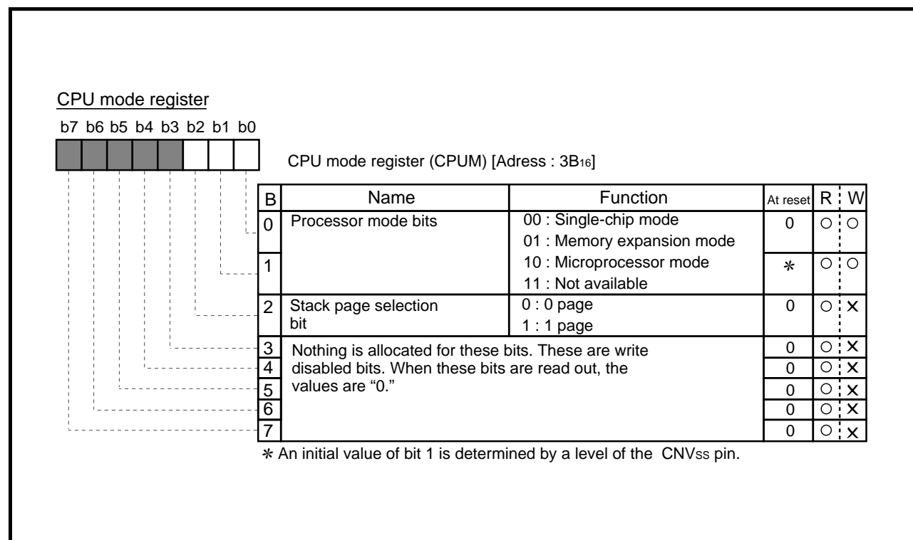
Fig. 3.5.13 Structure of CPU mode register
