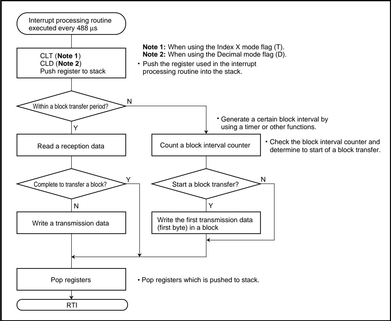
Fig. 2.3.27 Control in the master unit
