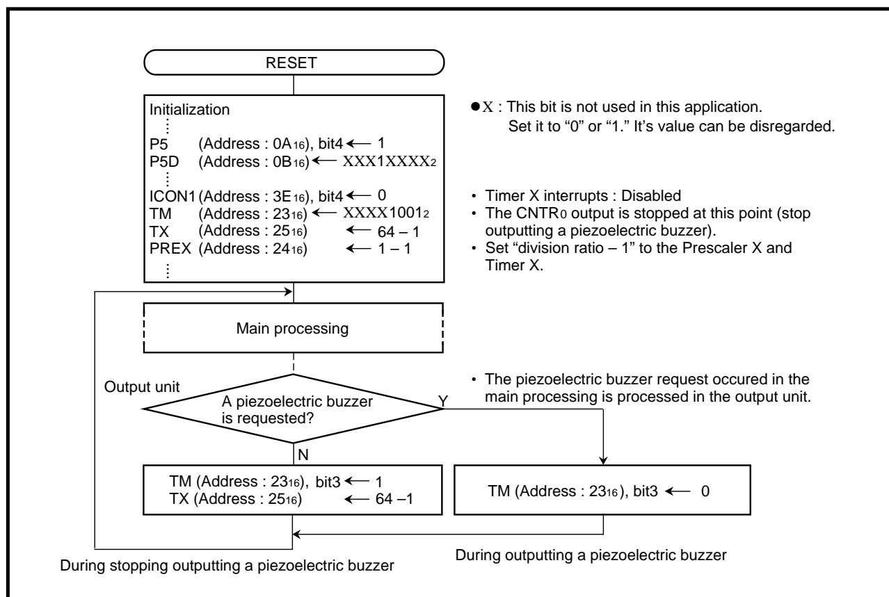
Fig. 2.2.16 Control procedure [Piezoelectric buzzer output]
