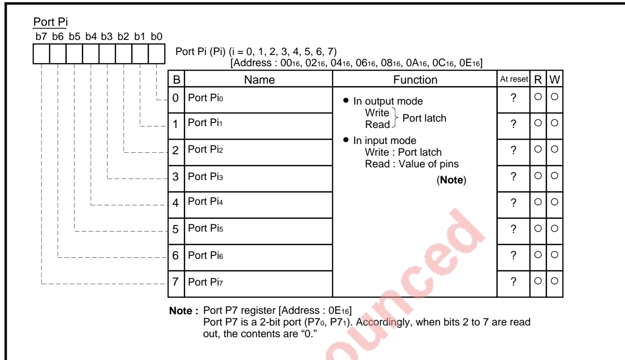
Fig. 3.5.1 Structure of Port Pi (i = 0, 1, 2, 3, 4, 5, 6, 7)
