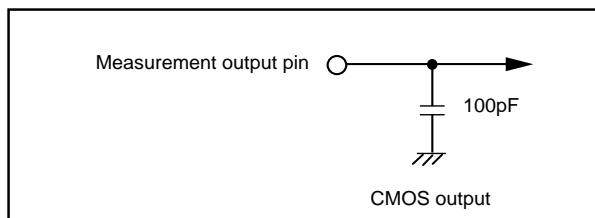
Fig. 3.1.1 Circuit for measuring output switching characteristics
