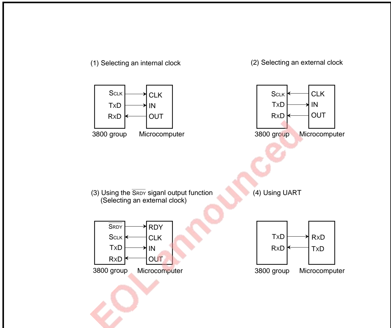
Fig. 2.3.11 Serial I/O connection examples (2)
