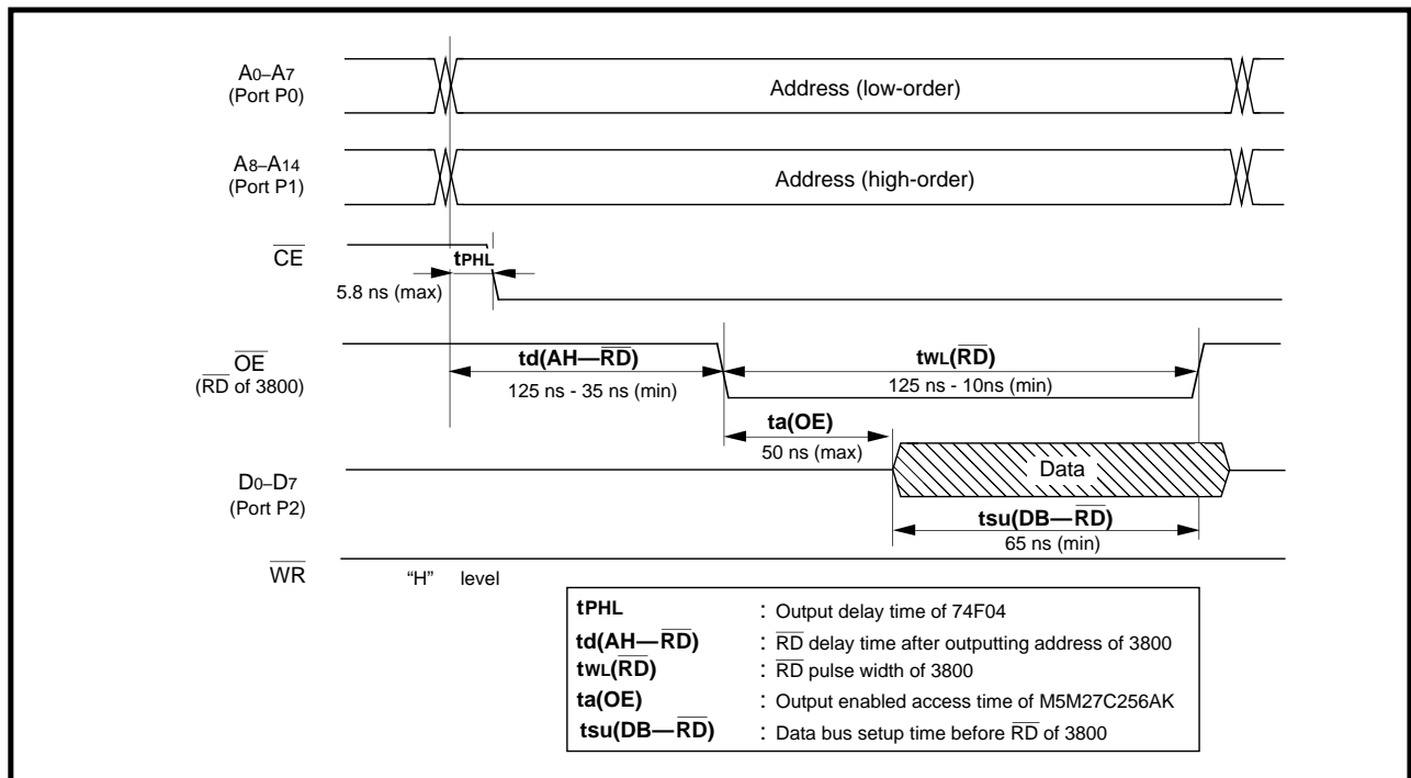
Fig. 2.4.5 Read-cycle (OE access, EPROM)
