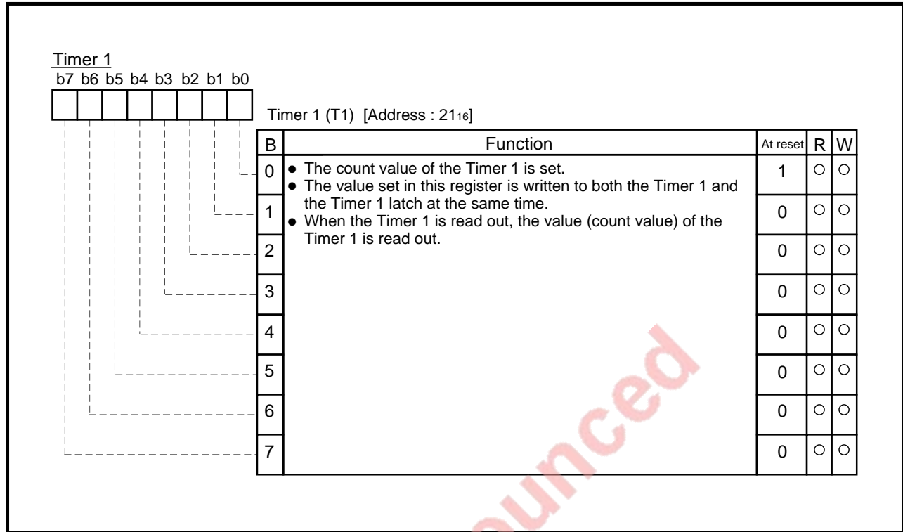
Fig. 3.5.9 Structure of Timer 1
