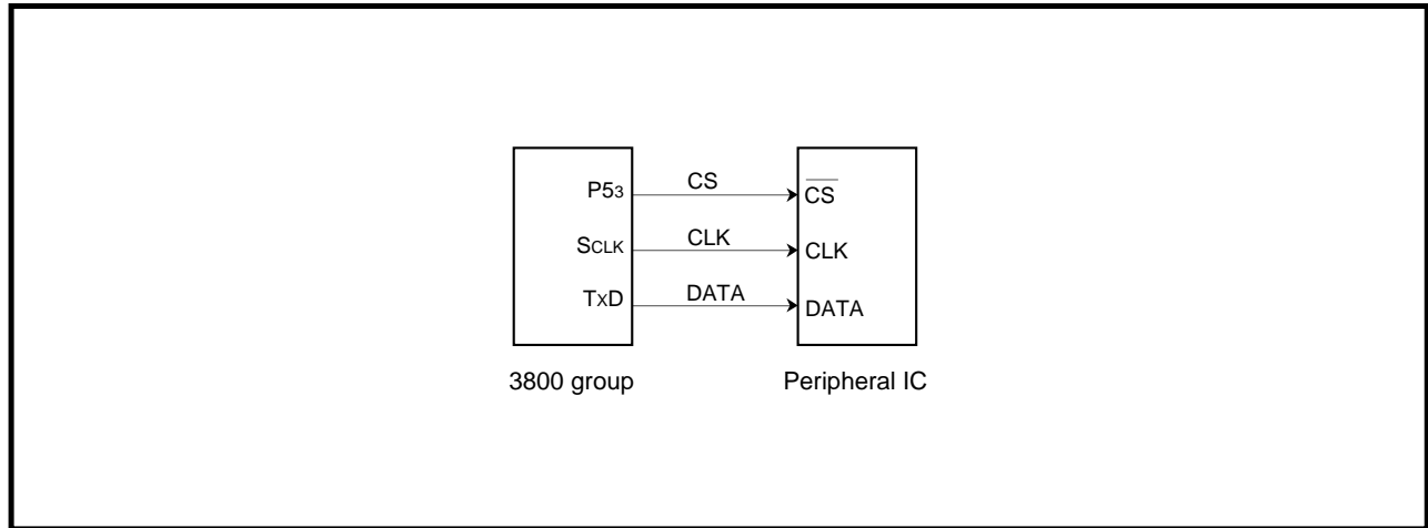
Fig. 2.3.19 Connection diagram [Output of serial data]
