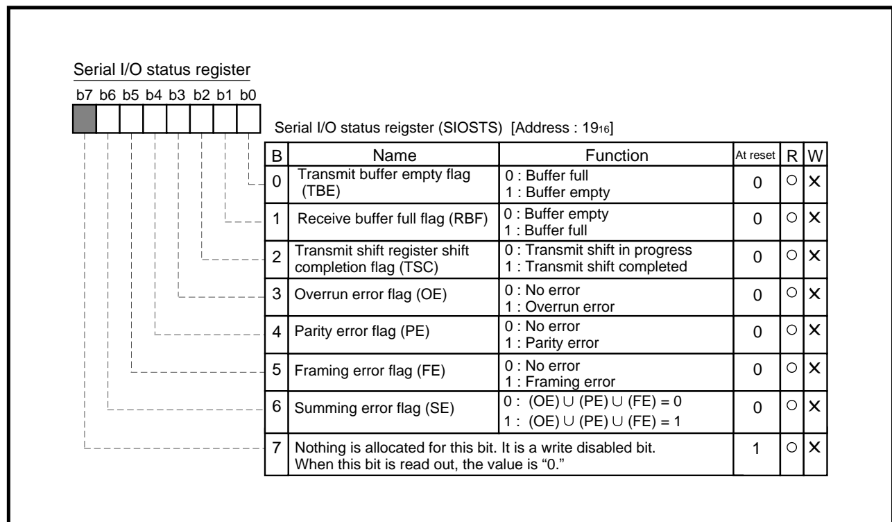
Fig. 3.5.4 Structure of Serial I/O status register
