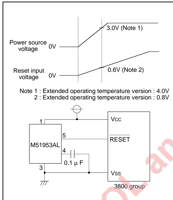
Fig. 22 Example of reset circuit
