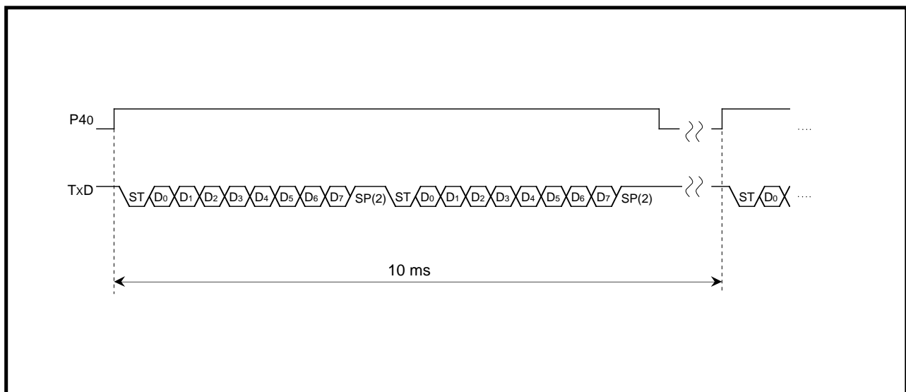
Fig. 2.3.30 Timing chart [Communication using UART]
