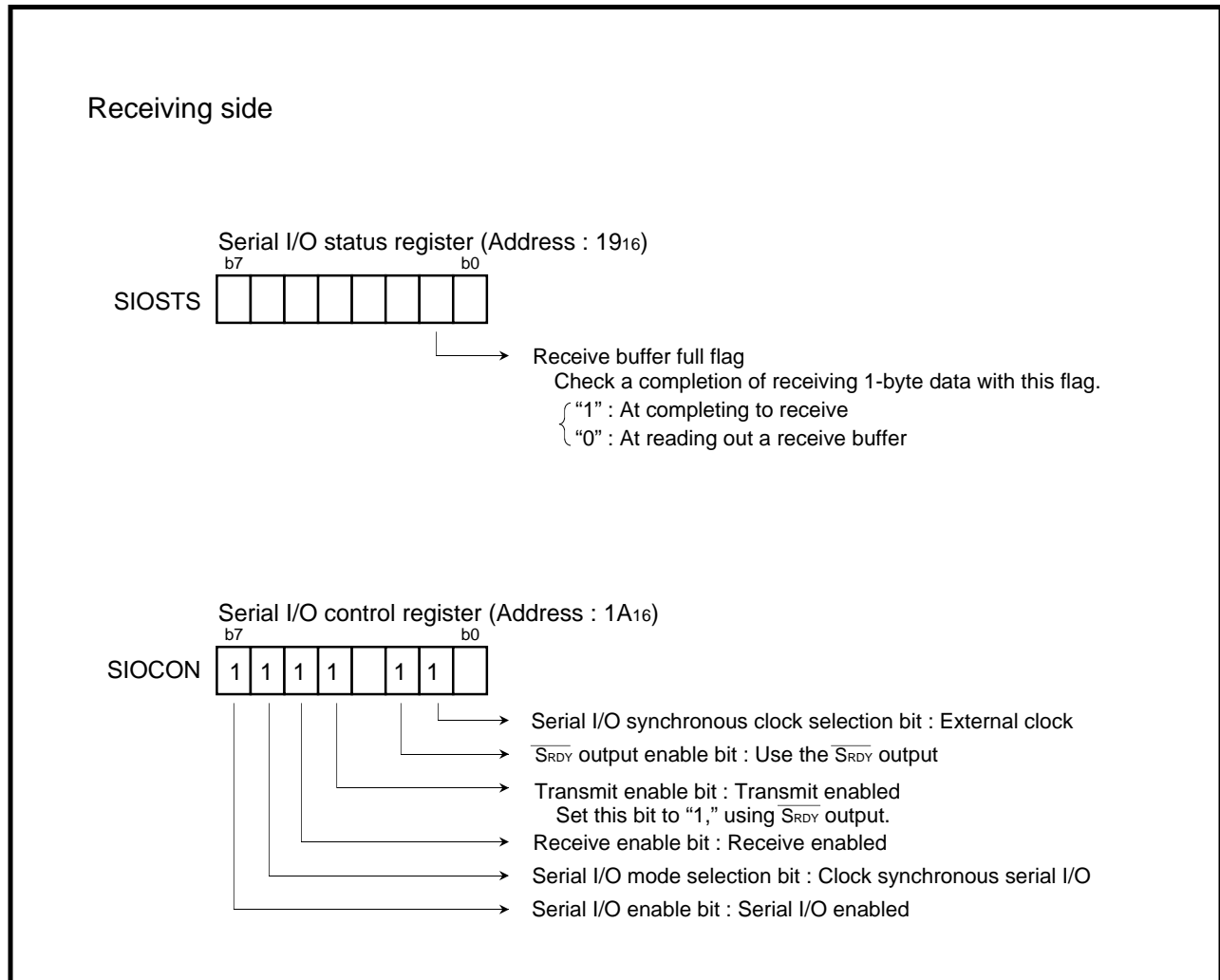
Fig. 2.3.16 Setting of related registers at a receiving side [Communication using a clock synchronous serial I/O]
