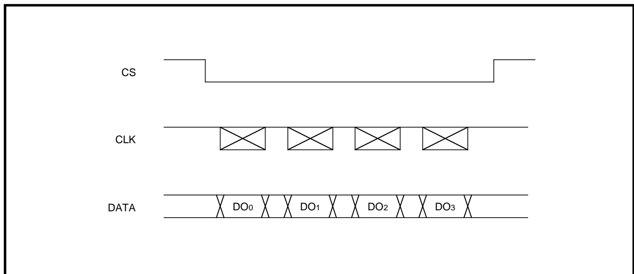
Fig. 2.3.20 Timing chart [Output of serial data]
