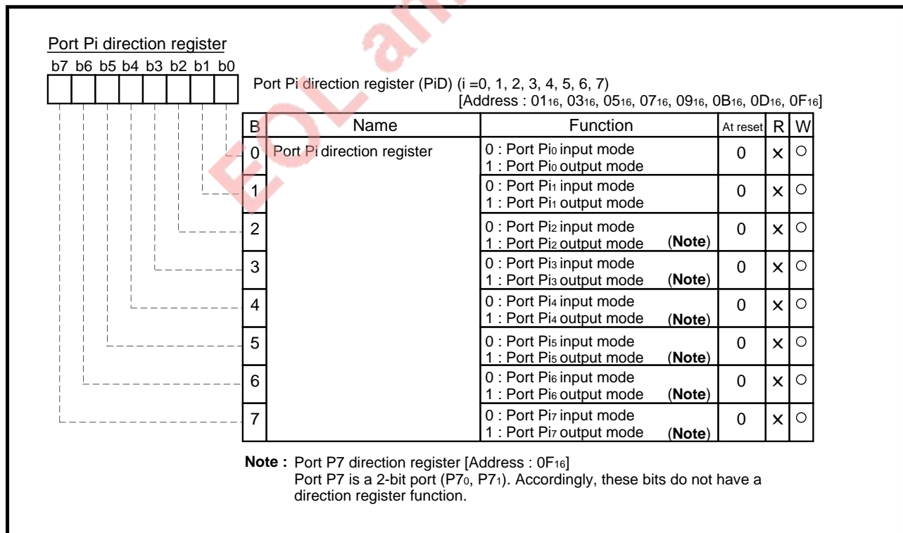
Fig. 3.5.2 Structure of Port Pi direction register (i = 0, 1, 2, 3, 4, 5, 6, 7)
