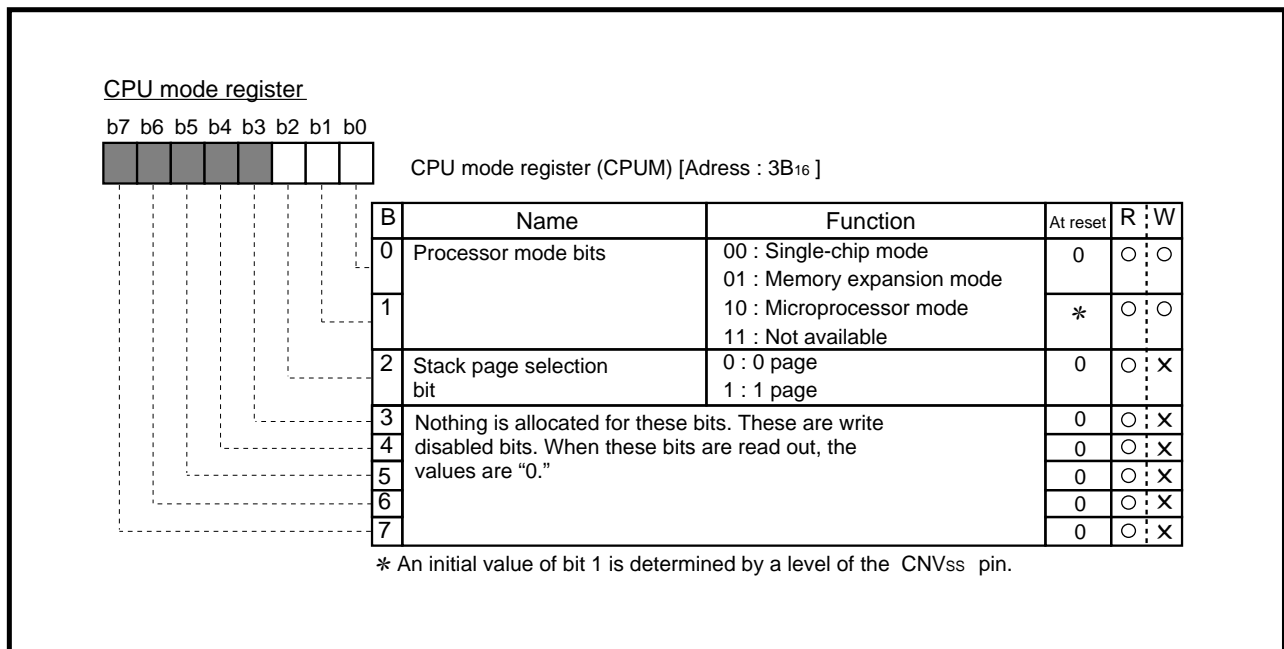
Fig. 2.4.2 Structure of CPU mode register
