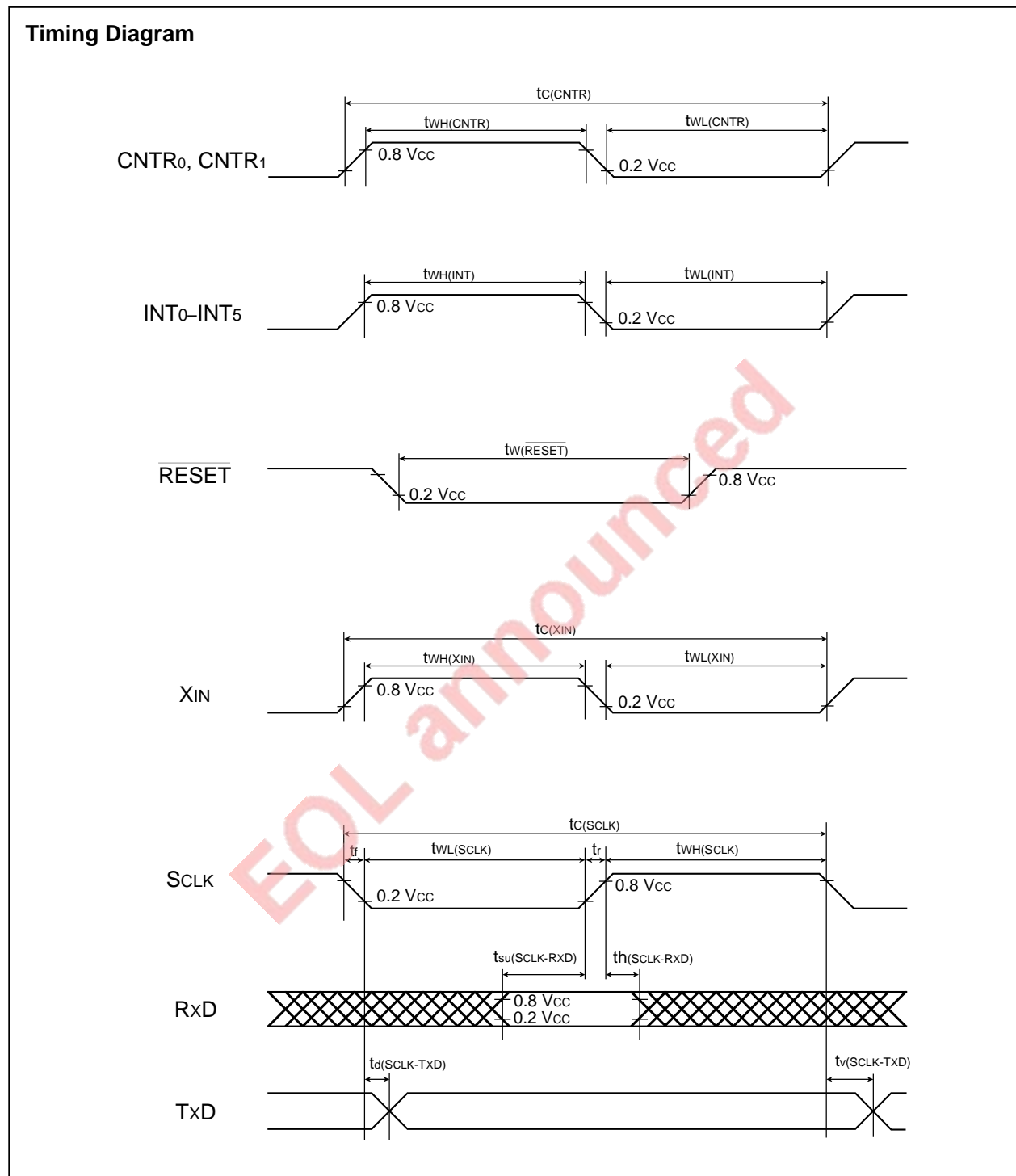
Fig. 3.1.2 Timing diagram (in single-chip mode)
