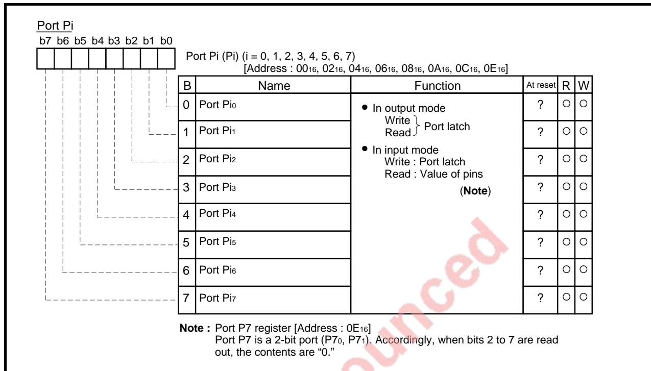
Fig. 2.1.2 Structure of Port Pi (i = 0, 1, 2, 3, 4, 5, 6, 7)
