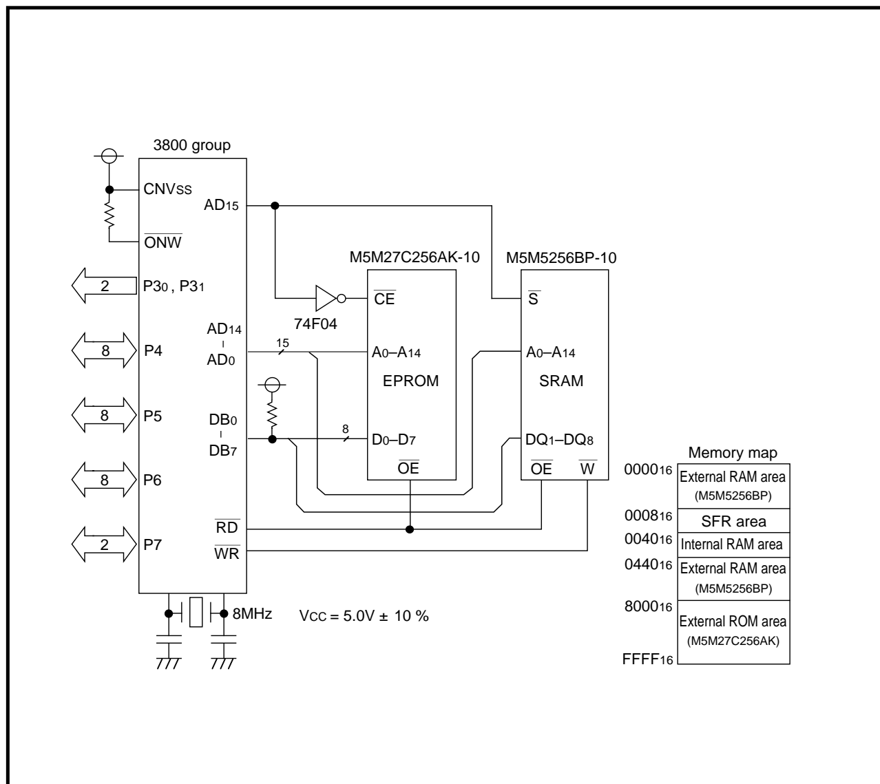
Fig. 2.4.3 Expansion example of ROM and RAM
