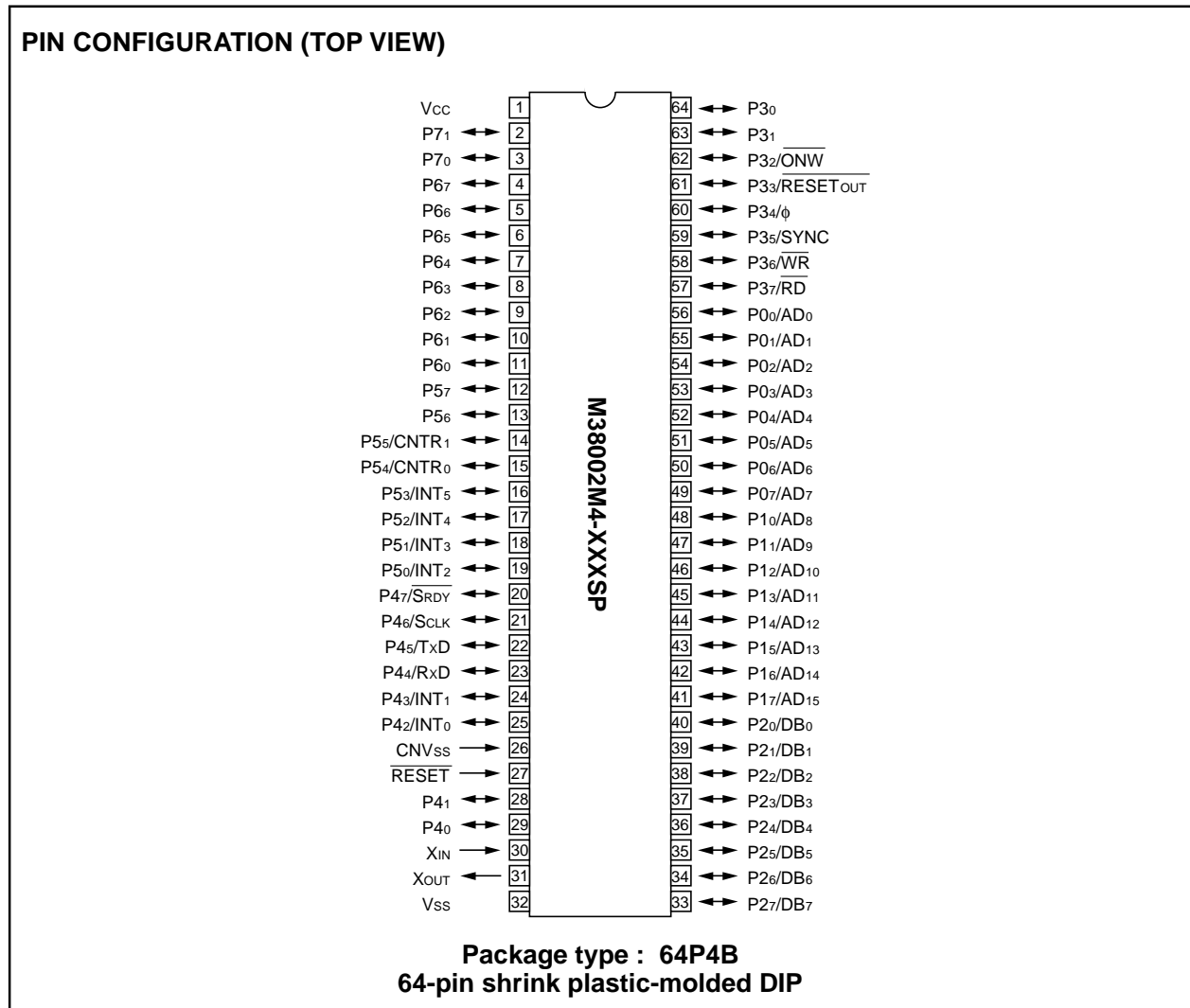
Fig. 2 Pin configuration of M38002M4-XXXSP
