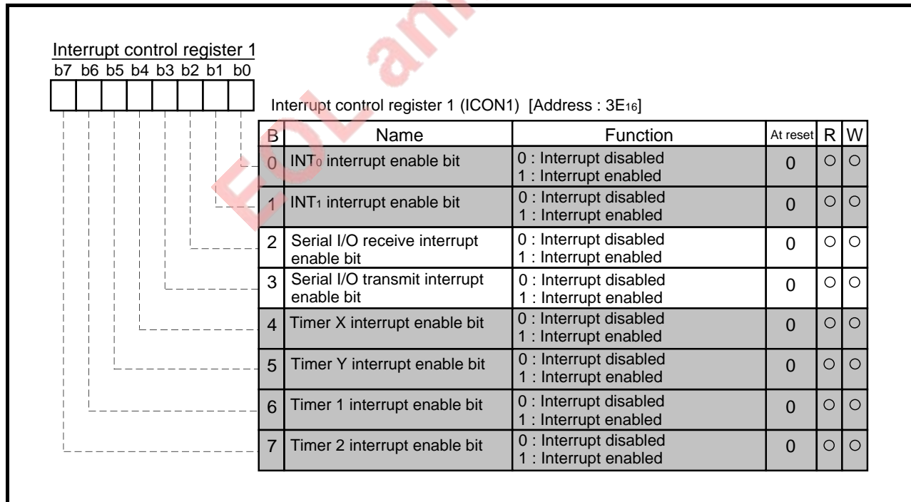
Fig. 2.3.9 Structure of Interrupt control register 1
