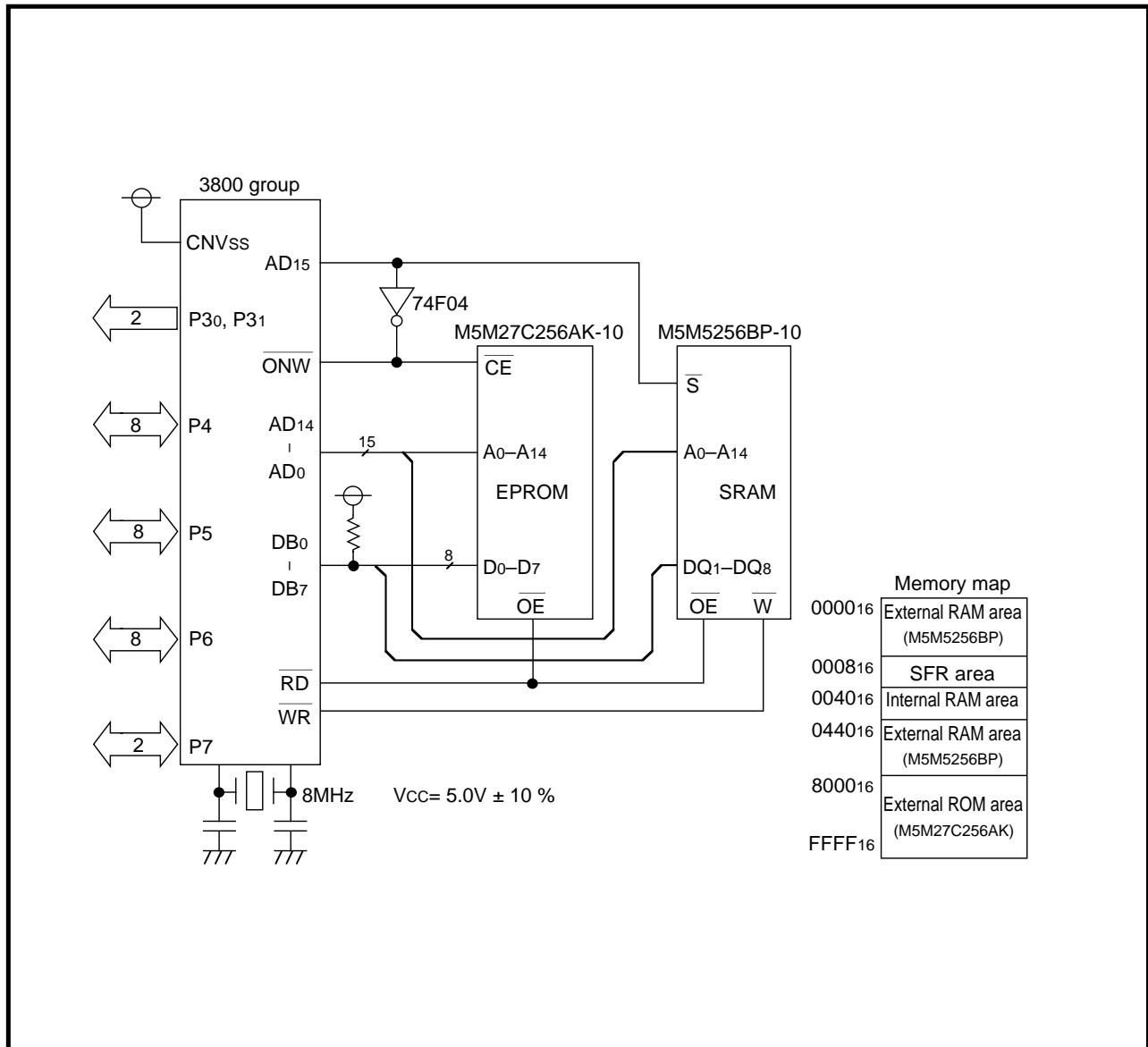
Fig. 2.4.7 Application example of the \overline{\text{ONW}} function
