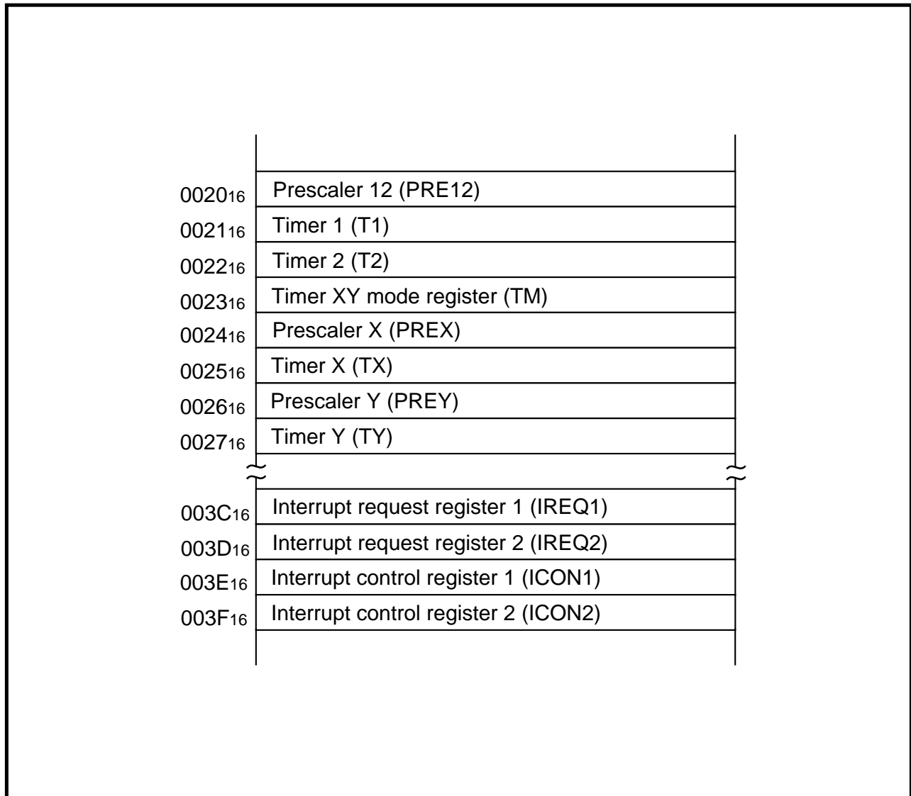
Fig. 2.2.1 Memory map of timer related registers
