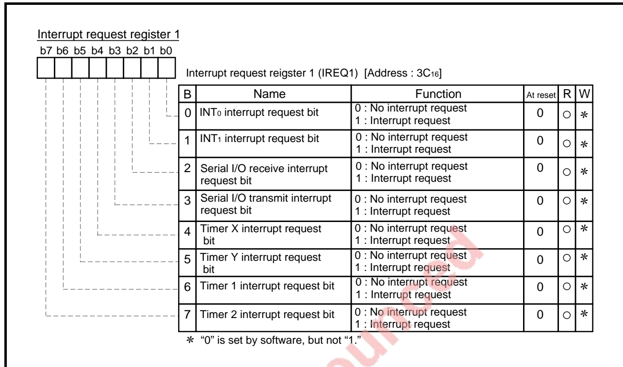
Fig. 3.5.14 Structure of Interrupt request register 1
