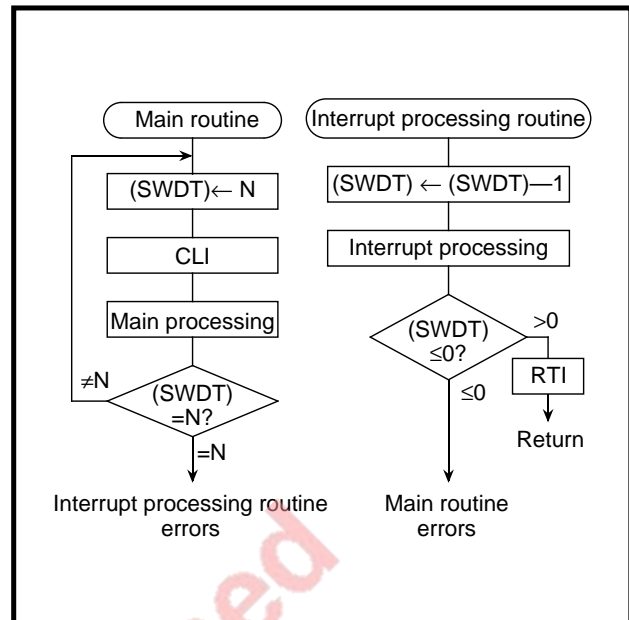
Fig. 3.4.8 Watchdog timer by software
