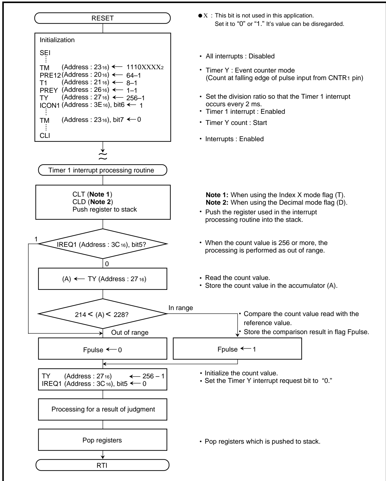
Fig. 2.2.19 Control procedure [Measurement of frequency]
