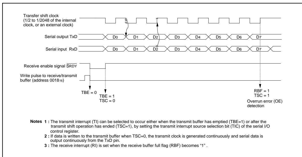
Fig. 18 Operation of clock synchronous serial I/O function
