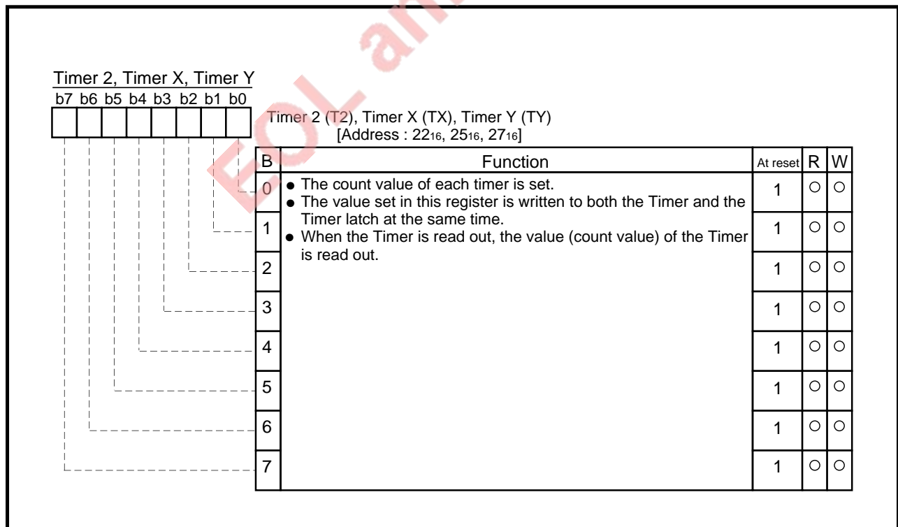
Fig. 3.5.10 Structure of Timer 2, Timer X, Timer Y
