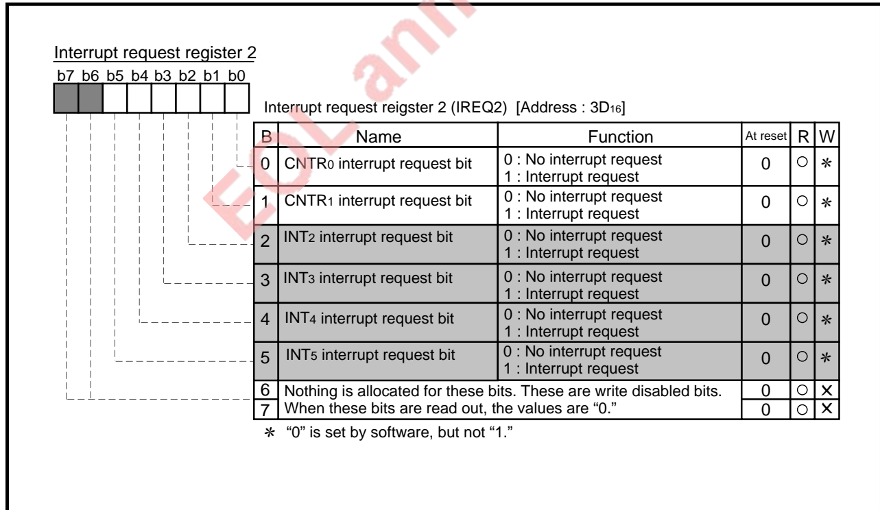
Fig. 2.2.7 Structure of Interrupt request register 2
