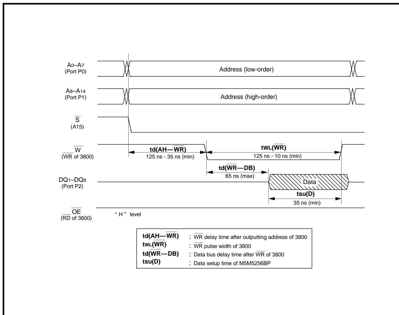
Fig. 2.4.6 Write-cycle (W control, SRAM)
