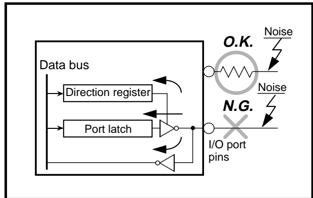
Fig. 3.4.7 Setup for I/O ports
