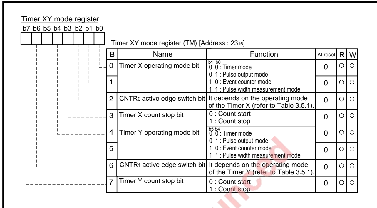
Fig. 3.5.11 Structure of Timer XY mode register
