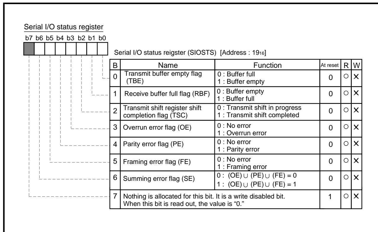
Fig. 2.3.3 Structure of Serial I/O status register
