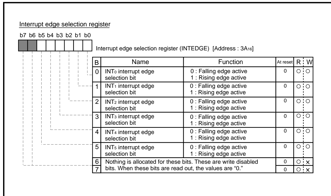
Fig. 3.5.12 Structure of Interrupt edge selection register
