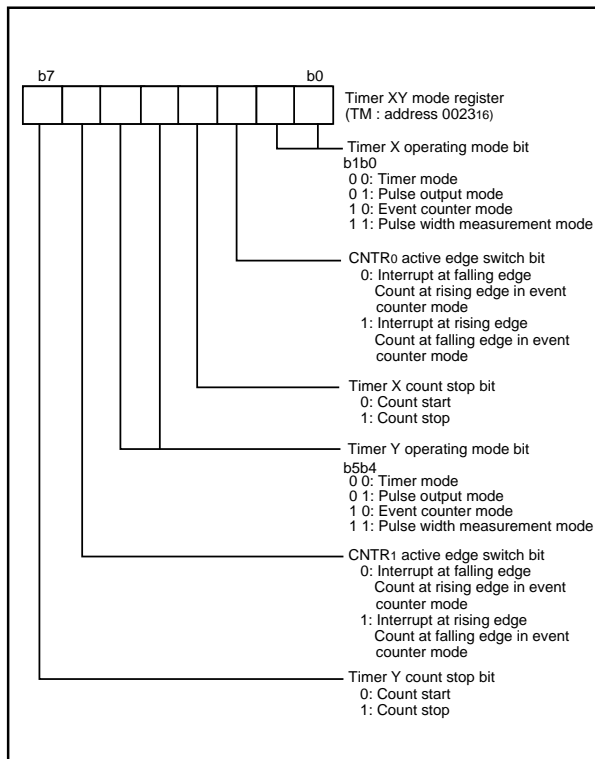
Fig. 15 Structure of timer XY register
