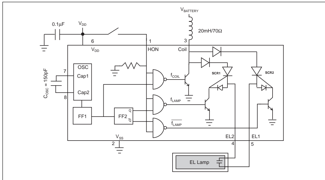
SP4423 Schematic
