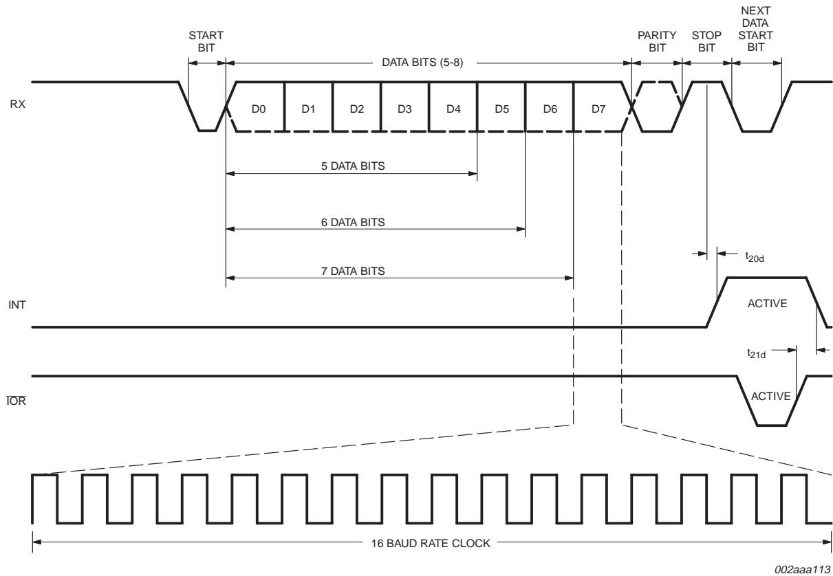
Fig 11. Receive timing.
