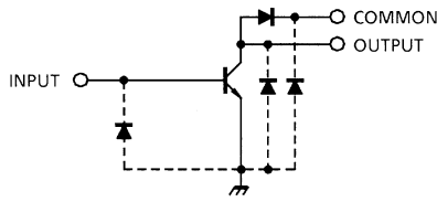
TD62595APG, TD62595AFG
