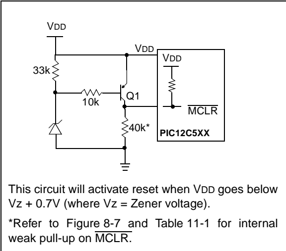
FIGURE 8-13: BROWN-OUT PROTECTION CIRCUIT 1
