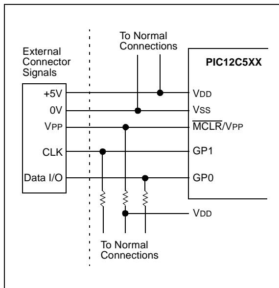
FIGURE 8-16: TYPICAL IN-CIRCUIT SERIAL PROGRAMMING CONNECTION
