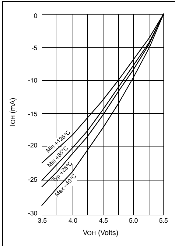
FIGURE 12-6: I_{OH} vs. V_{OH} , V_{DD} = 5.5 V
