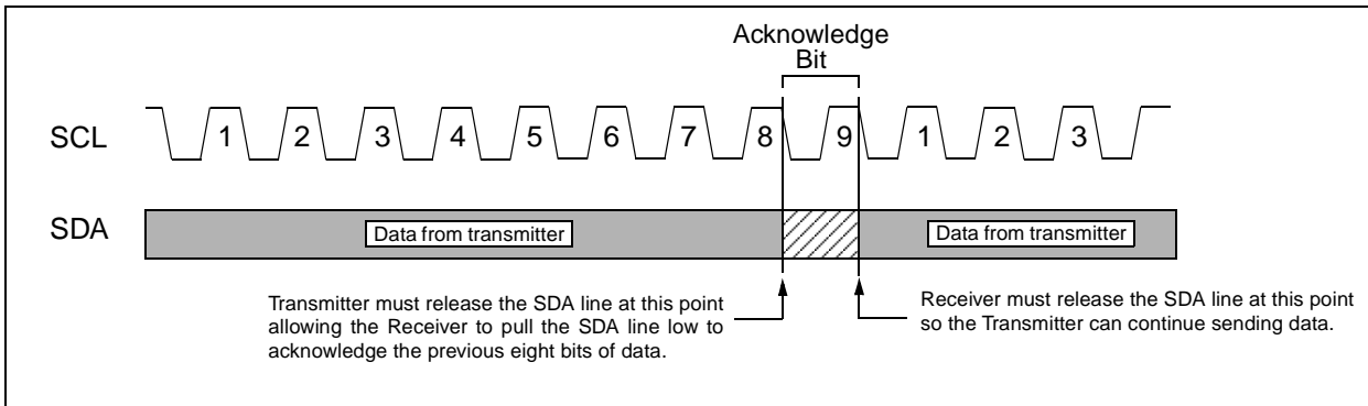
FIGURE 7-4: ACKNOWLEDGE TIMING
