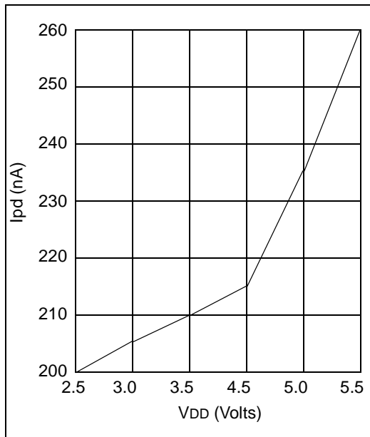
FIGURE 14-13: TYPICAL IPD VS. V DD , WATCHDOG DISABLED (25°C)
