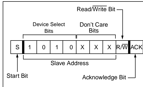
FIGURE 7-5: CONTROL BYTE FORMAT
