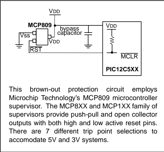
FIGURE 8-15: BROWN-OUT PROTECTION CIRCUIT 3
