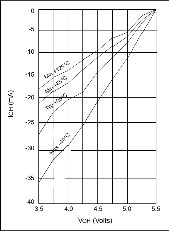
FIGURE 14-11: I_{OH} vs. V_{OH} , V_{DD} = 5.5\text{ V}
