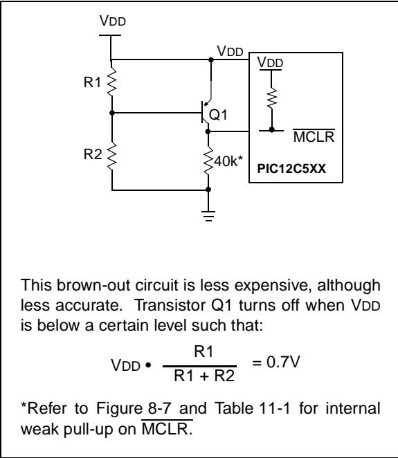
FIGURE 8-15: BROWN-OUT PROTECTION CIRCUIT 3
