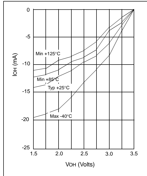
FIGURE 14-8: I_{OH} vs. V_{OH} , V_{DD} = 3.5 \text{ V}
