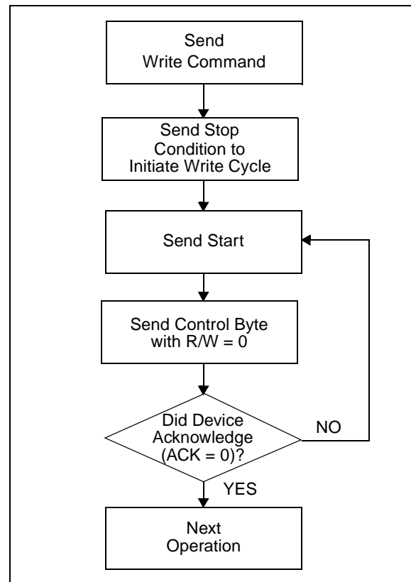
FIGURE 7-6: ACKNOWLEDGE POLLING FLOW
