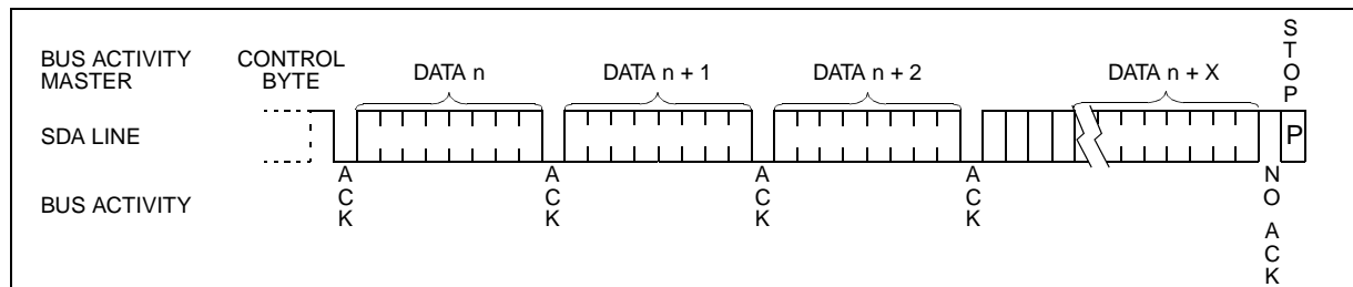
FIGURE 7-10: SEQUENTIAL READ
