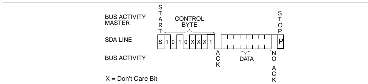
FIGURE 7-9: RANDOM READ
