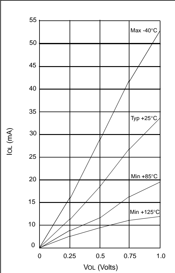
FIGURE 14-12: I_{OL} vs. V_{OL} , V_{DD} = 5.5\text{ V}
