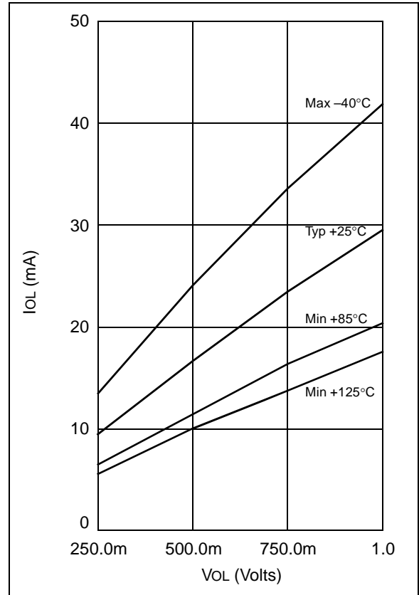
FIGURE 12-8: I_{OL} vs. V_{OL} , V_{DD} = 5.5 V
