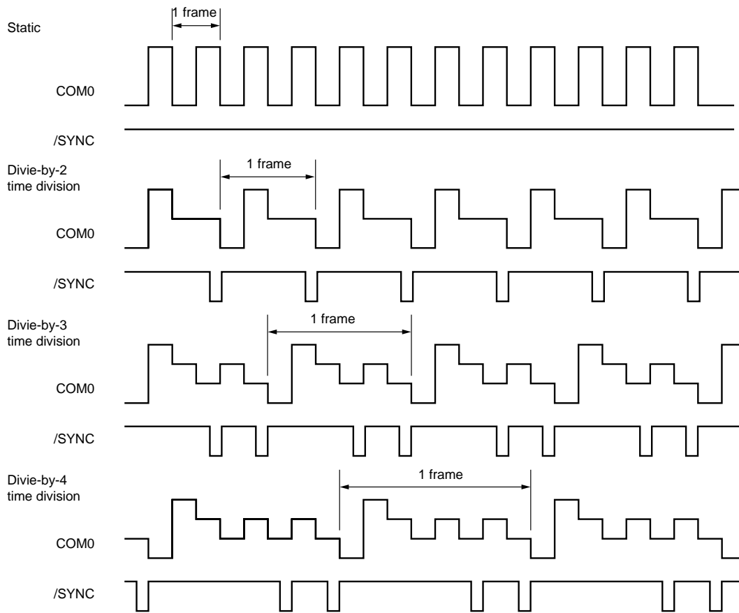
Figure 1-2. /SYNC Pin Status after Reset (/RESET = 1)
