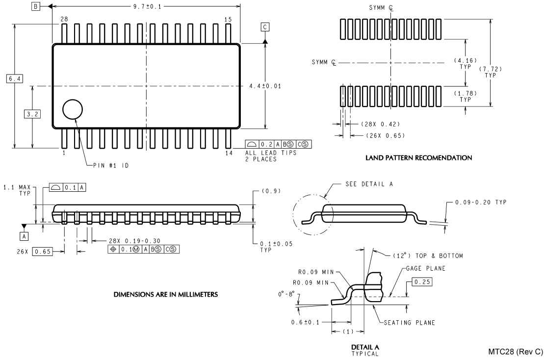
TSSOP Package Order Number LM4836MT NS Package Number MTC28 for TSSOP
