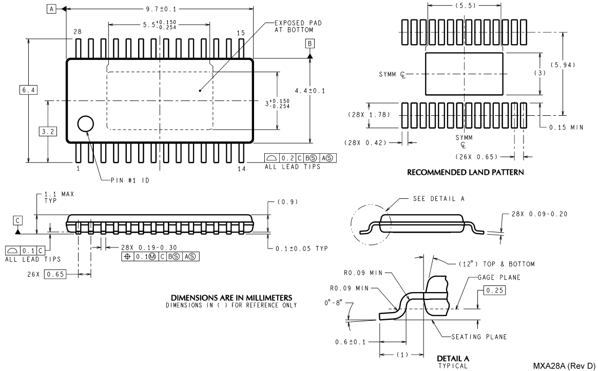
Exposed-DAP TSSOP Package Order Number LM4836MTE NS Package Number MXA28A for Exposed-DAP TSSOP
