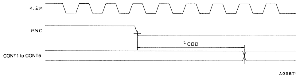
Figure 5 General-Purpose Port Output Timing
