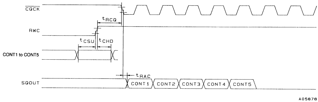
Figure 4 General-Purpose Port Input Timing
