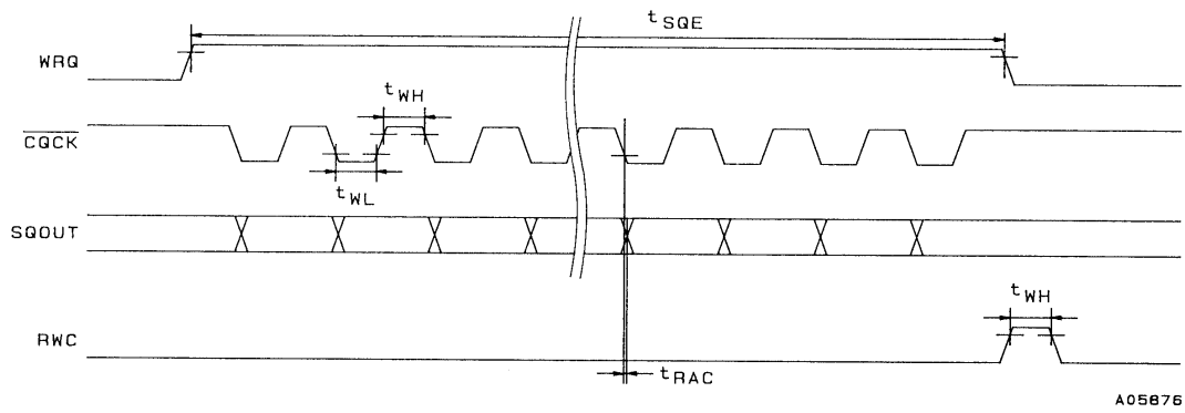
Figure 2 Subcode Q Output
