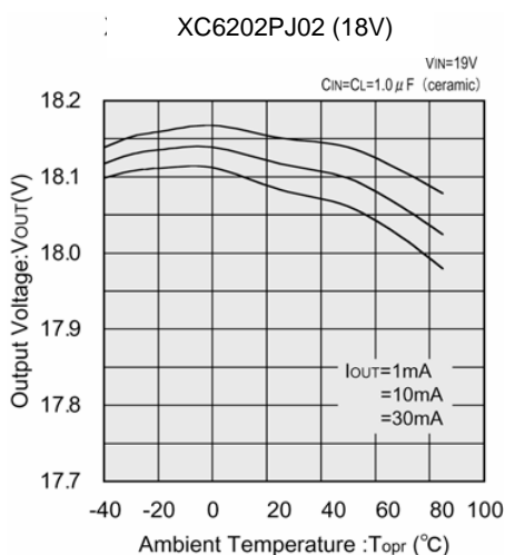
(5) Output Voltage vs. Ambient Temperature
