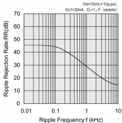
XC6202PC02 (12V)
