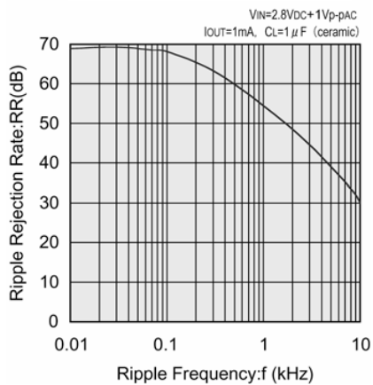
XC6202P182 (1.8V)
