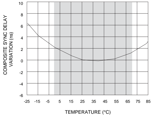
Fig. 7 Composite Sync Delay Variation vs Temperature
