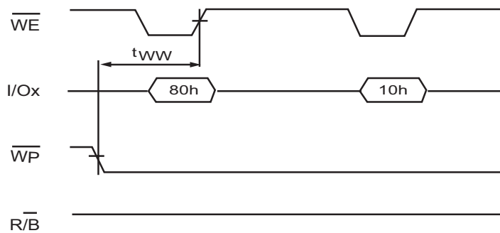
Figure 30: Disable Programming
