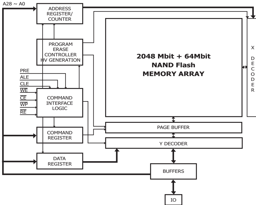
Figure 4: Block Diagram
