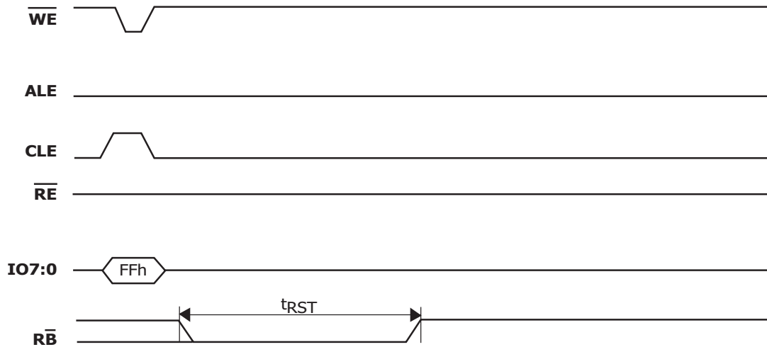
Figure 24: Reset Operation
