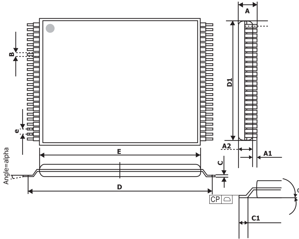
Figure 34. 48pin-USOP1, 12 x 17mm, Package Outline
