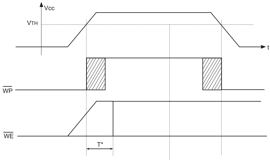
Figure 25: Power On/Off Timing
