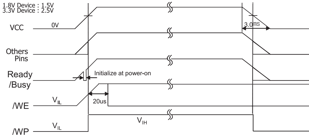
Figure 35: Power-on/off sequence
