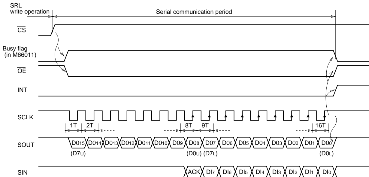
Serial Communication Timing Chart
