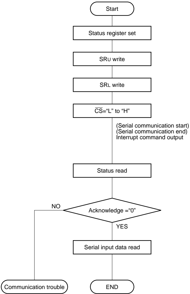
When INT Output Is Used
