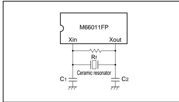
Clock Oscillation Circuit
