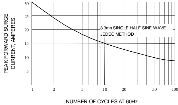
Fig. 3-MAXIMUM NON-REPETITIVE SURGE CURRENT
