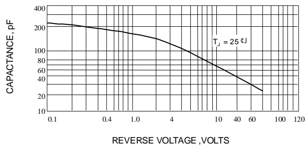
Fig. 4-TYPICAL JUNCTION CAPACITANCE
