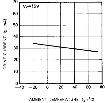
DRIVE CURRENT VS. AMBIENT TEMPERATURE
