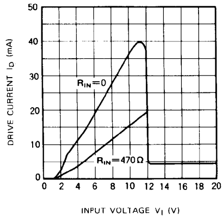
Fig. 2 DRIVE CURRENT VS. INPUT VOLTAGE
