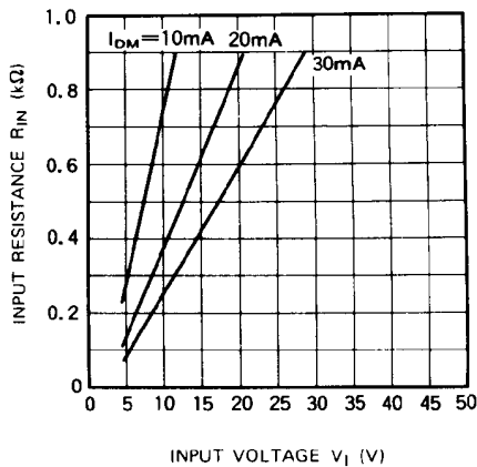
Fig. 1 MAXIMUM DRIVE CURRENT
