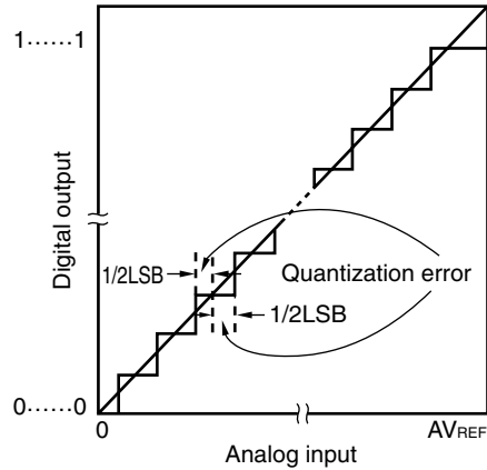
Figure 13-9. Quantization Error
