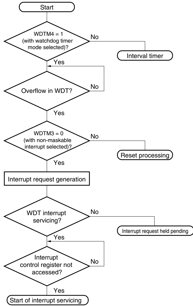
Figure 19-7. Non-Maskable Interrupt Request Generation to Acknowledge Flowchart
