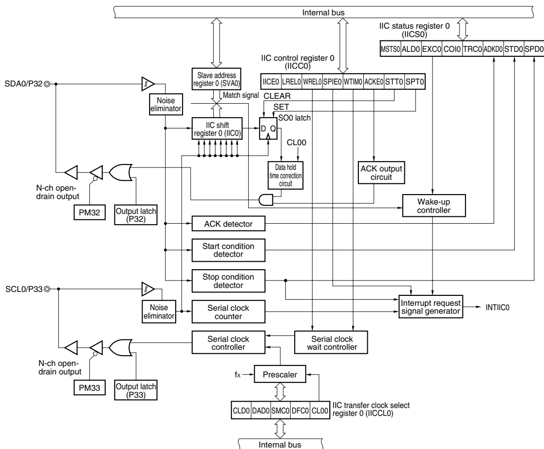
Figure 18-1. Block Diagram of Serial Interface IIC0
