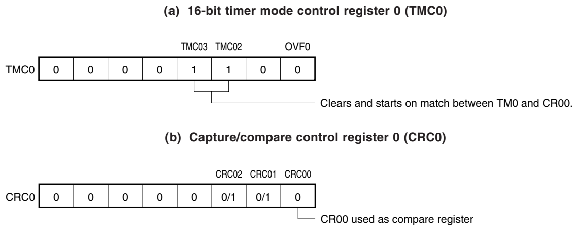
Figure 8-11. Control Register Settings in External Event Counter Mode
