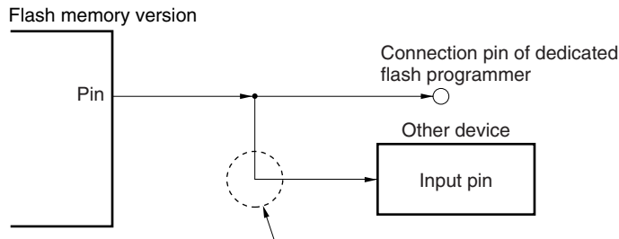
Figure 23-7. Abnormal Operation of Other Device
