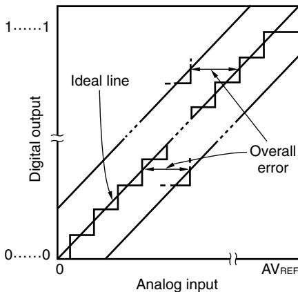
Figure 14-9. Overall Error
