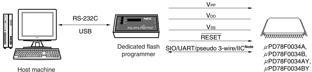
Figure 23-2. Environment for Writing Program to Flash Memory
