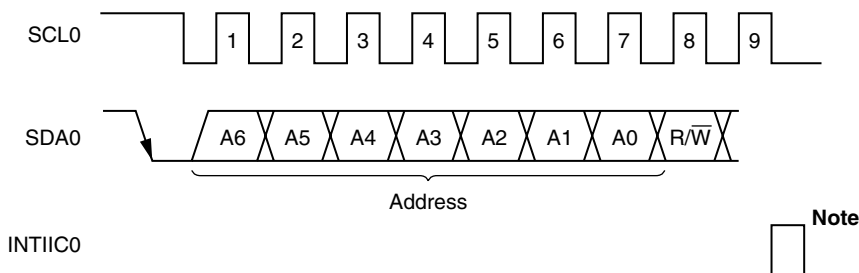
Figure 18-12. Address
