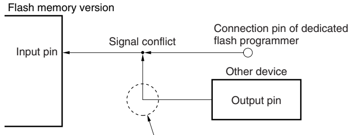
Figure 23-6. Signal Conflict (Input Pin of Serial Interface)
