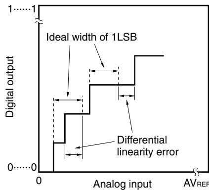
Figure 14-14. Differential Linearity Error
