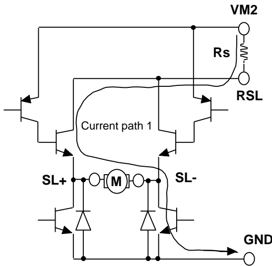
FORWARD Current path timing 1.
