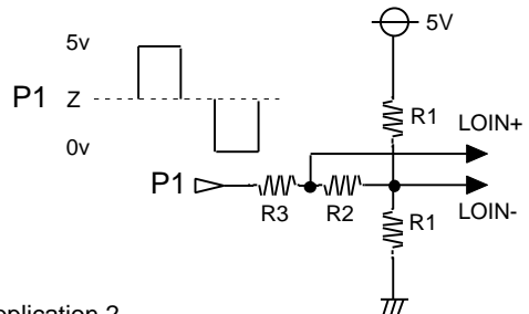
application.2 (One port H/Z/L control)
