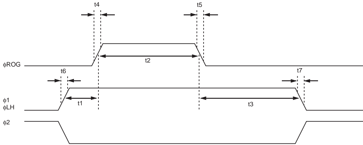
Clock Timing Chart 2
