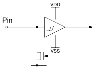
Fig. 3-7: I 2 C Interface SDA, SCL
