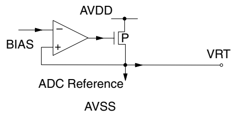
Fig. 3–11: Reference Voltage VRT
