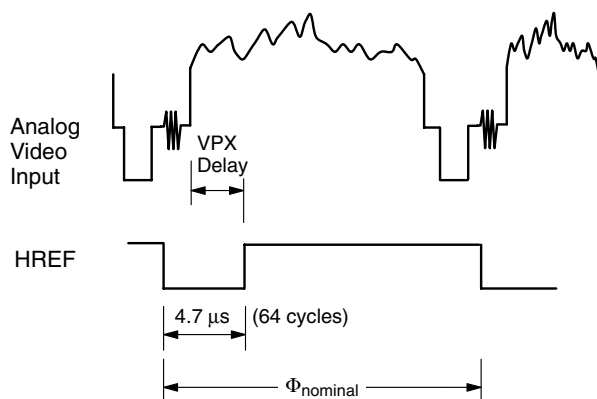
Fig. 2–27: HREF relative to input video
