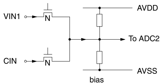
Fig. 3–13: Video Inputs ADC2
