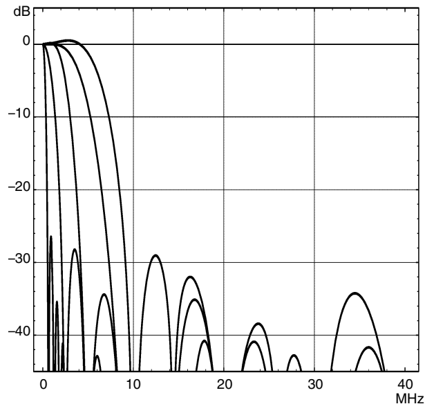
Fig. 2-13: Freq. response of 5 widely spaced filters
