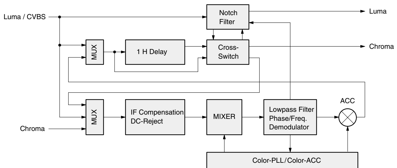
Fig. 2–5: Color decoder
