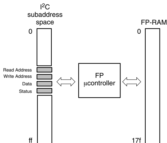
Fig. 2–40: FP register addressing
