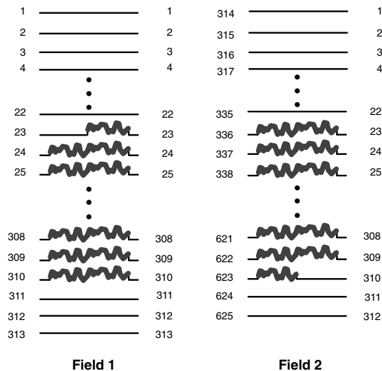
Fig. 2-35: Mapping for 625/50 line systems
