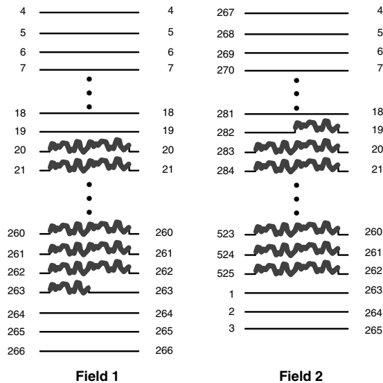
Fig. 2-34: Mapping for 525/60 line systems
