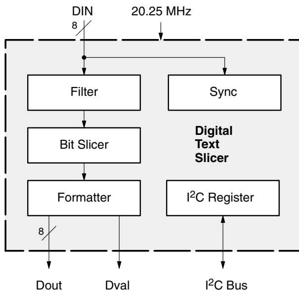
Fig. 2–36: Slicer block diagram
