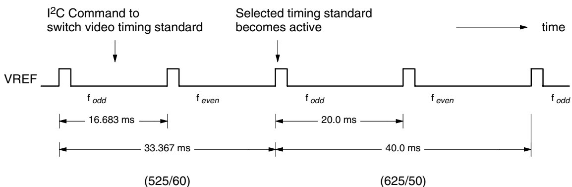
Fig. 2–31: Transition between timing standards
