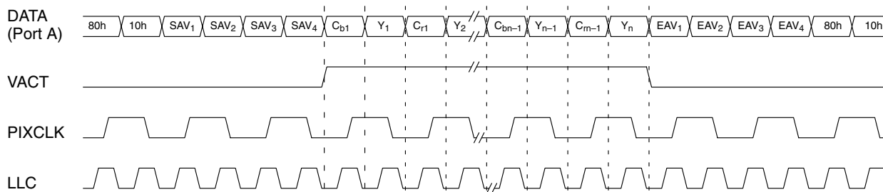
Fig. 2–20: Detailed data output (double clock mode)
