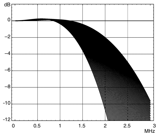
Fig. 2-14: Freq. response of 50 adjacent filters
