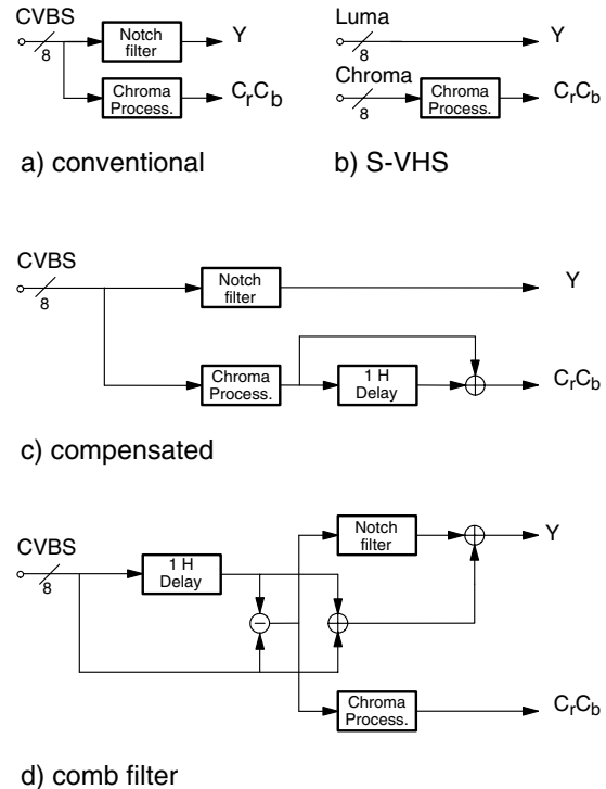
Fig. 2–7: NTSC color decoding options
