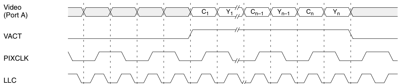
Fig. 2–25: Output timing in double clock mode
