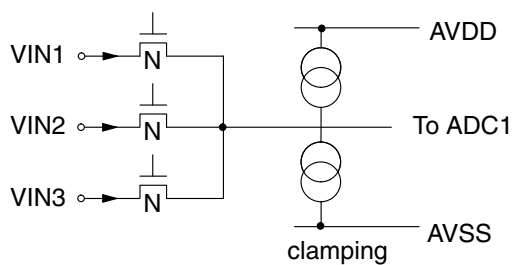
Fig. 3–12: Video Inputs ADC1
