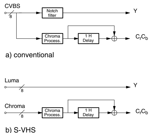
Fig. 2–8: PAL color decoding options
