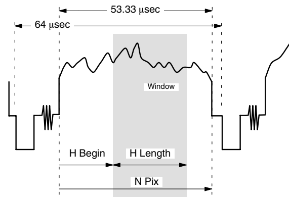
Fig. 2–33: Horizontal dimensions of sampling window
