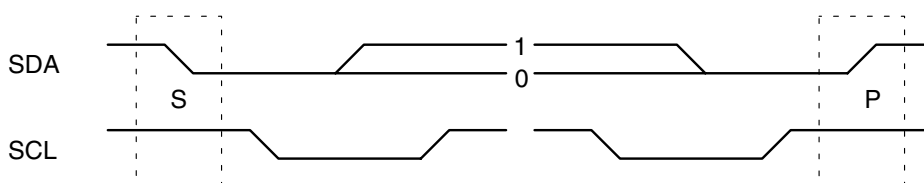
Fig. 2–41: I 2 C bus protocol (MSB first)
