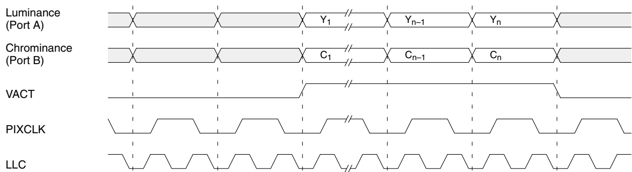
Fig. 2–24: Output timing in single clock mode
