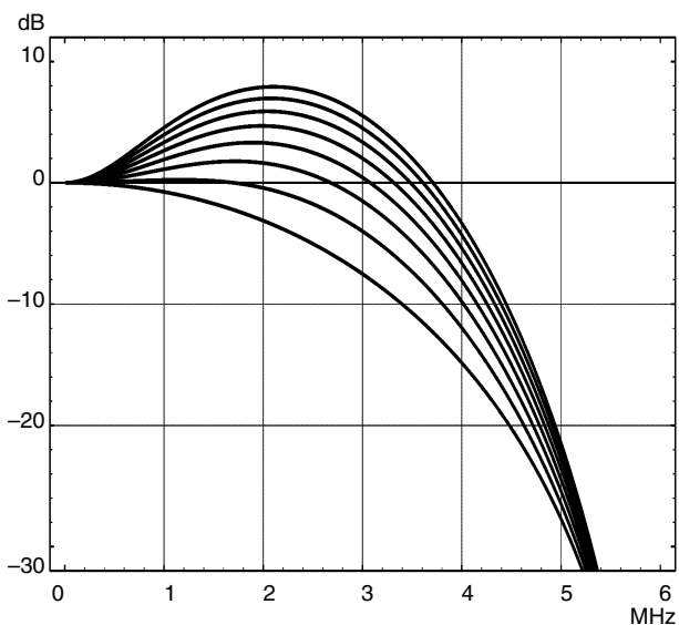
Fig. 2-15: Frequency response of peaking filter
