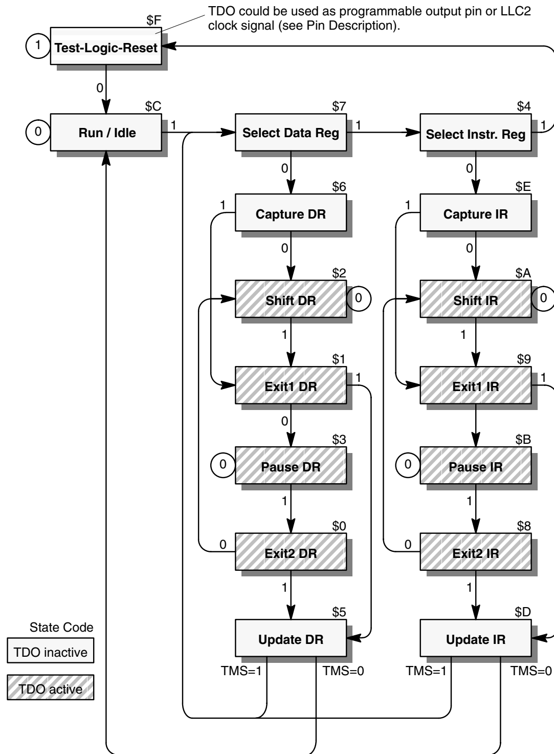
Fig. 2-43: TAP state transitions
