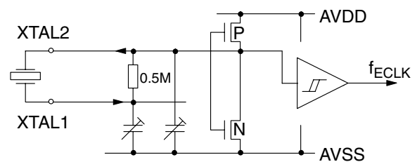
Fig. 3-10: Crystal Oscillator
