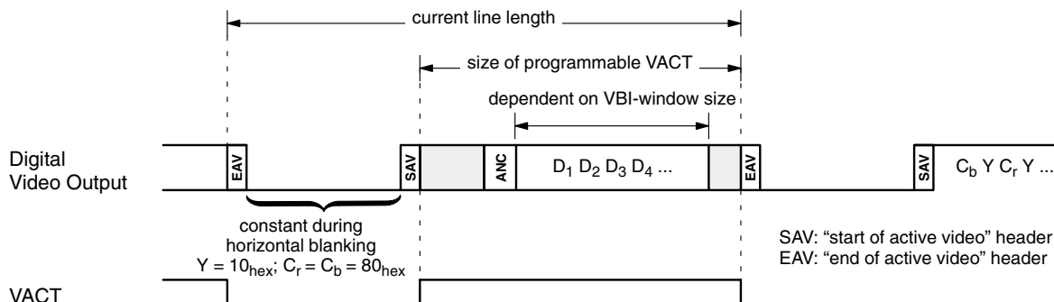
Fig. 2–21: Output of VBI-data as ancillary data
