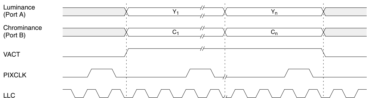
Fig. 2–26: Output timing in half clock mode
