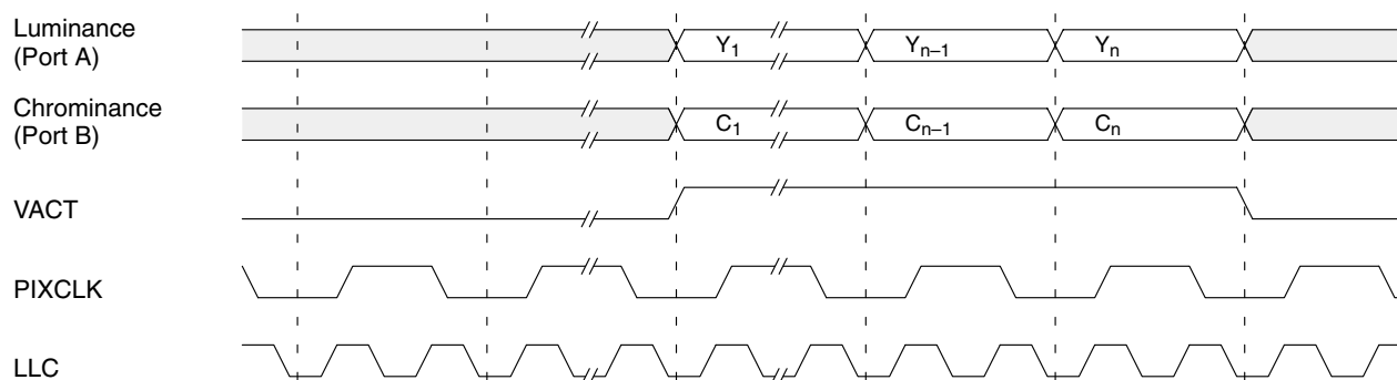
Fig. 2–18: Detailed data output (single clock mode)
