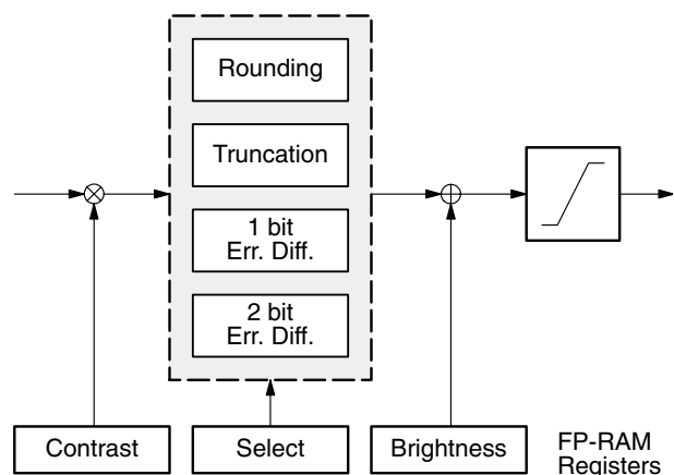
Fig. 2-16: Contrast and brightness adjustment
