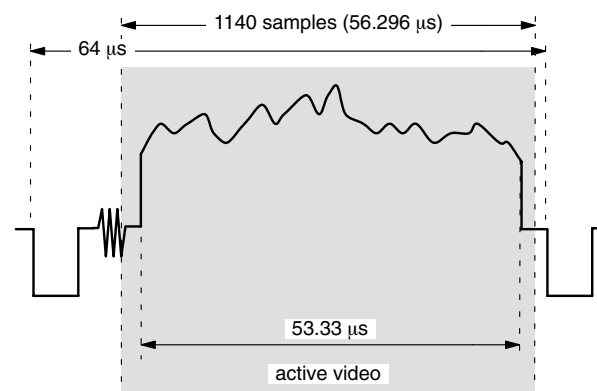
Fig. 2–38: Horizontal dimensions of the window for raw VBI-data
