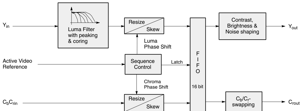
Fig. 2–12: Component processing stage
