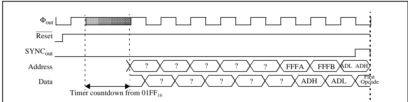
Fig. 1.99. Internal Processing Sequence after RESET
