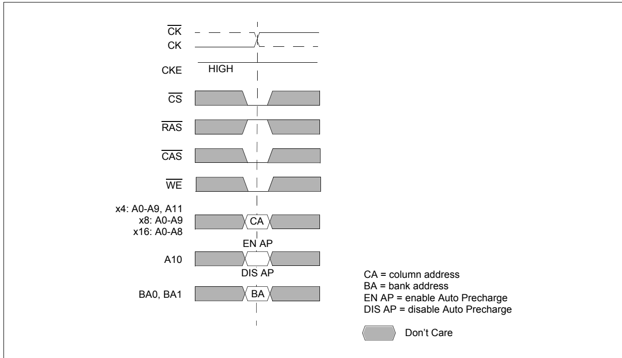
Figure 17 Write Command
