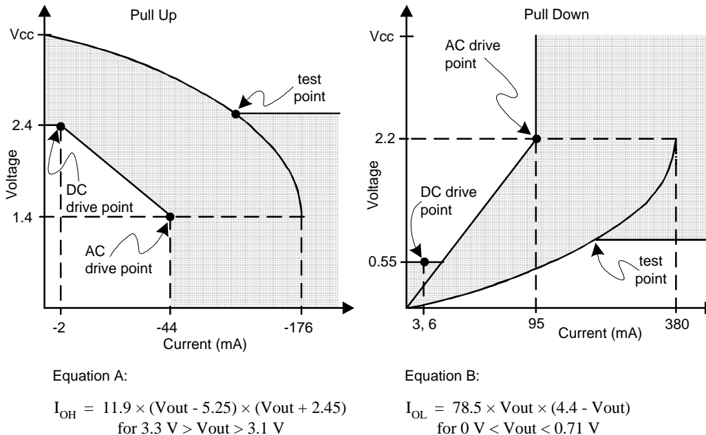
Figure 1. AC Characteristics
