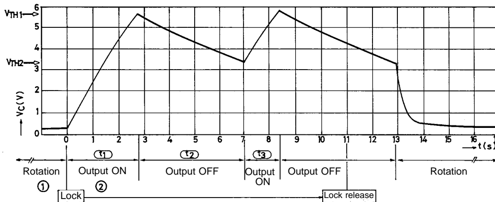
Automatic Return Circuit C Pin Voltage
