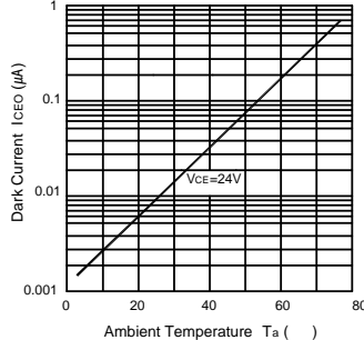
Dark Current vs. Ambient Temperature
