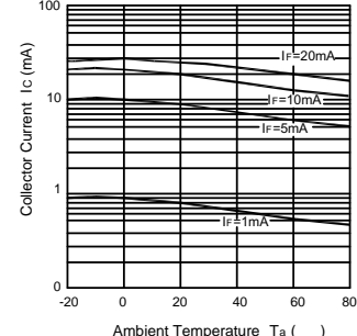
Collector Current vs. Ambient Temperature
