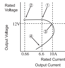
Fig2. Output Voltage/Current
