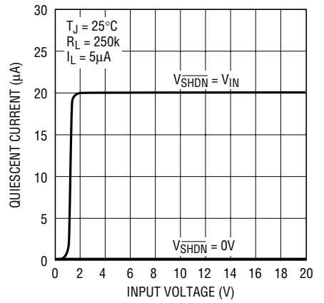
LT1761-BYP, LT1761-SD Quiescent Current
