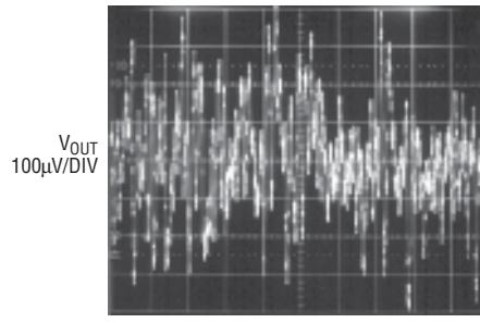
LT1761-5 10Hz to 100kHz Output Noise C_{BYYP} = 0
