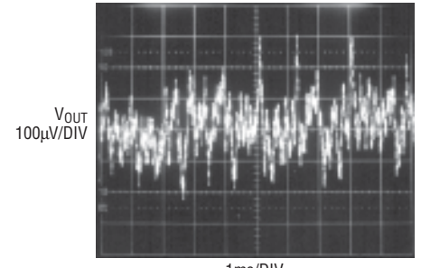
LT1761-5 10Hz to 100kHz Output Noise C_{BYYP} = 100\text{pF}
