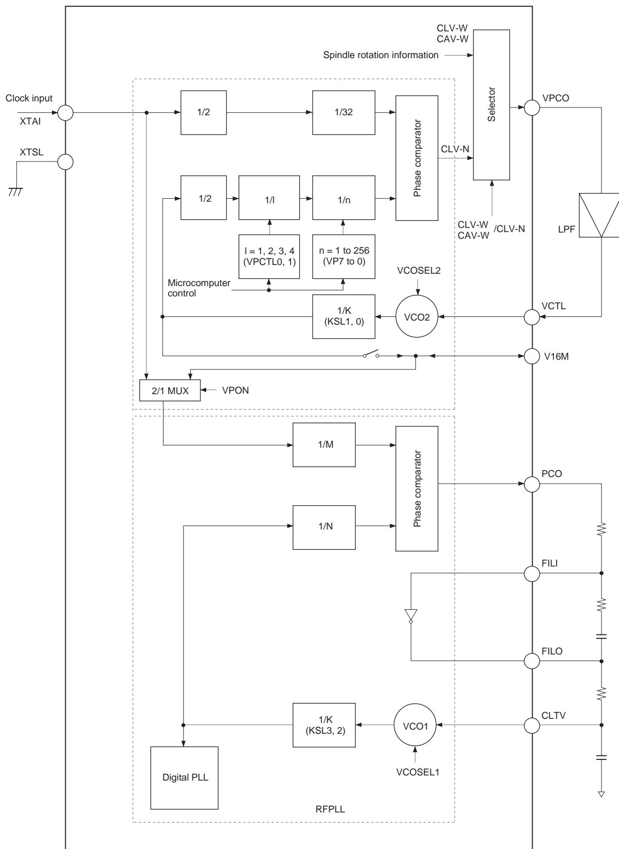
Block Diagram 4-1
