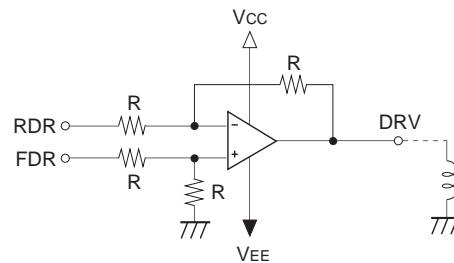
Fig. 5-21. Drive Circuit
