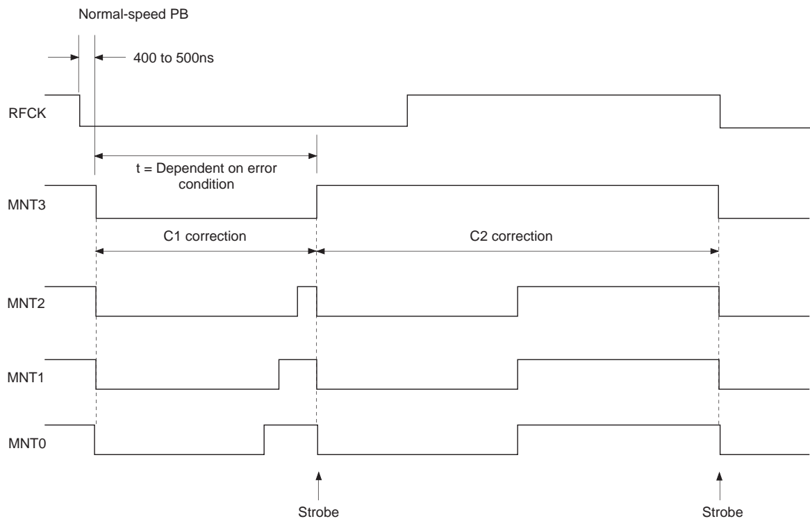
Timing Chart 4-3
