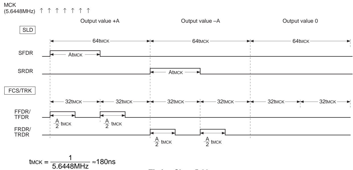
Timing Chart 5-20
