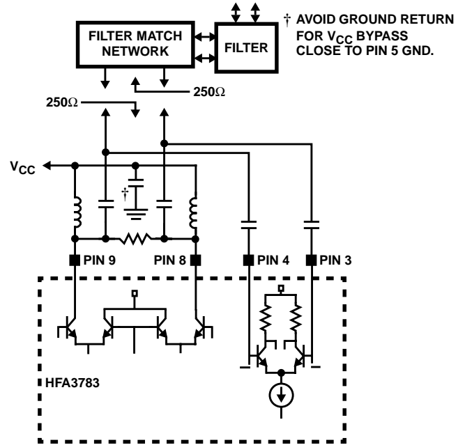
FIGURE 7. SIMPLIFIED IF INPUT/OUTPUT COMBINED MATCH NETWORK
