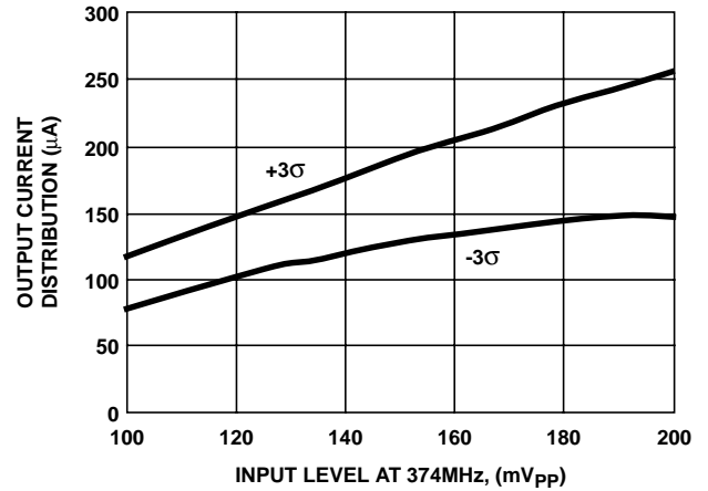
FIGURE 29. IF DETECTOR OUTPUT CURRENT, ±3 SIGMA DISTRIBUTION AT ALL TEMPERATURE AND V CC
