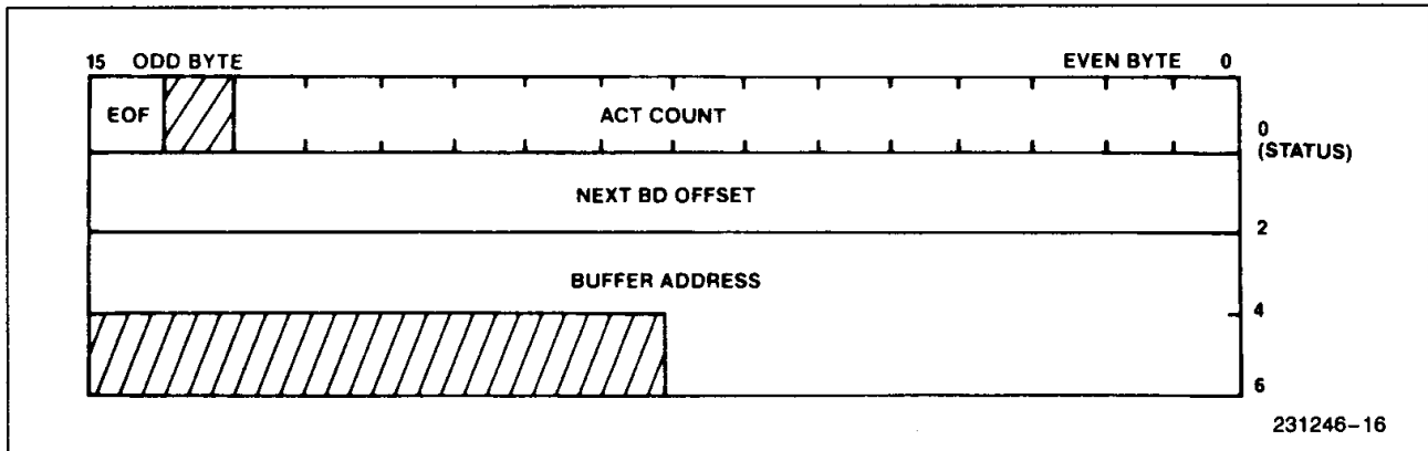
Figure 16. The Transmit Buffer Description
