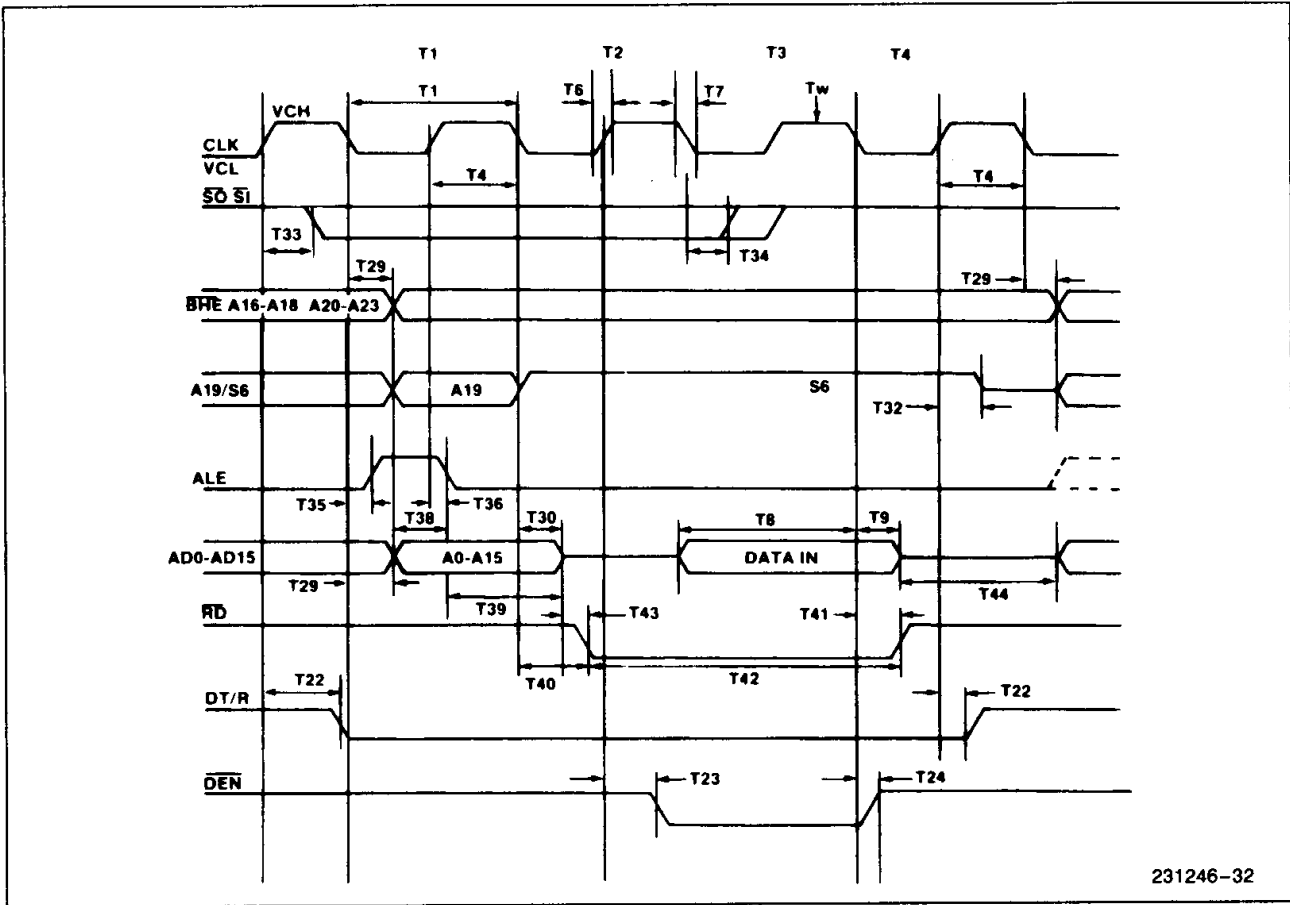
Figure 31. Read Cycle Timing
