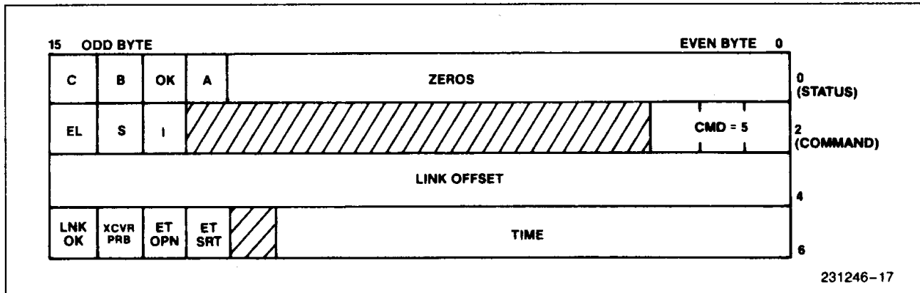
Figure 17. The TDR Command Block
