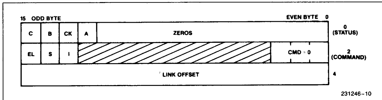
Figure 11. The NOP Command Block
