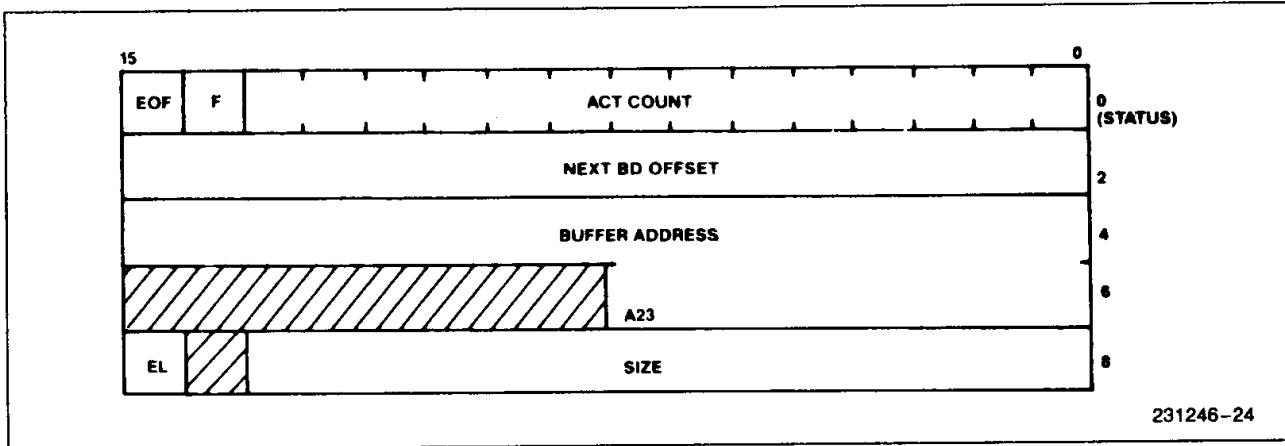
Figure 23. The Receive Buffer Descriptor (RBD) Format
