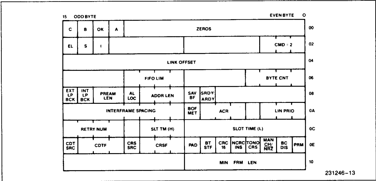
Figure 13. The CONFIGURE Command Block
