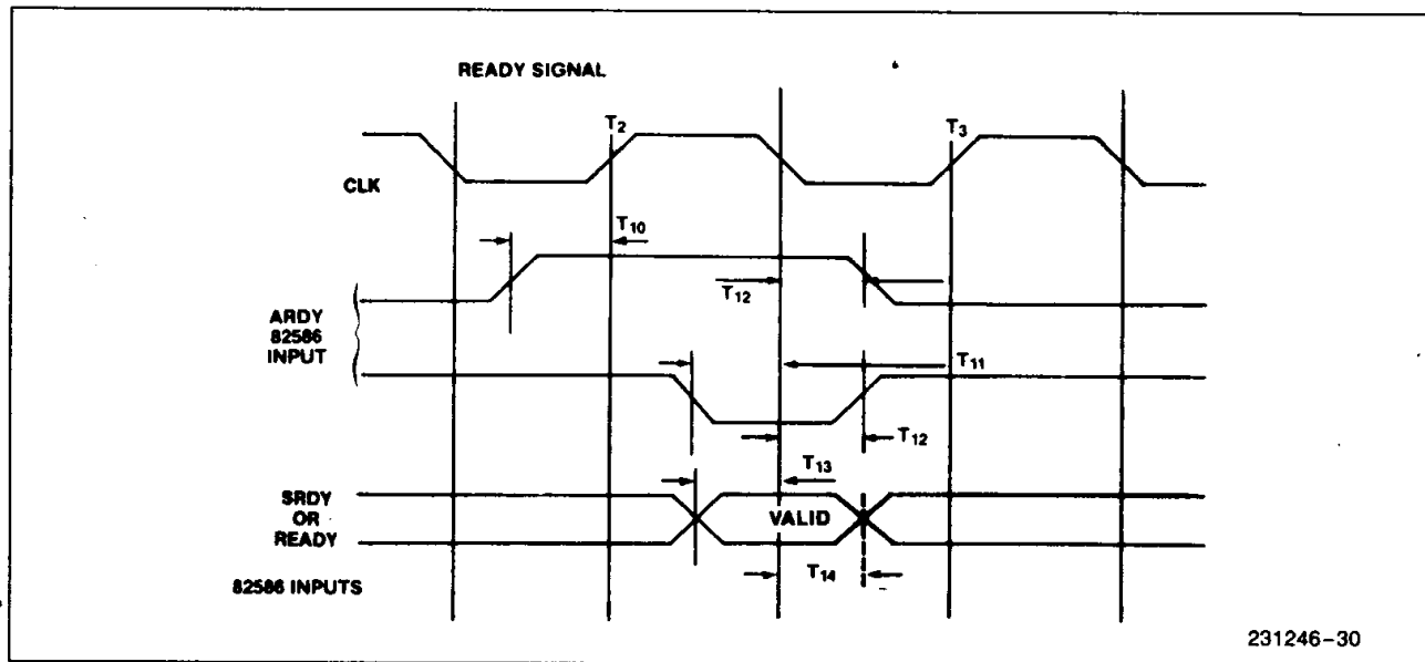
Figure 29. ARDY and SRDY Timings Relative to CLK
