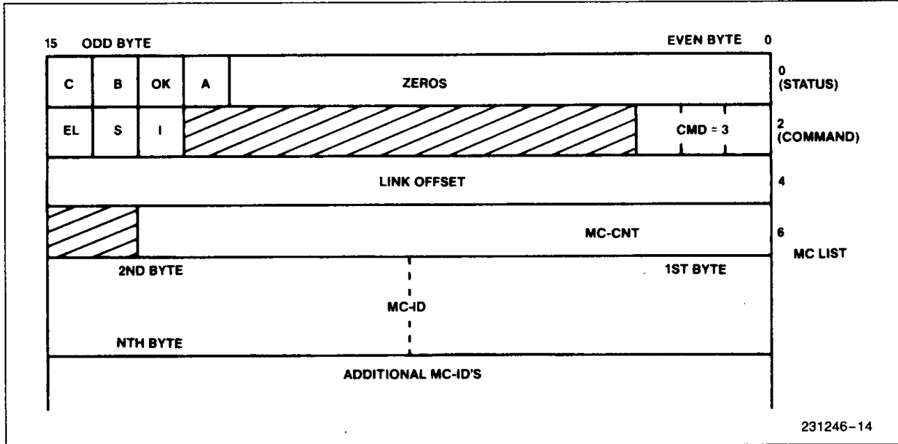
Figure 14. The MC-SETUP Command Block
