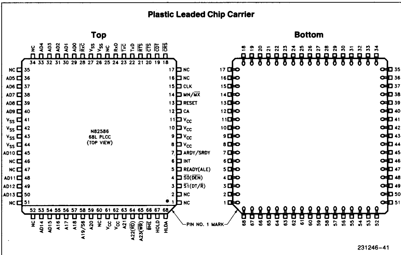
Figure 2. 82586 Pinout Diagrams
