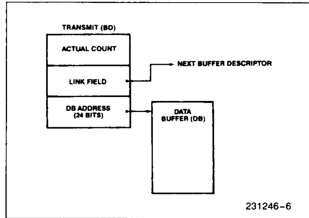
Figure 6. Data Buffer Descriptor and Data Buffer Structure
