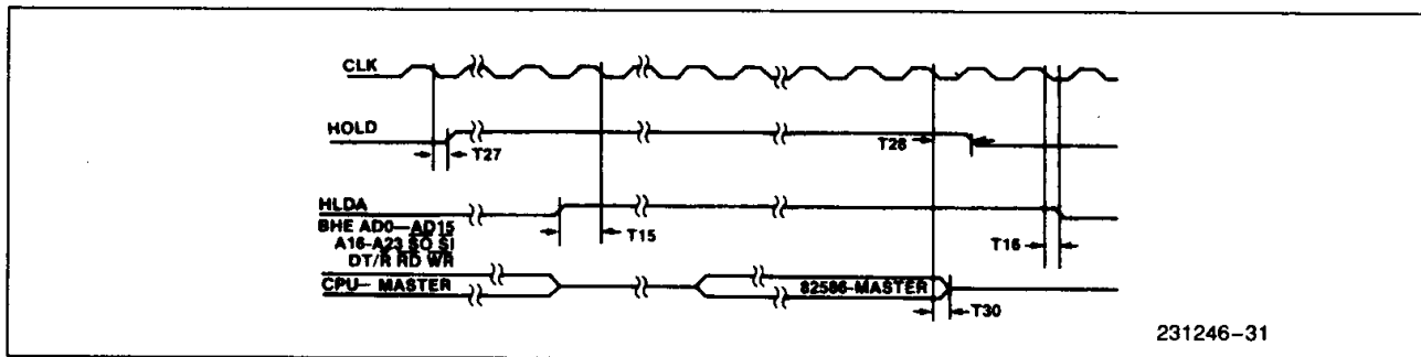
Figure 30. HOLD/HLDA Timing Relative to CLK
