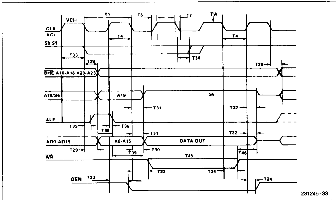
Figure 32. Write Cycle Timing
