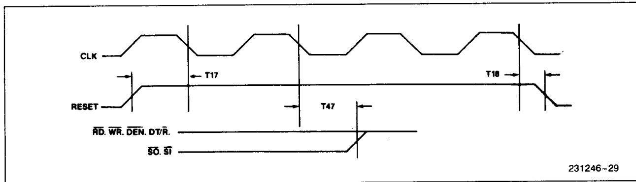
Figure 28. RESET Timing
