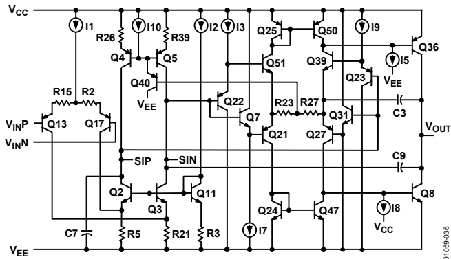
Figure 35. Simplified Schematic
