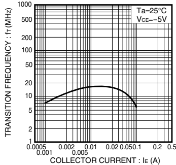
Fig.7 TRANSITION FREQUENCY vs. EMITTER CURRENT
