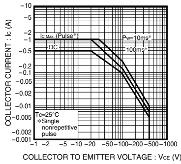
Fig. 11 Safe operating area (2SA1727)
